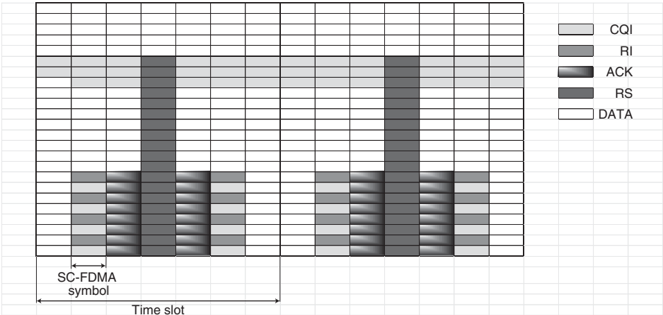
Figure 11.49 Mapping of UCI to PUSCH [19].
