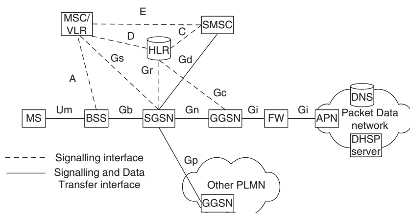
Figure 8.2 GPRS interfaces.
