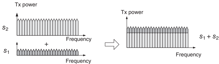
Figure 13.3 Downlink NOMA power allocation.
