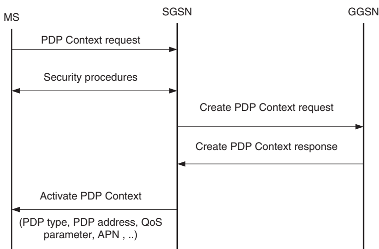
Figure 8.5 PDP context activation procedure.
