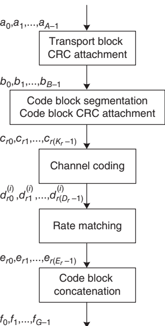
Figure 11.37 Transport block processing for DL-SCH, PCH and MCH channel coding [18].
