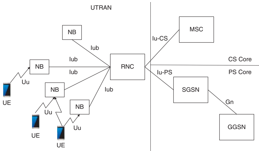
Figure 9.1 UMTS architecture.
