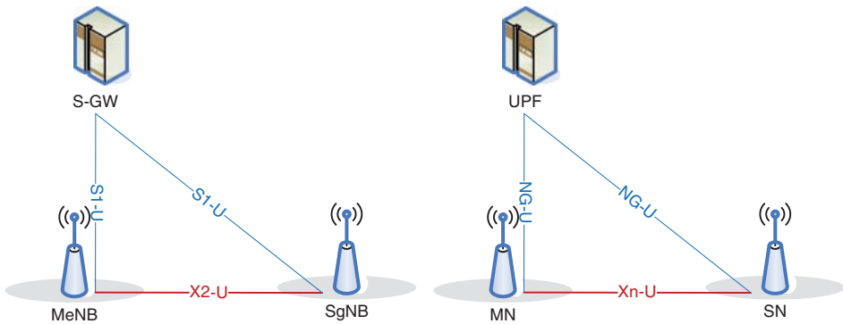
Figure 13.29 U-plane connectivity for EN-DC (left) and MR-DC with 5GC (right) [30].
