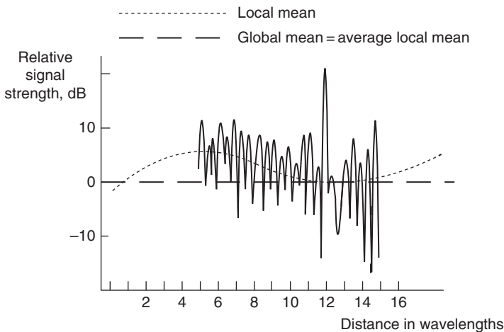
Figure 5.13 Rayleigh fading.
