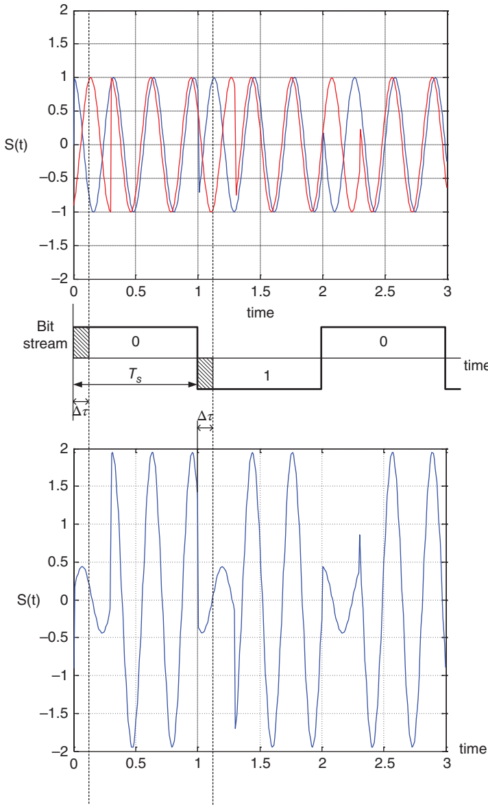
Figure 5.6 Inter-symbol interference.
