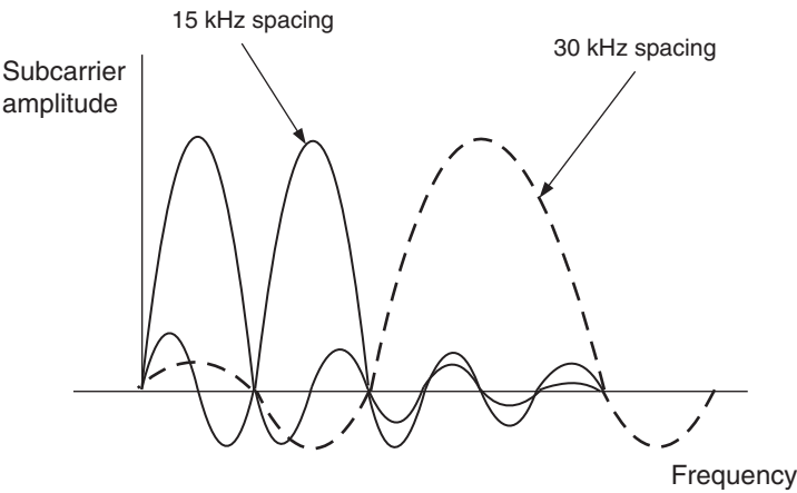
Figure 13.21 Inter-subcarrier interference.
