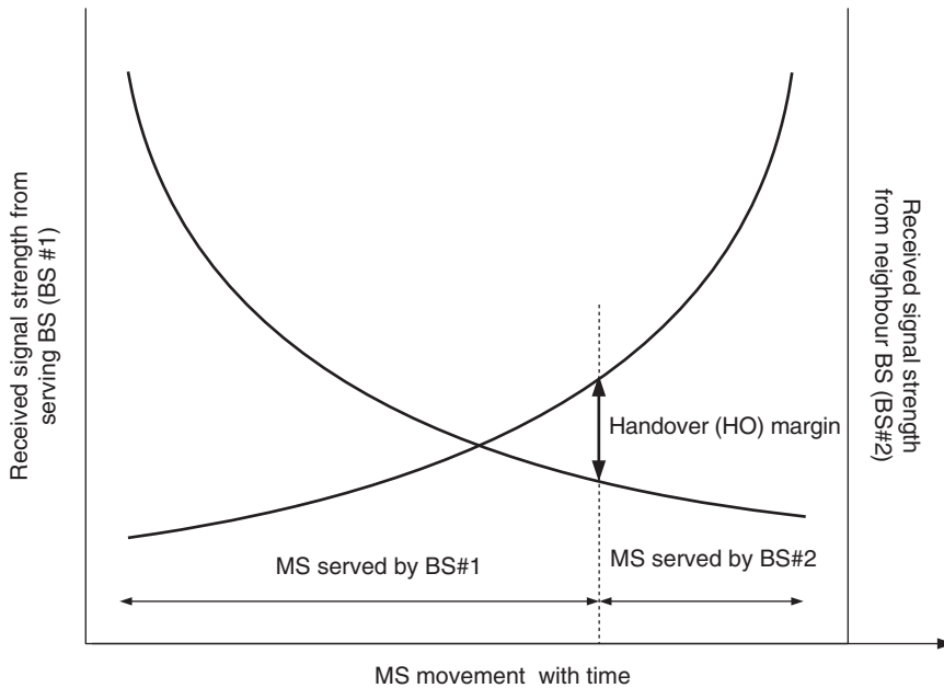
Figure 7.28 Handover decision.
