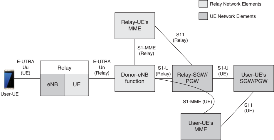
Figure 12.15 Functional entities in relaying architecture [7].
