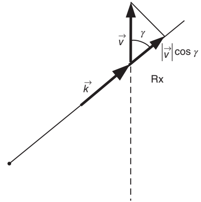
Figure 5.8 Projection of velocity vector |\vec{v}| onto the direction of propagation \vec{k} .
