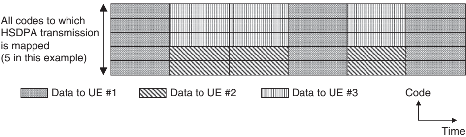
Figure 10.2 Sharing by means of time multiplex as well as code multiplex [1].
