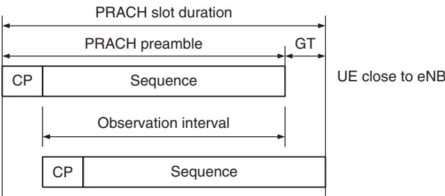
Figure 11.52 Random access with PRACH [16].
