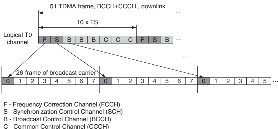
Figure 7.24 Mapping the control channels onto broadcast carrier with signalling over Time Slot 0.
