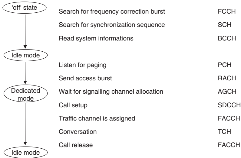
Figure 7.20 Utilization of logical channels during call setup.
