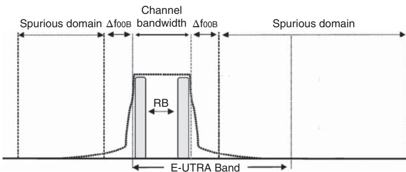
Figure 11.19 Transmitter RF spectrum [13].
