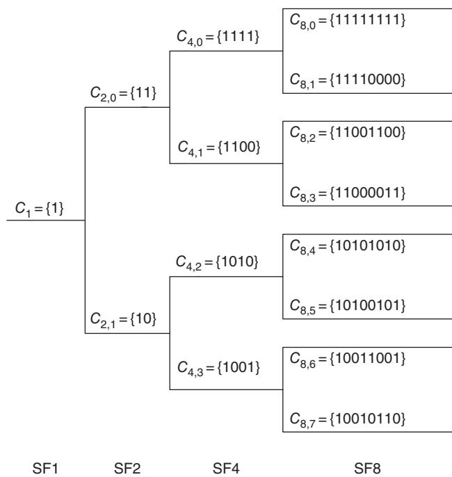
Figure 9.7 OVFS code tree.
