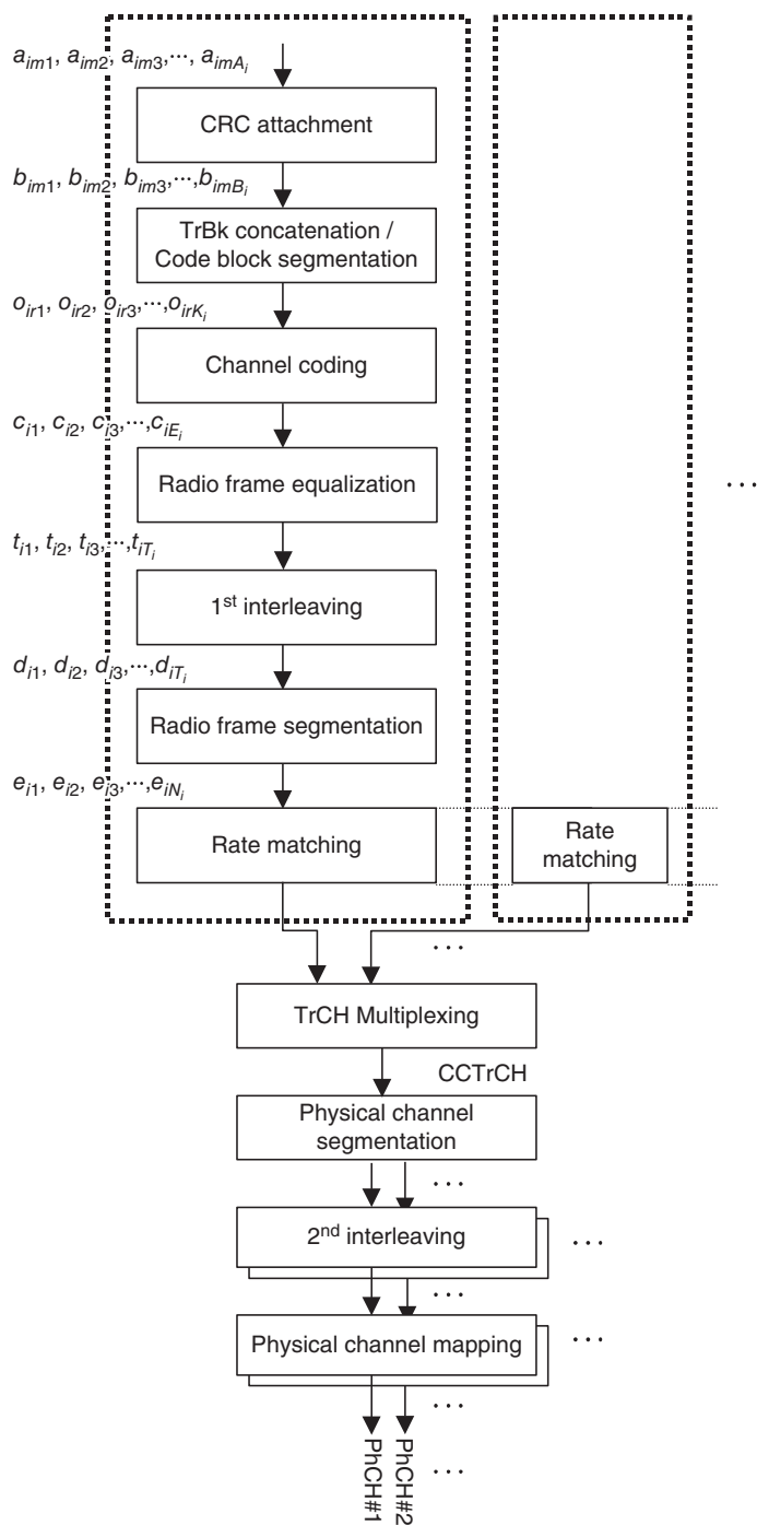
Figure 9.23 Transport channel multiplexing structure for the uplink [11].
