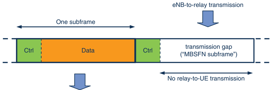
Figure 12.20 Relay Node DL radio frame configuration: normal subframes (left) composed with reference, control signals and user data, and gap in transmission to UE on Uu in declared MBSFN subframes (right). This gap is used for reception of Un by RN from DeNB [8].
