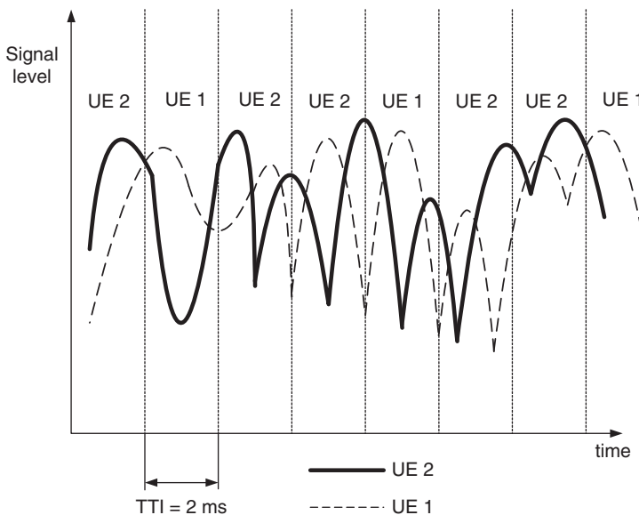
Figure 10.3 Channel-dependent scheduling.
