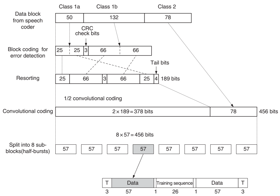
Figure 7.30 Channel coding.
