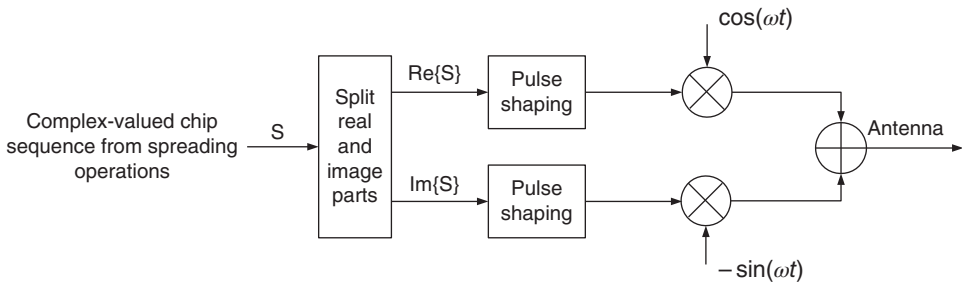
Figure 9.27 Modulation process [14].
