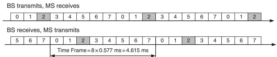
Figure 7.9 Burst schedule at the BS. Time slot 2 is assigned to mobile user.
