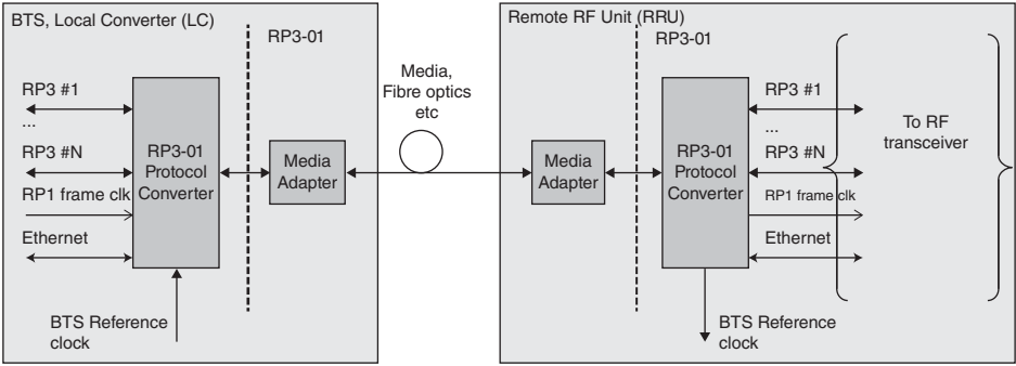
Figure 14.3 Logical structure of RP3-01 interface [3].
