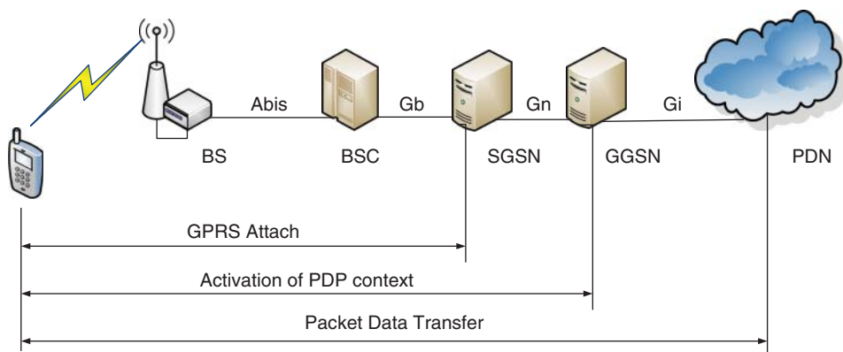
Figure 8.3 GPRS procedures.
