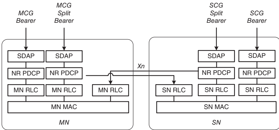
Figure 13.28 Radio Protocol Architecture for MGC, MCG split, SCG and SCG split bearers in MR-DC with 5GC (NGEN-DC, NE-DC) [30].
