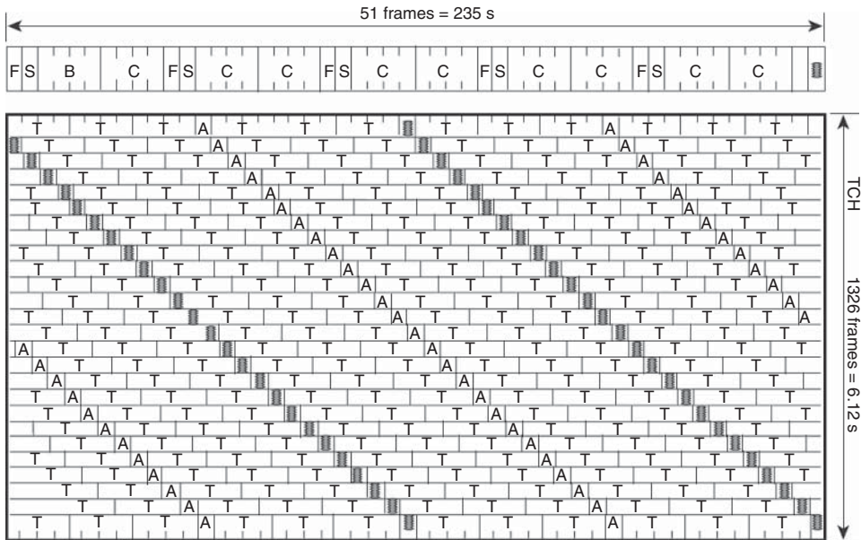
Figure 7.27 Sliding frames [4].
