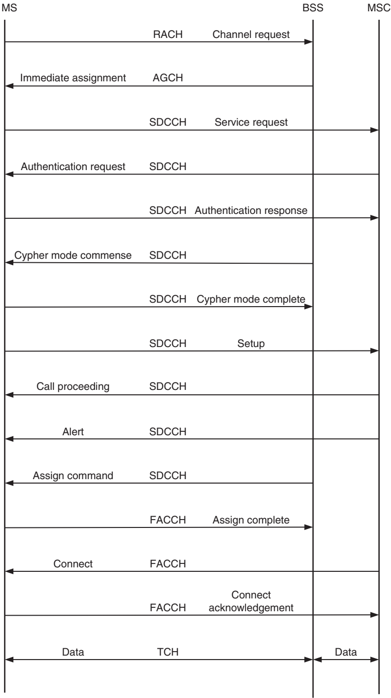
Figure 7.25 Mobile-initiated call setup.
