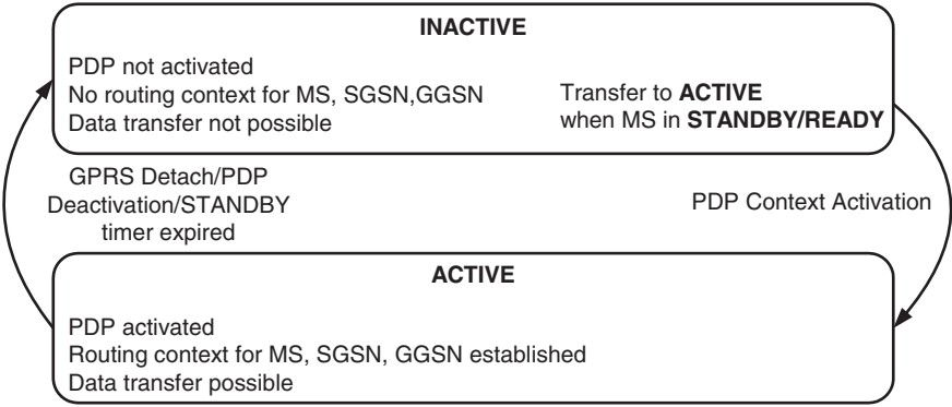
Figure 8.6 PDP states/phases.
