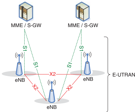
Figure 11.3 E-UTRAN and EPS with S1-flex interface [1].
