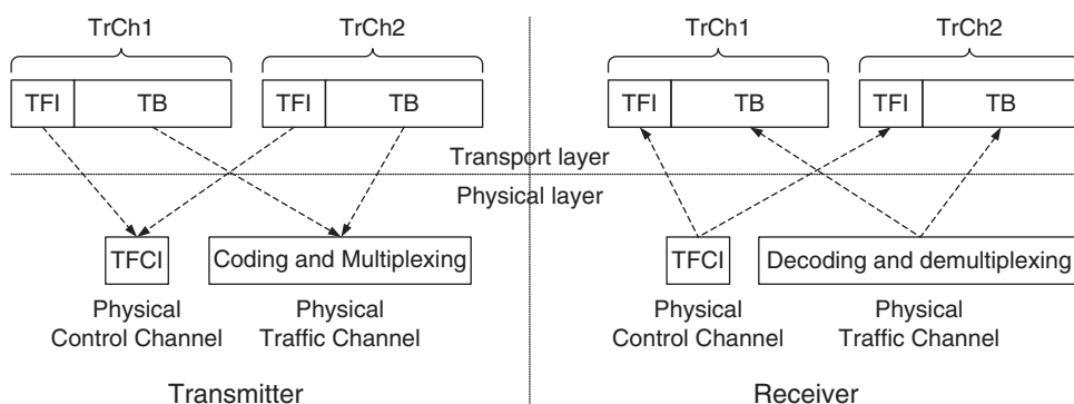
Figure 9.22 Multiplexing the transport channels.
