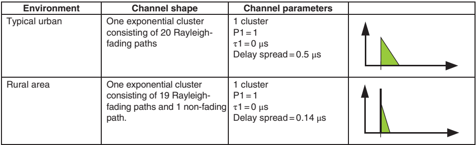
Figure 7.11 The GSM channel models [2].
