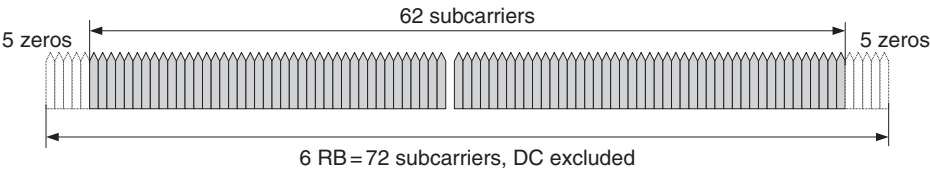
Figure 11.41 Definition and structure of PSS.
