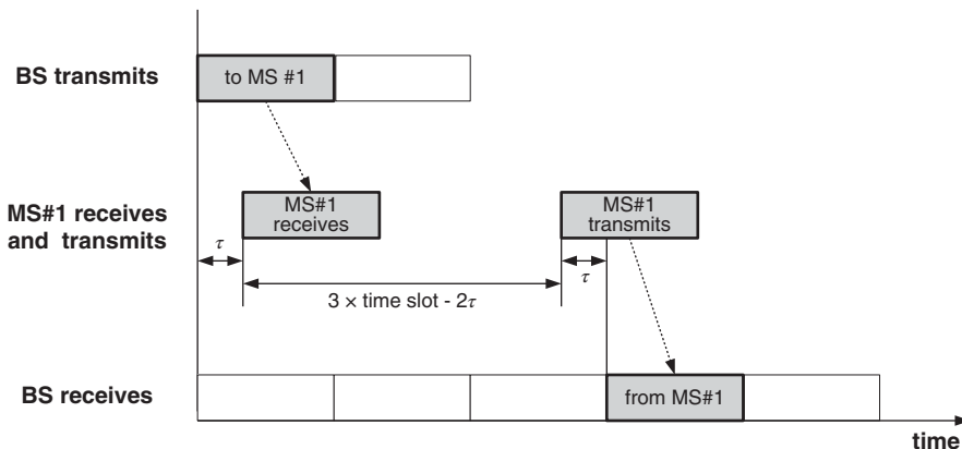
Figure 7.18 Timing alignment.
