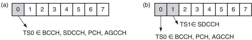
Figure 7.32 SDCCH configuration: (a) combined configuration and (b) separate SDCCH.
