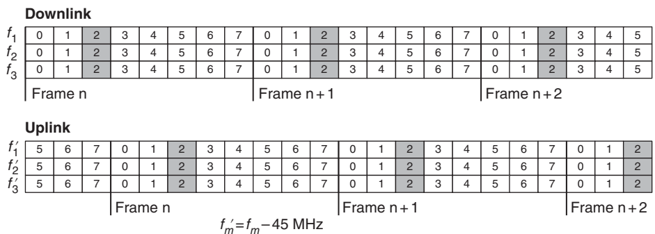
Figure 7.10 Duplex arrangement with three frequency channels allocated to a sector/cell. Total number of available channels is 3 \times 8 = 24 channels.
