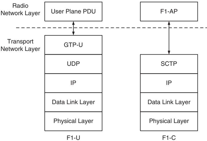
Figure 13.16 Interface protocol structure for F1 [23].
