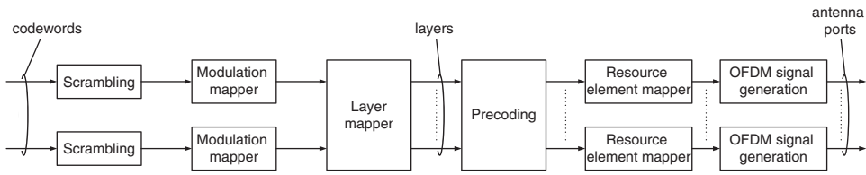
Figure 11.38 Physical-layer processing [16].
