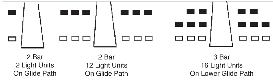
Figure 4-11. Various VASI configurations: dark = red; white = white.
