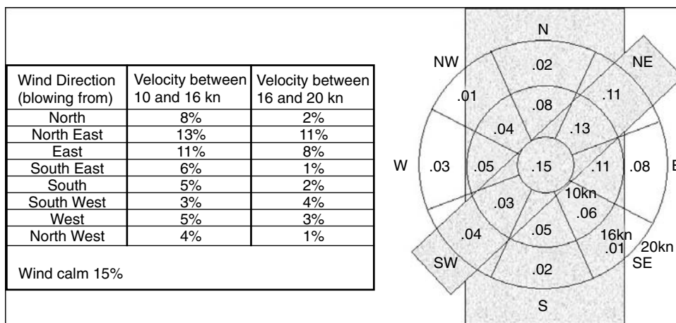
Figure 11-4. Wind rose analysis.
