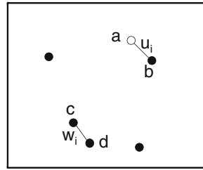
Fig. 11.10. Example of Hopkins statistic. Filled circles represent subjects in a bidimensional space. Open circles represent geometrical points. u_i is the minimal distance between a geometrical point (a) and a subject (b). w_i is the minimal distance between a subject (c) and another subject (d). Both a and c are randomly selected.
