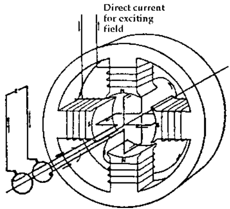
Figure 6-19a. Simple four-pole, single-phase revolving armature generator.
