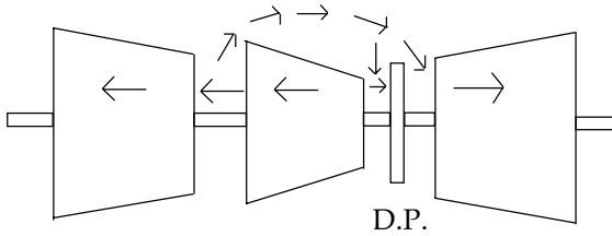
Figure 5-11c. Single-double flow.
