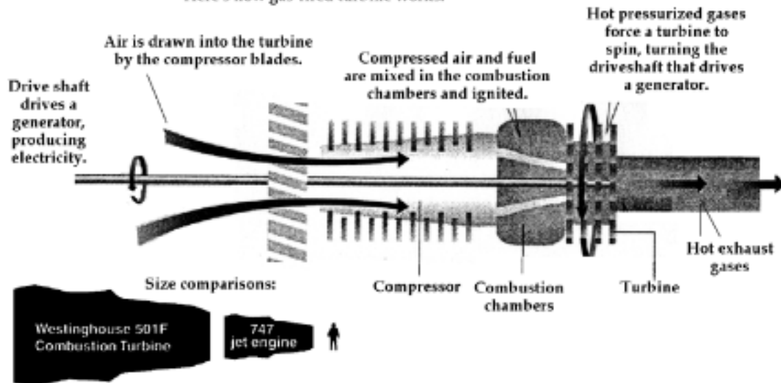
Figure 5-22a. Turbine Engine.
