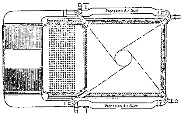
Figure 4-10. Combustion steam generator showing corner-tangential firing.
