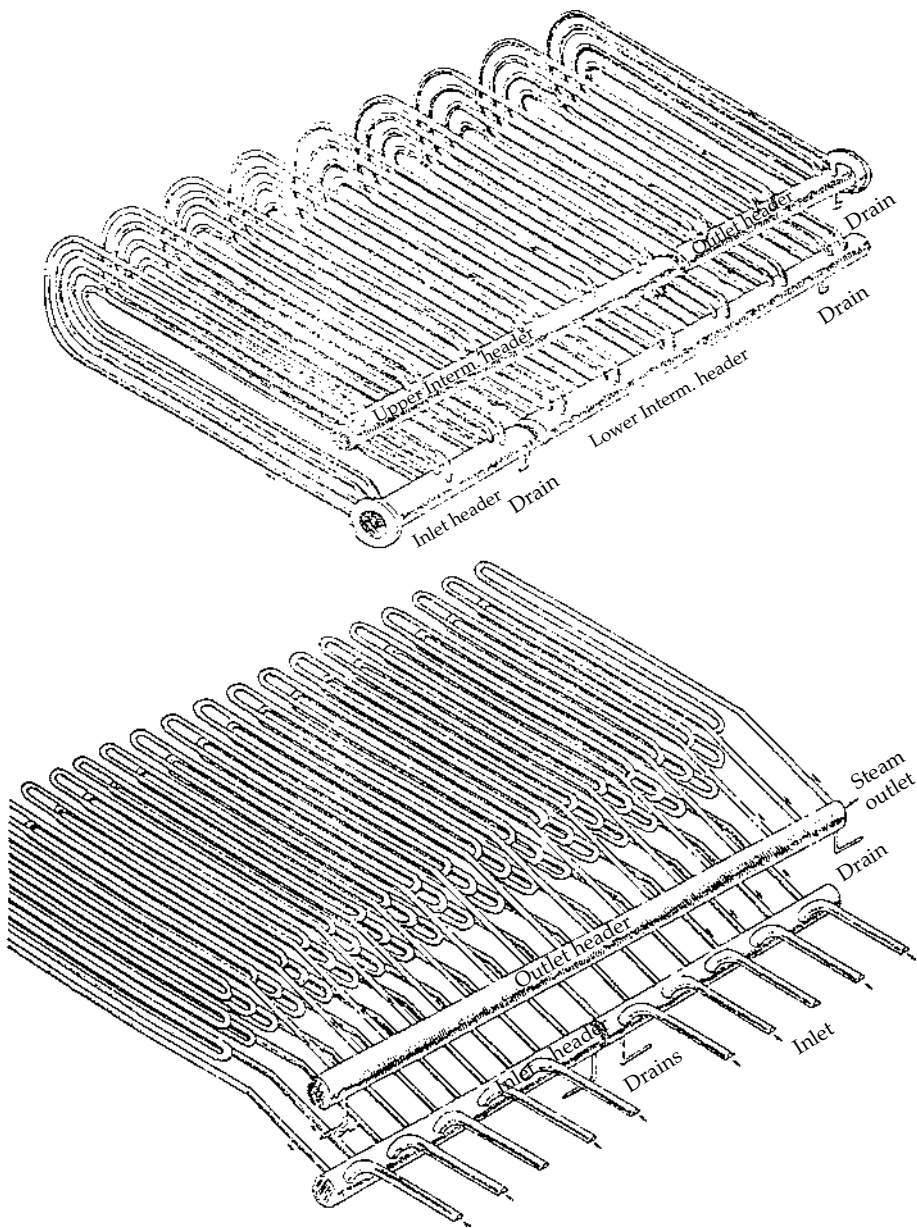
Figure 4-18a. Superheater Tubes.
