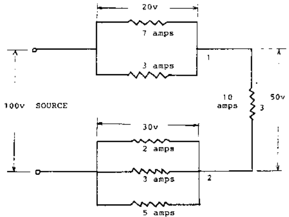
Figure 6-9. Series-parallel circuit.
