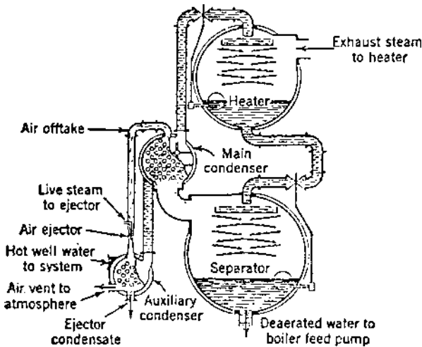
Figure 4-19. Deaerator.
