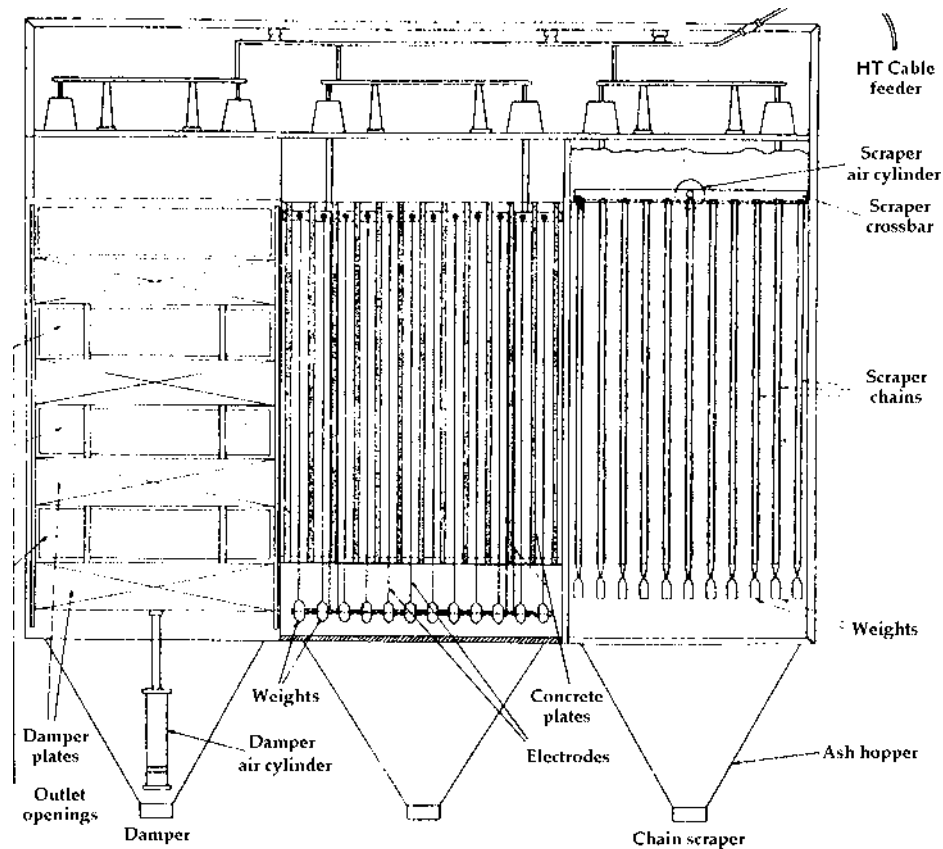
SECTIONS THROUGH PRECIPITATOR Plates and Electrodes
