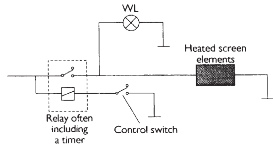
Figure 8.77 Screen heating circuit
