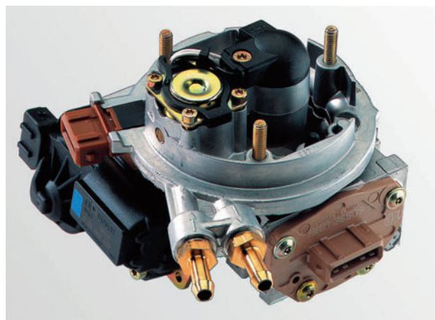
Figure 4.46 Throttle body with a single injector
