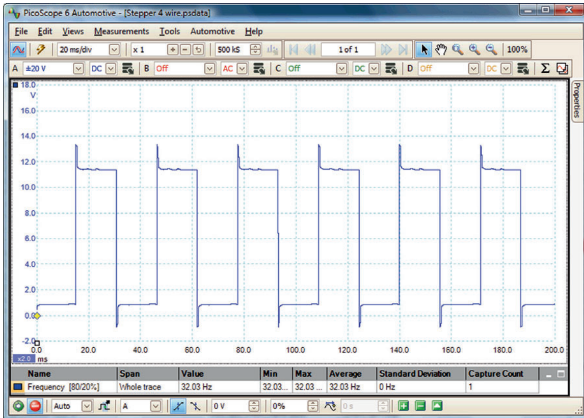
Figure 4.44 Stepper motor signals
