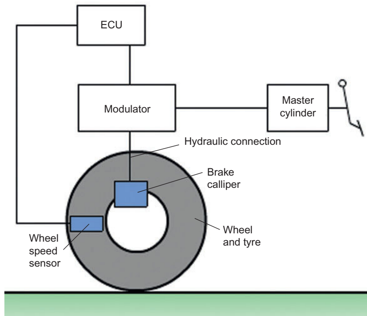
Figure 7.9 ABS closed loop block diagram
