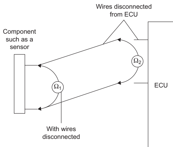
Figure 2.10 Ohmmeter testing
