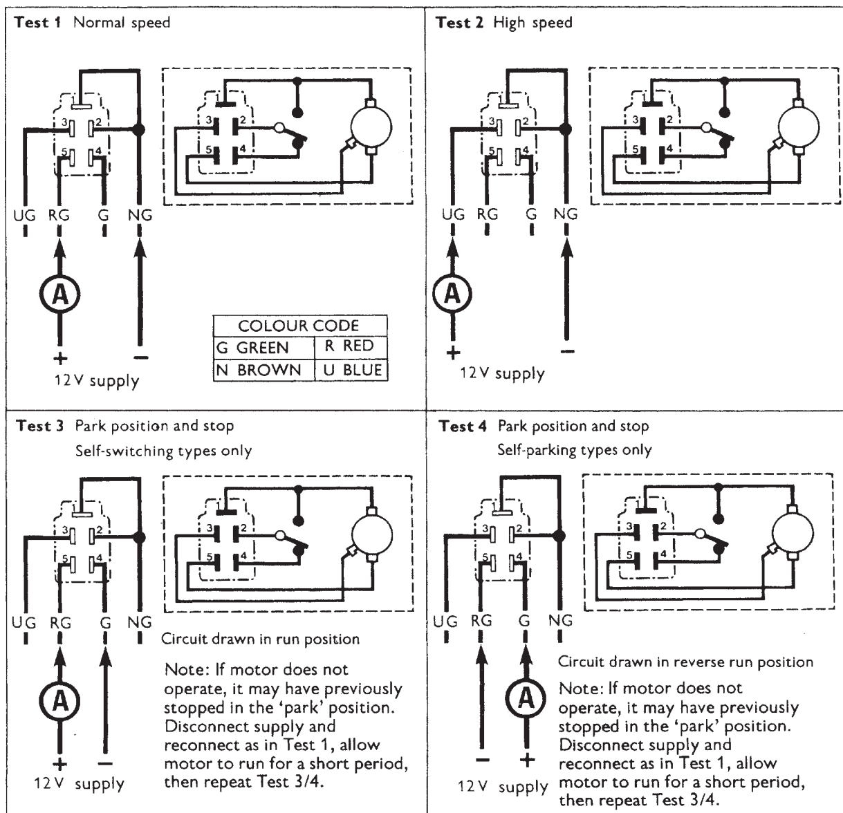
Figure 8.47 Early type wiper motor test procedure
