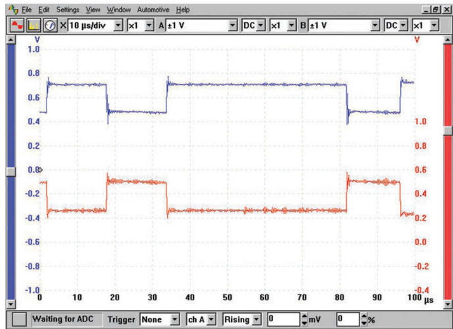
Figure 8.18 CAN signals on a fast timebase
