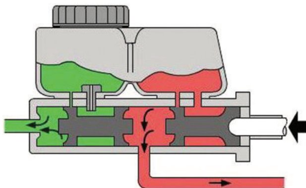
Figure 7.2 Master cylinder operation
