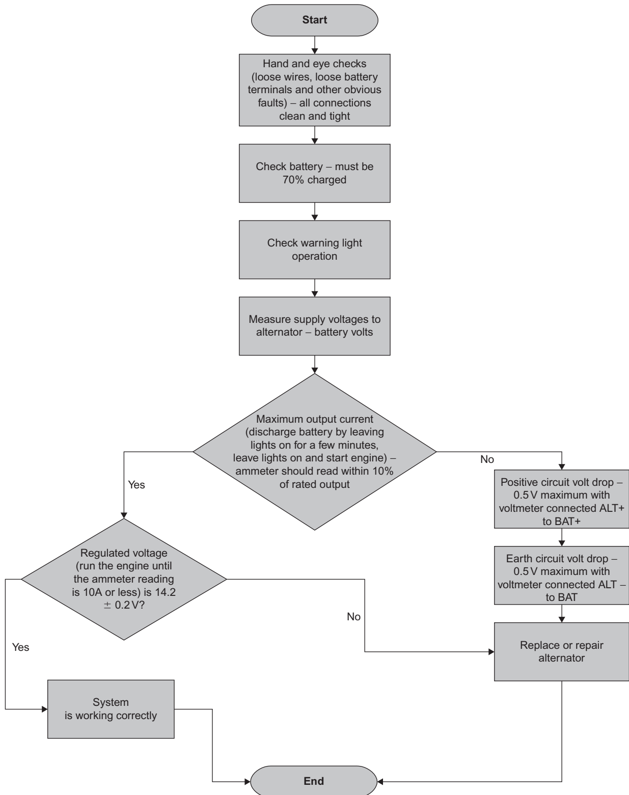
Figure 6.109 Charging system diagnosis chart
