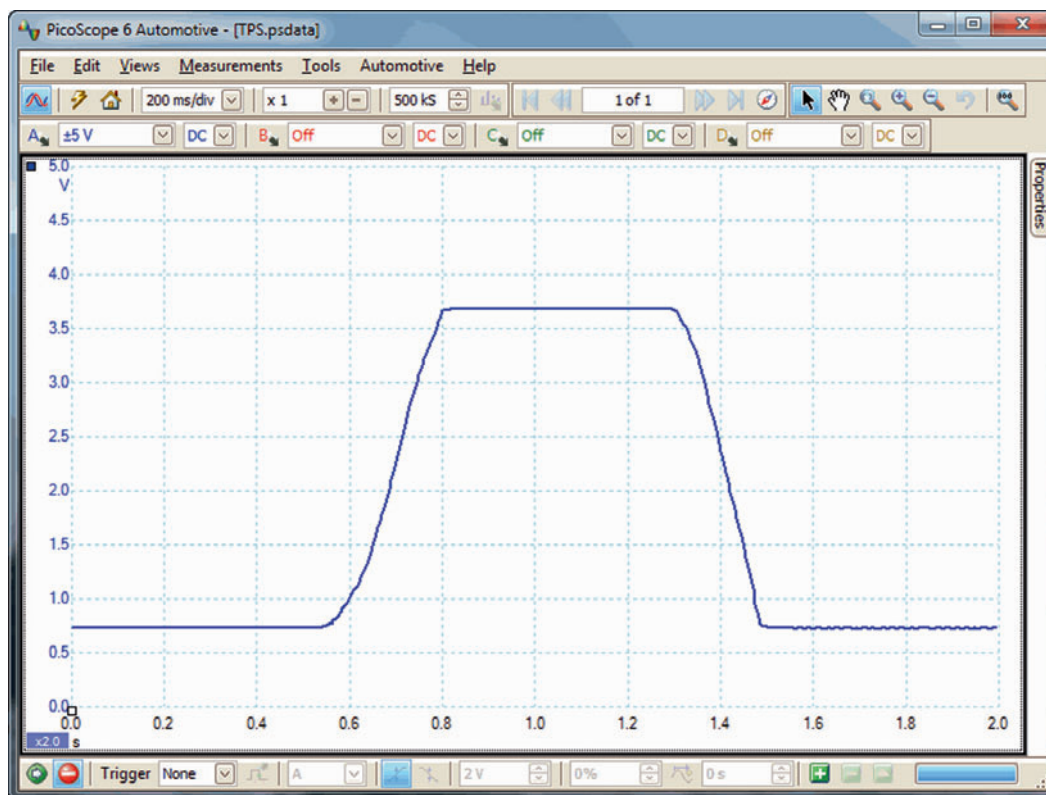
Figure 4.8 Throttle pot output voltage
