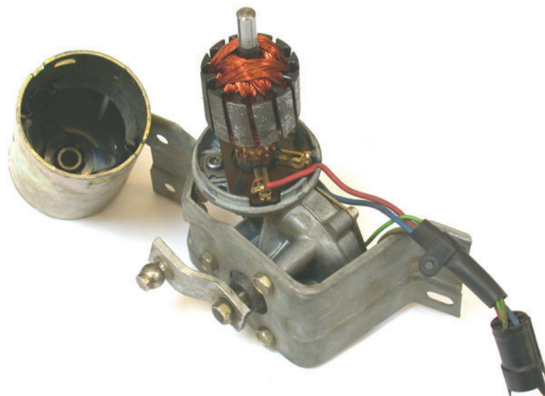
Figure 8.34 Wiper motor using three brushes for two-speed operation
