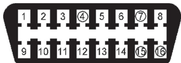
Figure 3.16 Connector pin-out: 4 – battery ground/earth, 7 – K-line, 15 – L-line, 16 – battery positive
