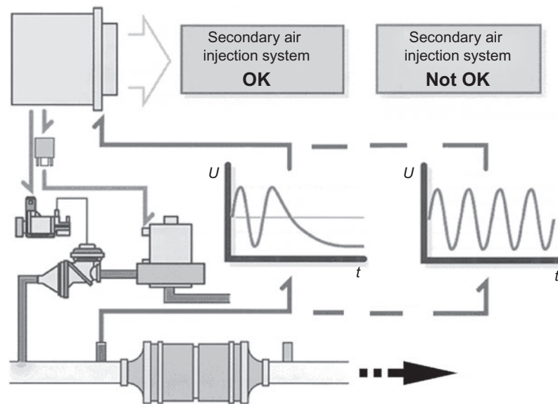
Figure 5.15 Secondary airflow diagnostic monitoring
