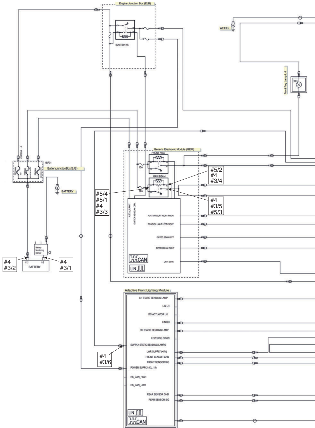
Figure 10.4 (simulation) Supply and earth on the light switch
