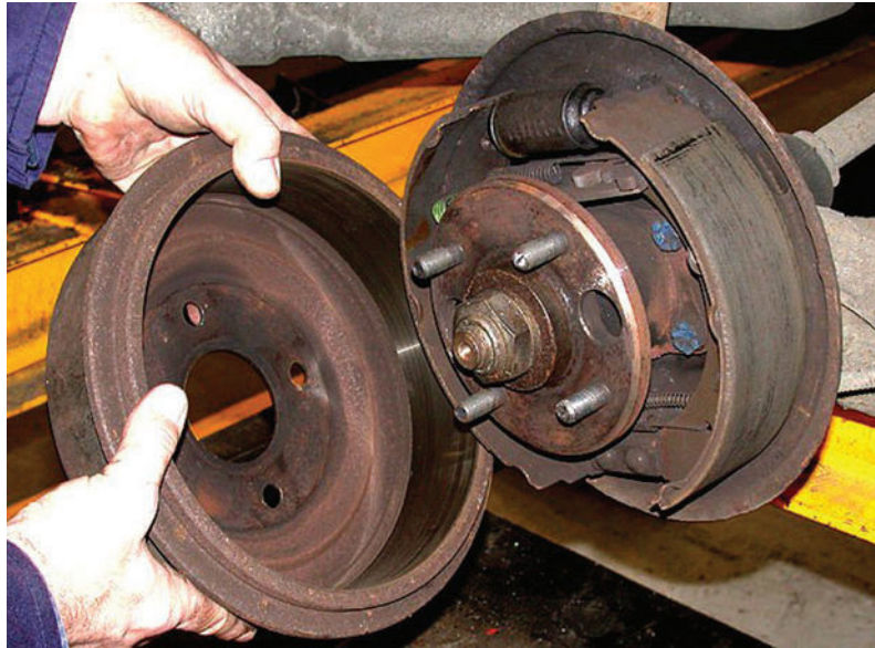
Figure 7.4 Drum brakes showing the shoes and wheel cylinder
