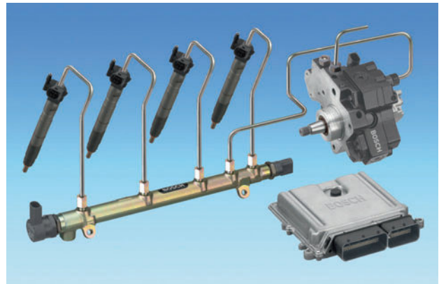
Figure 4.51 Common rail diesel pump, rail, injectors and ECU (Source: Bosch Press)
