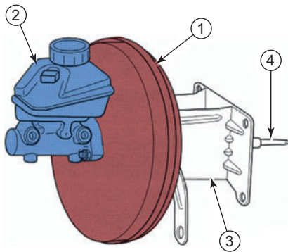
Figure 7.5 Servo unit: 1 – brake servo (booster); 2 – master cylinder and fluid reservoir; 3 – bracket; 4 – diaphragm rod connection to brake pedal
