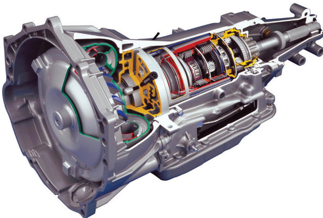
Figure 9.10 RWD automatic gearbox (Source: GM Media)
