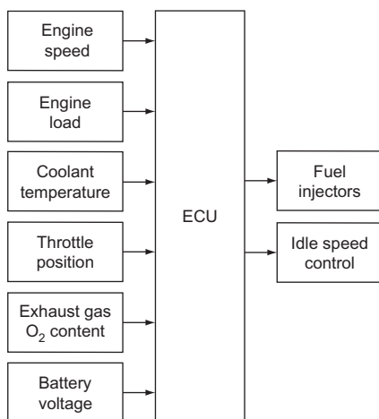
Figure 6.44 Fuel injection simplified block diagram
