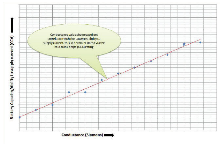
Figure 6.93 Conductance and battery capacity (with respect to the ability to supply large current) have a direct relationship (Source: www.autoelelex.co.uk )
