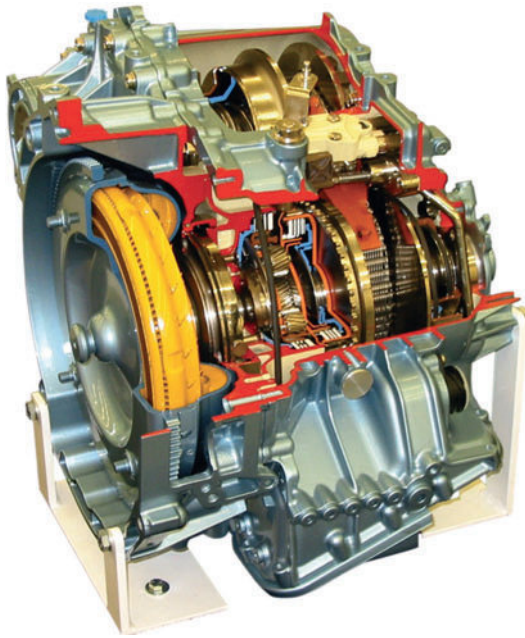
Figure 9.11 Constantly variable transmission (Source: Ford Media)
