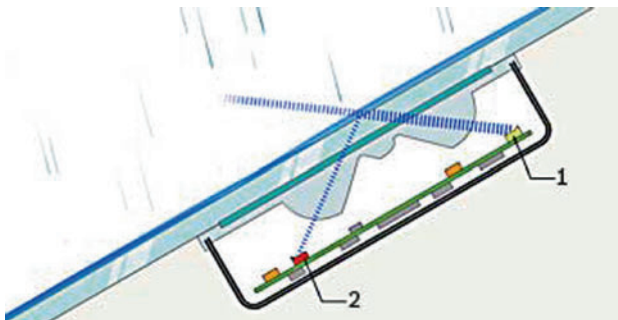
Figure 4.37 Rain sensor principle: 1 – LED; 2 – photo diode
