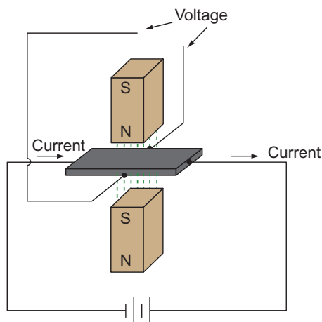
Figure 4.15 Hall effect
