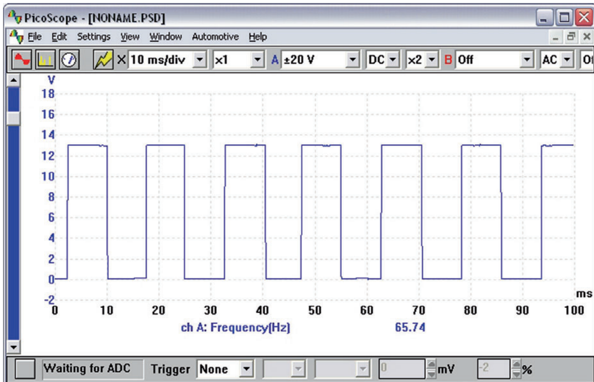
Figure 4.19 Hall effect road speed sensor waveform
