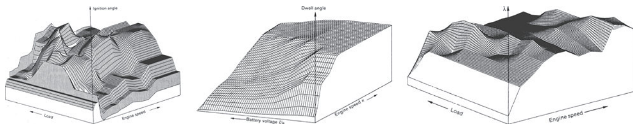
Figure 6.58 Ignition timing, dwell and lambda maps
