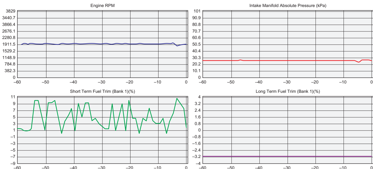
Figure 6.74 Fuel trim – high idle speed. STFT is now positive, LTFT has switched negative. This shows how both work together to achieve the required target of lambda 1
