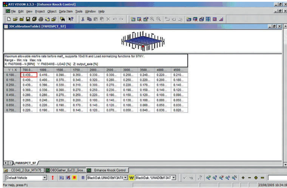
Figure 5.19 System development screen showing type A misfire rates normalised by engine speed and load (Source: Ford Motor Company)
