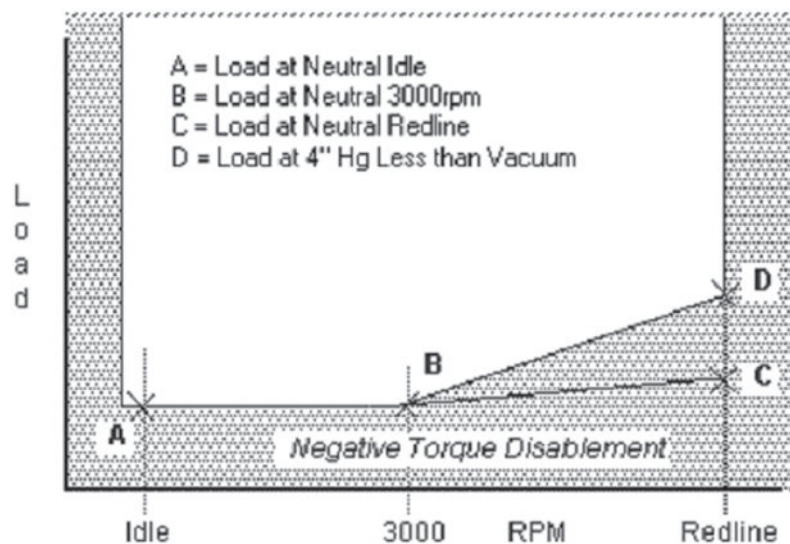
Figure 5.17 Misfire enablement window (Ford Motor Company)
