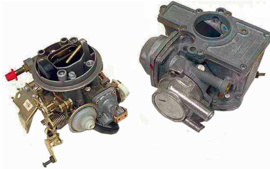
Figure 6.8 Fixed-choke and variable-choke carburetors
