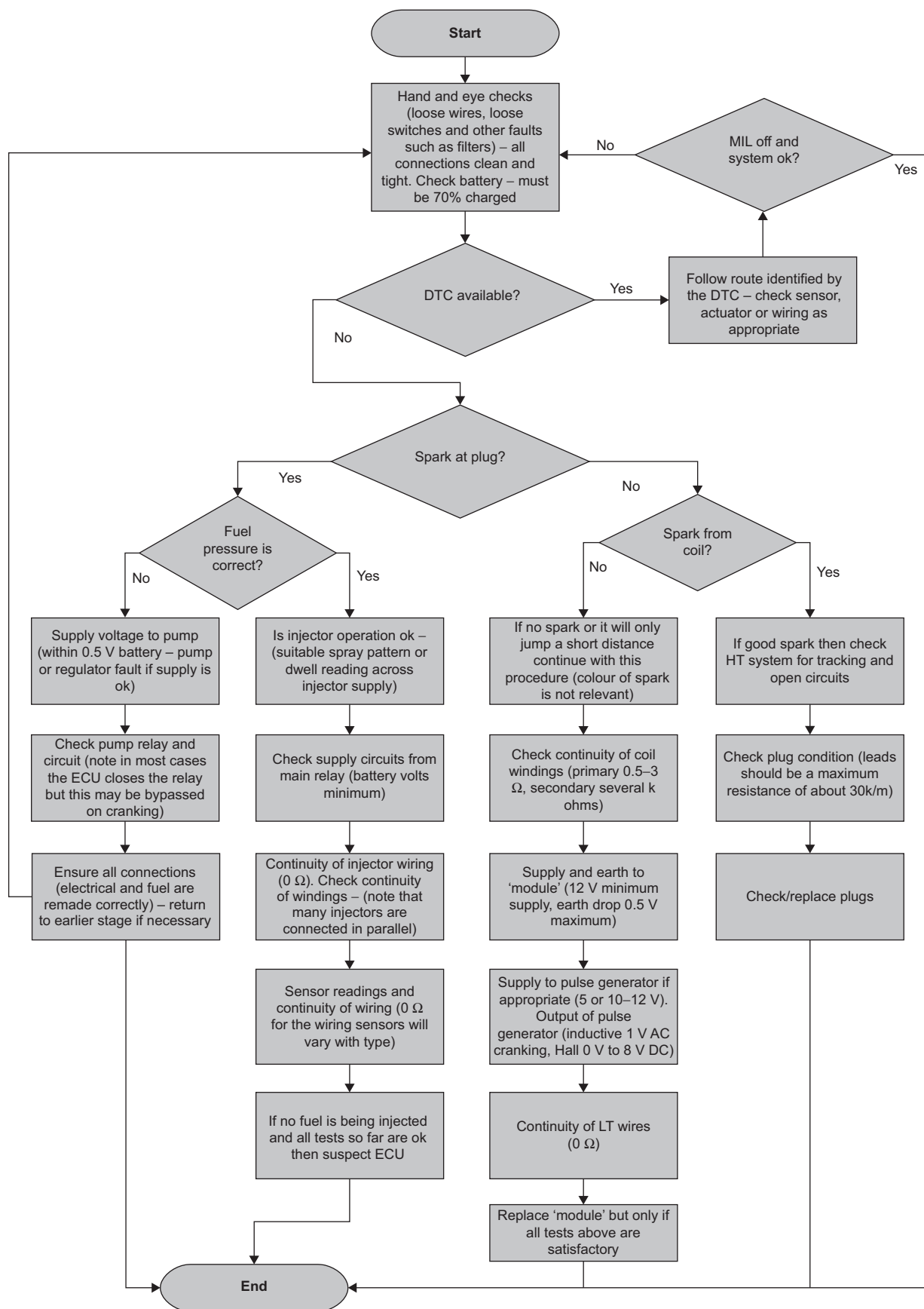
Figure 6.67 Engine management faultfinding chart
