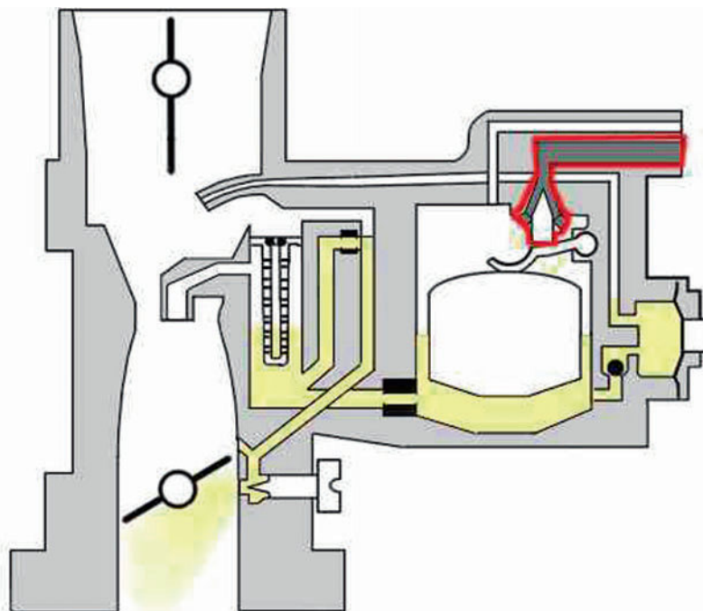
Figure 6.10 Fuel level is controlled by a float and needle valve
