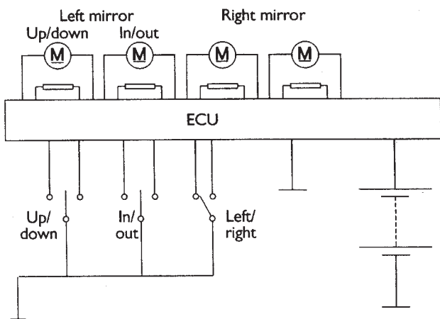
Figure 8.55 Mirror adjustment circuit
