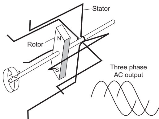
Figure 6.105 Alternator principle
