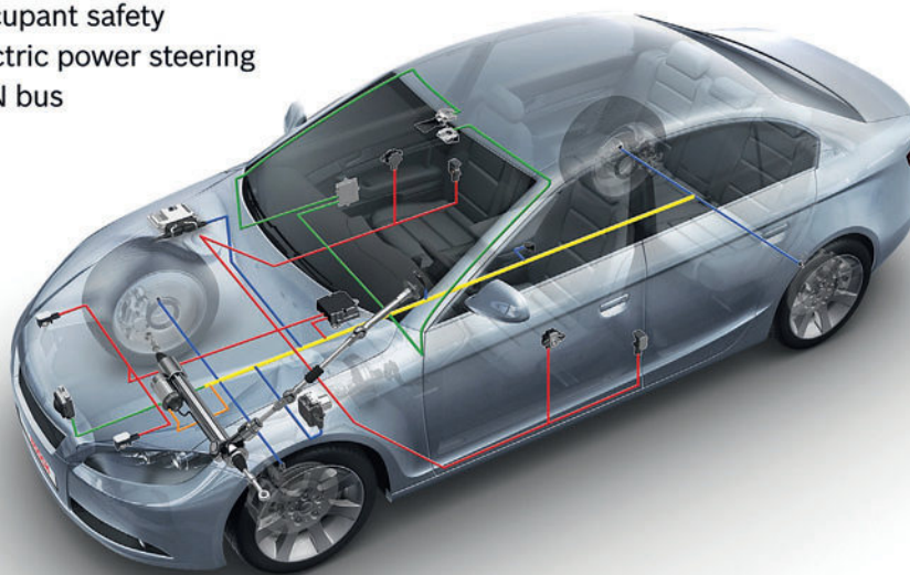
Figure 8.6 A data bus connects all networked components
