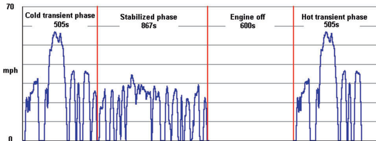
Figure 5.27 US Federal Test Procedure
