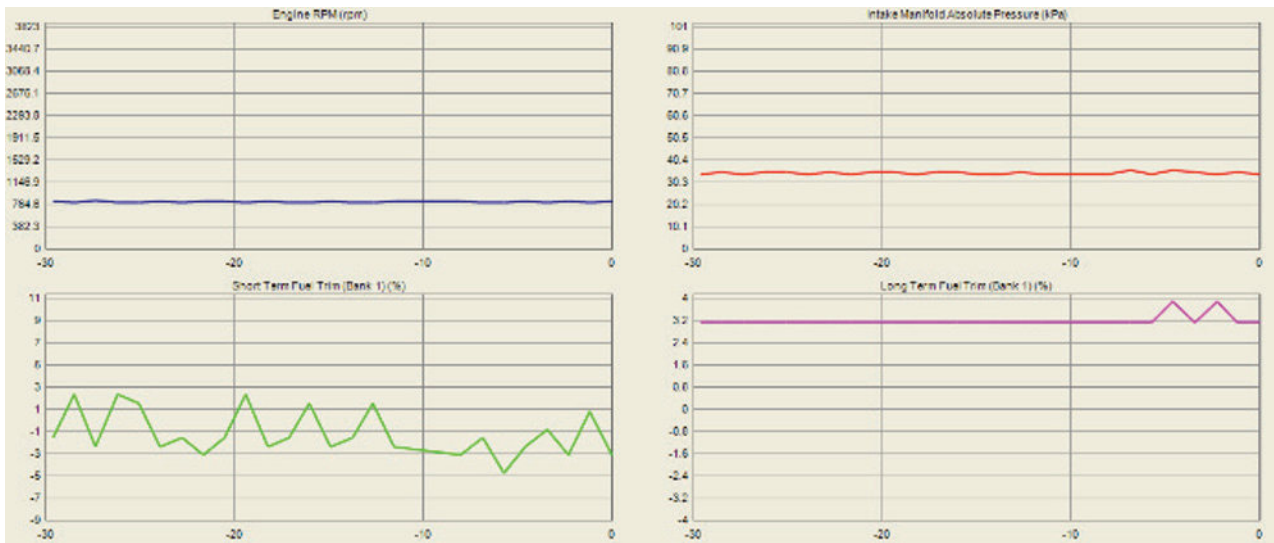
Figure 6.73 Typical fuel trim values at idle, as shown on a standard scan tool, connected to the vehicle OBD connector. Note that STFT is negative and follows closed-loop lambda operation. LTFT is much more stable over time, and is a positive value. Both are within acceptable limits
