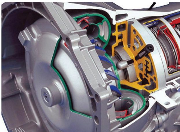
Figure 9.8 Cutaway torque converter (green, red and blue)
