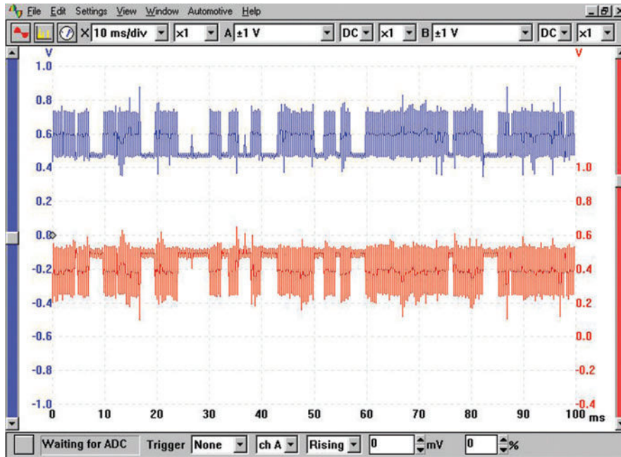
Figure 8.17 CAN signals
