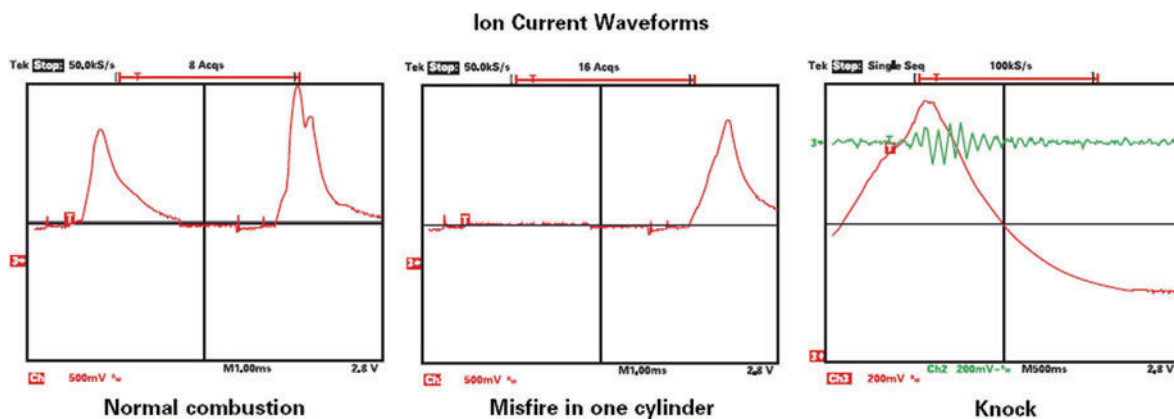
Figure 5.22 Resulting waveforms from the ion-sensing system
