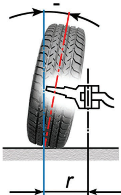
Figure 7.19 Negative camber
