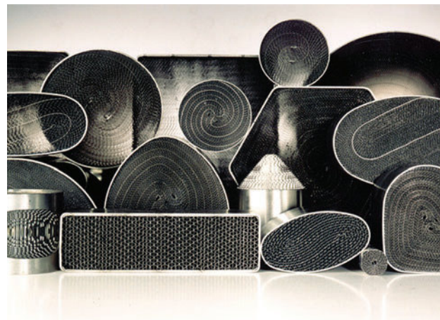
Figure 6.38 Catalytic converter metal substrates
