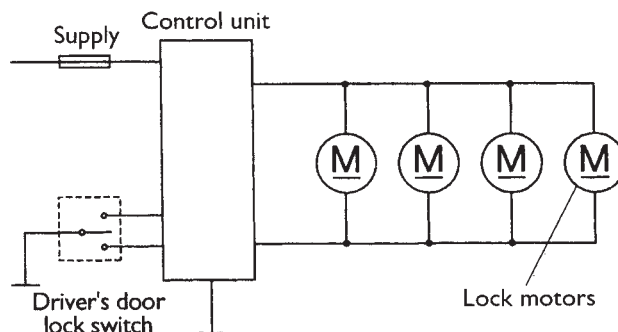
Figure 8.57 Door lock circuit
