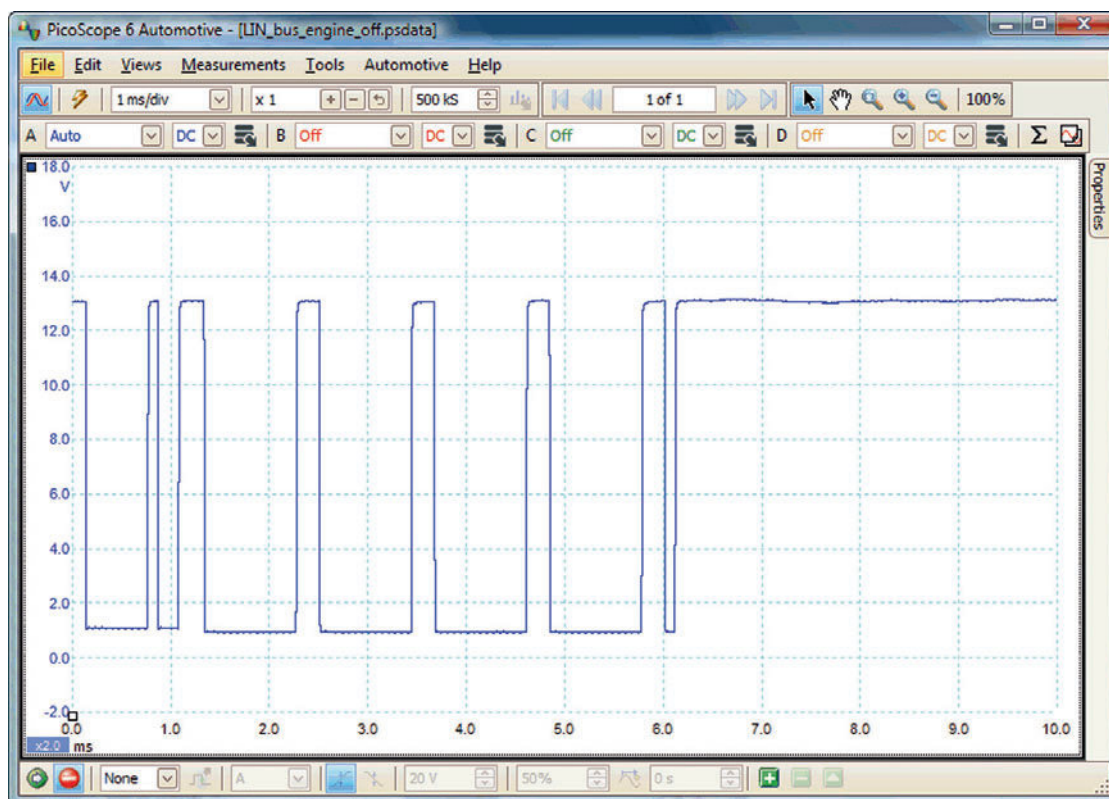
Figure 4.71 LIN waveform
