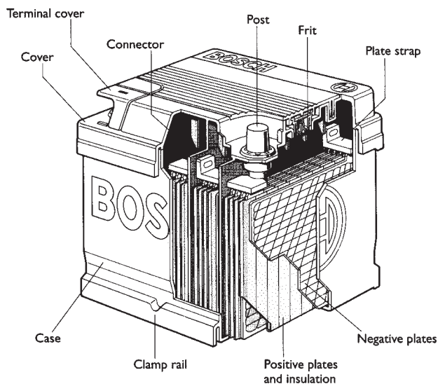
Figure 6.85 Vehicle battery components
