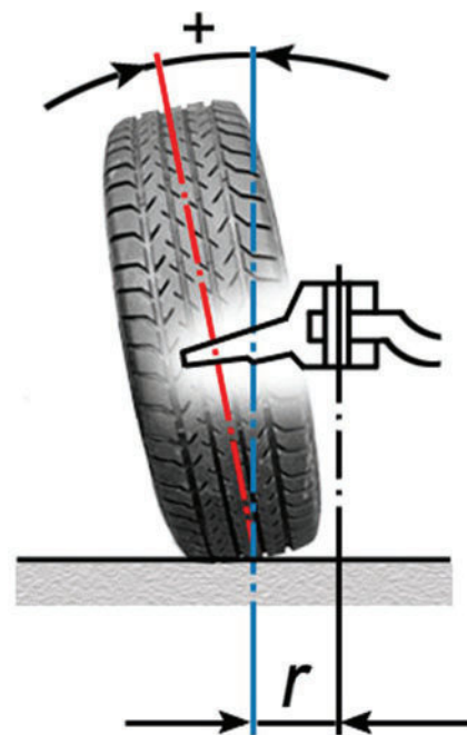
Figure 7.18 Positive camber
