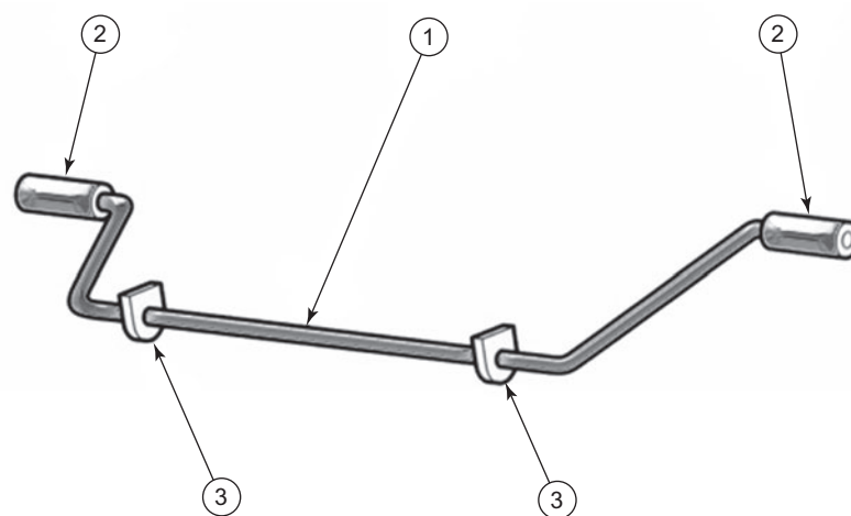
Figure 7.32 Anti-roll bar: 1 – torsion bar; 2 – pivots on suspension lower arms; 3 – fixings to vehicle body
