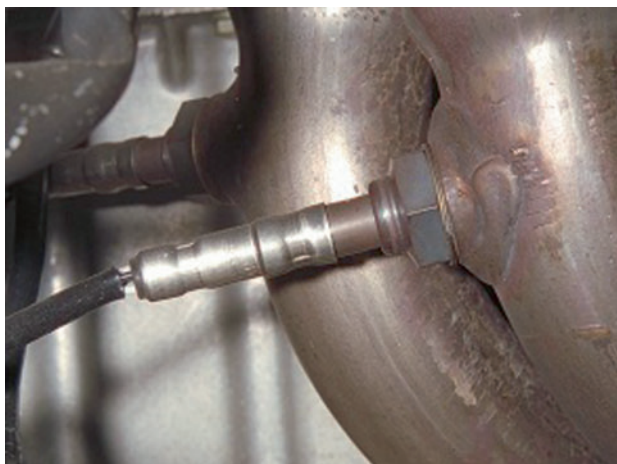
Figure 4.22 Lambda sensor in the exhaust downpipe
