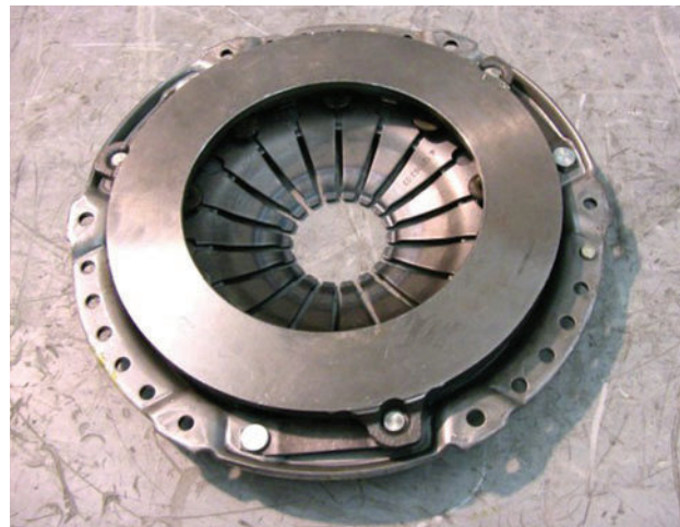
Figure 9.1 Clutch cover and pressure plate
