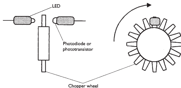
Figure 4.34 Optical sensor
