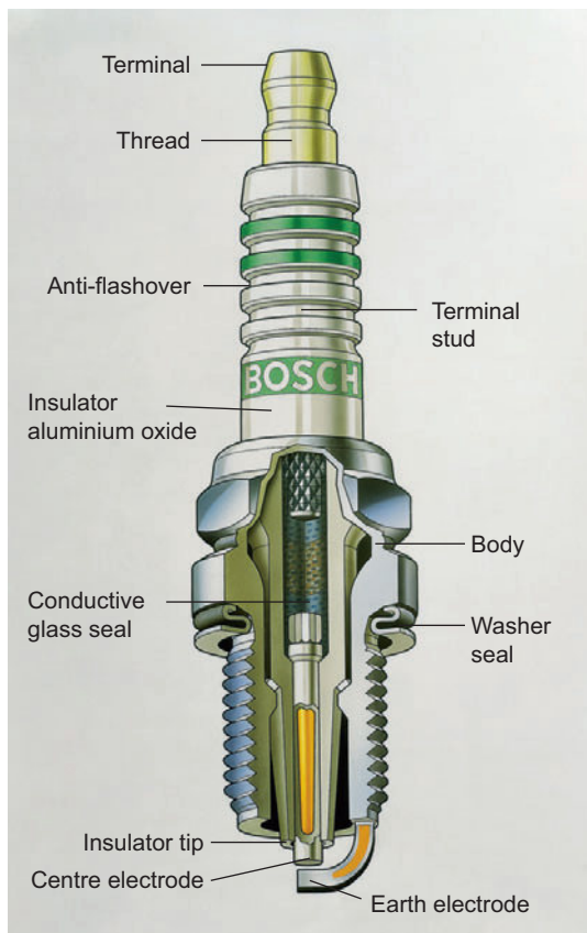
Figure 6.27 Construction of a copper-cored spark plug
