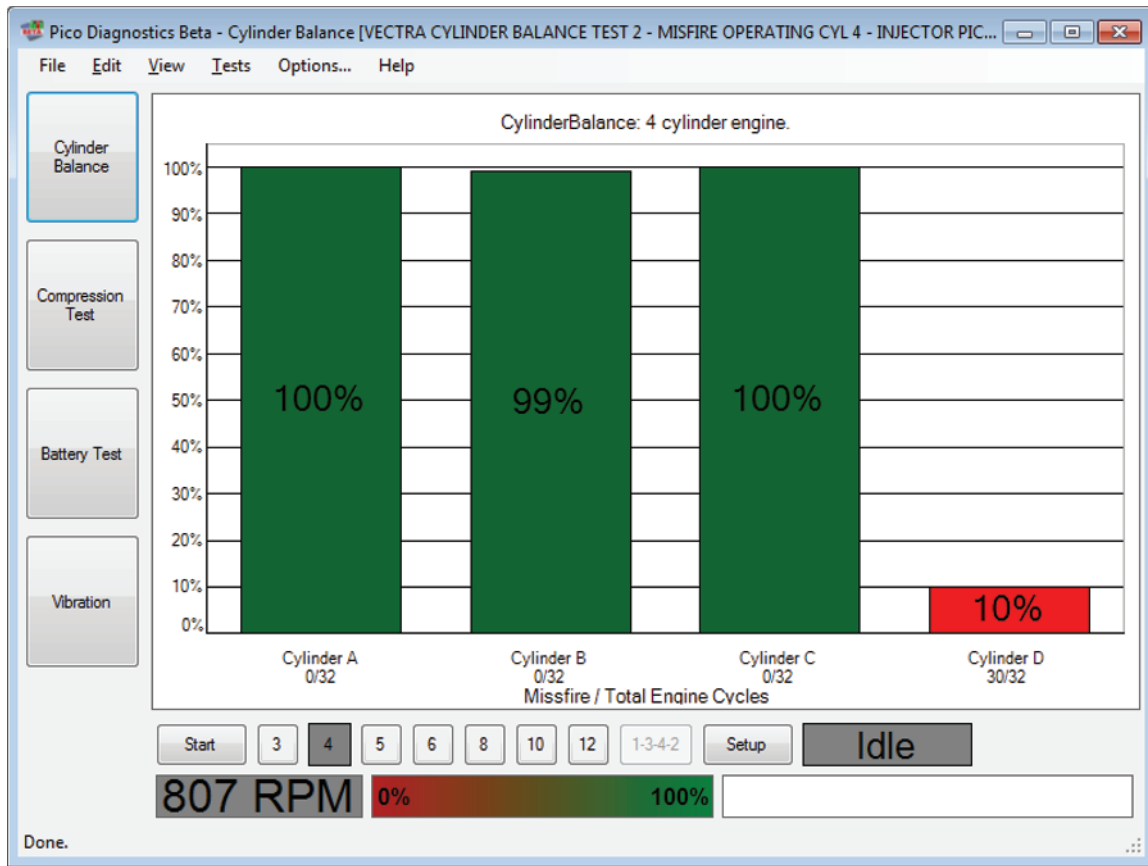
Figure 3.12 Cylinder balance
