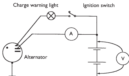
Figure 6.110 Alternator circuit testing
