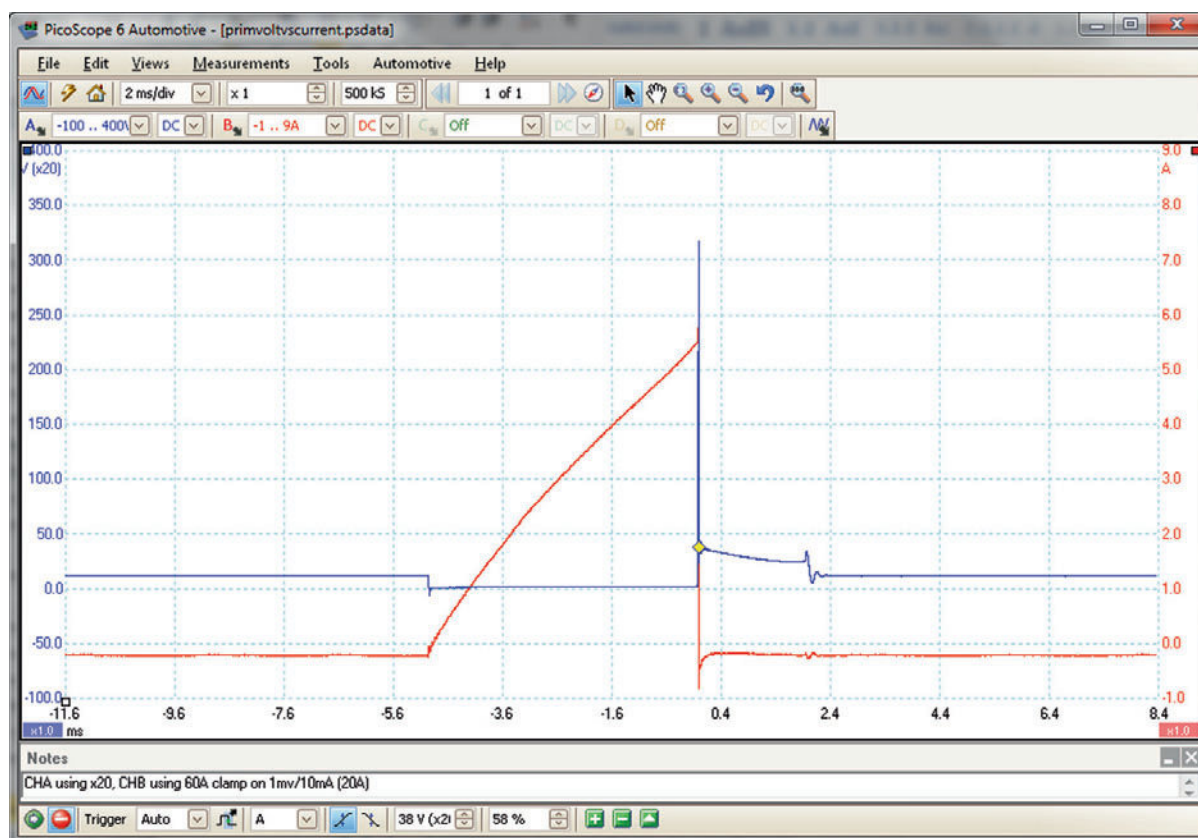
Figure 4.59 Primary ignition voltage and current traces
