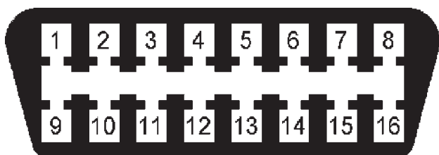
Figure 5.7 Sixteen pin DLC OBD2/EOBD connector
