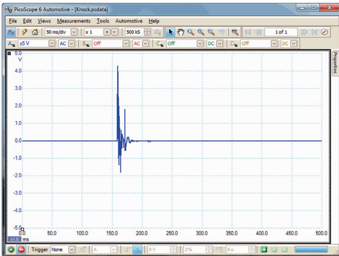
Figure 4.21 Knock sensor output signal
