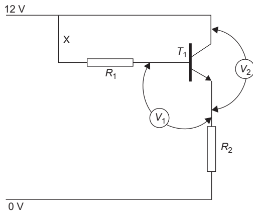
Figure 8.4 Transistor testing: Use resistors R_1 = R_2 of approximately 1 k \Omega , when connected as shown, V_1 should read 0.6–0.7V and V_2 approximately 1V. Disconnect wire X, V_1 should now read 0V and V_2 12V
