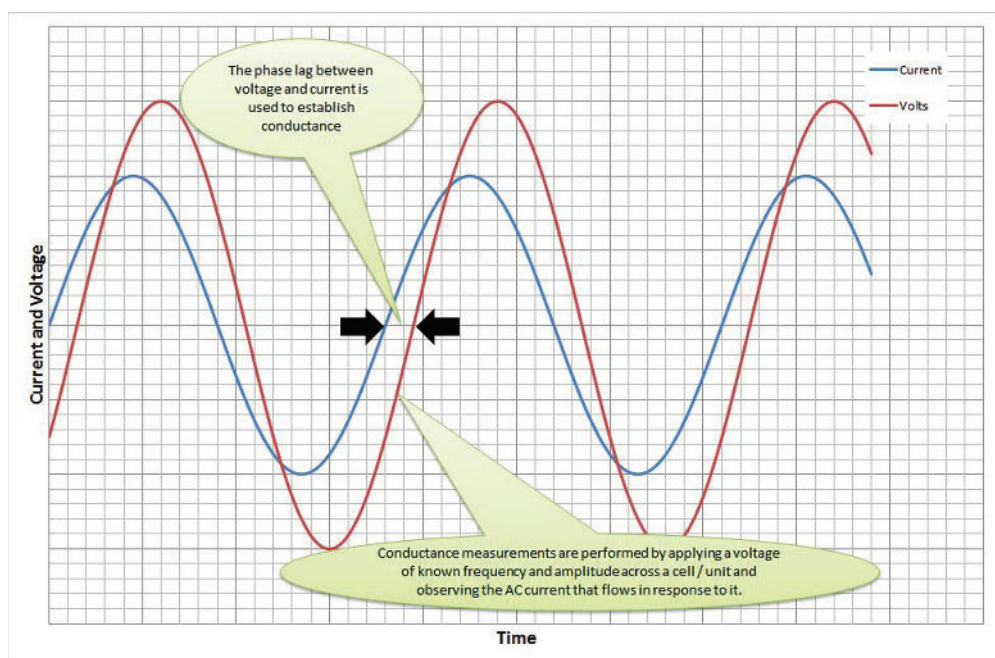
Figure 6.92 AC voltage across the DC battery allows a measurement of the battery's conducting capability to be made (Source: www.autoelex.co.uk )
