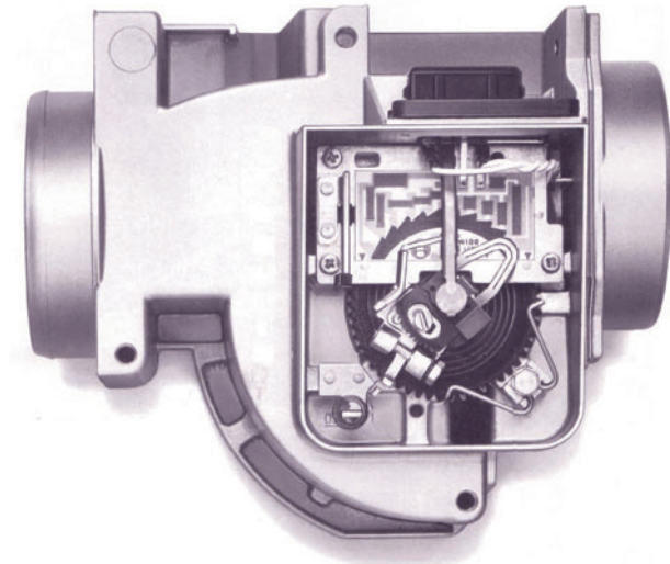
Figure 4.9 Vane- or flap-type airflow sensor (Source: Bosch)
