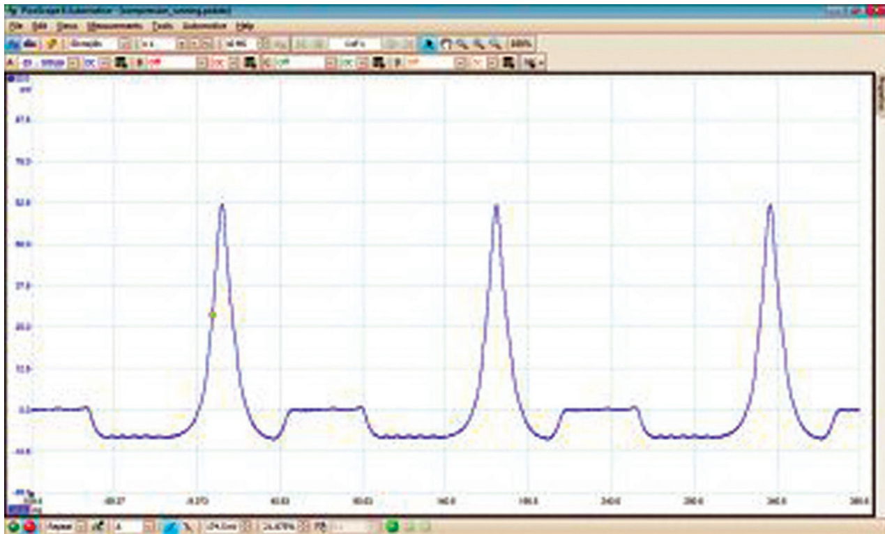
Figure 3.43 Running compression waveform
