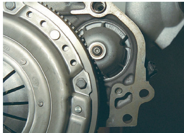
Figure 4.66 Starter and ring gear
