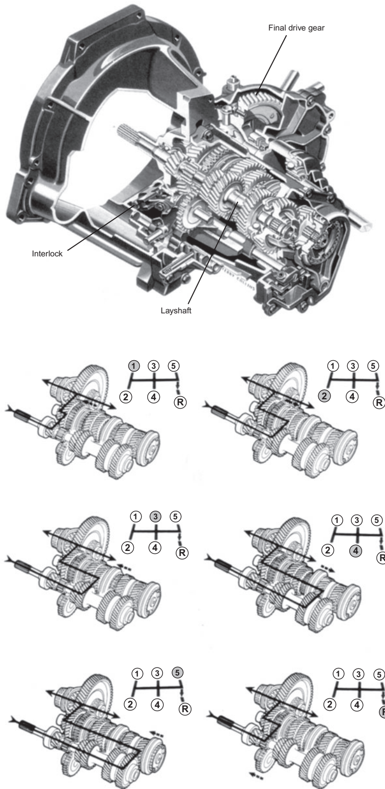
Figure 9.4 Five-speed manual gearbox and power flows
