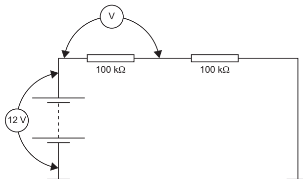
Figure 3.2 Loading effect of a meter
