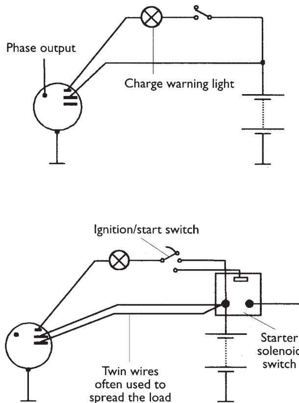
Figure 6.108 Example charging circuits
