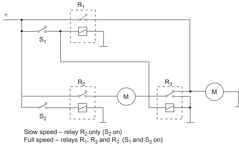
Figure 8.43 Two-speed, twin cooling fan circuit
