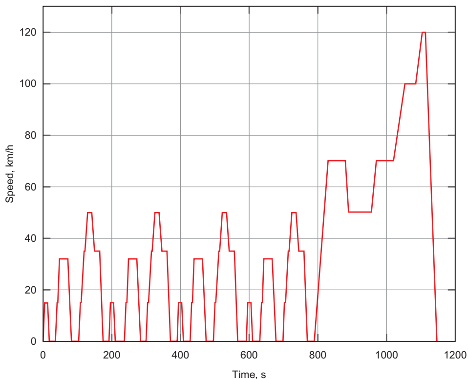
Figure 5.26 Modified New European Driving Cycle (MNEDC)
