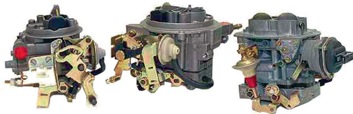
Figure 6.7 Single-choke and twin-choke carburetors
