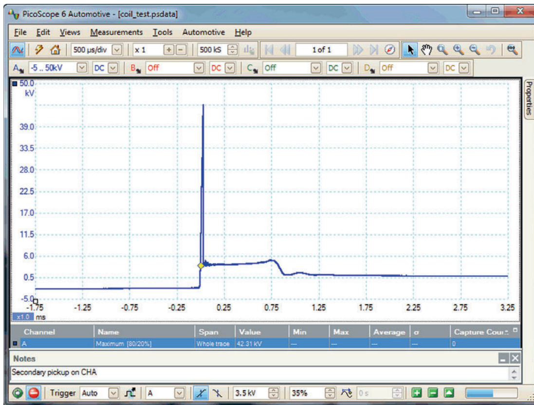
Figure 4.61 Ignition secondary trace
