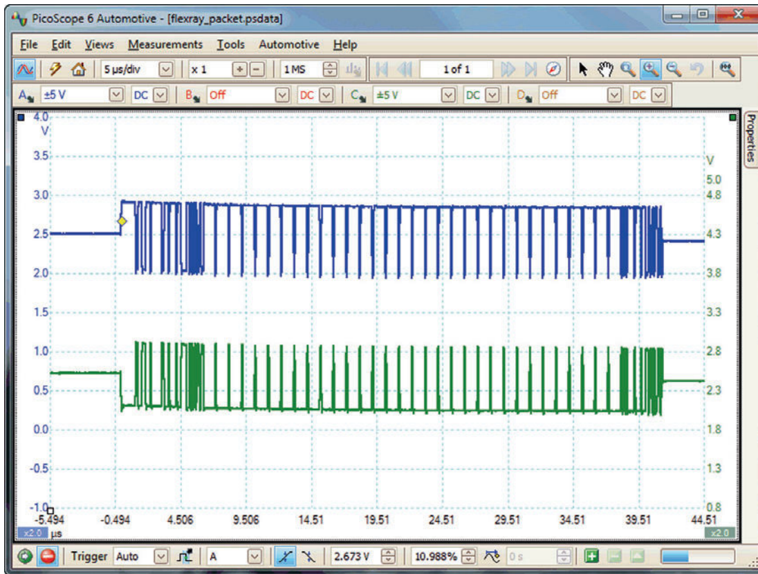
Figure 4.72 FlexRay signal
