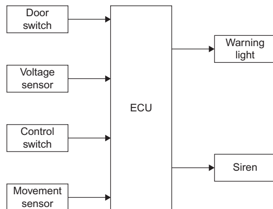
Figure 2.16 Block diagram
