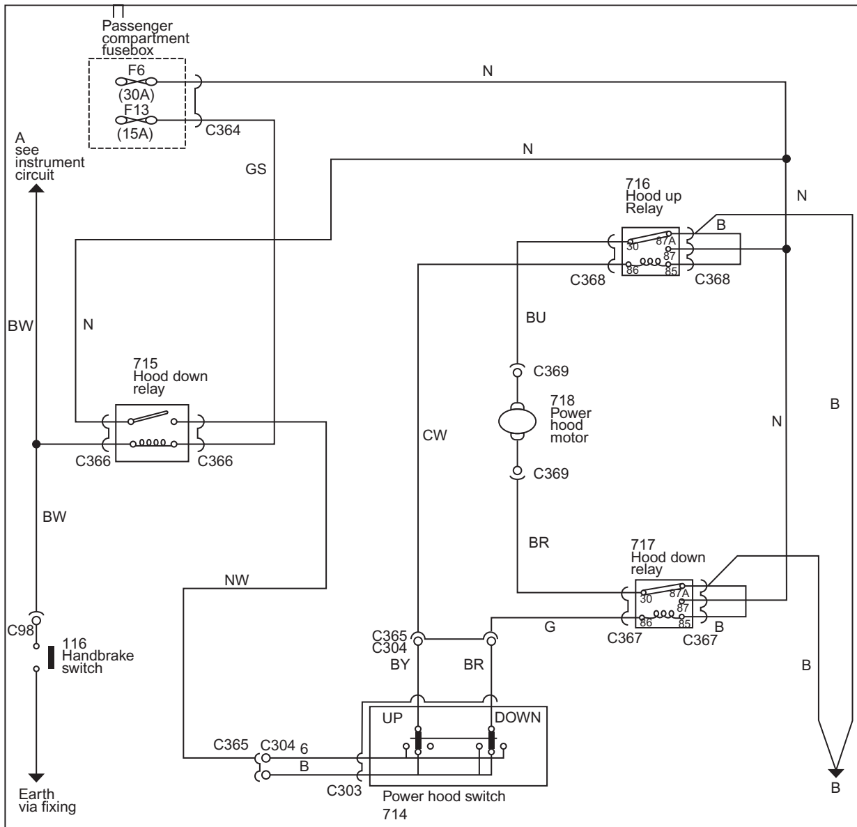
Figure 8.60 Power hood (roof) circuit
