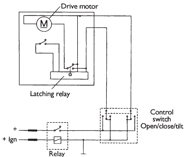
Figure 8.56 Sunroof circuit example
