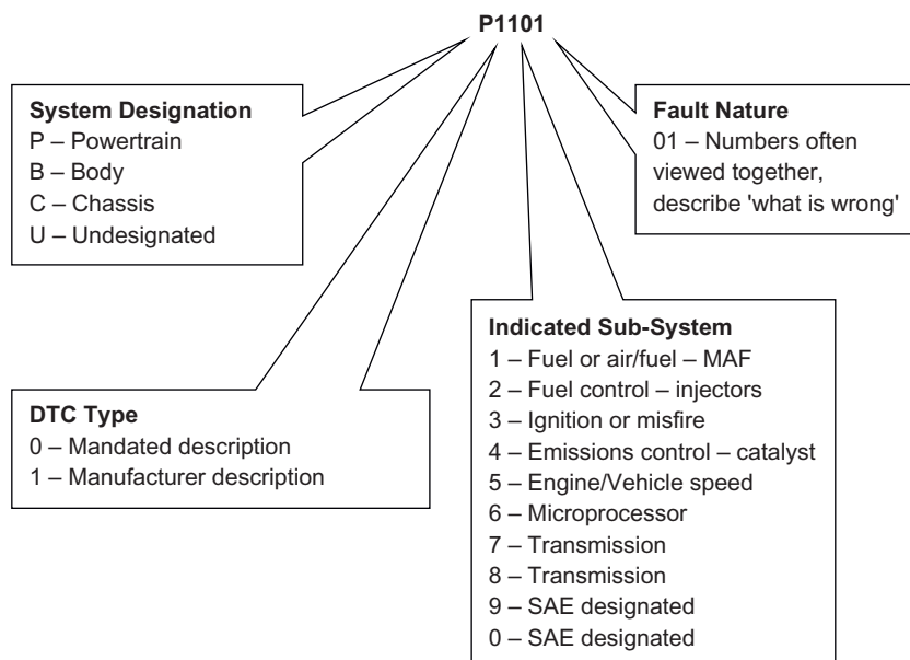
Figure 5.6 P-code composition
