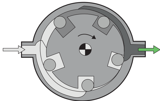
Figure 6.61 Roller cell pump (2)
