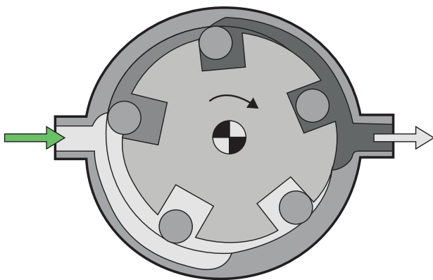
Figure 6.60 Roller cell pump (1)
