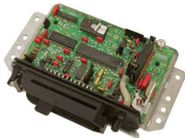
Figure 6.45 Engine management ECU
