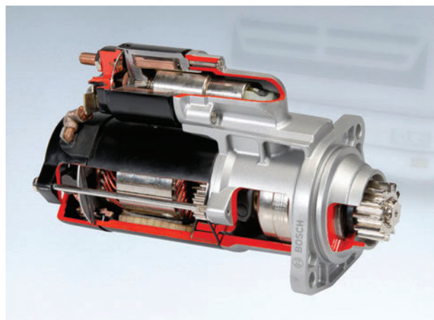
Figure 6.97 Intermediate transmission starter (Source: Bosch Media)
