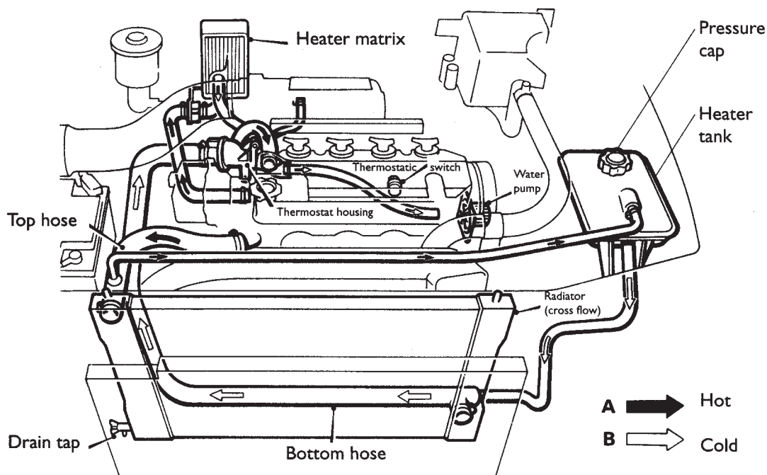
Figure 6.80 Semi-sealed cooling system
