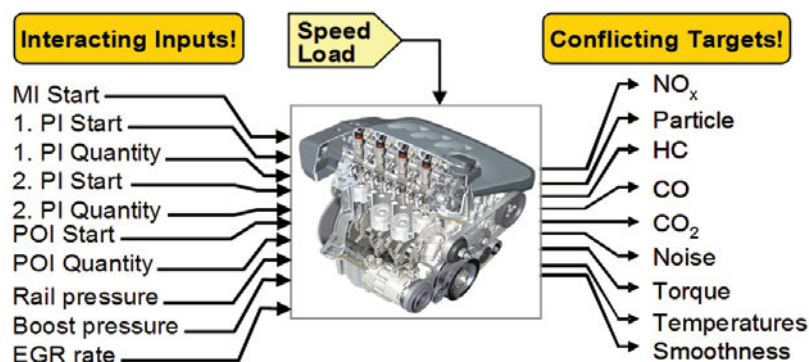
Figure 6.64 Typical ECU parameters needing to be adjusted in order to achieve the required targets for a modern diesel engine – this is ECU calibration (Source: www.autoelex.co.uk )
