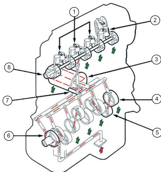
Figure 6.82 Oil flow: 1 – oil to rocker arms; 2 – hydraulic tappets; 3 – filter; 4 – crank main bearings; 5 – big-end bearings; 6 – crank driven oil pump; 7 – oil under pressure; 8 – camshaft
