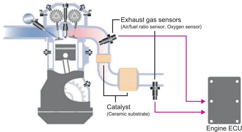
Figure 5.8 Exhaust gas oxygen sensors positioned pre- and post-catalyst (Source: http://www.globaldensoproductions.com )
