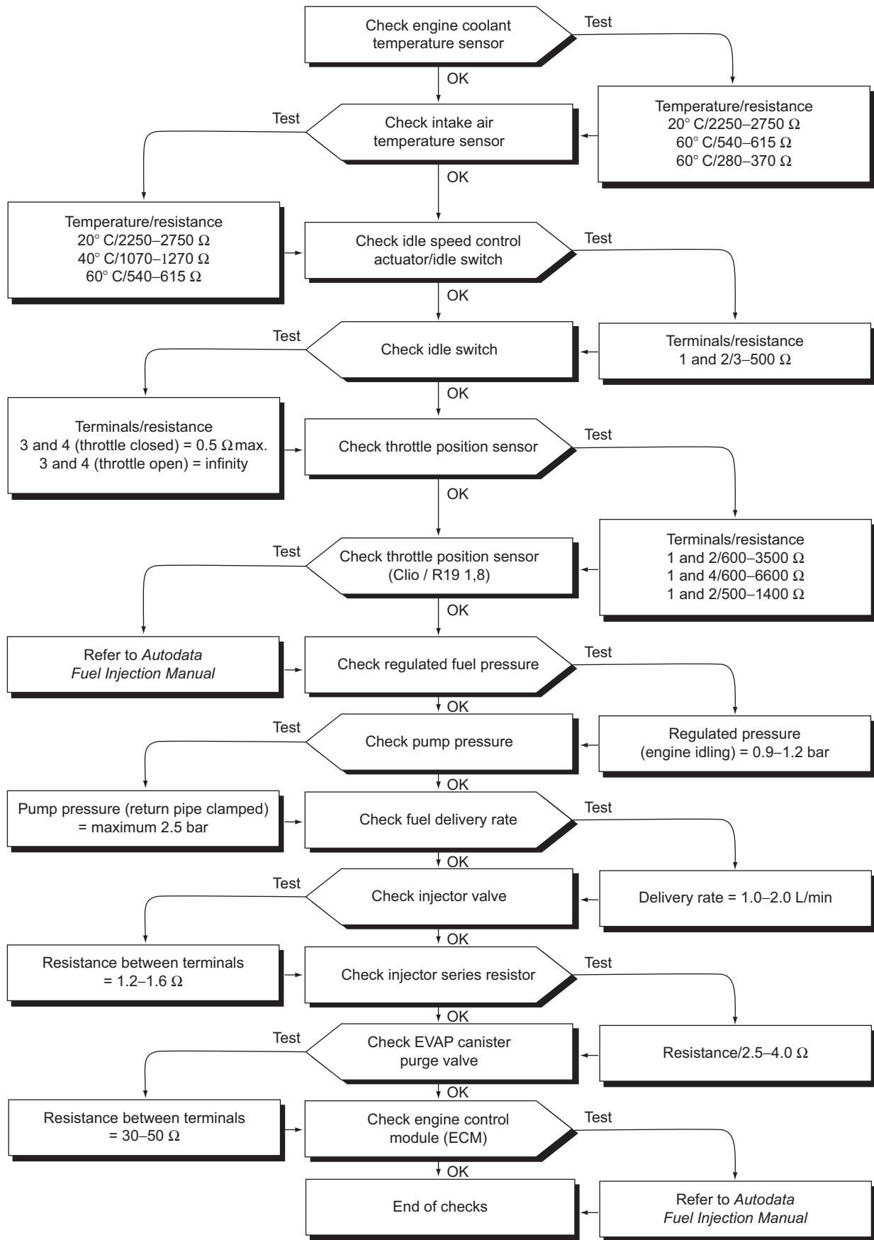
Figure 6.75 Faultfinding chart
