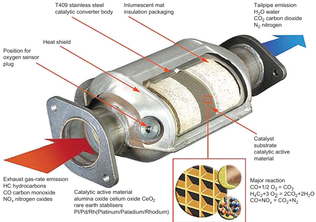
Figure 6.79 Catalytic converter components and operation
