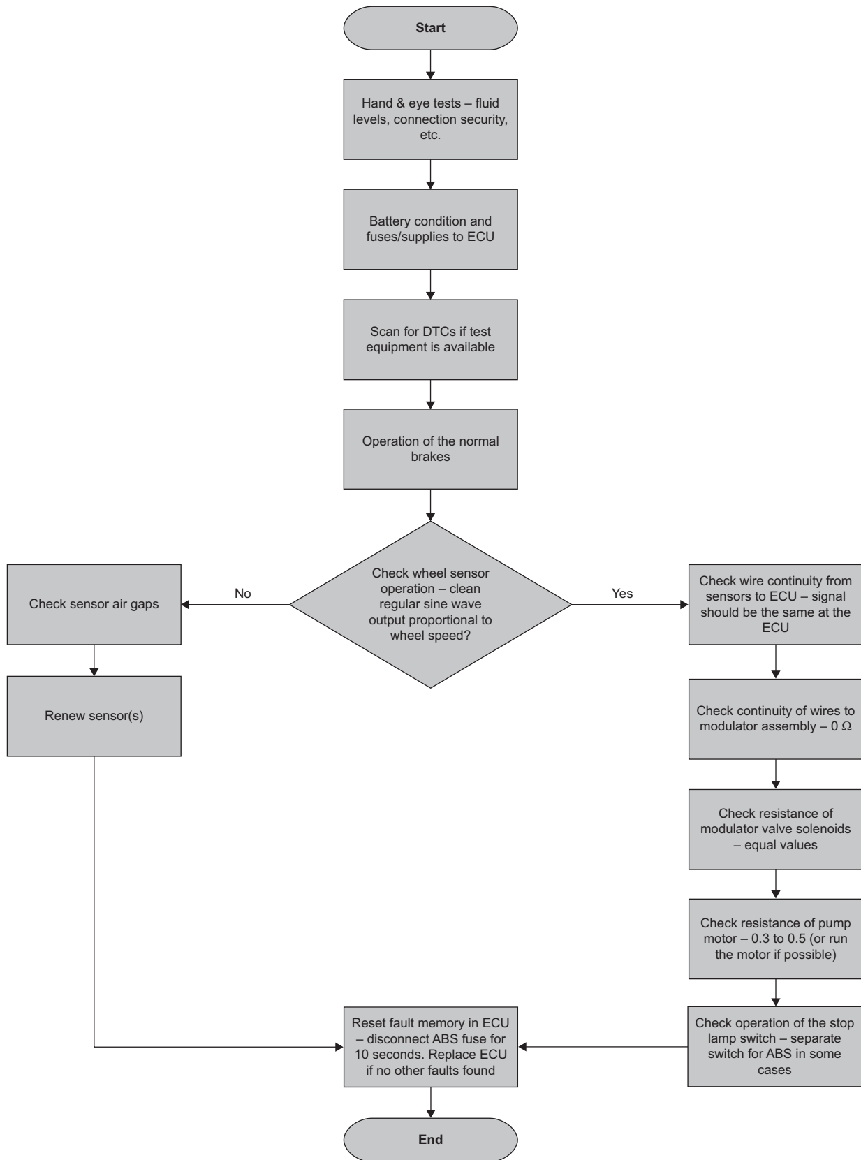
Figure 7.11 ABS diagnosis chart
