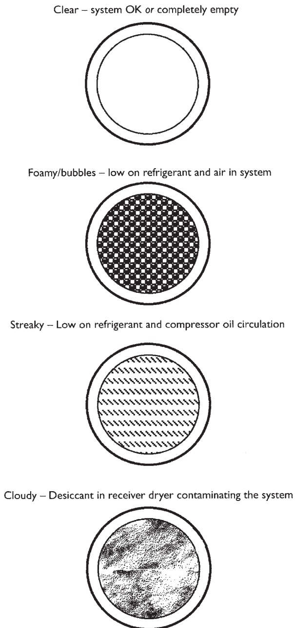
Figure 8.80 AC receiver drier sight glass
