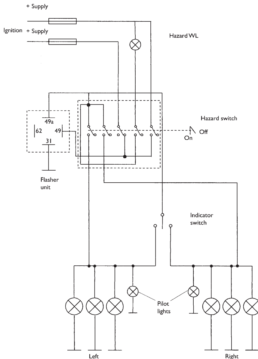
Figure 8.39 Indicator and hazard circuit
