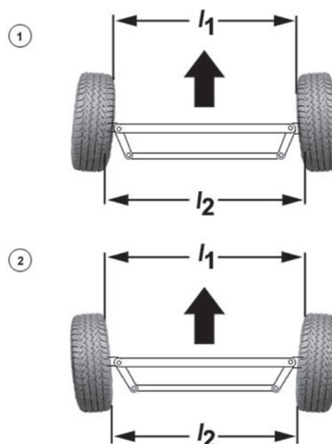
Figure 7.23 Tracking: 1 – toe-in; 2 – toe-out
