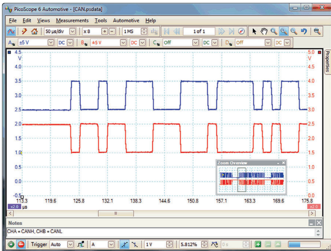
Figure 4.70 CAN signal zoomed in
