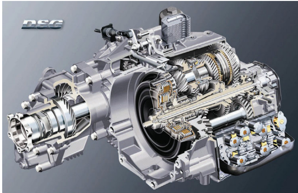
Figure 9.14 DSG (Source: Volkswagen Media)
