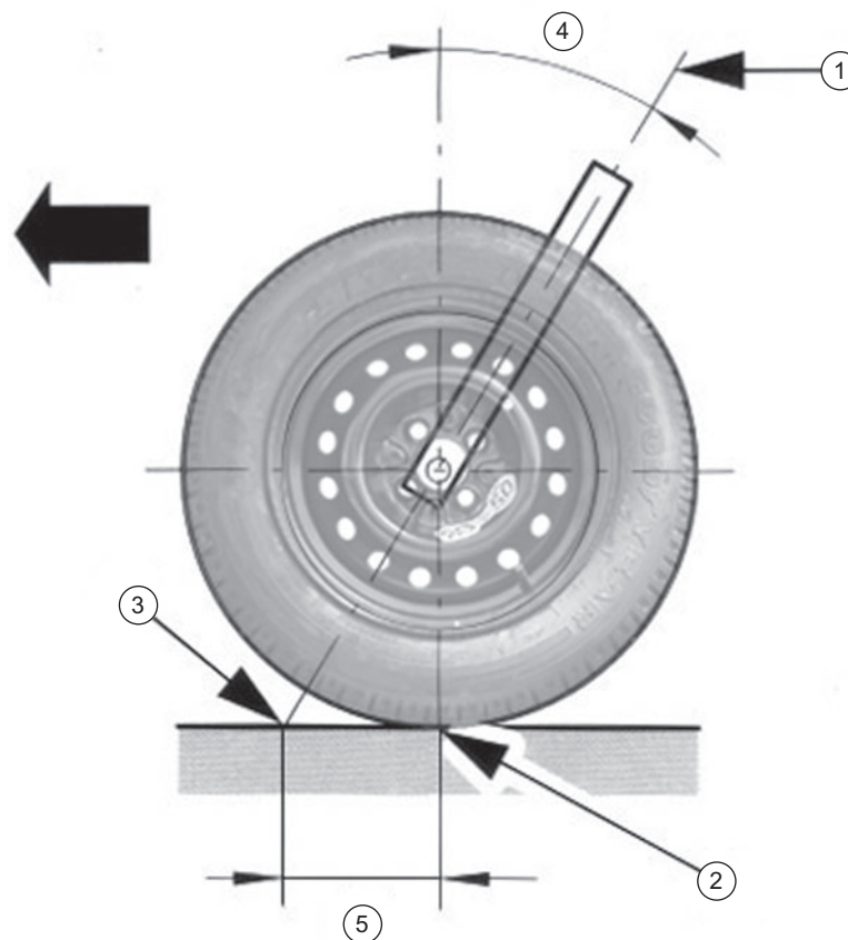
Figure 7.20 Castor angle – Positive: 1 – steering axis; 2 – wheel contact point; 3 – positive castor point of intersection of steering axis with the road surface; 4 – castor angle; 5 – castor distance
