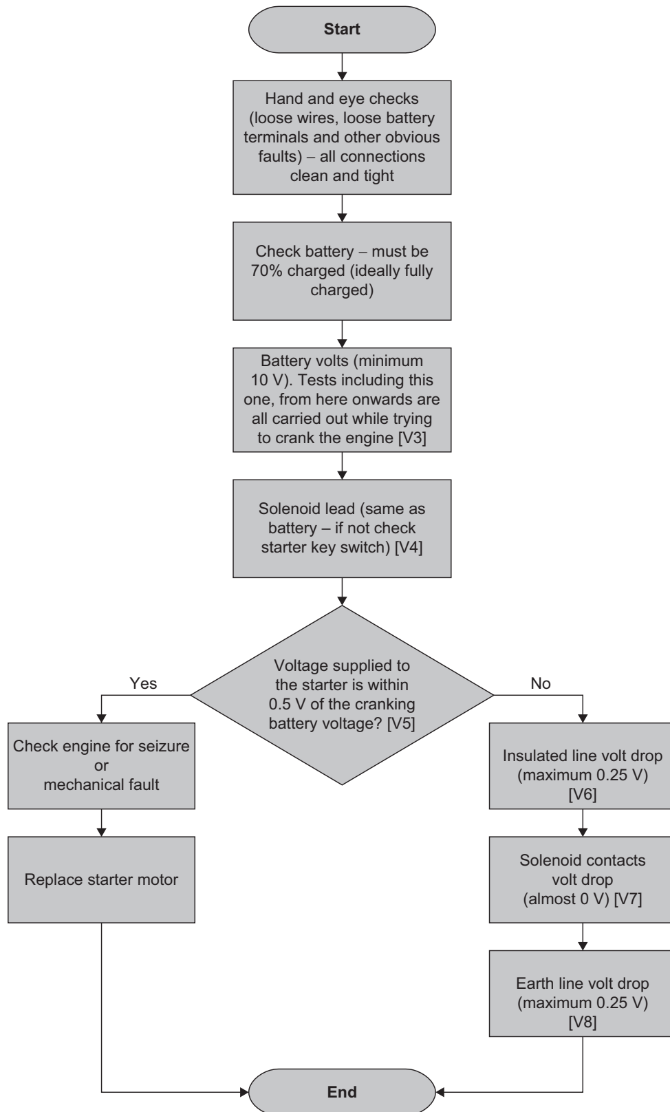
Figure 6.101 Starting system diagnosis chart
