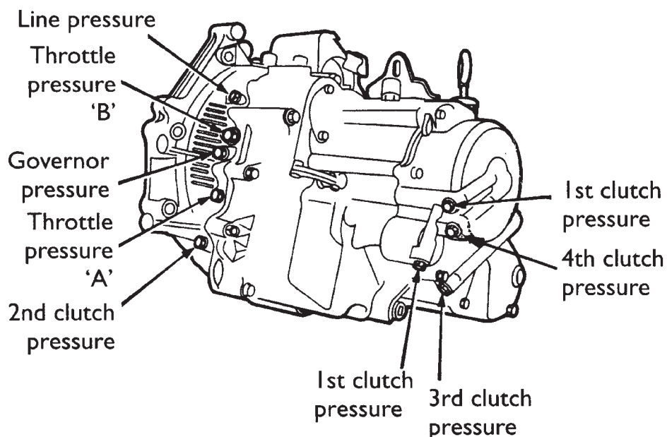
Figure 9.17 Transmission pressure testing points
