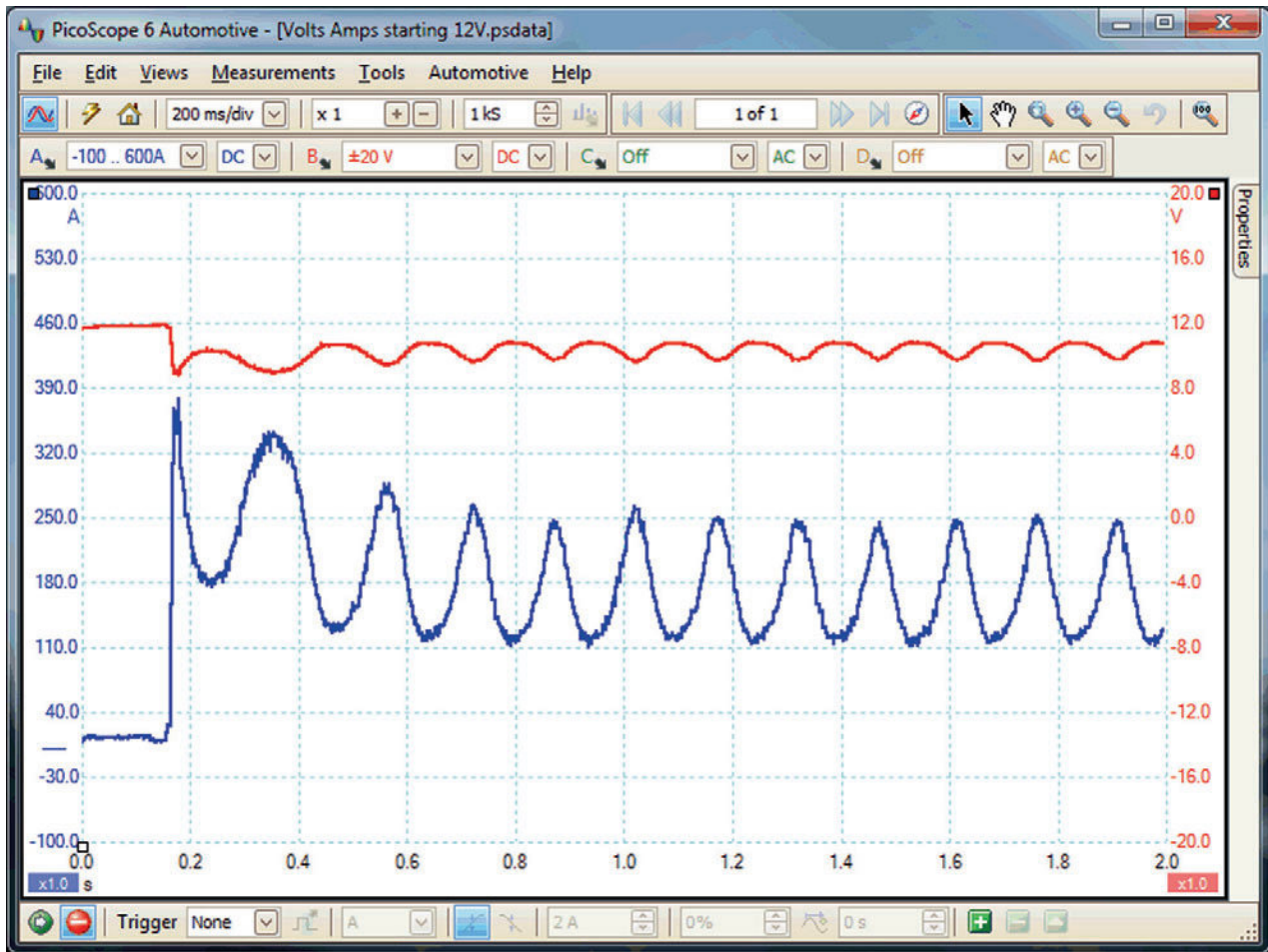
Figure 4.67 Spark ignition engine cranking amps
