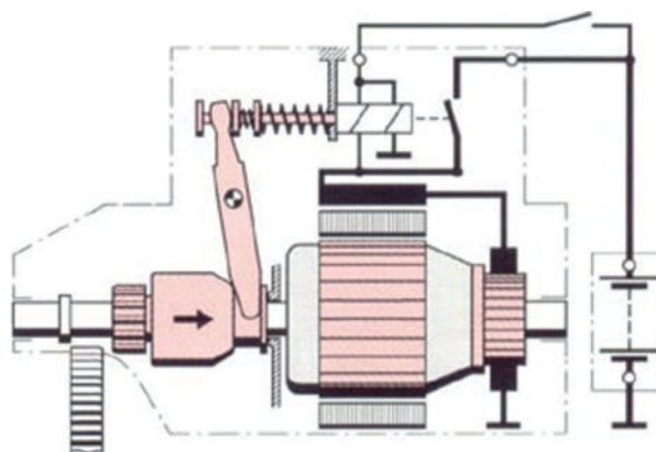
Figure 6.99 Starter circuit and engagement mechanism
