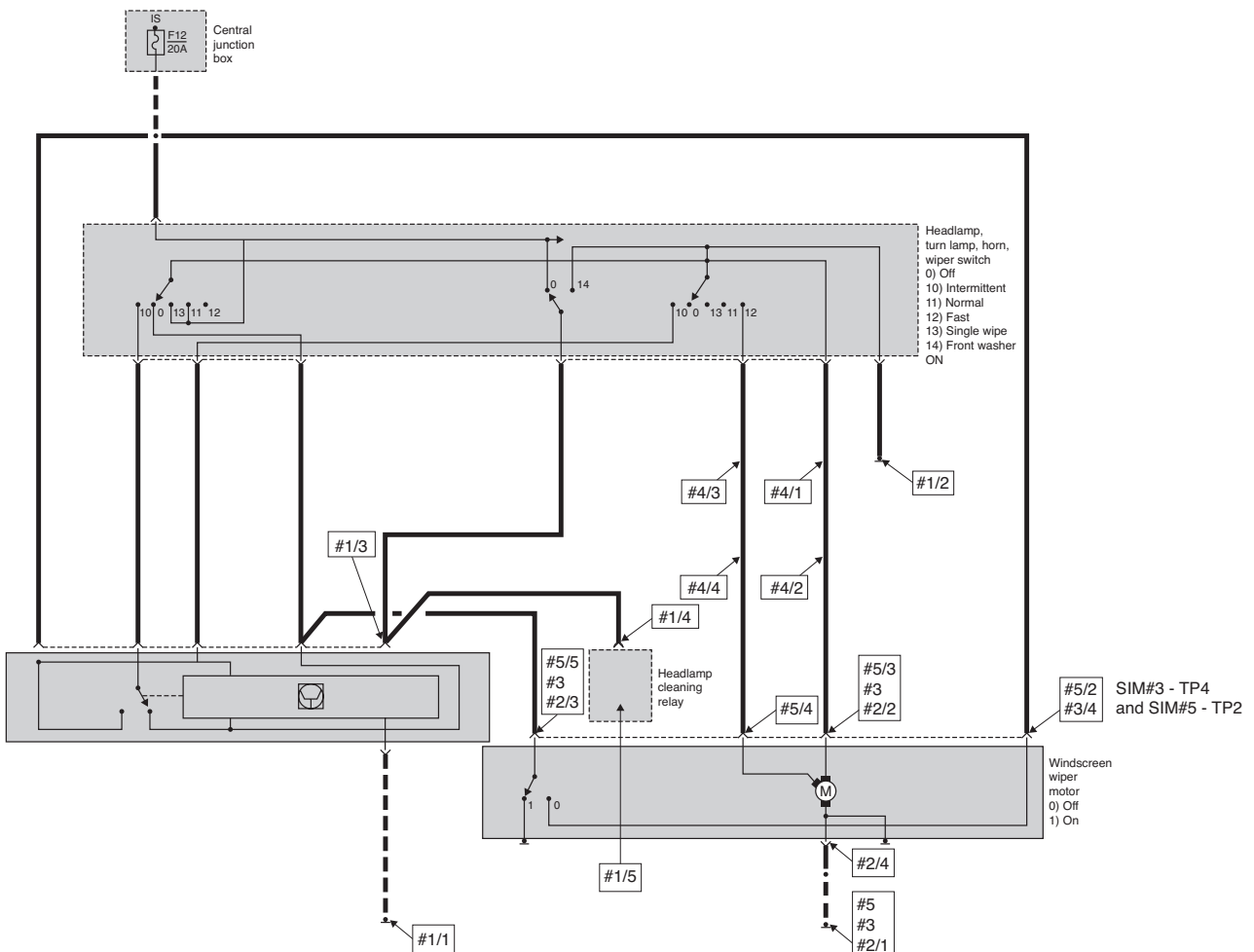
Figure 10.5 (simulation) Full circuit with test points on washer circuits
