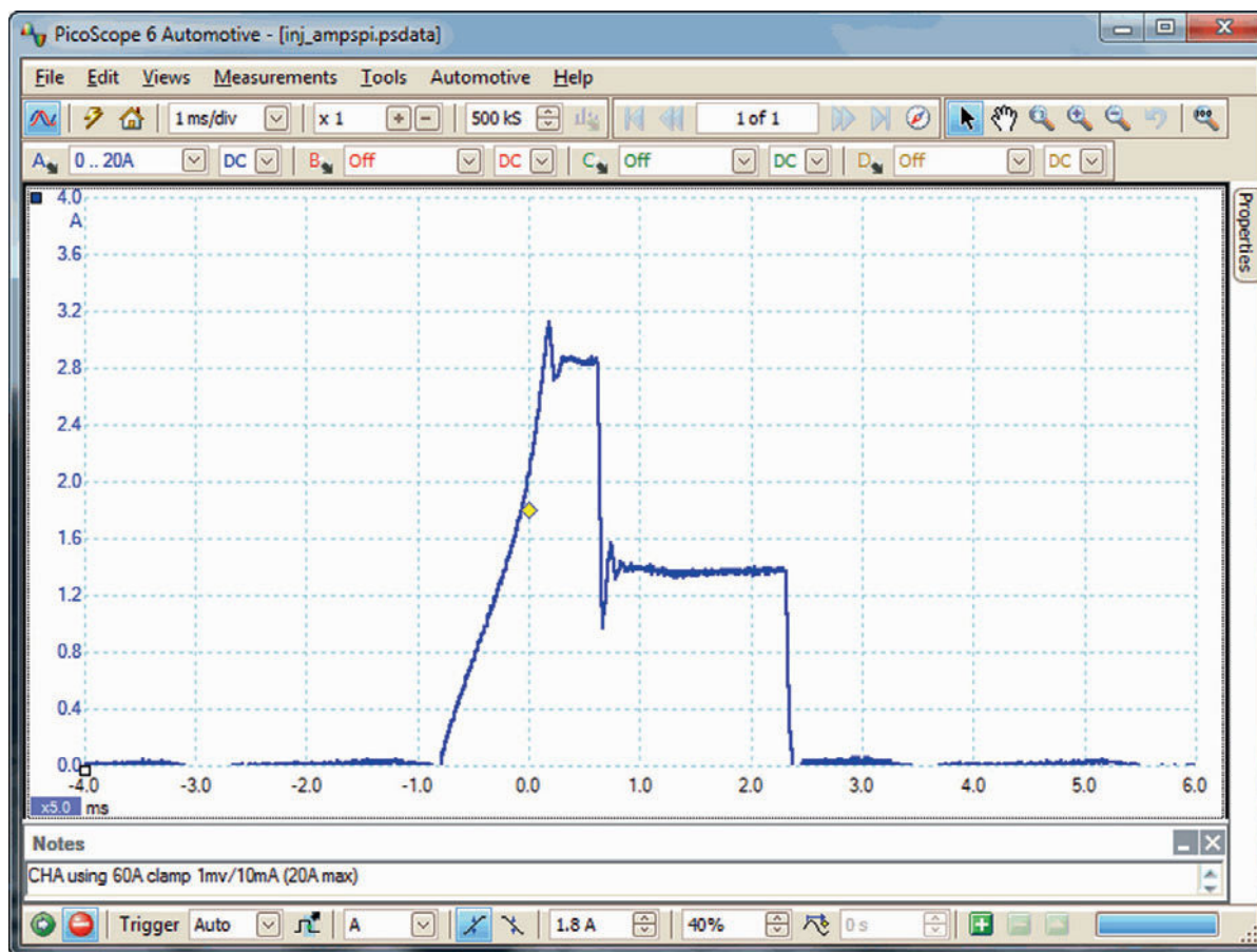
Figure 4.48 Single-point injector current waveform
