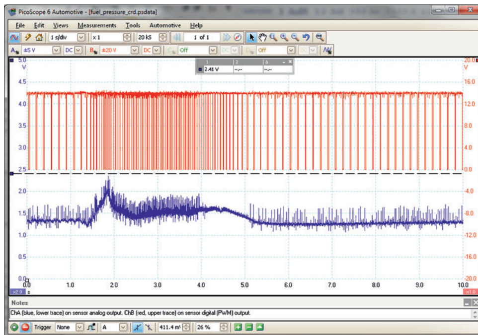
Figure 4.29 Common rail fuel pressure, the blue trace is from the sensor analogue output and the red trace is from sensor digital (PWM) output
