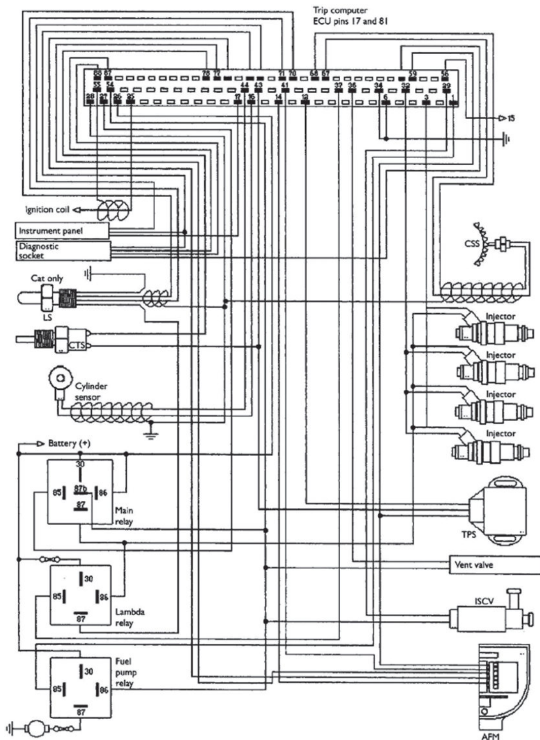
Figure 6.76 Engine management circuit diagram
