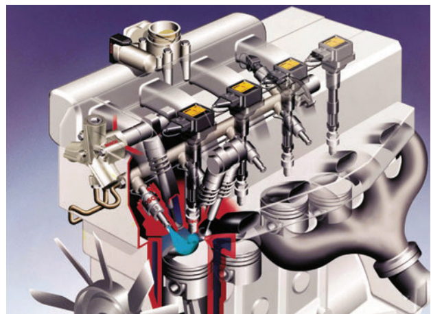
Figure 6.62 Gasoline direct injection (GDI)
