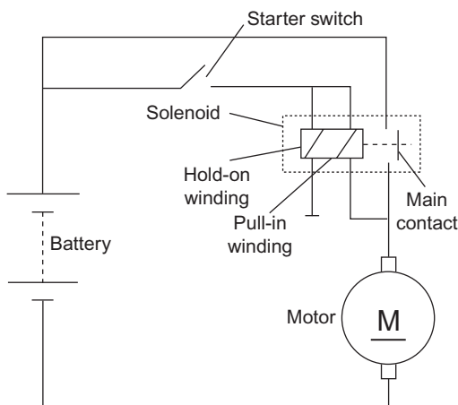
Figure 6.95 Starter circuit
