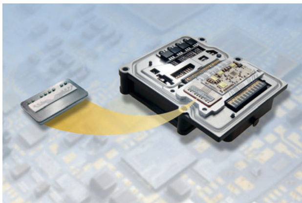
Figure 4.36 Yaw rate and acceleration sensor integrated into an electric stability program (ESP) control unit (Source: Bosch Media)
