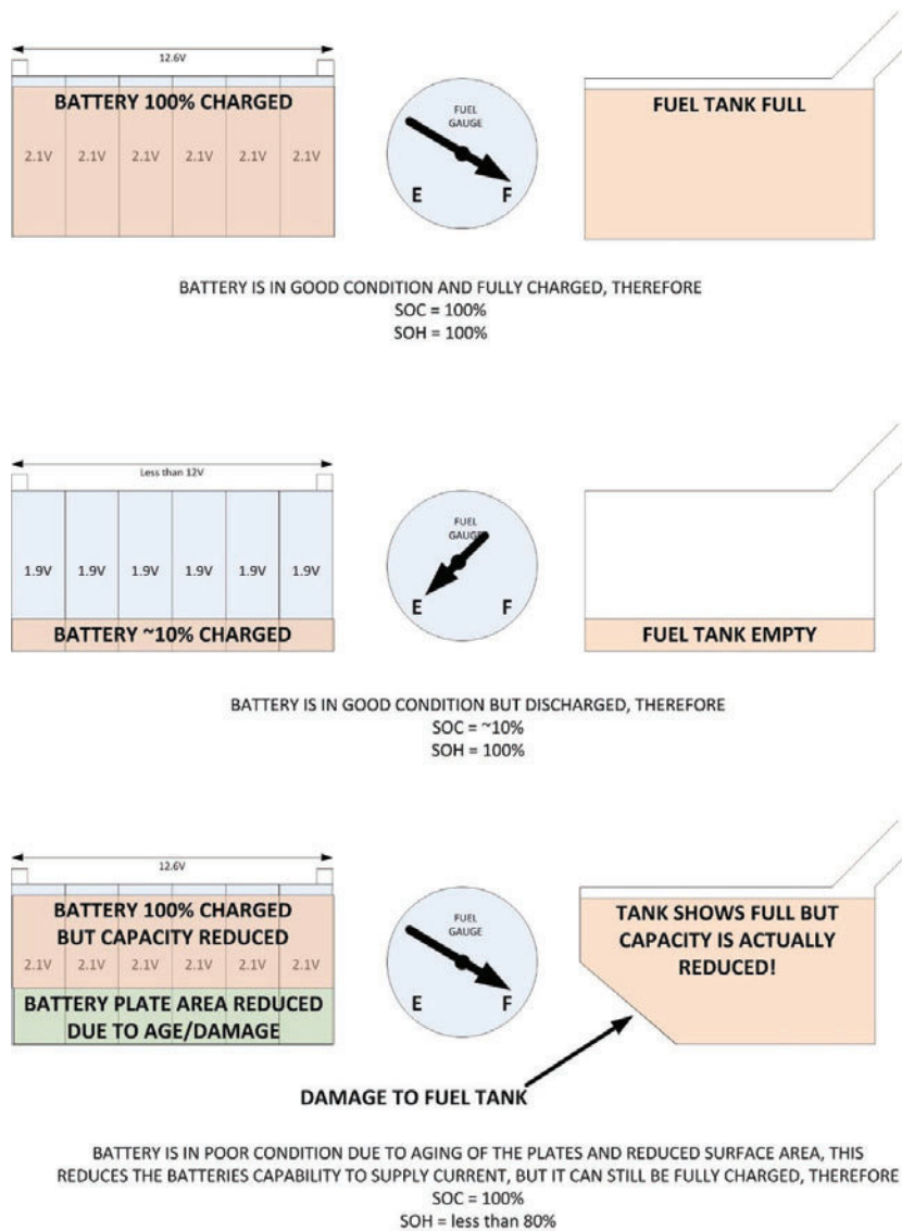
Figure 6.94 Battery SOC and SOH, for illustration, compared to a fuel tank
