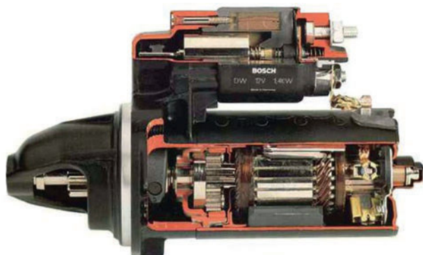
Figure 6.98 Permanent magnet fields are used in this starter motor
