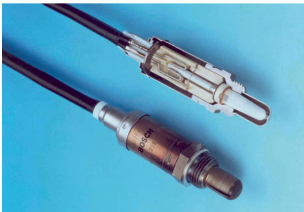
Figure 4.25 Zirconia-type oxygen sensor
