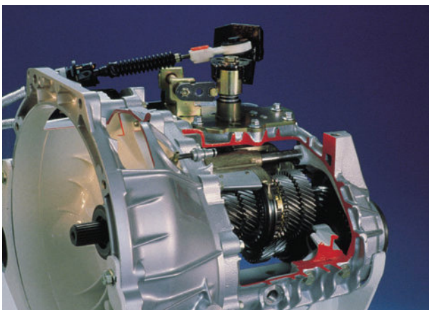
Figure 9.3 Manual gearbox with a cable change mechanism (Source: Ford Media)
