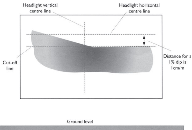
Figure 8.32 Asymmetric dip beam pattern
