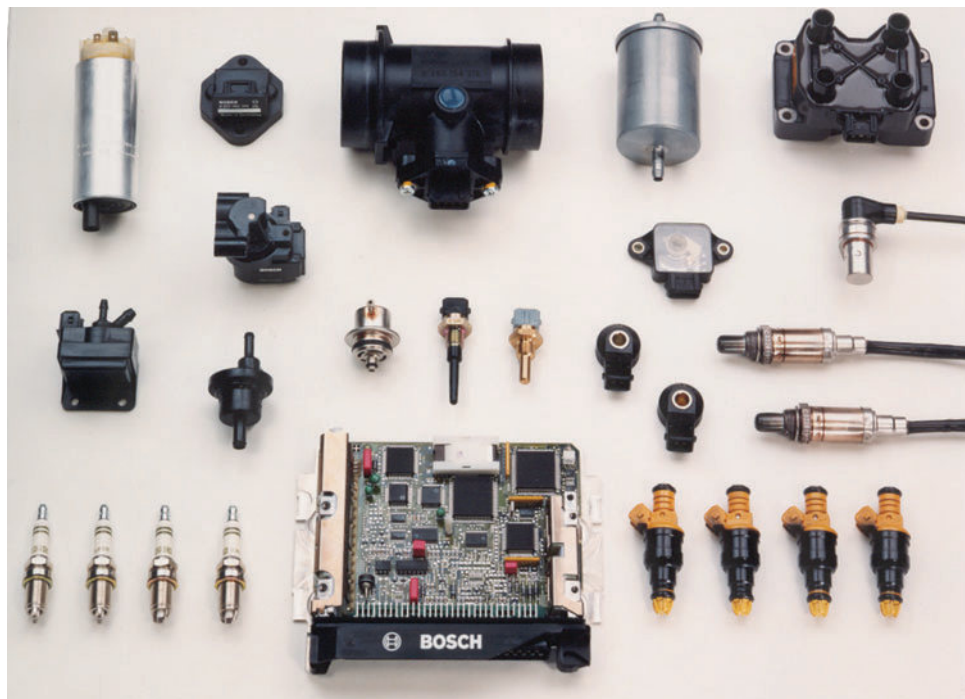
Figure 6.46 Earlier Motronic system components
