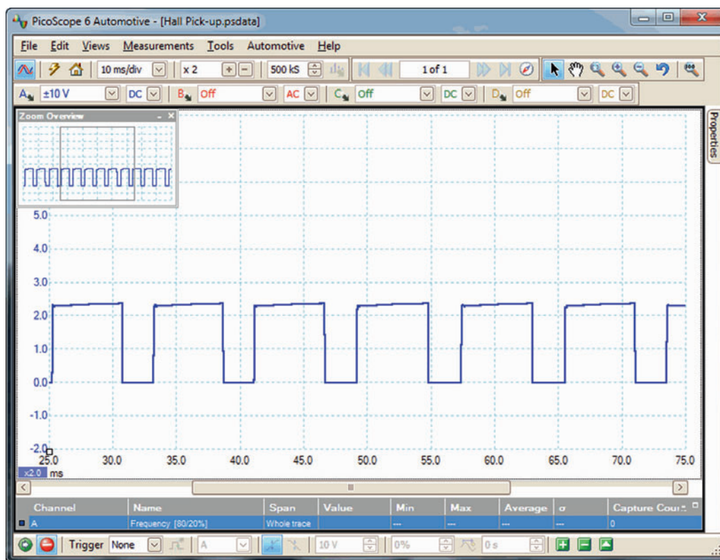
Figure 4.17 Hall output waveform
