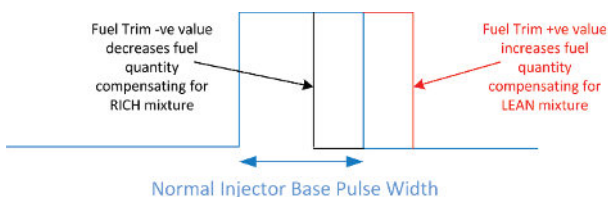
Figure 6.72 Fuel trim is effected by modifying the basic injector demand, for the engine operating condition
