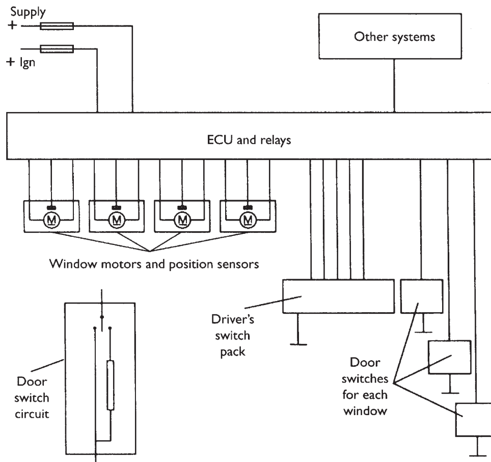
Figure 8.58 Electric window circuit
