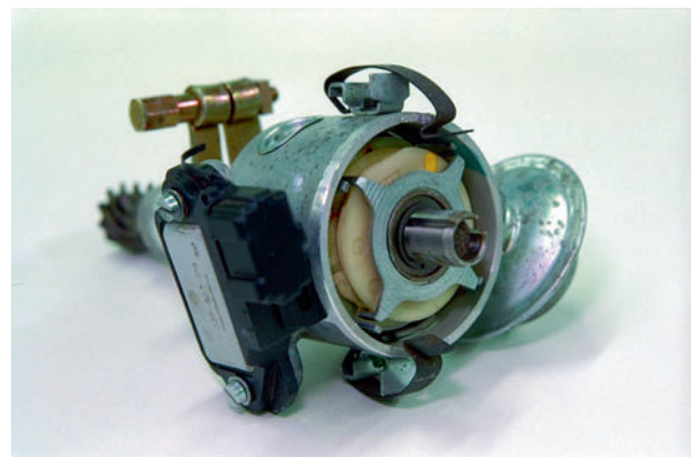
Figure 6.21 Inductive distributor
