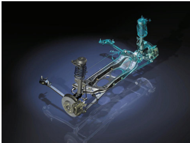
Figure 7.29 Rear suspension layout (Source: Ford Media)
