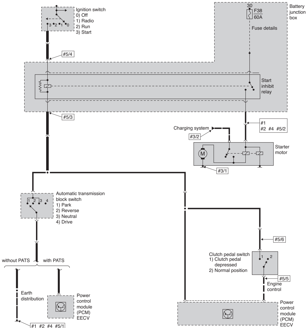
Figure 10.1 (simulation) Voltmeter on terminal 50 during cranking
