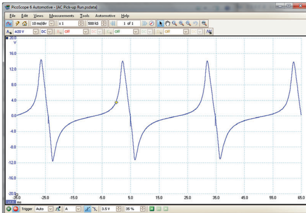
Figure 4.7 Inductive pick-up output signal (engine running)
