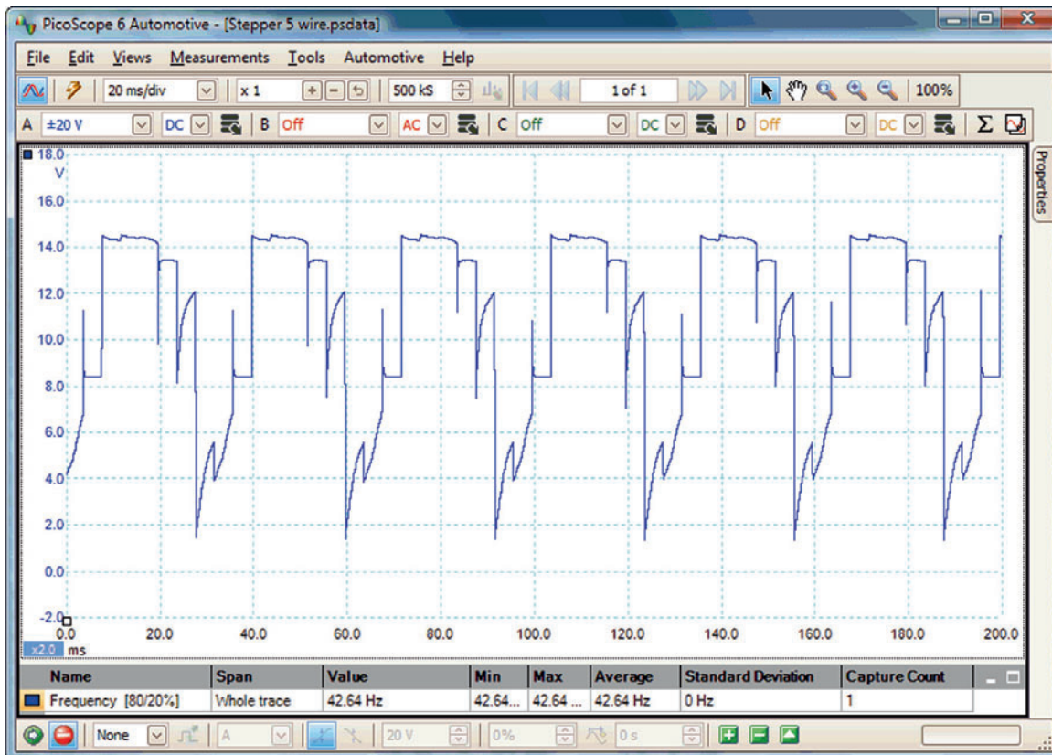
Figure 4.45 Alternative stepper motor signal
