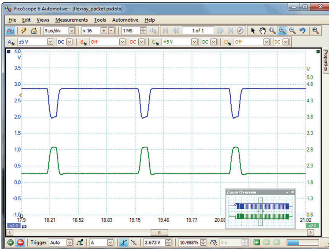
Figure 4.73 A closer view of a FlexRay signal
