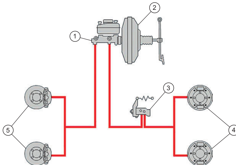
Figure 7.1 Brake system: 1 – master cylinder; 2 – brake servo or booster; 3 – pressure regulator; 4 – brake shoes; 5 – brake discs (rotors) and pads
