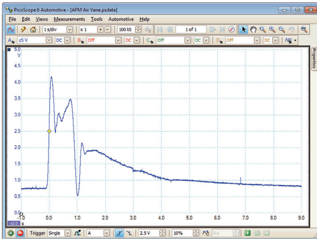
Figure 4.10 Air vane output voltage
