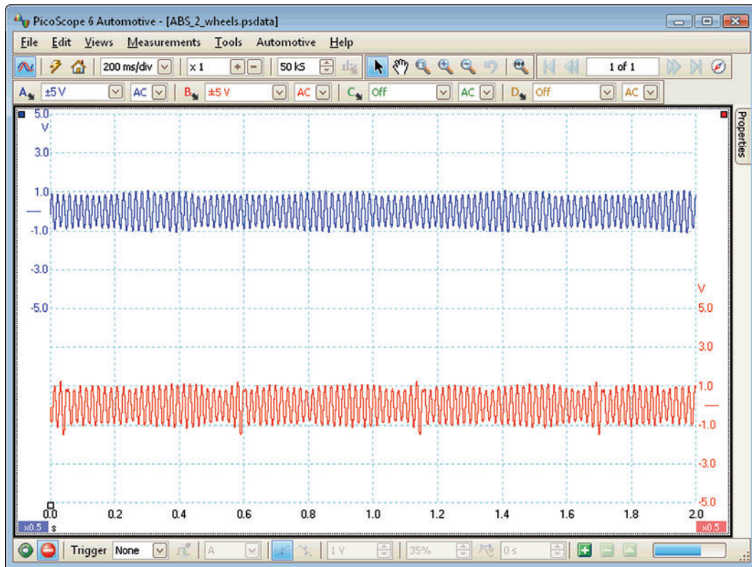
Figure 4.5 ABS speed sensor waveform
