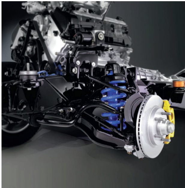
Figure 7.30 Front wishbone suspension system
