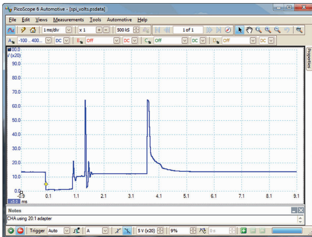
Figure 4.47 Single-point injector voltage waveform
