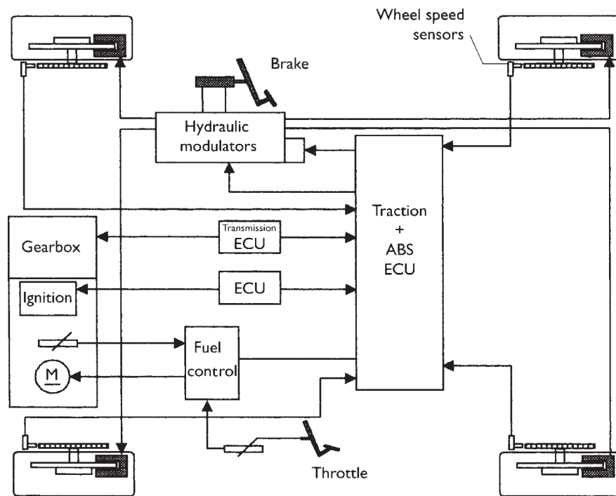
Figure 7.13 Integrated traction control system
