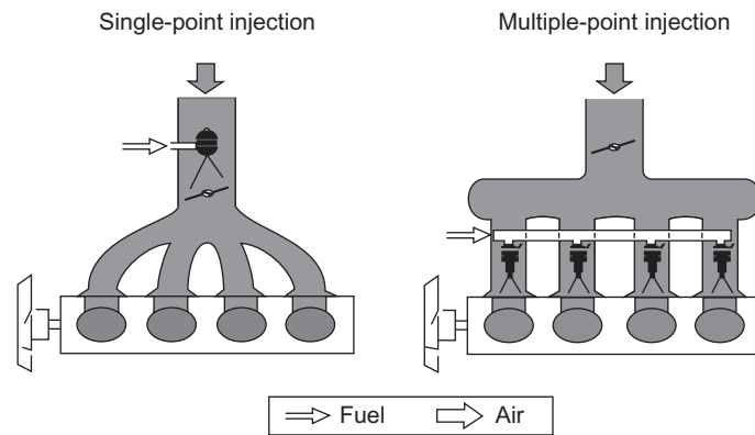
Figure 6.42 Fuel injection system layout
