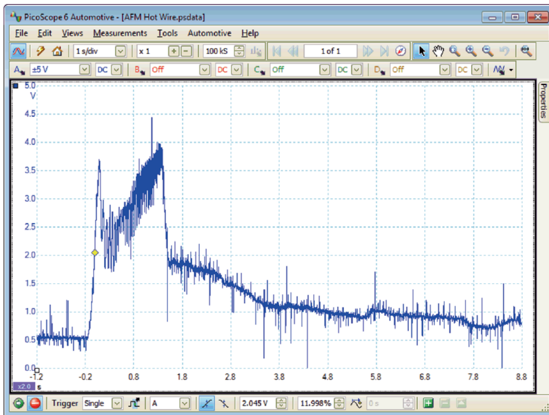
Figure 4.12 Air mass hot wire waveform
