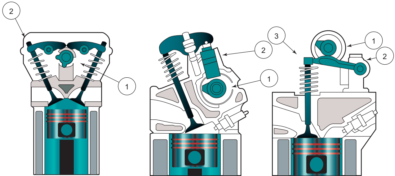
Figure 6.4 Valve operating mechanisms. Left: 1 – Cam; 2 – adjusting screw in direct acting rocker. Centre: 1 – Cam; 2 – hydraulic follower. Right: 1 – Cam; 2 – pivot and adjuster; 3 – finger follower
