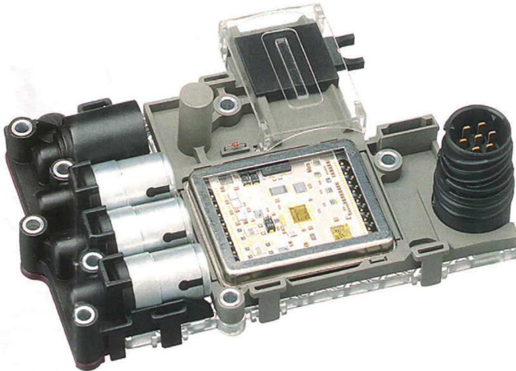
Figure 9.13 Electrohydraulic valve block
