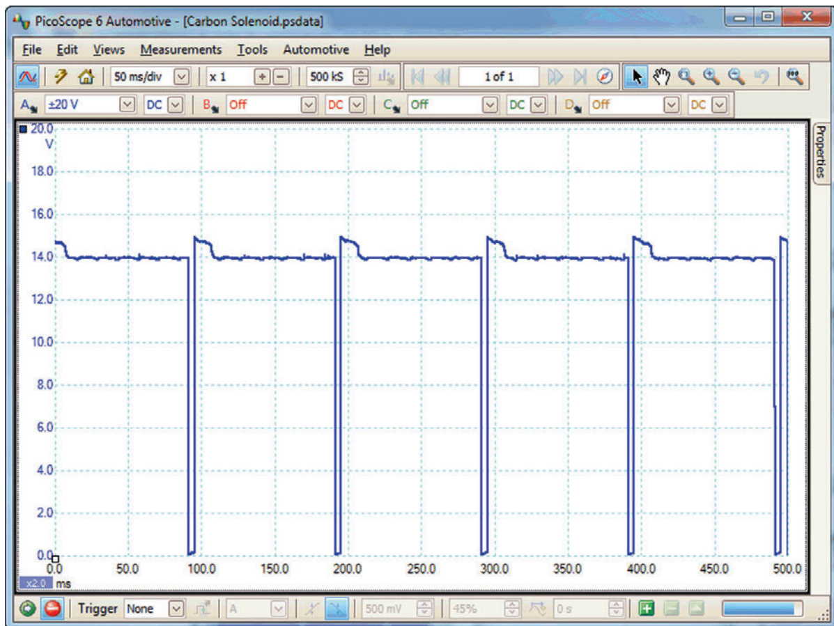
Figure 4.56 Carbon canister control valve signal
