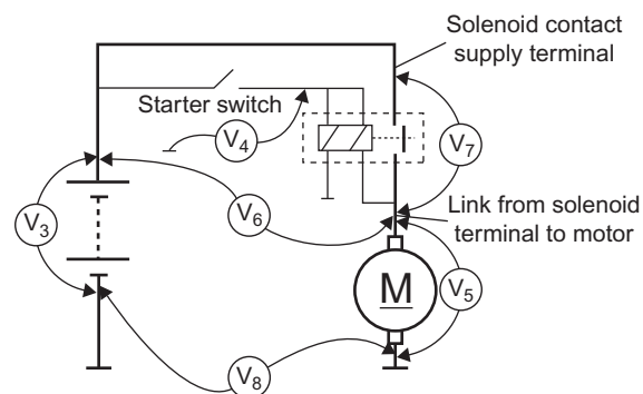
Figure 6.102 Starter circuit testing
