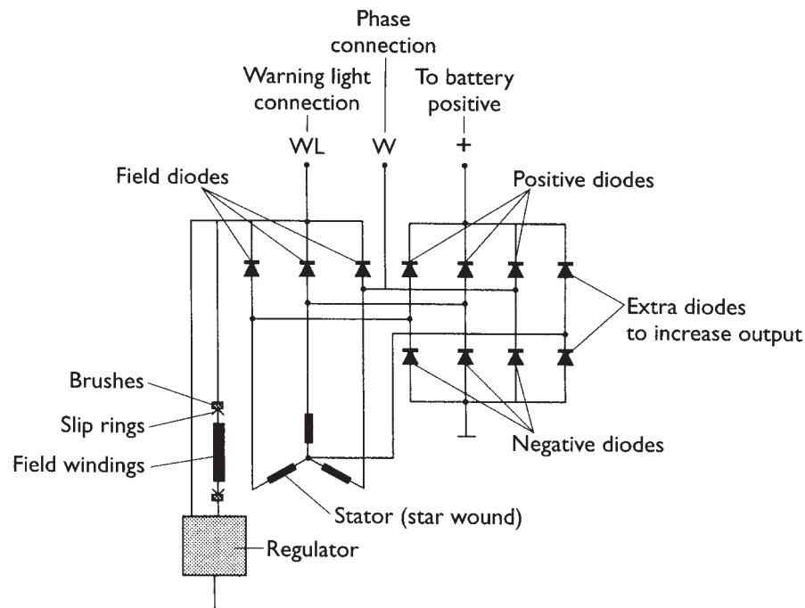
Figure 6.106 Alternator internal circuit
