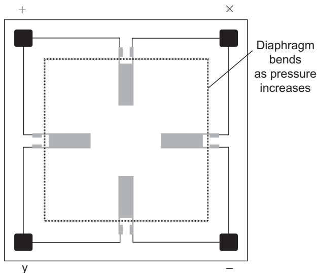
Figure 4.28 Strain gauge pressure sensor (+ and – are the supply, x and y the output signal)
