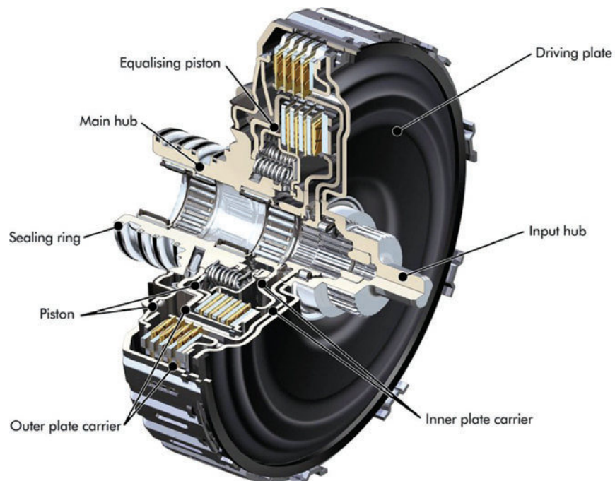
Figure 9.15 Multiplate twin clutch (Source: Volkswagen Media)
