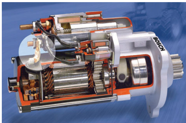
Figure 6.103 The link from the solenoid contacts and the motor is highlighted in this image
