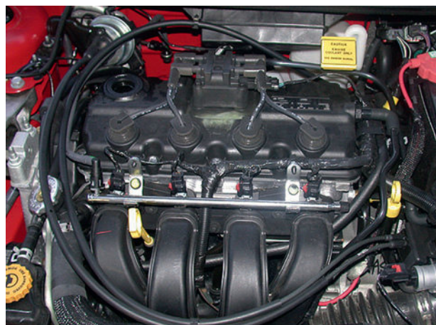
Figure 6.25 DIS coil on a four-cylinder engine
