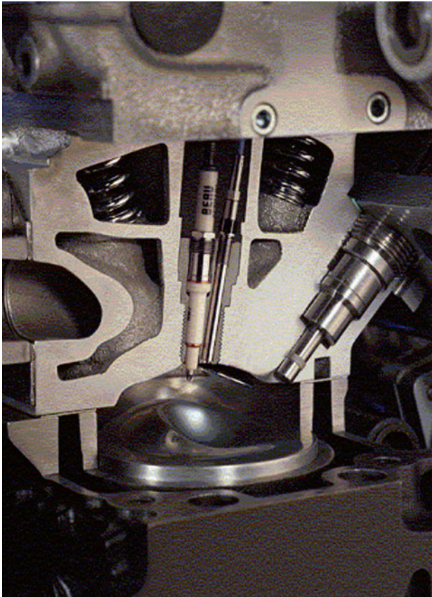
Figure 5.23 Cylinder pressure sensor mounted in the engine
