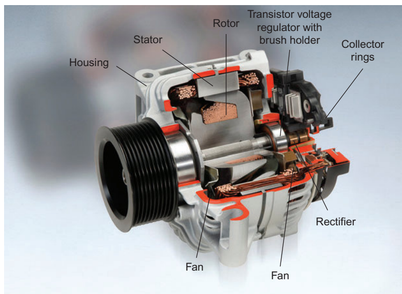
Figure 6.104 Alternator components
