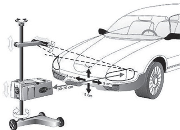
Figure 8.31 Headlamp alignment (Source: Hella)
