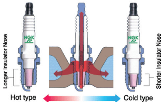
Figure 6.28 Hot and cold plugs. The cold plug is able to transfer heat more easily so is suitable for a hot engine
