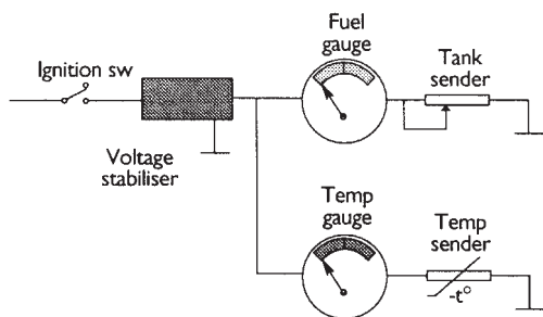
Figure 8.61 Simplified thermal gauge circuit
