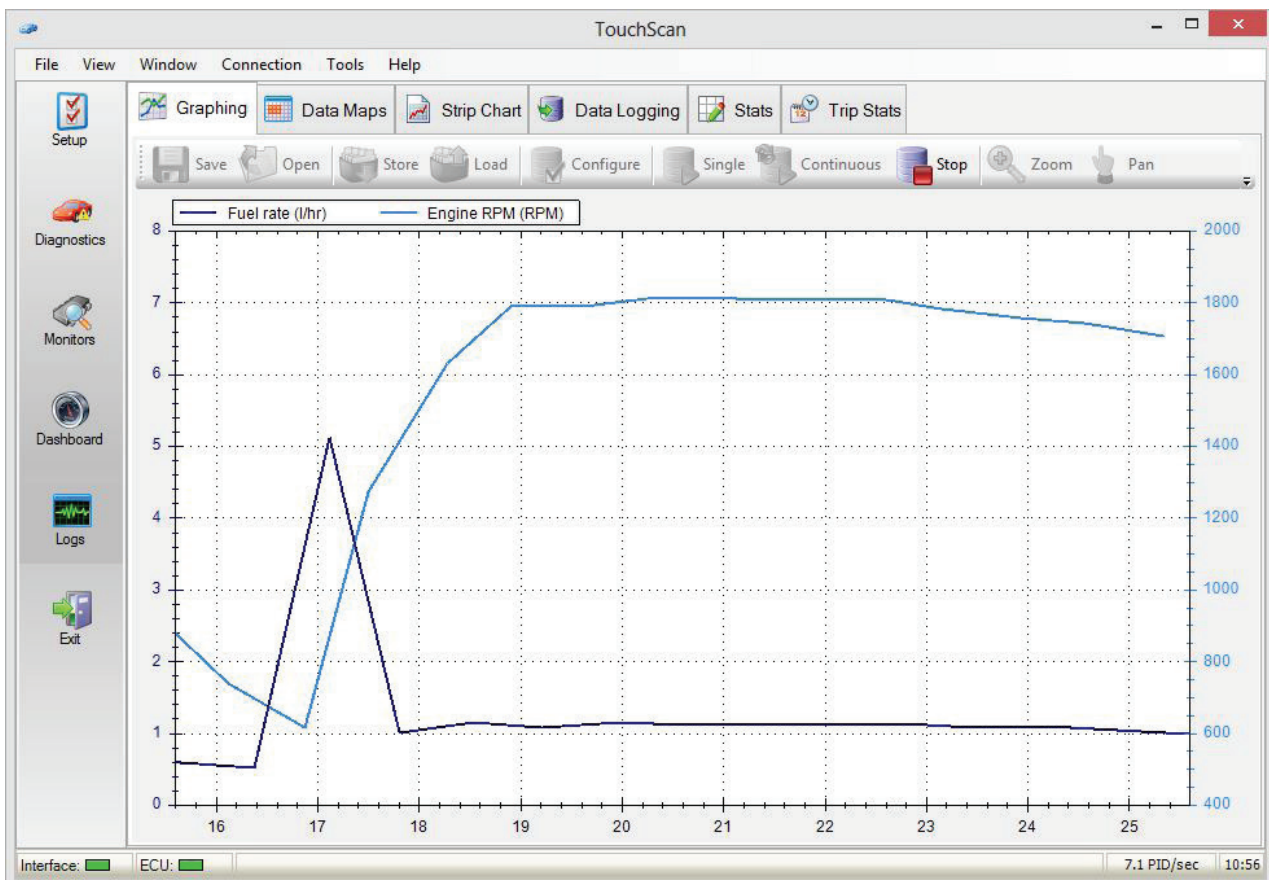
Figure 3.23 Logging of data allows variables to be compared over a set time. In this screen grab I was looking at fuel rate compared to engine rpm.
