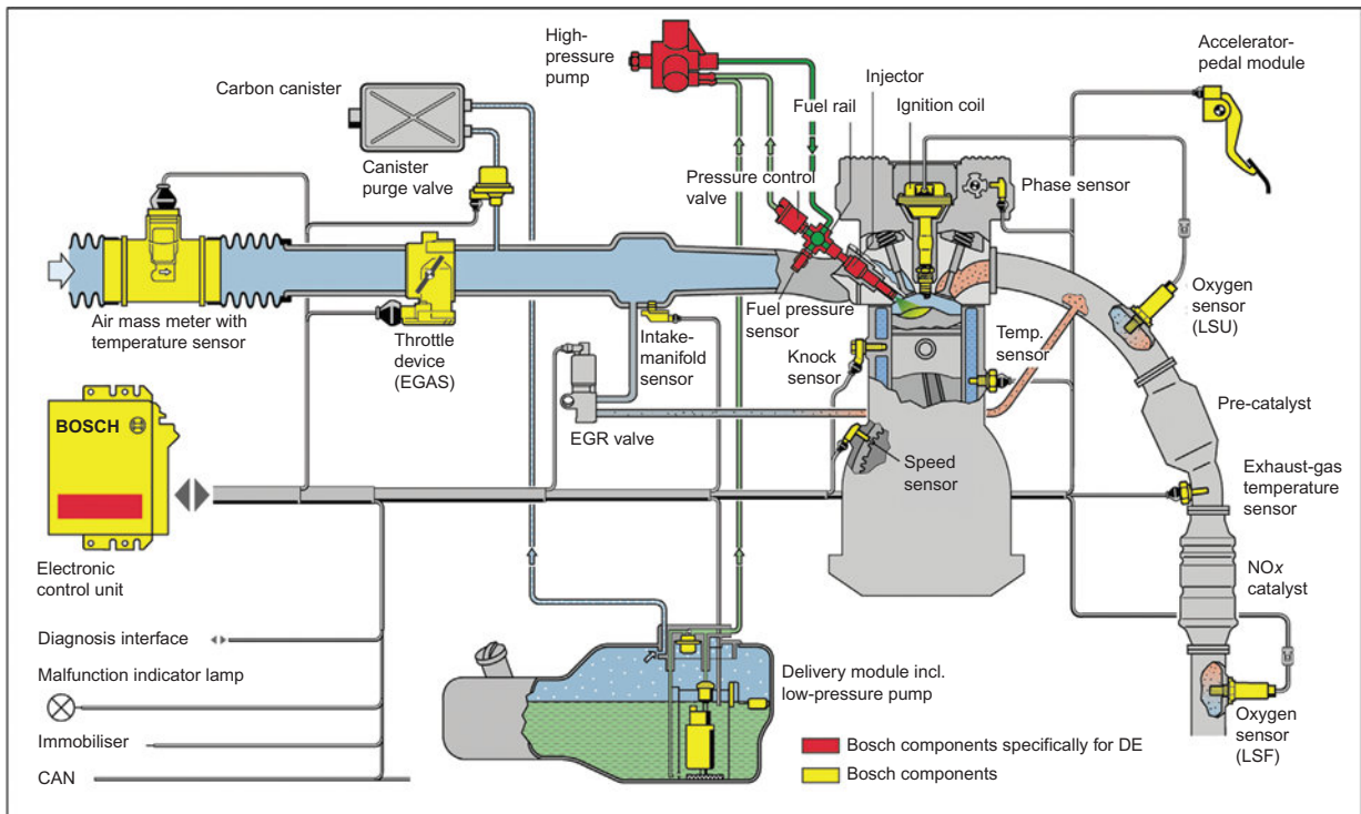
Figure 6.69 Motronic M5 with OBD2 (Source: Bosch Media)
