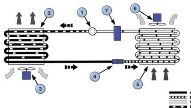
Figure 8.74 AC system layout: 1 – compressor; 2 – condenser; 3 – auxiliary fan (depending on model); 4 – fixed orifice tube; 5 – evaporator; 6 – heater/air conditioning blower; 7 – suction accumulator/drier; A – high-pressure warm liquid; B – low-pressure cool liquid; C – low-pressure, gaseous and cool; D – high-pressure, gaseous and hot (Source: Ford Motor Company)
