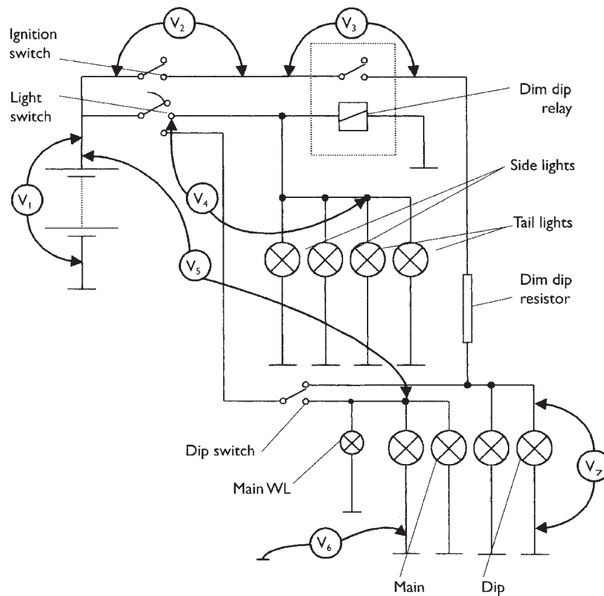
Figure 8.29 Lighting circuit under test
