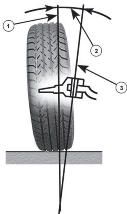
Figure 7.22 King pin or swivel axis inclination: 1 – perpendicular; 2 – swivel angle; 3 – steering axis
