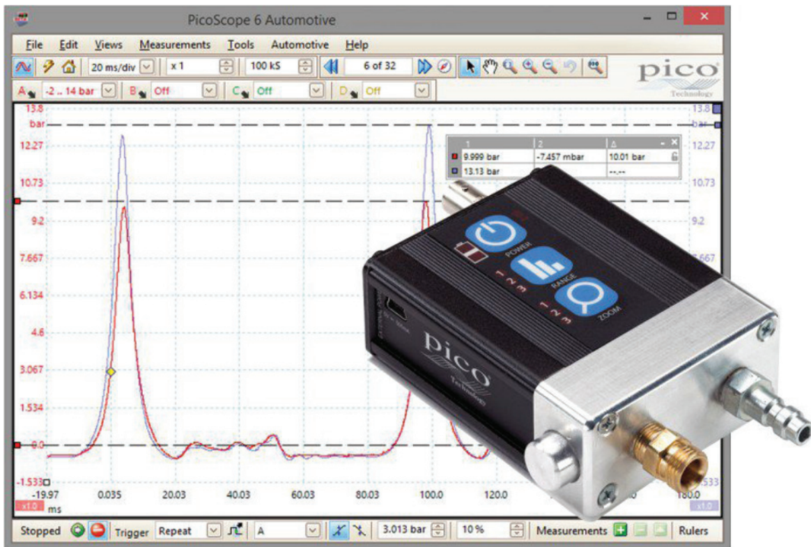
Figure 3.13 Pressure sensor and waveform
