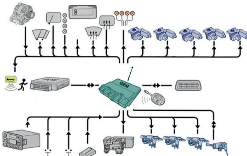
Figure 8.37 GEM and components (Source: Ford Motor Company)
