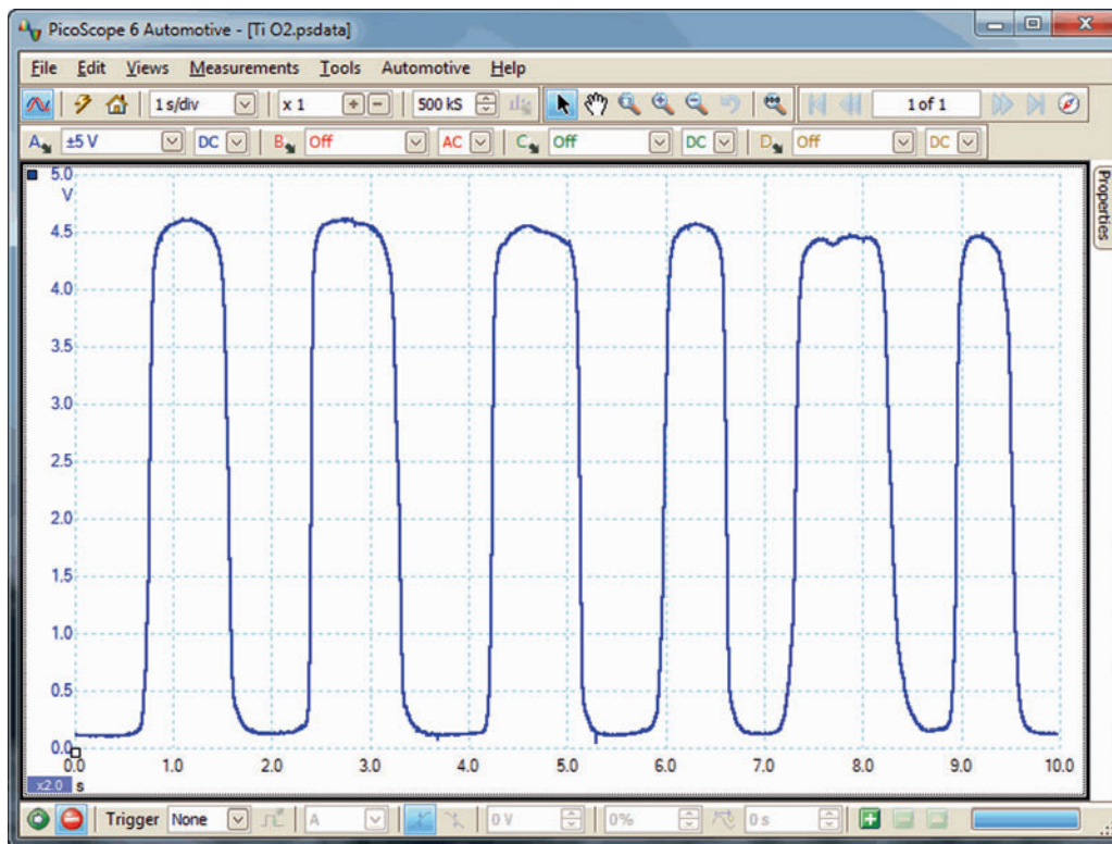
Figure 4.24 Titania lambda sensor output
