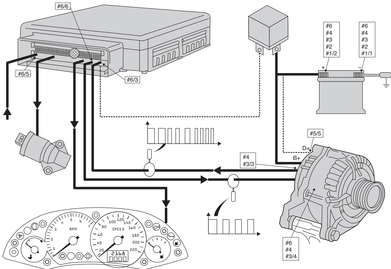
Figure 10.2 (simulation) Voltmeter to be connected across battery
