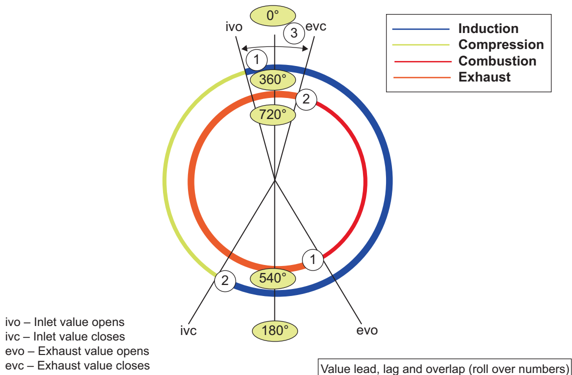
Figure 6.5 Valve timing diagrams (1 – lead; 2 – lag; 3 – overlap)
