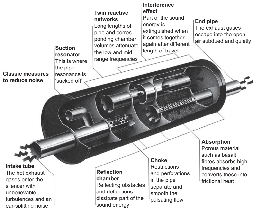
Figure 6.78 Exhaust noise reduction methods
