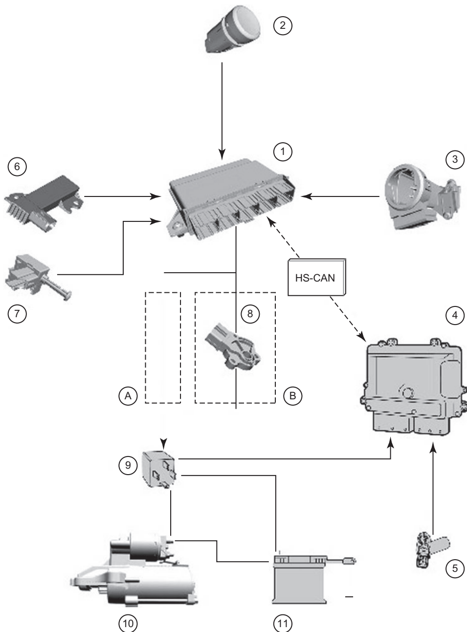
Figure 6.100 Keyless starting system: 1 – keyless vehicle module; 2 – start/stop button; 3 – electronic steering lock; 4 – powertrain control module; 5 – crank sensor; 6 – keyless vehicle antenna; 7 – vehicles with manual transmission: clutch pedal position switch/vehicles with automatic transmission: stoplamp switch; 8 – the TR sensor; 9 – starter relay; 10 – starter motor; 11 – battery; A – manual transmission (sensor not used); B – automatic transmission (Source: Ford Motor Company)
