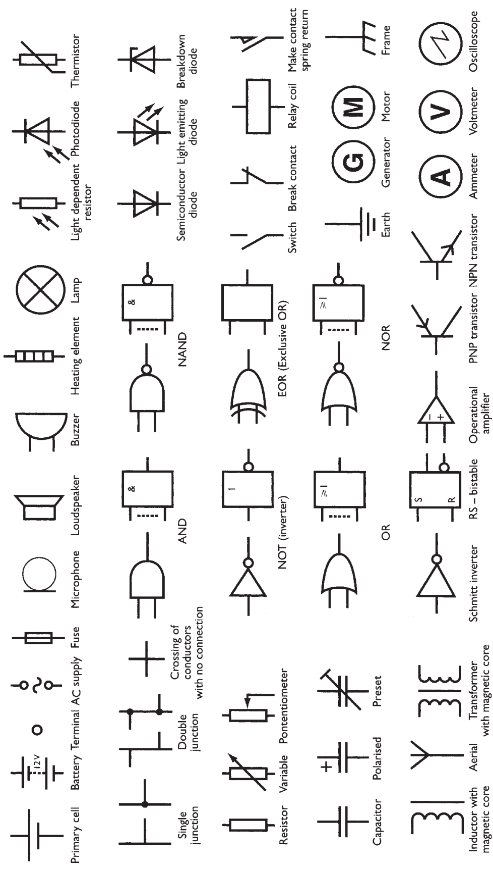
Figure 8.1 Circuit symbols
