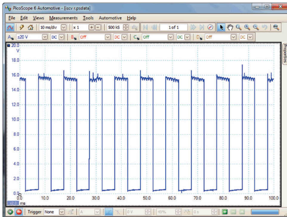
Figure 4.41 Signal supplied to a rotary idle control valve
