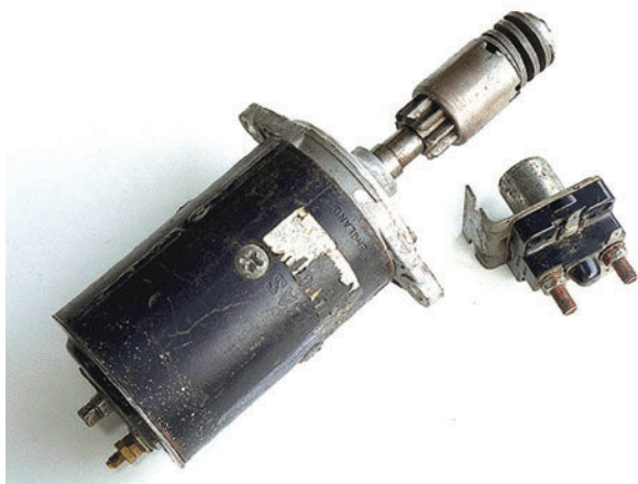
Figure 6.96 Inertia engagement starter and solenoid switch
