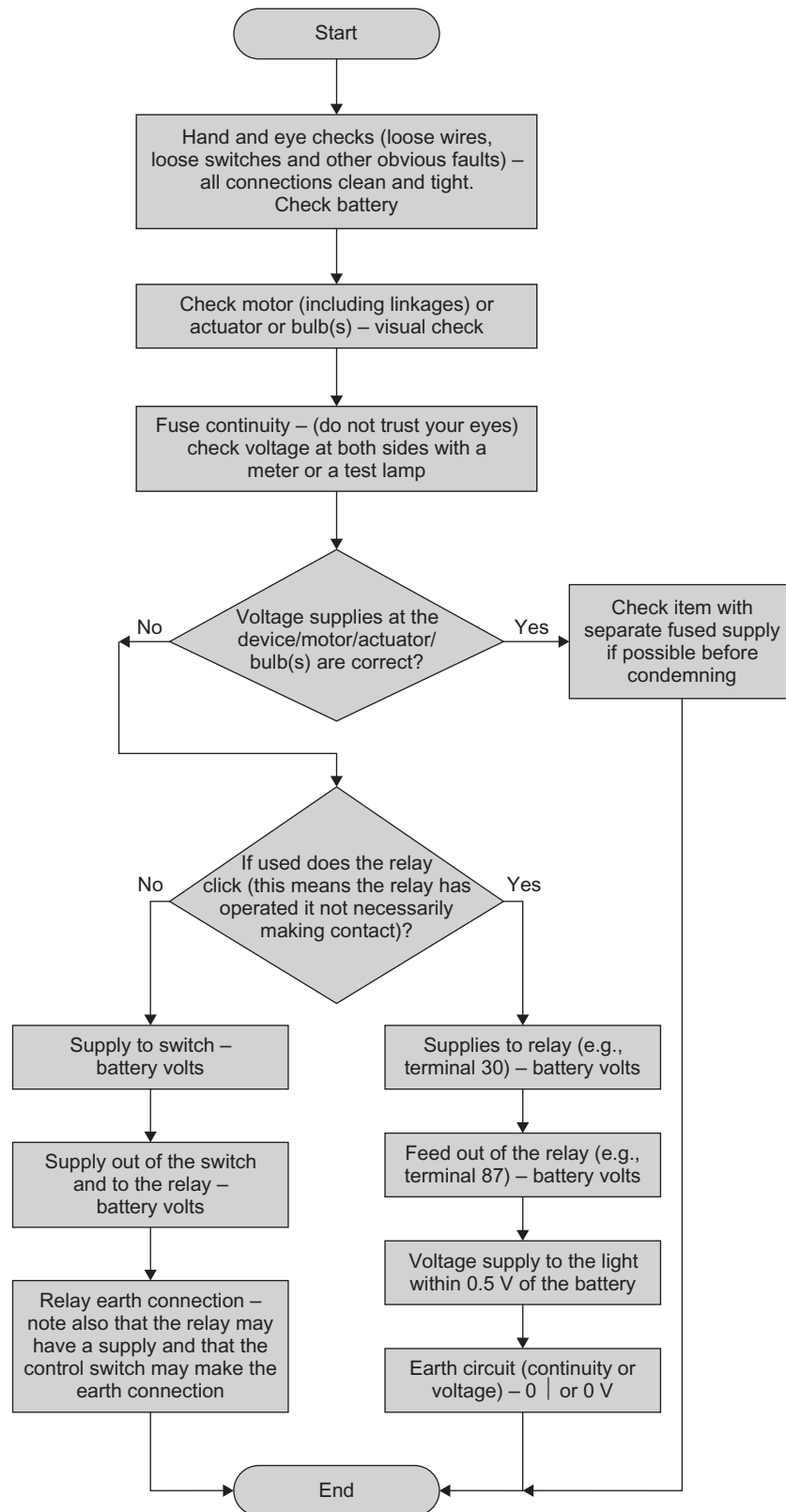
Figure 2.7 Generic electrical diagnostics chart
