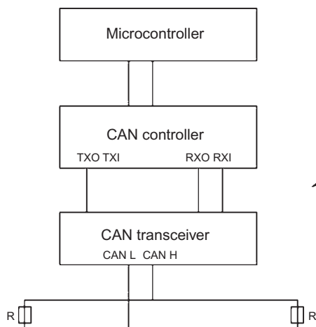
Figure 8.10 CAN nodes can be disconnected by the control program
