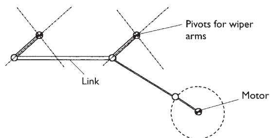
Figure 8.33 Wiper linkage
