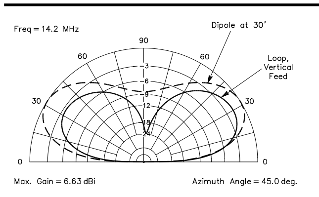
Fig 32 —Elevation-plane response of 7-MHz loop used on 14.2 MHz. This is for a feed point at the center of one of the two vertical wires. The dashed line is the response of a flattop 20-meter dipole at 30 feet in height for comparison.
