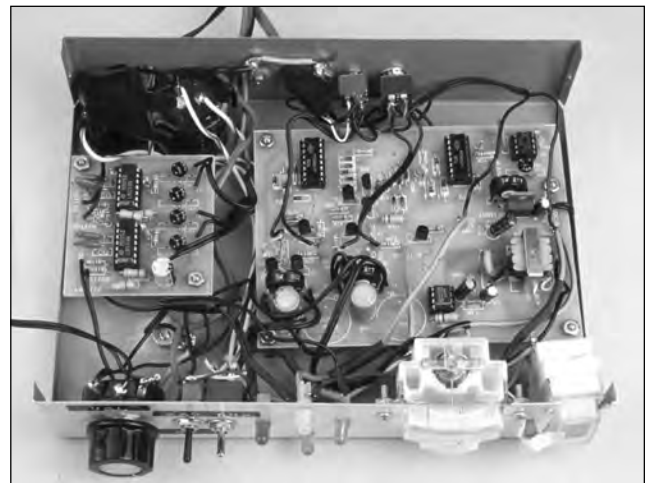
Fig 42—An inside view of one DF unit built into a 2 \times 8 \times 5\frac{3}{4} -inch (HWD) box. Because of the height restriction, the two 4700-μF damping capacitors (C8 and C10) are not mounted on the PC board, but near the rear panel behind the smaller of the two PC boards. One of the 4700-μF damping capacitors is a standard electrolytic, the other is a parallel combination of five 1000-μF, 6.3-V bipolar (nonpolarized) capacitors wrapped in electrical tape.
