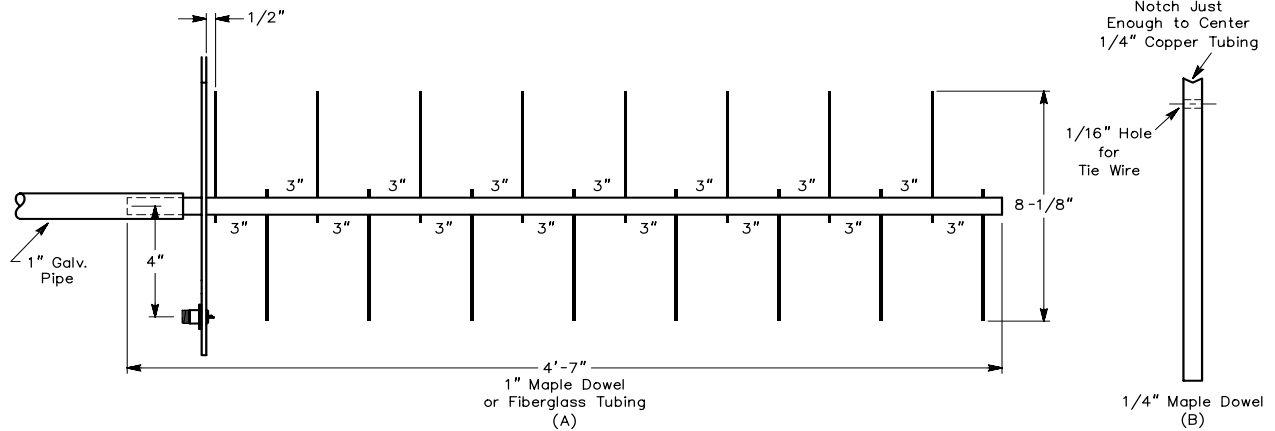
Fig 50 —At A, the layout of the portable 435-MHz helix is shown. Spacing between the first 5-inch winding-support dower and the ground plane is \frac{1}{2} inch; all other dowers are spaced 3 inches apart. At B, the detail of notching the winding-support dowers to accept the tubing. As indicated, drill a \frac{1}{16} -inch hole below the notch for a piece of small wire to hold the tubing in place.
