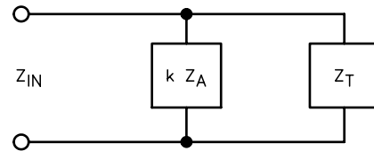
Fig 30—Equivalent circuit of an open sleeve antenna.
