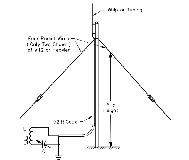
Fig 13—A ground-plane antenna is effective for DX work on 7 MHz. Although its base can be any height above ground, losses in the ground underneath will be reduced by keeping the bottom of the antenna and the ground plane as high above ground as possible. Feeding the antenna directly with 50-Ω coaxial cable will result in a low SWR. The vertical radiator and the radials are all \lambda/4 long electrically. Contrary to popular myth, the radials need not necessarily be 5% longer than the radiator. Their physical length will depend on their length-to-diameter ratios, the height over ground and the length of the vertical radiator, as discussed in text.
