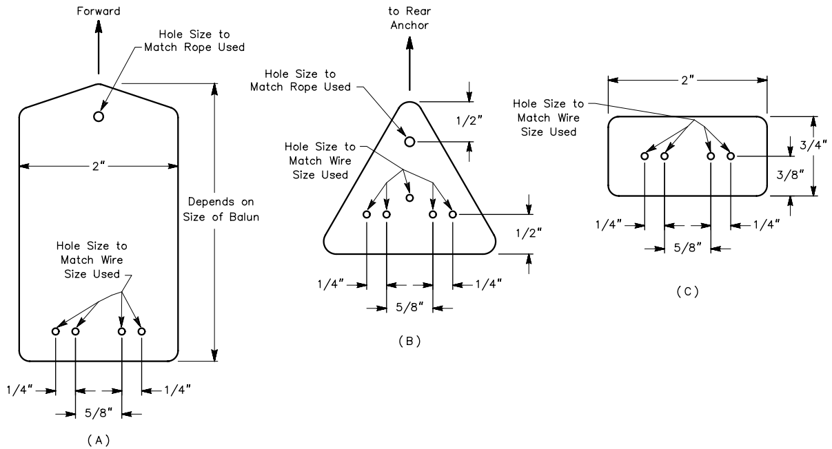
Fig 16—Pieces for the LPDA that require fabrication. At A is the forward connector, made from 1/2-inch Lexan (polycarbonate). At B is the rear connector, also made from 1/2-inch Lexan. At C is the pattern for the phase-line spacers, made from 1/4-inch Plexiglas. Two spacers are required for the array.
