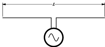
Fig 1—The center-fed dipole antenna. It is assumed that the source of power is directly at the antenna feed point, with no intervening transmission line. Most commonly in amateur applications, the overall length of the dipole is \lambda/2 , but the antenna can in actuality be any length.
