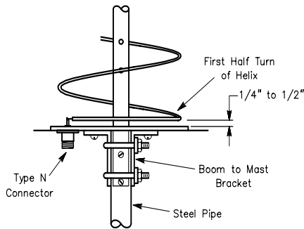
Fig 54—Side view of the helix feed-point assembly. The first half turn of the helix should be kept between \frac{1}{4} and \frac{1}{2} inch above the ground screen during winding. The height above the screen is adjusted for optimum match to a 52\text{-}\Omega transmission line after the antenna is completed.
