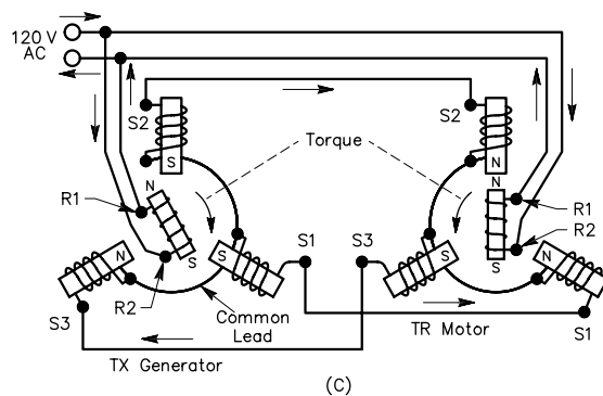
Fig 6—At A, a schematic diagram of the synchro or Selsyn transformer. Connection of two synchros in a repeater loop is shown at B. The drawing at C shows the instantaneous forces in the repeater loop with the rotor shafts at different positions. The “TX” and “TR” notations stand for torque transmitter and torque receiver , respectively. Synchros are sometimes listed in catalogs by these “type” symbols.
