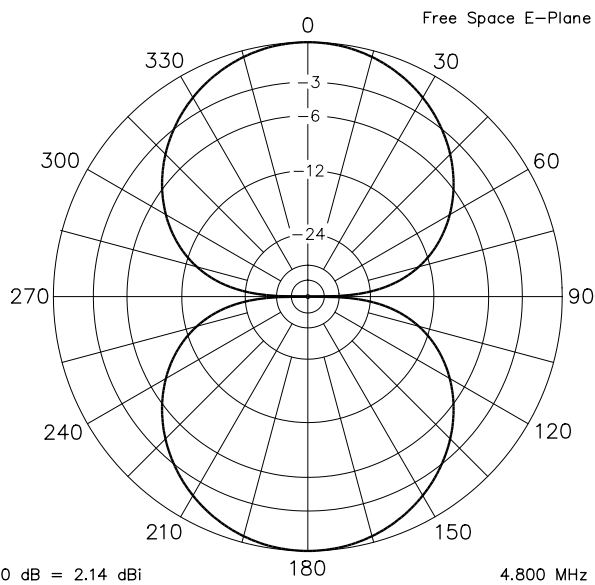
Fig 13—Free-space E-Plane radiation pattern for a 100-foot dipole at its half-wave resonant frequency of 4.80 MHz. This antenna has 2.14 dBi gain. The dipole is located on the line from 90° to 270°.
