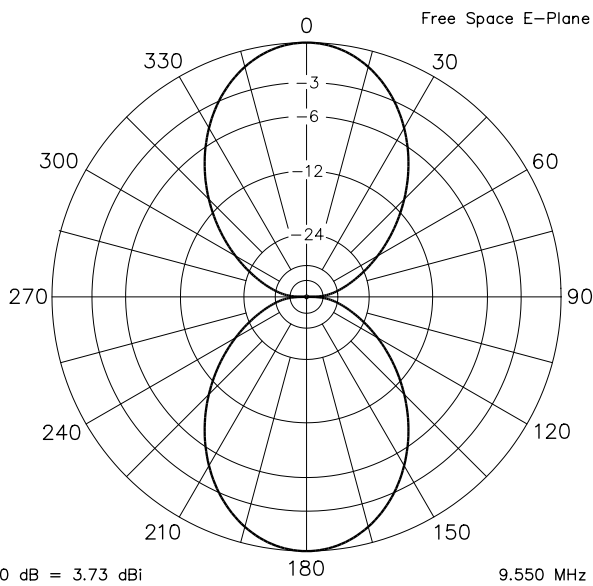
Fig 14—Free-space E-Plane radiation pattern for a 100-foot dipole at its full-wave resonant frequency of 9.55 MHz. The gain has increased to 3.73 dBi, because the main lobes have been focused and sharpened compared to Fig 13.
