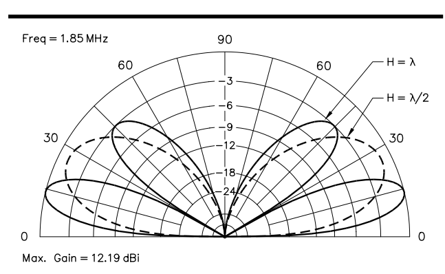
Fig 76 —Elevation-plane pattern for the four-element antenna of Fig 74 when mounted horizontally at two heights over flat ground. Solid line = 1\lambda high; dashed line = \frac{1}{2}\lambda high.
