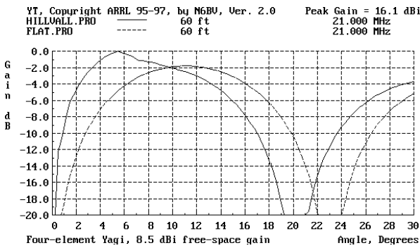
Fig 26 —Elevation response computed by Y T program for single 4-element Yagi at 60 feet above “Hill-Valley” terrain shown in Fig 25. Note that the slope has caused the response in general to be shifted toward lower elevation angles. At 5° elevation, the diffraction components add up to increase the gain slightly above the amount a GO-only analysis would indicate.
