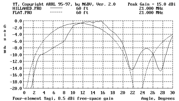
Fig 28 —Elevation response computed by Y T for “Hill-Ahead” terrain shown in Fig 27. Now the hill blocks direct rays and also precludes possibility of any constructive reflections. Above 10°, diffraction components add up together with direct rays to create the response shown.
