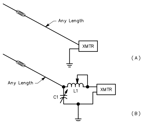
Fig 1 —At A, a random-length wire driven directly from the pi-network output of a transmitter. At B, an L network for use in cases where sufficient loading cannot be obtained with the arrangement as at A. C1 should have about the same plate spacing as the final tank capacitor in a vacuum-tube type of transmitter; a maximum capacitance of 100 pF is sufficient if L1 is 20 to 25 \mu H. A suitable coil would consist of 30 turns of #12 wire, 2 1/2 inches diameter, 6 turns per inch. Bare wire should be used so the tap can be placed as required for loading the transmitter.
