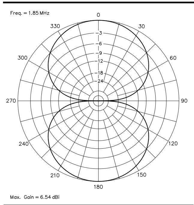
Fig 75 —Free-space E-plane pattern for the antenna shown in Fig 74 , with \frac{1}{8}\lambda spacing. The elements are parallel to the 90^\circ - 270^\circ line in this diagram. Less than a 1^\circ change in half-power beamwidth results when the spacing is changed from \frac{1}{8} to \frac{1}{4}\lambda .
