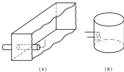
Fig 2 —Coupling coaxial line to waveguide and resonators.
