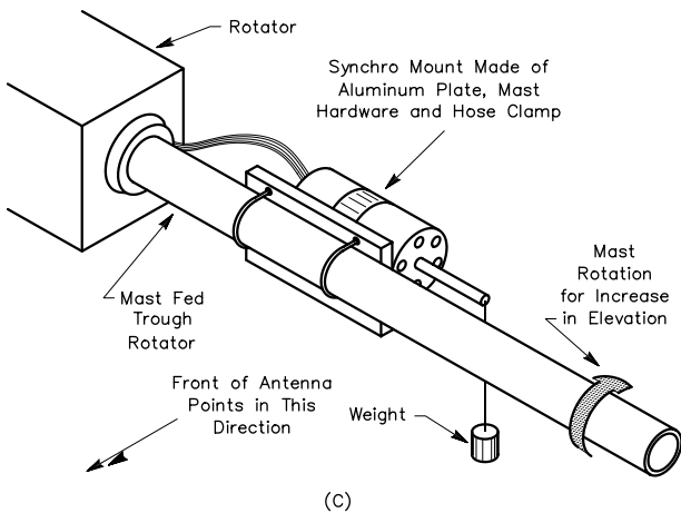
Fig 7 —Shown at A are the circuits for the modified control unit and the synchro power supply. T1, DS1 and C1 are from the stock U-100 or U-110 control box. See text. At B, the mounting method used to secure the synchro motor is shown. Details of the synchro generator mounting are shown at C. See text for description of materials.
