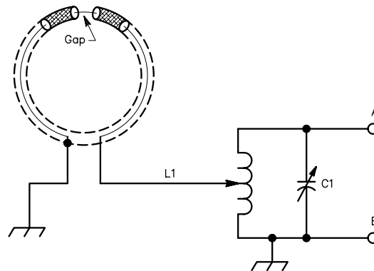
Fig 23 —Input circuit for lower frequency bands. Points A and B are connected to corresponding points in the circuit of Fig 22, substituting for the loop and C1 in that circuit. L1-C1 should resonate within the desired amateur band, but the L/C ratio is not critical. After construction is completed, adjust the position of the tap on L1 for maximum signal strength. Instead of connecting the RDF loop directly to the tap on L1, a length of low impedance line may be used between the loop and the tuned circuit, L1-C1.
