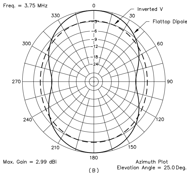
Fig 3—At A, elevation and at B, azimuthal radiation patterns comparing a normal 80-meter dipole and an inverted-V dipole. The center of both dipoles is at 65 feet and the ends of the inverted V are at 20 feet. The frequency is 3.750 MHz.
