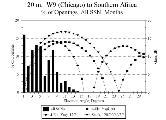
Fig 19—Graph showing 20-meter percentage of all openings from Chicago to Southern Africa, together with overlay of elevation patterns over flat ground for three 20-meter antenna systems. On this long-distance path, higher antennas are most effective.
