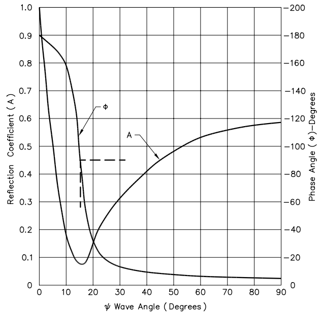
Fig 7 —Reflection coefficient for vertically polarized waves. A and \phi are magnitude and angle for wave angles \Psi . This case is for average earth, ( k = 13 , G = 0.005 S/m), at 21 MHz.
