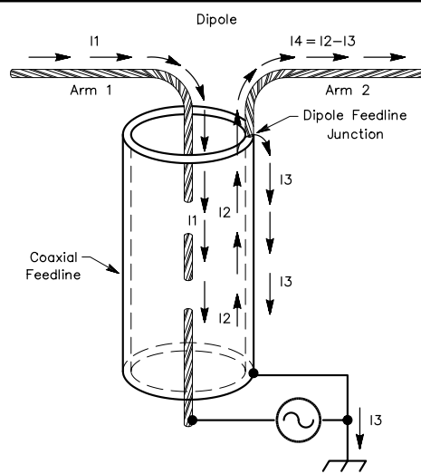
Fig 24—Drawing showing various current paths at feed point of a balanced dipole fed with unbalanced coaxial cable. The diameter of the coax is exaggerated to show currents clearly.
