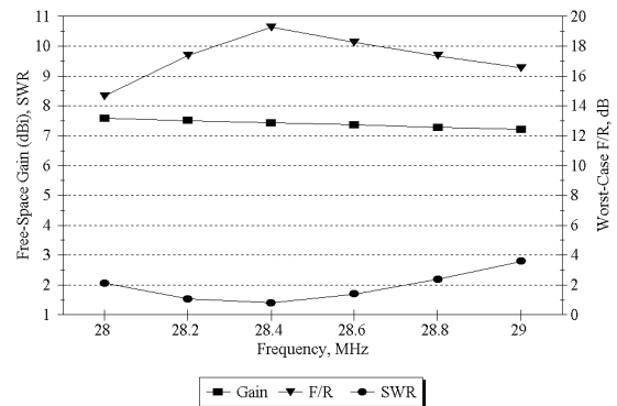
Fig 21—Computed performance of the pentaband two-element quad on 10 meters. The SWR curve is slightly above the target 2:1 at the low end of the band and rises to about 2.2:1 at 28.8 MHz. This unlikely to be a problem, even with rigs with automatic power-reduction due to SWR, since the SWR at the input of a typical coax feed line will be lower than that at the antenna due to losses in the line.
