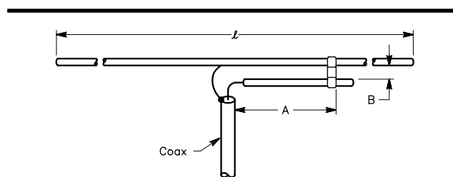
Fig 11—The gamma match, as used with tubing elements. The transmission line may be either 50-Ω or 75-Ω coax.
