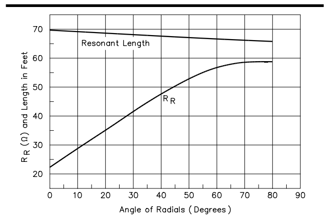
Fig 15—Radiation resistance and resonant length for a 4-radial ground-plane antenna > 0.3 \lambda above ground as a function of radial droop angle ( \theta ).
