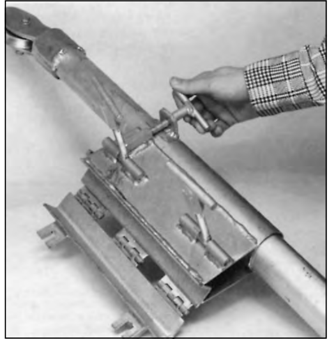
Fig 4 —A gin pole is a mechanical device that can be clamped to a tower leg to aid in the assembly of sections as well as the installation of the mast. The aluminum tubing extends through the clamp and may be slipped into position before the tubing clamp is tightened. A rope should be routed through the tubing and over the pulley mounted at the top.
