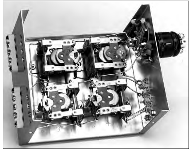
Fig 62—Inside view of relay box. Four relays provide control over five antennas. See text. The relays pictured here are Potter and Brumfield type MR11D.
