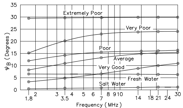
Fig 8 —Pseudo-Brewster angle ( \Psi_B ) for various qualities of earth over the 1.8 to 30-MHz frequency range. Note that the frequency scale is logarithmic. The constants used for each curve are given in Table 2.
