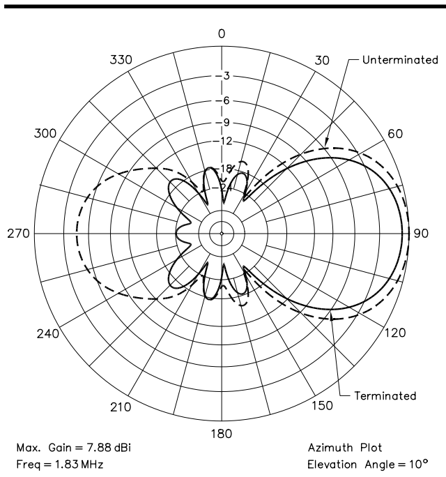
Fig 36—Comparing the azimuthal patterns for a 2-λ Beverage, terminated (solid line) and unterminated (dashed line).
