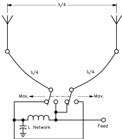
Fig 34—90° fed, 90° phased array reversal switching. All interconnections must be very short. Grounds and cable shields have been omitted for clarity.
