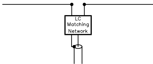
Fig 20 —Efficient broadband matching with an lumped element LC network. The antenna in this example has a resistance of 72 \Omega and a Q of 12. The matching network has an impedance level of 12.4 \Omega , and a Q of 200. The feed line is 50\text{-}\Omega coax, and the matching network provides an impedance step-up ratio of 2.8:1.
