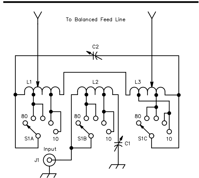
Fig 14—Schematic diagram of the link coupler. The connections marked as “to balanced feed line” are steatite feedthrough insulators. The arrows on the other ends of these connections are alligator clips.
