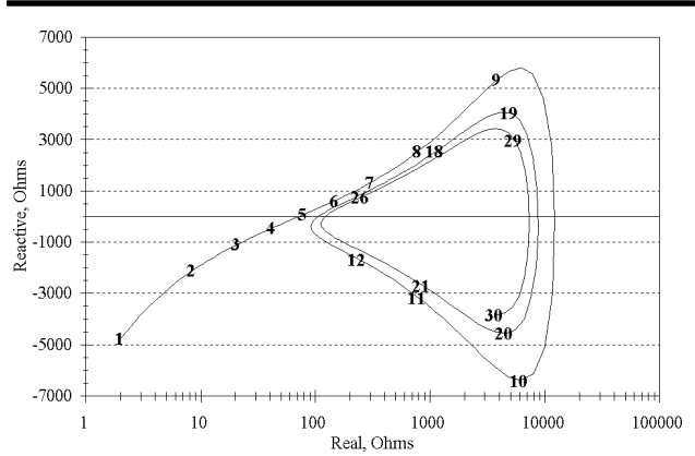
Fig 2—Feed-point impedance versus frequency for a theoretical 100-foot long dipole, fed in the center in free space, made of extremely thin 0.001-inch diameter wire. The y-axis is calibrated in positive (inductive) series reactance up from the zero line, and negative (capacitive) series reactance in the downwards direction. The range of reactance goes from -6500 \Omega to +6000 \Omega . Note that the x-axis is logarithmic because of the wide range of the real, resistive component of the feed-point impedance, from roughly 2 \Omega to 10,000 \Omega . The numbers placed along the curve show the frequency in MHz. Note that the curve spirals in towards 377 \Omega , the theoretical intrinsic impedance of free space.
