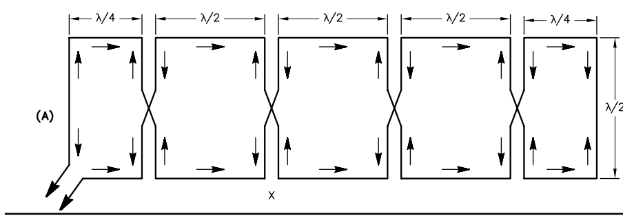
Fig 46 —Typical Sterba array, a 10-element version.
