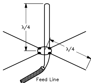
Fig 17—The folded monopole antenna. Shown here is a ground plane of four \lambda/4 radials. The folded element may be operated over an extensive counterpoise system or mounted on the ground and worked against buried radials and the earth. As with the folded dipole antenna, the feed-point impedance depends on the ratios of the radiator conductor sizes and their spacing.
