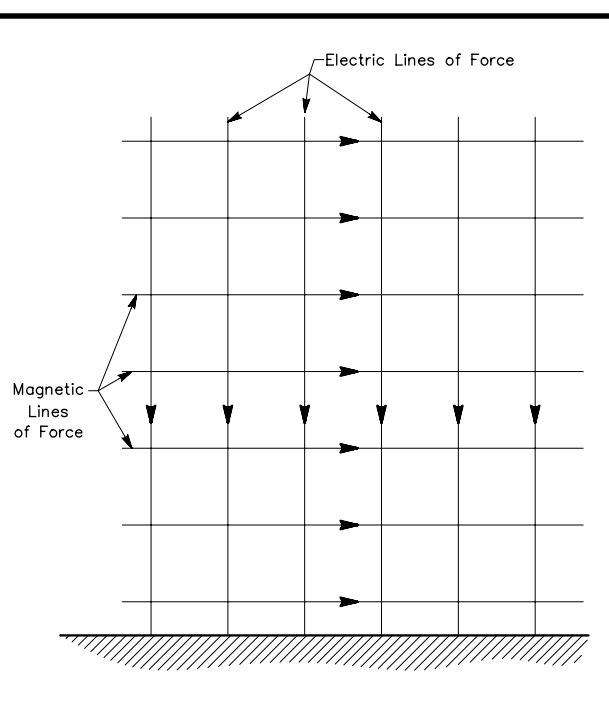
Fig 1 —Representation of the magnetic and electric fields of a vertically polarized plane wave traveling along the ground. The arrows indicate instantaneous directions of the fields for a wave traveling perpendicularly out of the page toward the reader. Reversal of the direction of one set of lines reverses the direction of travel. There is no change in direction when both sets are reversed. Such a dual reversal occurs in fact once each half cycle.
