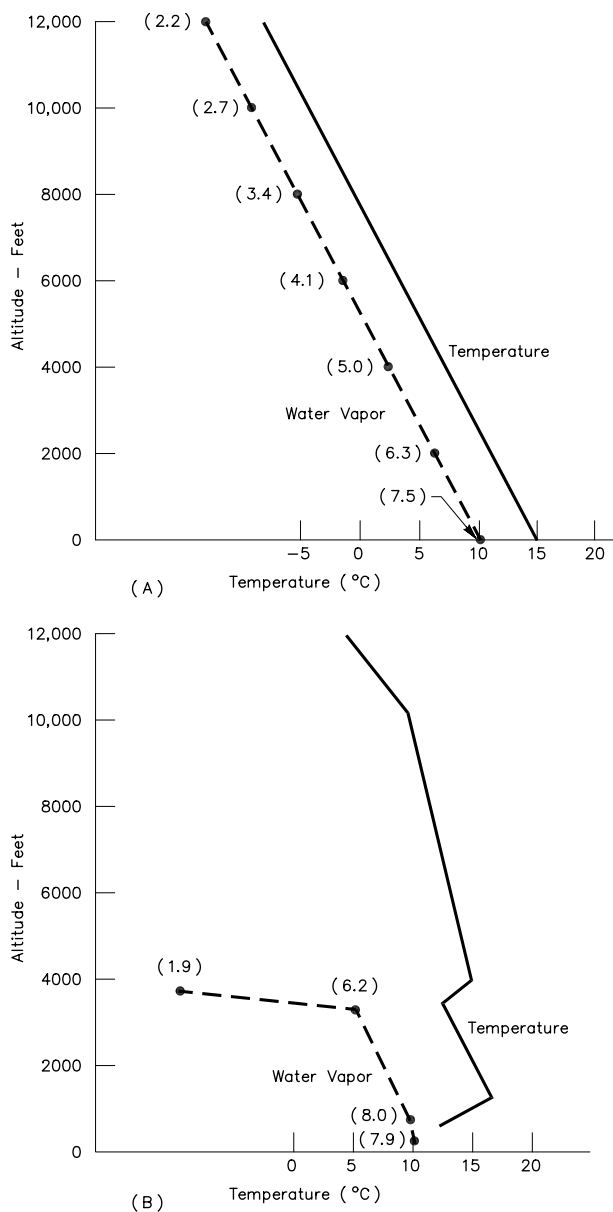
Fig 8—Upper air conditions that produce extended-range communication on the VHF bands. At the top is shown the US Standard Atmosphere temperature curve. The humidity curve (dotted) is what would result if the relative humidity were 70%, from ground level to 12,000 feet elevation. There is only slight refraction under this standard condition. At the bottom is shown a sounding that is typical of marked refraction of VHF waves. Figures in parentheses are the “mixing ratio”—grams of water vapor per kilogram of dry air. Note the sharp break in both curves at about 3500 feet.
