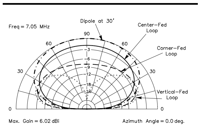
Fig 31 —Elevation-plane responses for the 7-MHz loop, fed at different points. The solid line is for feeding it at the bottom; the dashed line is for feeding it at either corner at the bottom; the dotted line is for feeding it at the center of one of the vertical sides. For reference, the response of a simple flattop horizontal dipole at 30 feet in height is shown as a dashed-dotted line.
