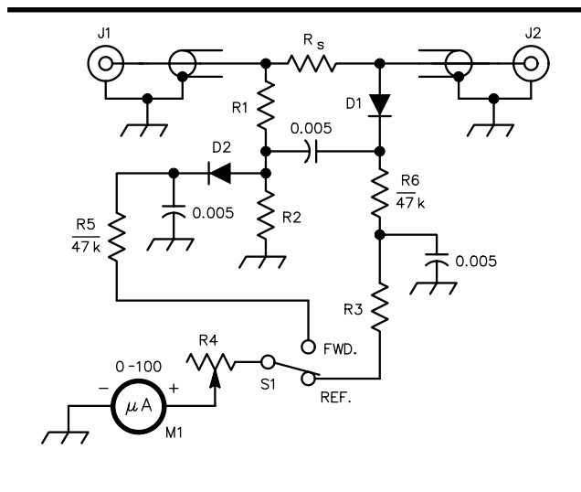
Fig 5—Resistance bridge for SWR measurement. Capacitors are disc ceramic. Resistors are 1/2-watt composition except as noted below. D1, D2— Germanium diode, high back resistance type (1N34A, 1N270, etc). J1, J2— Coaxial connectors, chassis-mounting type. M1— 0-100 dc microammeter. R1, R2— 47 \Omega , 1/2-W composition (see text). R3— See text. R4— 50-k \Omega volume control. R_S — Resistance equal to line Z_0 (1/2 or 1 W composition). S1— SPDT toggle.
