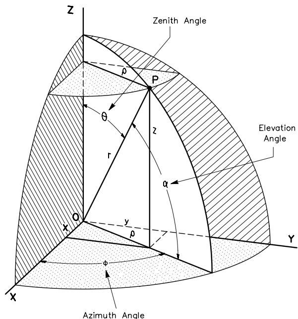
Fig 20 —Diagram showing polar representation of a point P lying on an imaginary sphere surround a point-source antenna. The various angles associated with this coordinate system are shown referenced to the x, y and z-axes.
