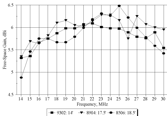
Short-Boom LPDAs: 14' to 18.5' Free-Space Gain: 14 to 30 MHz
