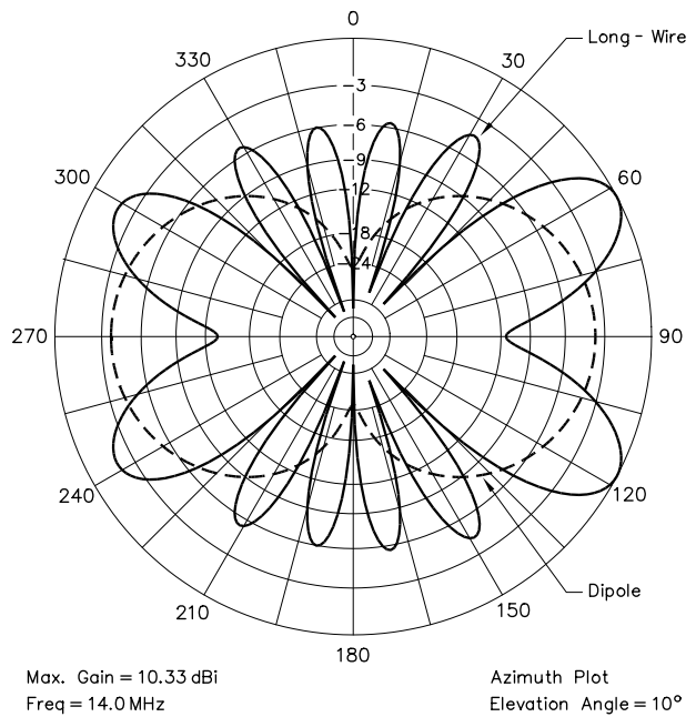
Fig 4—An azimuthal-plane comparison between a 3- \lambda (209 feet long) long-wire (solid line) and the comparison 1/2 - \lambda dipole (dashed line) at 70 feet high (1 \lambda ) at 14 MHz.
