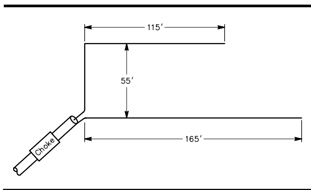
Fig 52—A single elevated radial can be used for the inverted L. This changes the directivity slightly.
