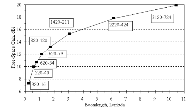
Fig 10—Theoretical gain versus boom length for 20-meter Yagis designed for optimal combination of F/R, SWR and gain across the entire 14.0 to 14.35 MHz band. The theoretical gain approaches 20 dBi for a gigantic 724-foot boom, populated with 31 elements. Such a design on 20 meters is not too practical, of course, but can readily be achieved on a 24-foot boom on 432 MHz.
