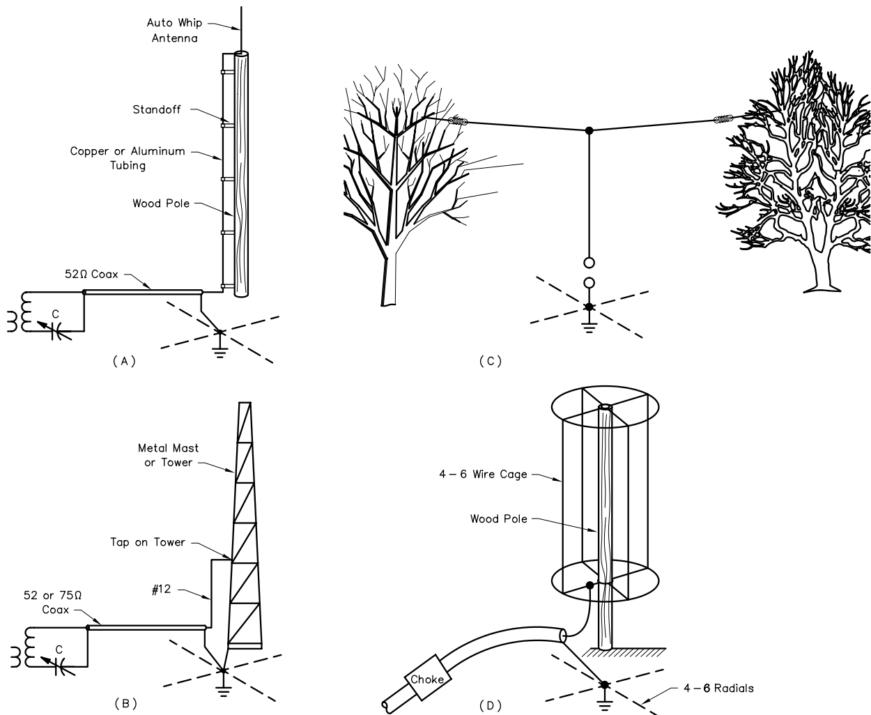
Fig 19 —Vertical antennas are effective for 3.5 or 7-MHz work. The \lambda/4 antenna shown at A is fed directly with 50-Ω coaxial line, and the resulting SWR is usually less than 1.5 to 1, depending on the ground resistance. If a grounded antenna is used as at B, the antenna can be shunt fed with either 50 or 75-Ω coaxial line. The tap for best match and the value of C will have to be found by experiment. The line running up the side of the antenna should be spaced 6 to 12 inches from the antenna. If tall trees are available the antenna can be supported from a line suspended between the trees, as shown in C. If the vertical section is not long enough then the horizontal support section can be made of wire and act as top loading. A pole or even a grounded tower can be used with elevated radials if a cage of four to six wires is provided as shown in D. The cage surrounds the pole which may be wood or a grounded conductor.
