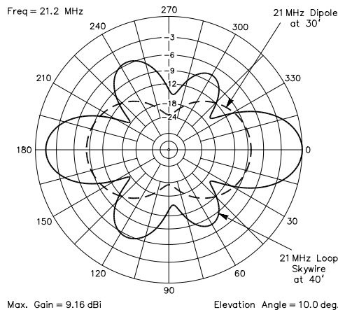
Fig 27—At A, azimuth-plane response of 142-foot long, 7-MHz Loop Skywire, 40 feet in the air at 7.2 MHz, compared with 1/2\lambda dipole 30 feet in the air. At B, response of same Loop Skywire at 14.2 MHz, compared with 1/2\lambda 14.2-MHz dipole 30 feet in the air. Now the loop has some advantage in certain directions. At C, response of the same Loop Skywire at 21.2 MHz compared to a 21.2-MHz dipole at 30 feet. Here, the Loop Skywire has more gain in almost all directions than the simple dipole. All azimuth-plane patterns were made at 10° elevation.
