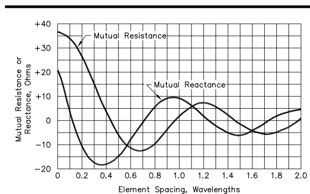
Fig 20—Mutual impedance between two parallel \frac{1}{4} \lambda vertical elements. Multiply the resistance and reactance values by two for \frac{1}{2}\text{-}\lambda dipoles. Values for vertical elements that are between 0.15 \lambda and 0.25 \lambda high may be approximated by multiplying the given values by R_R/36 , where R_R is the radiation resistance of the vertical given by graphs in Chapter 2.
