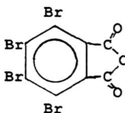
Tetrabromophthalic Anhydride
