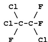
1,1,2-Trichloro- 1,2,2-Trifluoroethane (Freon TF) .
