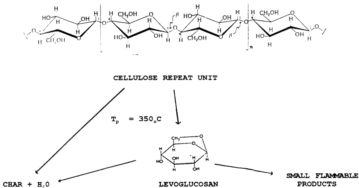
Figure 65. Cellulose Pyrolysis Products
