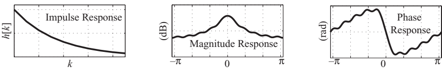
Figure 6.4 Impulse response h[k] (left) two-sided magnitude frequency response (middle), and two-sided phase response (right).
