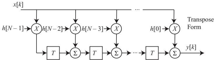
Figure 11.3 Transpose Nth-order FIR architecture.
