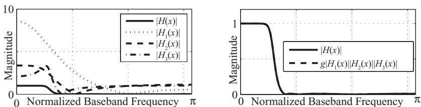
Figure 15.11 System output and individual subsystem responses. The maximum subsystem gain ranges from about 2 to nearly 9. The scaled by “ g ” cascaded response of the subsystems and original transfer function are seen to be in full agreement.
