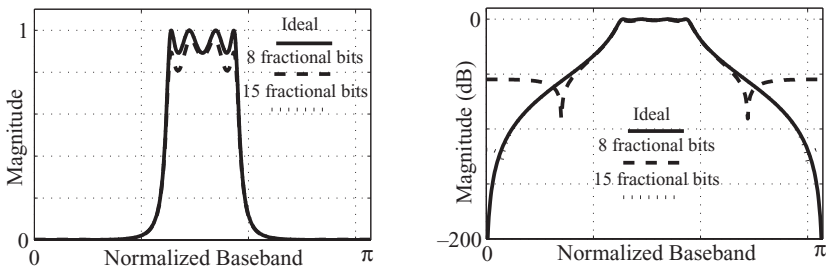
Figure 16.6 Eighth-order band-pass filter showing the magnitude frequency response of the ideal and 8- and 15-fractional-bit direct II filters (left) and in decibels (right).
