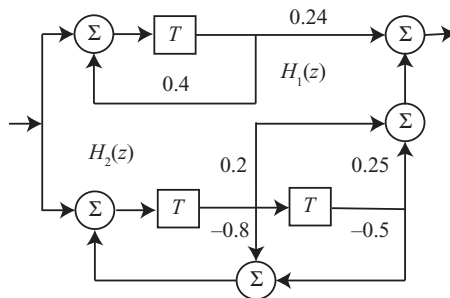
Figure 15.13 Parallel third-order IIR Filter.
