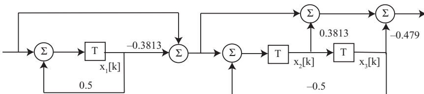
Figure 15.12 Cascade IIR filter.
