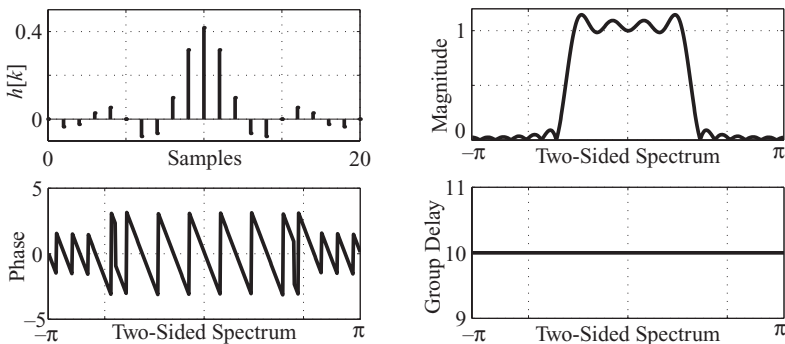
Figure 7.12 Twenty-first-order window (rectangular) FIR truncated Fourier design example showing realized impulse response (top left), two-sided spectrum (top right), phase response (lower left), and group delay (lower right).
