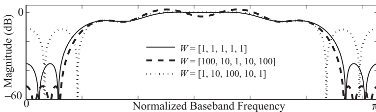
Figure 9.11 Multiple 31st-order equiripple Type 1 five-band linear phase equiripple FIRs with varying error weights.
