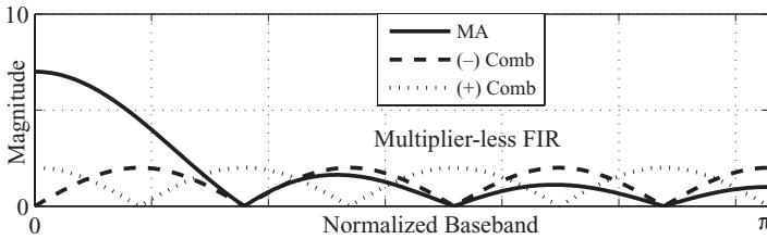
Figure 10.4 Magnitude frequency responses for an unnormalized MA FIR ( h_1[k] = \{1, 1, 1, 1, 1, 1, 1\} ) ( N = 8 ), a (-) comb filter ( h_2[k] = \{1, 0, 0, 0, 0, 0, -1\} ) ( N = 7 ), and (+) comb filter ( h_3[k] = \{1, 0, 0, 0, 0, 0, 1\} ) ( N = 7 ).
