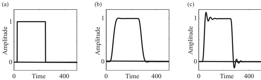
Figure 2.10 Pulse response of a Bessel and Chebyshev low-pass filter. (a) Pulse waveform; (b) Bessel filter; (c) Chebyshev filter.
