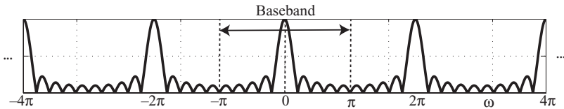
Figure 6.2 Magnitude frequency response of a 10th-order MA FIR over the normalized frequency range \varpi \in [-4\pi, 4\pi] .
