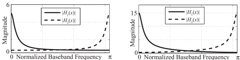
Figure 15.9 Magnitude frequency responses of subfilters. Proximity pairing (left) and nonproximity pairing (right).
