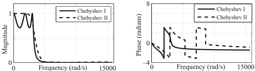
Figure 12.7 Chebyshev I and II filters showing magnitude frequency (left) and phase responses (right).
