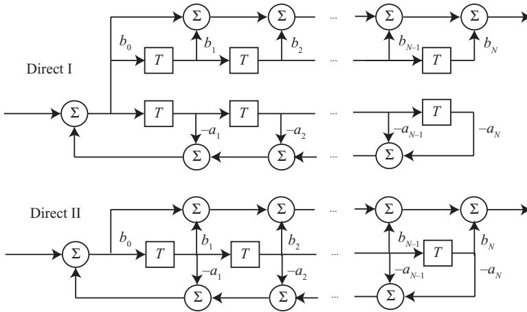
Figure 15.1 Direct I (top) and II (bottom) architectures. Coefficients a_i and b_i correspond to the multipliers of z^{-i} in D(z) and N(z) . State x_1[k] is closest to the output; state x_N[k] is closest to the input.
