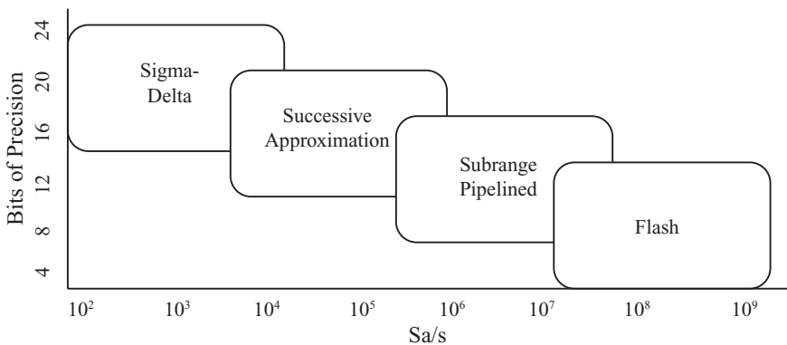
Figure 4.3 ADC precision as a function of performance (Sa/s) and architecture.
