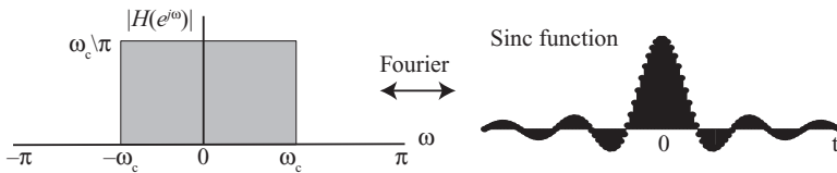
Figure 6.3 Ideal low-pass filter magnitude frequency response (left) and impulse response (right).
