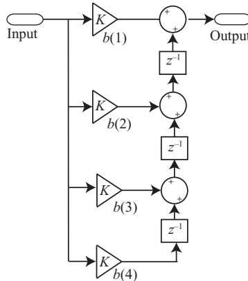
Figure 11.4 A fourth-order (third-order MATLAB) transpose FIR architecture (MATLAB style).
