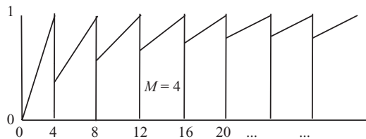
Figure 11.21 Speed-up potential of a four-multiplier FIR as a function of filter order.
