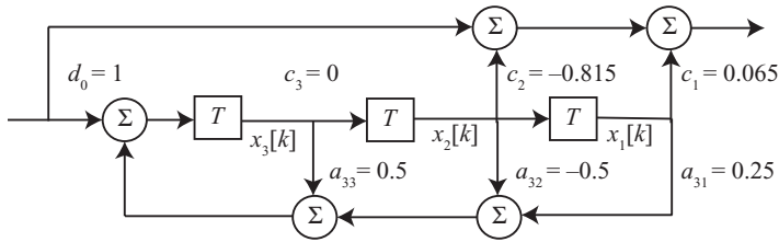
Figure 15.3 Third-order state-determined digital filter reduced to a direct II architecture showing traditional state assignments.
