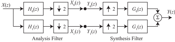
Figure 19.5 QMF filter architecture.
