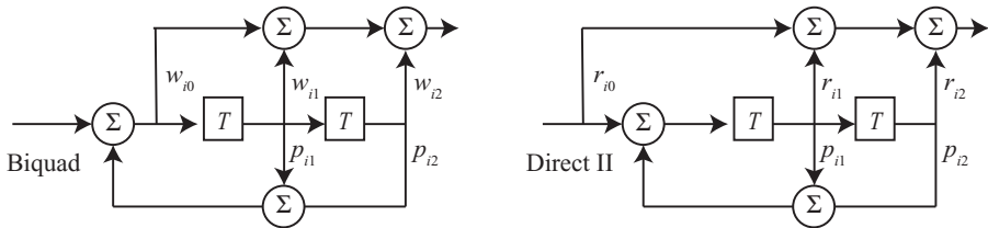
Figure 15.8 Implementation of a second-order section as a biquad H_i(z) = (w_{i0} + w_{i1}z^{-1} + w_{i2}z^{-2})/(1 - p_{i1}z^{-1} - p_{i2}z^{-2}) (left) or direct II section H_i(z) = r_{i0} + (r_{i1}z^{-1} + r_{i2}z^{-2})/(1 - p_{i1}z^{-1} - p_{i2}z^{-2}) (right).
