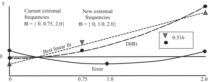
Figure 9.2 Second iteration outcome with the maximal error at \omega = 1.0 .
