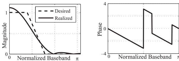
Figure 8.3 Magnitude frequency response (left) and linear phase response in radians (right).
