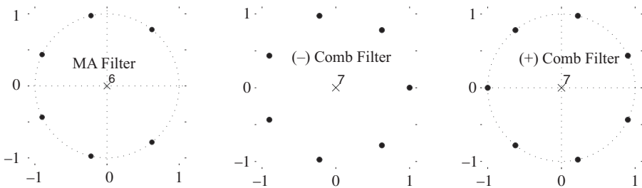
Figure 10.3 Pole-zero distributions of moving average and comb FIR filters all having numerators of (1 - z^{-7}) . Notice that the zeros are separated by angle 2\pi/7 radians.
