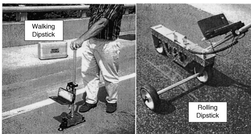
FIGURE 19.60 Walking and rolling dipstick (Source: Korchi, 2000) (used by permission).
