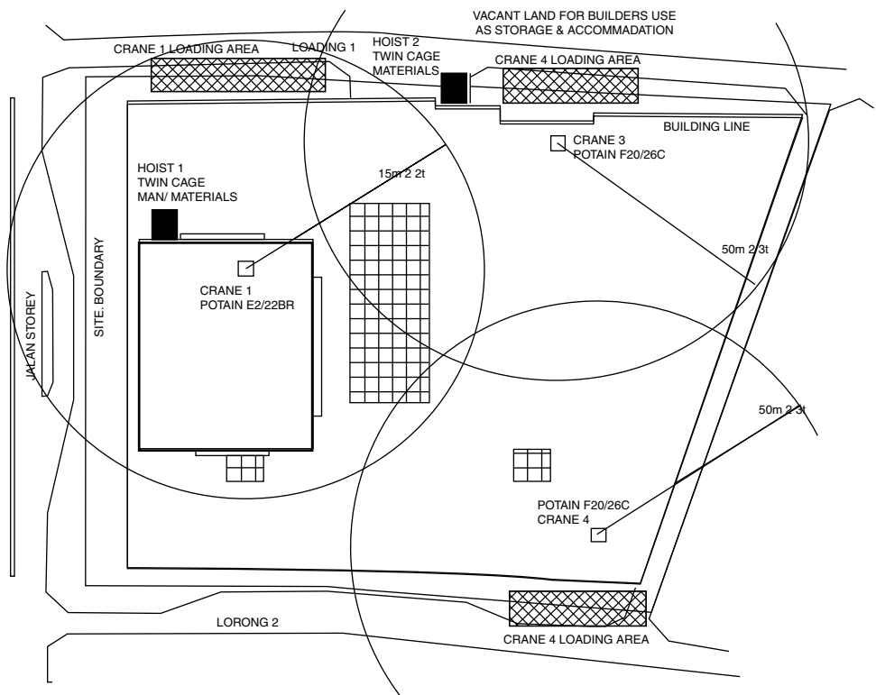
FIGURE 15.6 Site layout plan as part of a GMS.
