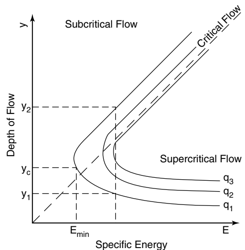
FIGURE 13.11 Specific energy vs. depth of flow (Source: Adapted from FHWA Highways in the River Environment , Training and Design Manual, 1990).
