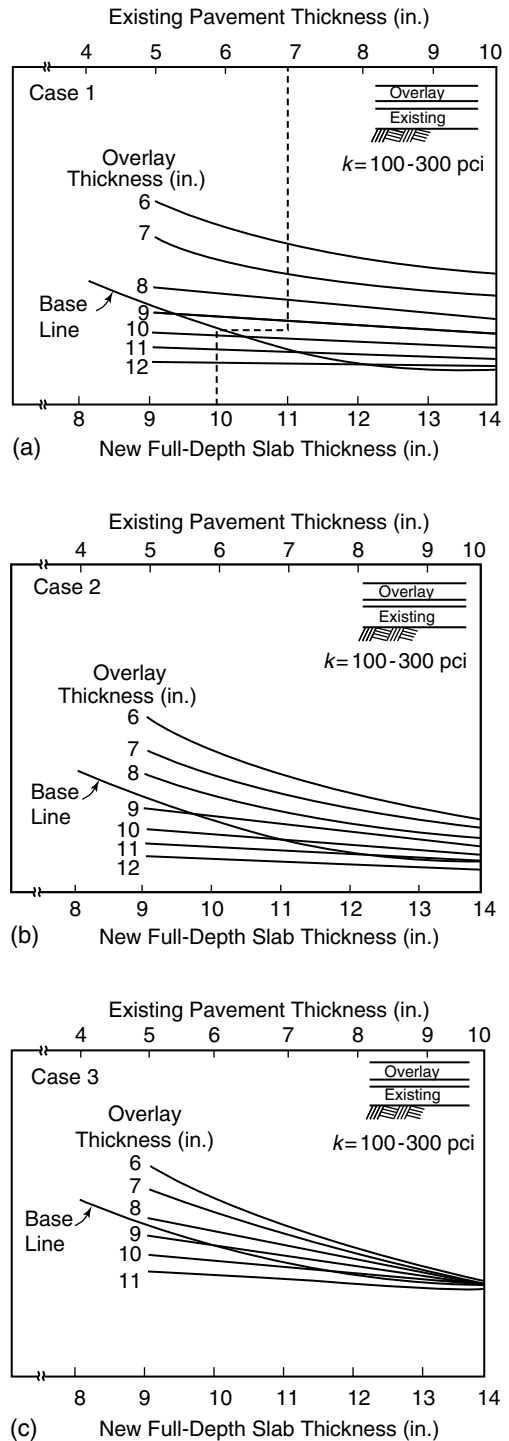
FIGURE 12.5 PCA design charts for unbonded overlays. Source: Proceedings of Third International Conference on Concrete Pavement Design and Rehabilitation. April 23 to 25, 1985, Purdue University, pp. 378–379. With permission.
