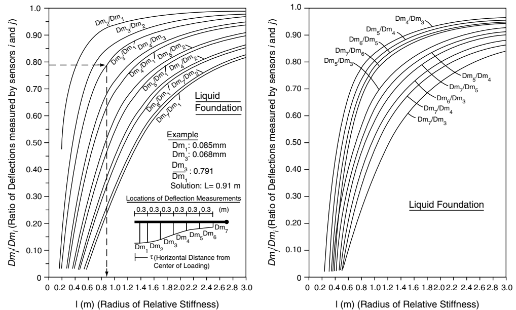
FIGURE 20.4 Graphical solution for backcalculating radius of relative stiffness of rigid pavement on liquid foundation (after Fwa et al., 1997, with permission).
