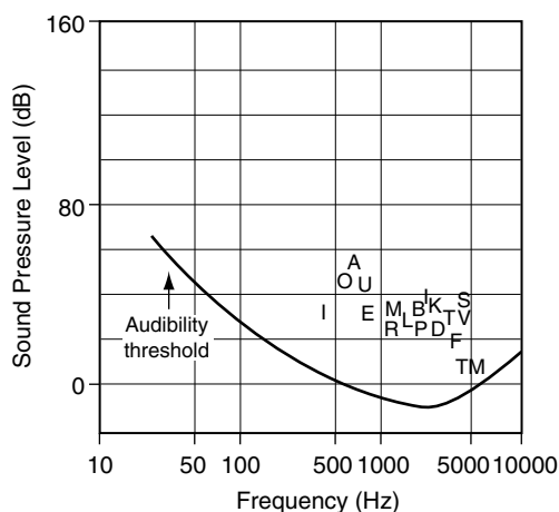
FIGURE 5.3 Human auditory response.
