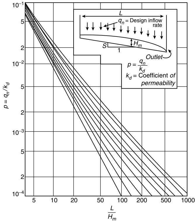
FIGURE 13.40 Chart for estimating maximum depth of flow caused by steady inflow (Source: From Highway Sub-Drainage Design , Report No. FHWA-TS-80-224, US Department of Transportation, Washington, DC, August 1980).
