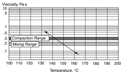
FIGURE 7.11 Selection of laboratory mixing and compaction temperatures. [Source: From Asphalt Institute, 2001. Superpave Mix Design , Superpave Series No. 2 (SP-2), Lexington, Kentucky. With permission.]
