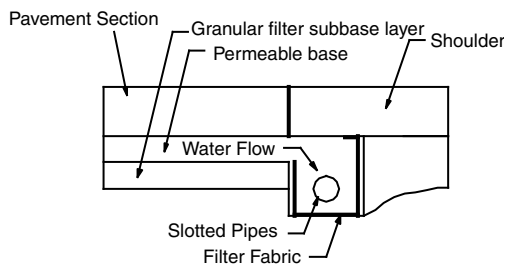
FIGURE 14.5 Under-drain system.
