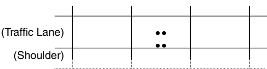
FIGURE 9.16 Critical loading position for fatigue analysis.
