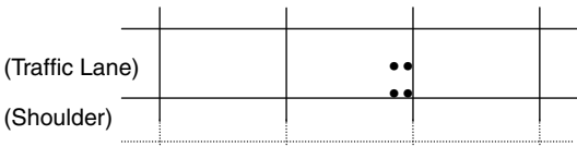
FIGURE 9.18 Critical loading position for erosion analysis.
