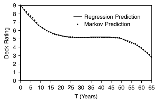
FIGURE 22.10 Comparison of Markov and regression predictions.
