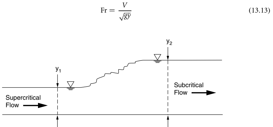
FIGURE 13.9 Hydraulic jump situation.
