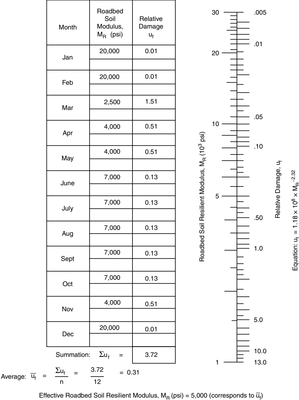
FIGURE 8.21 Worksheet for estimating effective roadbed soil resilient modulus (AASHTO, 1993).
