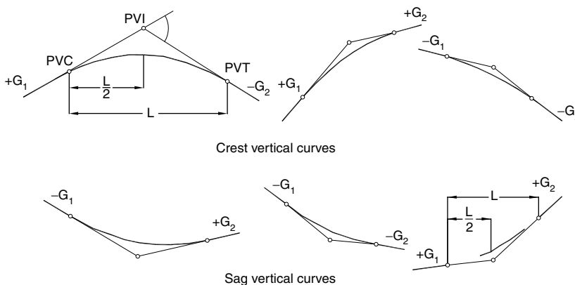
FIGURE 6.2 Crest vertical curves and sag vertical curves.
