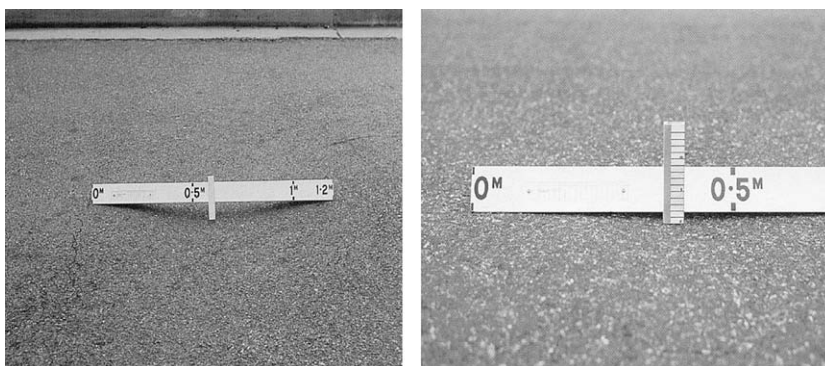
FIGURE 19.5 Depressions in flexible pavements (Source: Austroads, 1987).
