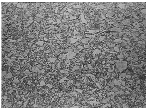
FIGURE 8.12 Polished aggregate.
