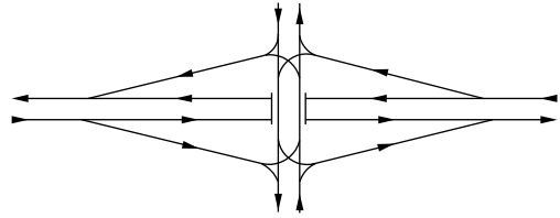
FIGURE 6.13 Diamond interchange.
