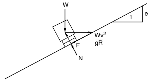
FIGURE 6.5 Super-elevation.
