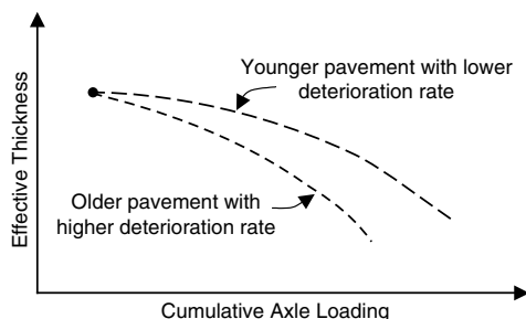
FIGURE 12.4 Remaining life concept for overlay design.
