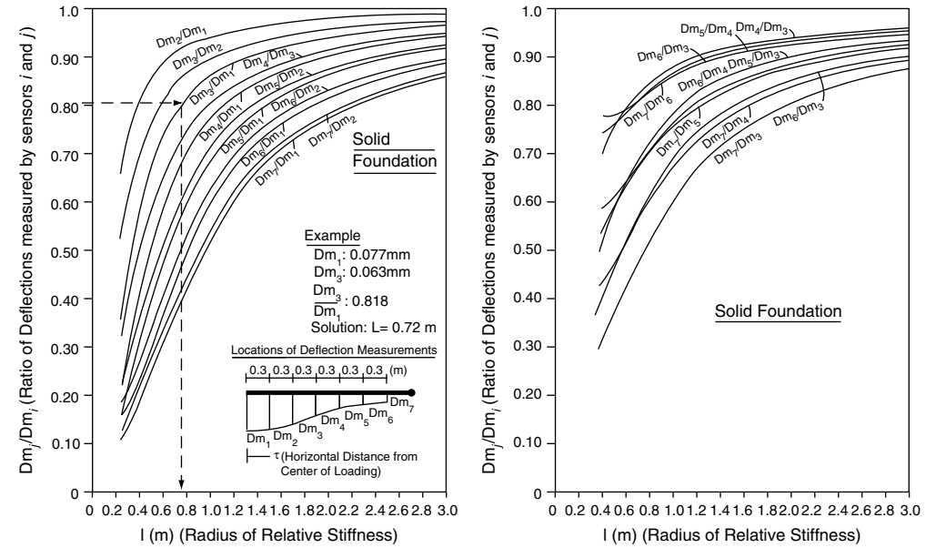
FIGURE 20.5 Graphical solution for backcalculating radius of relative stiffness of rigid pavement on solid foundation (after Fwa et al., 1997d, with permission).
