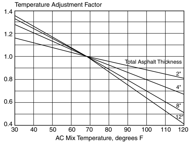
FIGURE 11.1 Adjustment to d_o for AC mix temperature for pavement with granular or asphalt-treated base. (Source: From Guide for Design of Pavement Structures, Volume I, 1993 by AASHTO, Washington, DC. With permission.)
