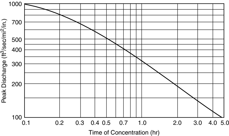
FIGURE 13.4 Peak discharge vs. time of concentration for 24 h, Type II storm distribution (Source: From Soil Conservation Service, 1973. A Method for Estimating Volume and Rate of Runoff in Small Watersheds ).
