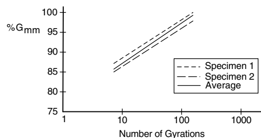
FIGURE 7.13 Example gyratory compaction data and curve.
