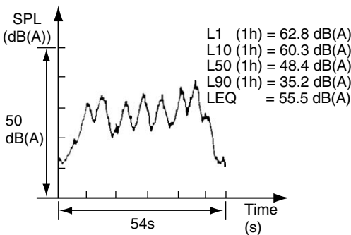
FIGURE 5.4 Noise/time history of a constant speed driveby of a platoon of seven cars.
