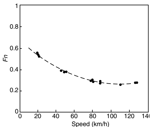
FIGURE 21.1 Frictional resistance versus speed.
