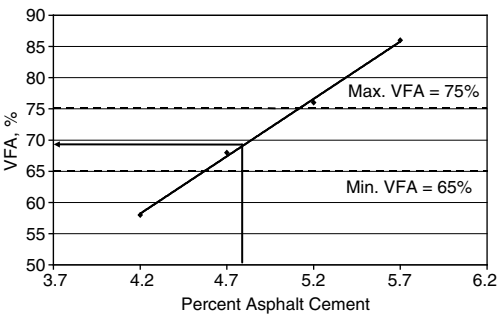
FIGURE 7.16 Percent VFA vs. percent asphalt content.
