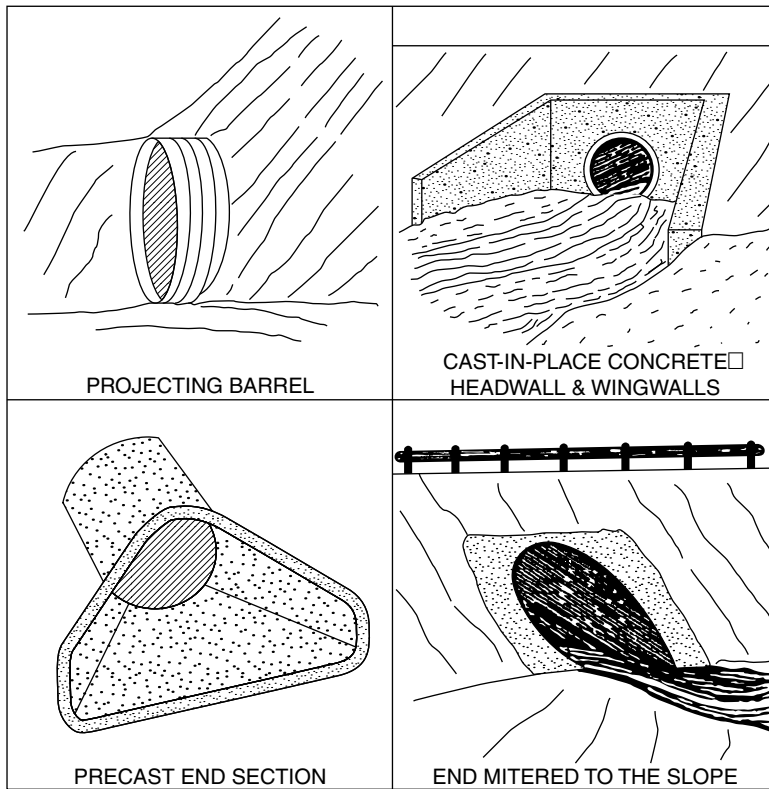
FIGURE 13.27 Four standard inlet types (Source: From Normann, J.M., Houghtalen, R.J., and Johnston, W.J., in Hydraulic Design of Highway Culverts , Report No. FHWA-IP-85-15, US Department of Transportation, Office of Implementation, McLean, VA, September 1985).
