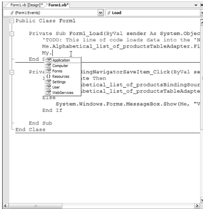
Figure 2-12: Using IntelliSense.
