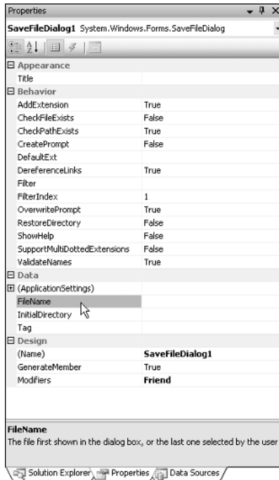
Figure 16-3: Options for the SaveFile Dialog control .
