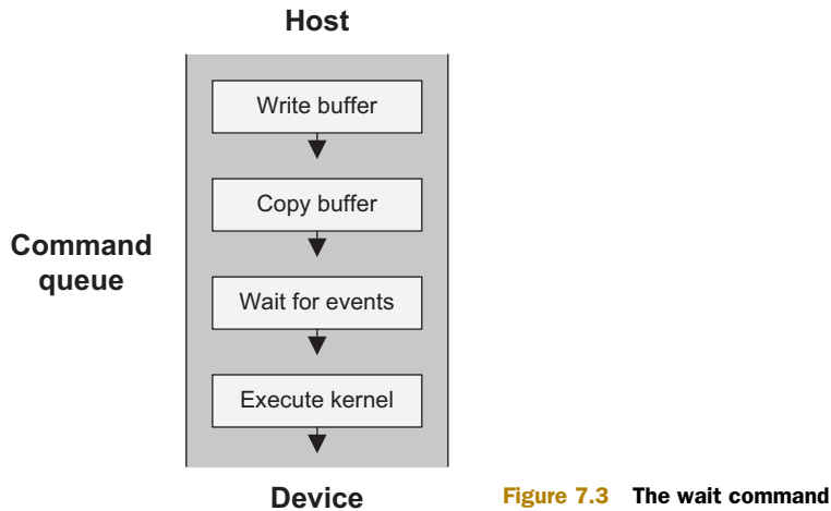
Figure 7.3 The wait command
