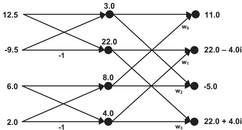
Figure 14.10 Butterfly diagram of a four-element FFT
