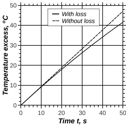
Figure 6.11: Slug response with and without heat loss for q = 10000 \text{ W/m}^2
