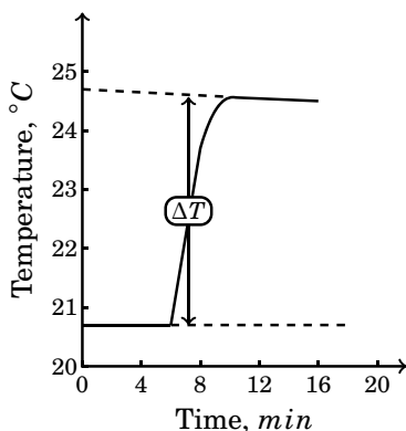
Figure 11.15: Bomb calorimeter data for Example 11.6
