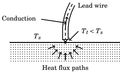
Figure 5.1: Temperature measurement of a surface
