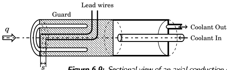
Figure 6.9: Sectional view of an axial conduction guarded heat flux probe
