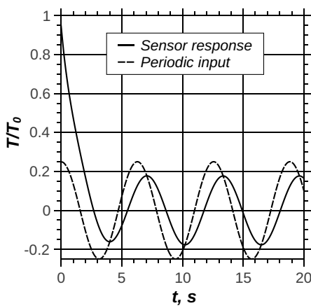
Figure 4.66: Amplitude and phase of a first order system subject to periodic input
