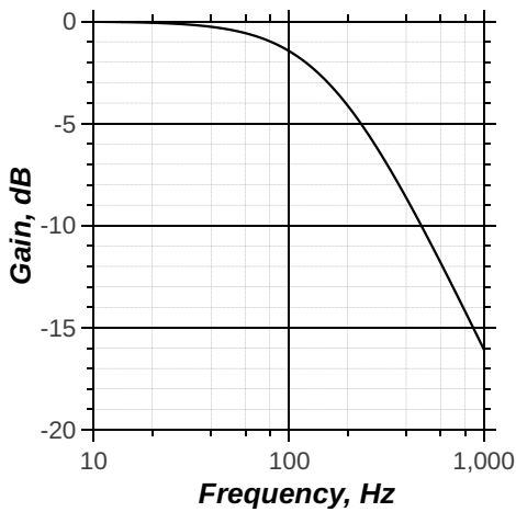
Figure 15.15: Low pass filter frequency response
