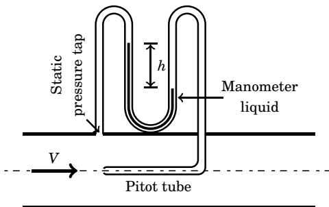
Figure 8.2: Pitot tube arranged to measure fluid velocity
