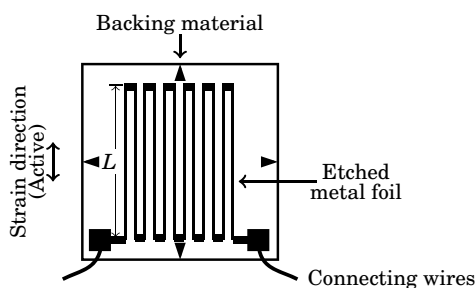
Figure 7.11: Strain gauge construction schematic (not to scale). L is the active gauge length, \blacktriangle - Alignment marks
