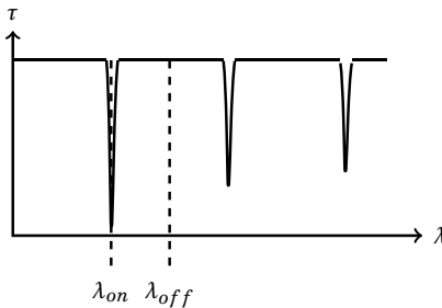
Figure 13.4: Principle of differential absorption
