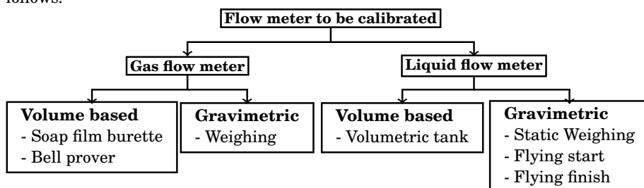
Figure 9.19: Different methods of calibration of flow meters
