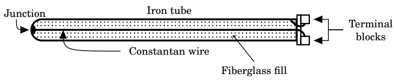
Figure 4.22: Bayonet or pencil type of thermocouple probe
