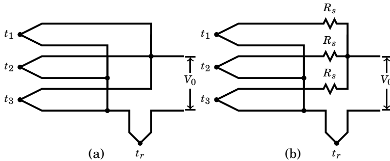
Figure 4.25: Thermocouples connected in: (a) parallel (b) parallel with “swamp” resistors R_s
