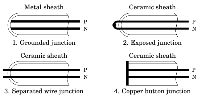
Figure 4.20: Types of thermocouple junctions
