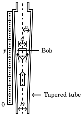
Figure 9.14: Schematic representation of a rotameter
