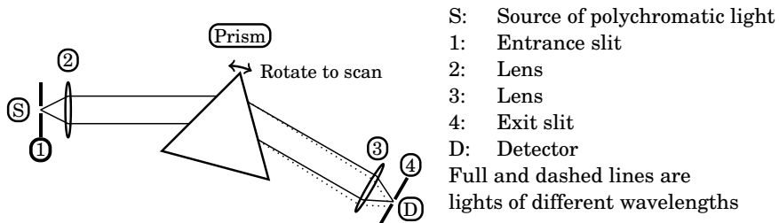
Figure 12.6: Schematic of a Prism Monochromator
