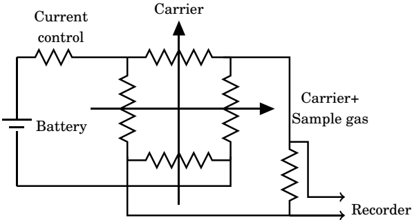
Figure 13.10: Thermal conductivity detector schematic
