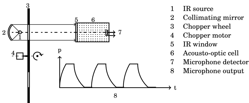
Figure 13.1: Schematic of an acousto-optic cell
