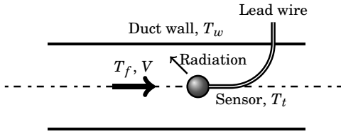
Figure 5.11: Radiation and lead wire conduction errors in temperature measurement with T_f > T_t > T_w
