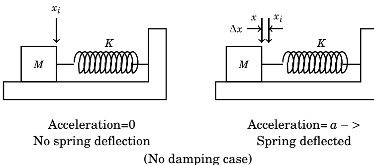
Figure 14.6: Spring mass system under the influence of an external force
