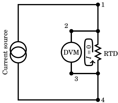
Figure 4.33: Practical circuit with four wire RTD
