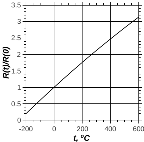
Figure 4.28: Characteristics of a Platinum resistance thermometer
