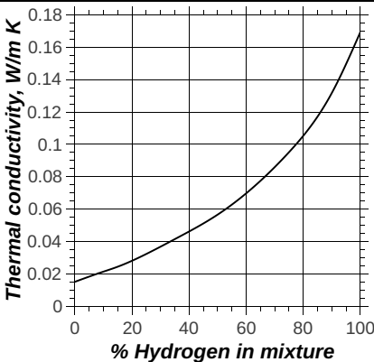
Figure 13.9: Thermal conductivity of a mixture of Hydrogen and Carbon dioxide
