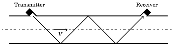
Figure 8.36: Method of increasing path length in TOF measurement
