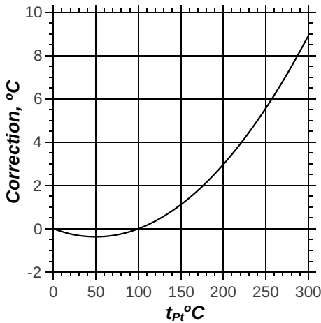
Figure 4.30: Callendar correction as a function of t_{Pt}
