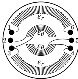
Figure 7.18: Strain gauges mounted on a diaphragm gauge (Based on “Strain Gages and Instruments”, Tech Note TN-510-1, Document Number: 11060, Revision: 01-Nov-2010, Vishay Precision Group accessible at www.micro-measurements.com )
