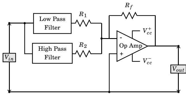
Figure 15.18: Notch filter followed by a summing amplifier to reject an unwanted frequency component
