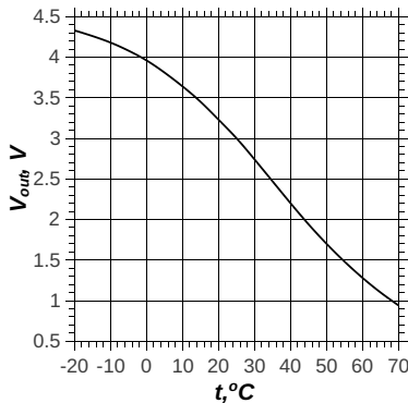
Figure 4.40: Variation of voltmeter reading with temperature
