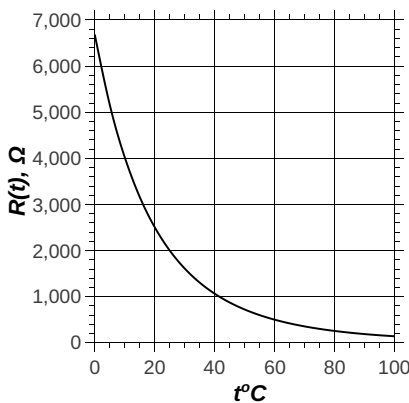
Figure 4.36: Variation of resistance of thermistor with temperature
