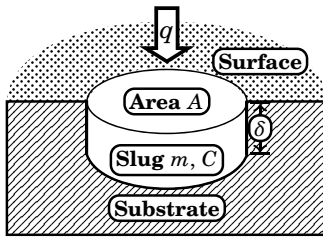
Figure 6.10: Slug type heat flux sensor
