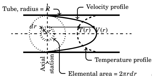
Figure 10.4: Flow of a fluid in a circular tube
