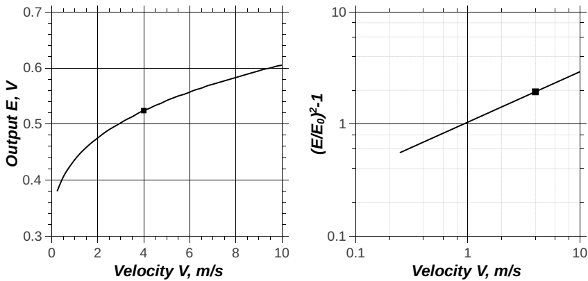
Figure 8.17: Actual and linearized response of hot wire sensor of Example 8.5 in CT mode
