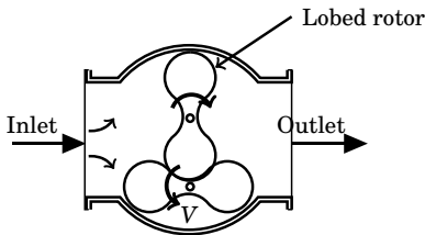
Figure 9.16: Positive Displacement type with Lobed Rotors
