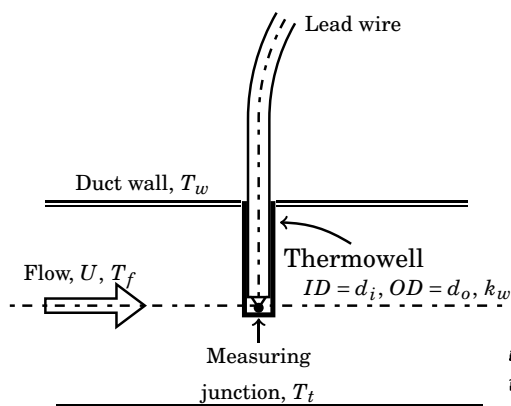
Figure 5.14: Nomenclature for the thermometer well problem
