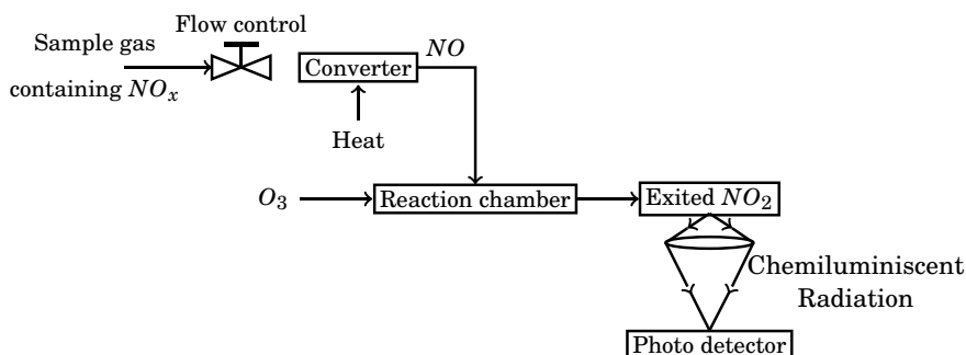
Figure 13.6: Schematic of a chemiluminescent \text{NO}_x analyzer
