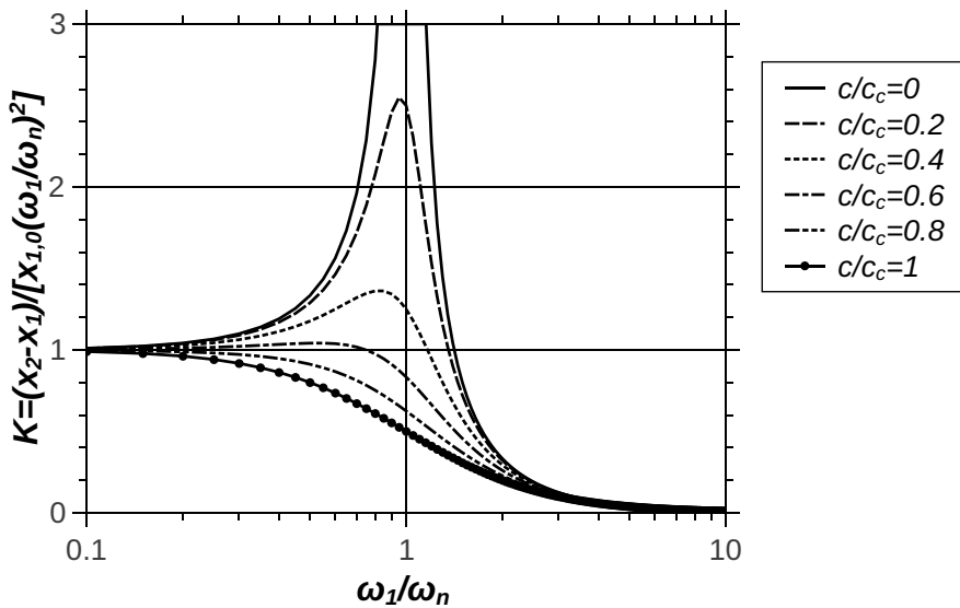
Figure 14.13: Acceleration response of a second order system
