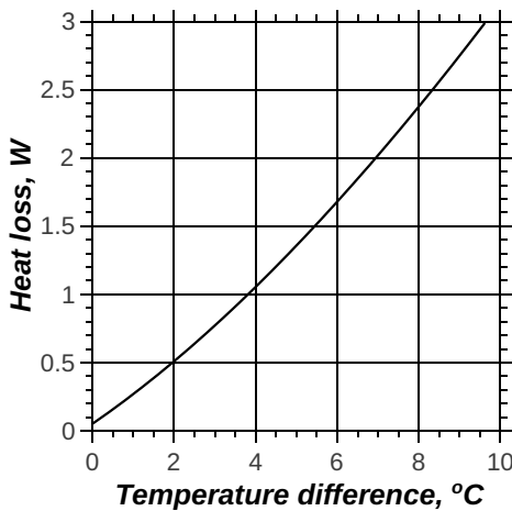
Figure 11.5: Heat loss calibration data for a radial flow thermal conductivity apparatus
