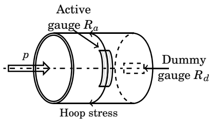
Figure 15.11: Pressure tube with bonded strain gauge in Example 15.1
