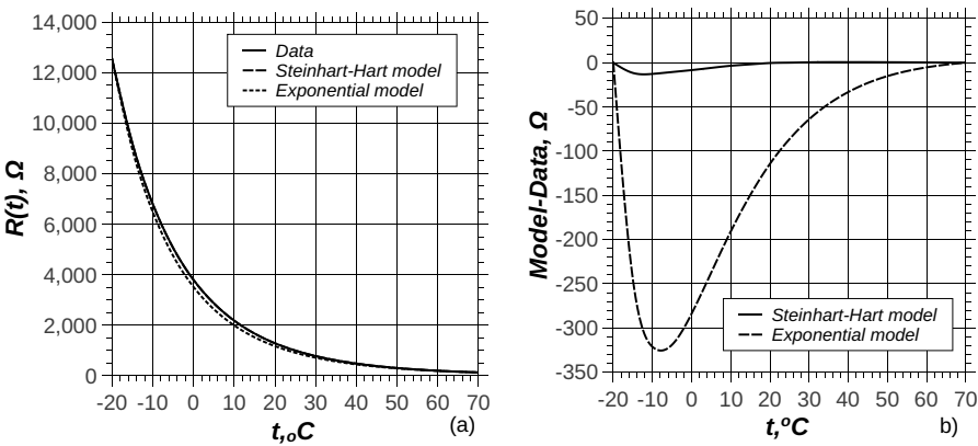
Figure 4.37: (a) Variation of resistance vs. temperature for the thermistor of Example 4.9. (b) Errors due to Steinhart-Hart and exponential models
