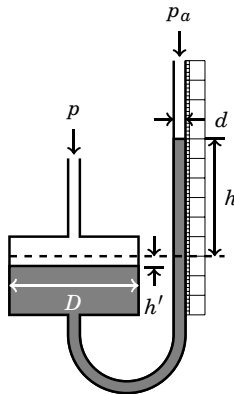
Figure 7.2: Schematic of a well type manometer
