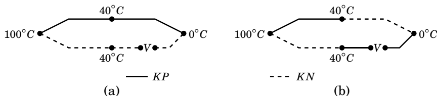
Figure 4.27: Thermocouple circuits for Example 4.5
