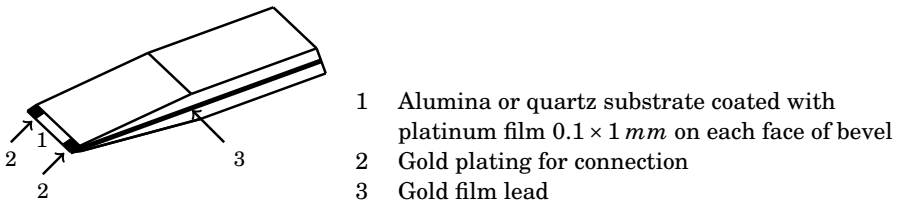
Figure 8.21: Hot film wedge probe
