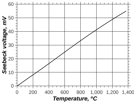
Figure 4.17: Seebeck volts - temperature relationship for K type thermocouple
