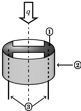
Figure 6.15: Construction detail of a thin film gauge
