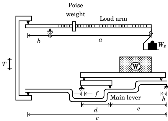
Figure 14.1: Sectional skeletal view of a platform balance
