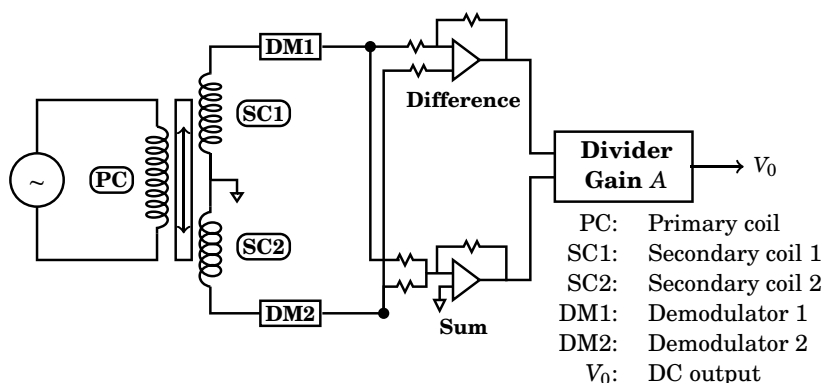
Figure 7.21: Typical LVDT signal conditioner circuit
