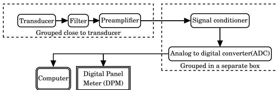
Figure 15.20: Schematic of a general instrument
