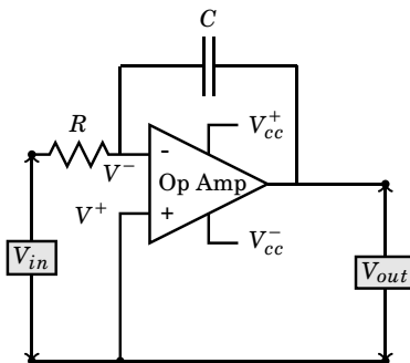
Figure 15.6: Integrating amplifier
