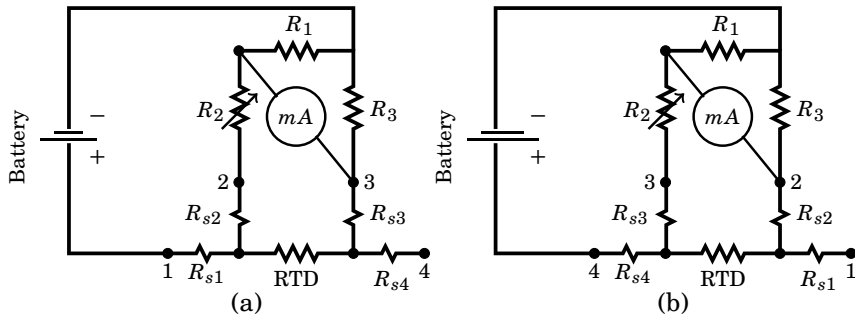
Figure 4.32: Bridge circuit with lead wire compensation (four wire arrangement). R_{s1} - R_{s4} are the lead wire resistances.
