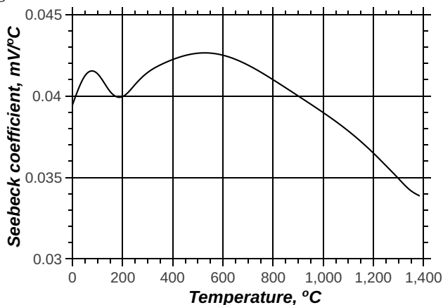
Figure 4.8: Variation of Seebeck coefficient with temperature for Chromel-Alumel thermocouple pair
