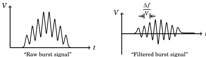
Figure 8.31: Scattered "burst" signal before and after filtering
