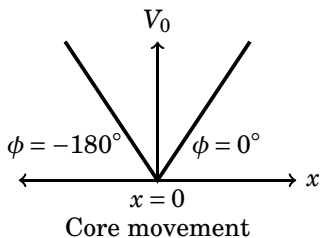
Figure 7.20: Output of an LVDT excited by alternating current supply. The phase ( \phi ) is with respect to the phase of the supply.
