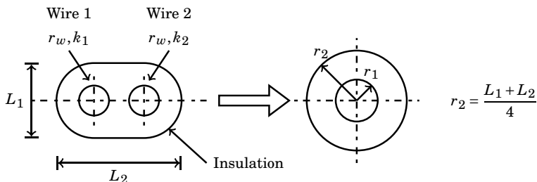
Figure 5.6: Single wire equivalent of a thermocouple
