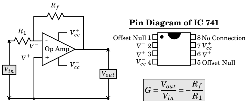
Figure 15.3: Basic operational amplifier circuit showing pin diagram for a DIP package. Also shown is the formula for Gain.
