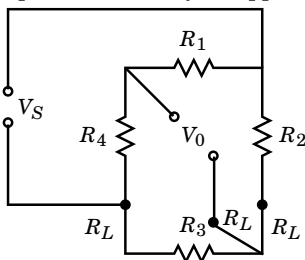
Figure 7.14: Three wire arrangement for lead wire compensation
