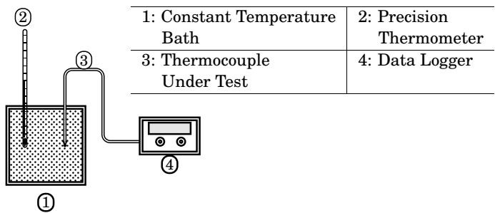
Figure 16.1: Thermocouple calibration arrangements using a data logger
