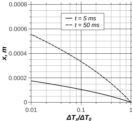
Figure 6.14: Thickness of substrate of a thin film gauge with quartz substrate. Incident flux is q = 10^5 \text{ W/m}^2 .
