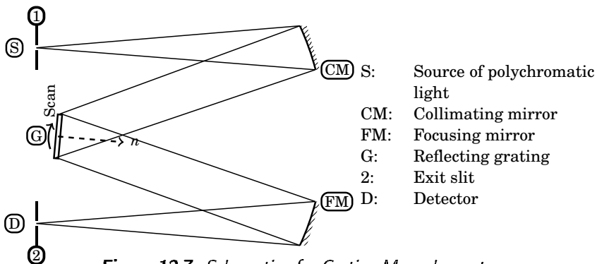
Figure 12.7: Schematic of a Grating Monochromator
