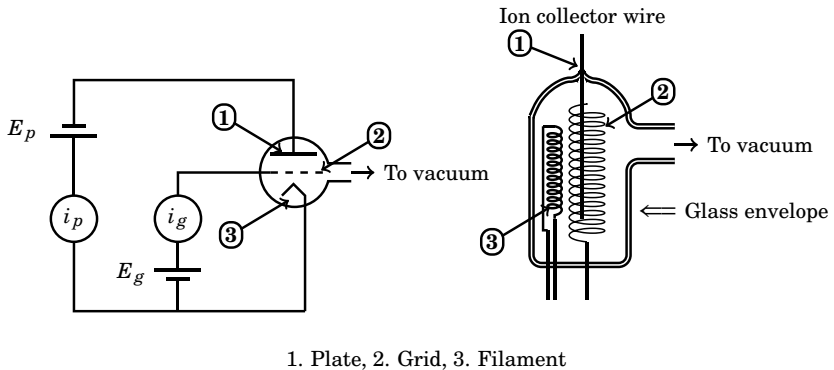
Figure 7.30: Ionization gauge - (a) circuitry and (b) schematic
