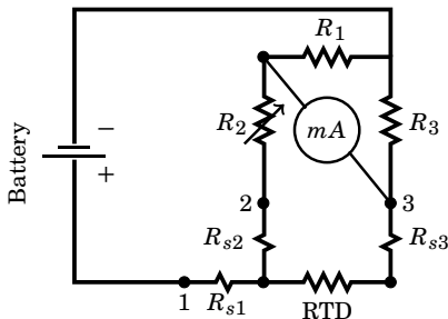
Figure 4.31: Bridge circuit with lead wire compensation (three wire arrangement). R_{s1} - R_{s3} are lead wire resistances.
