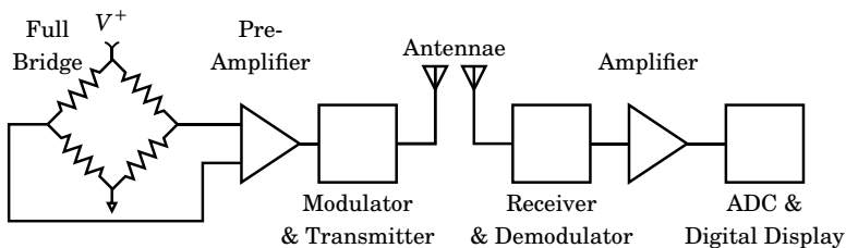
Figure 16.7: Schematic of circuit for torque measurement
