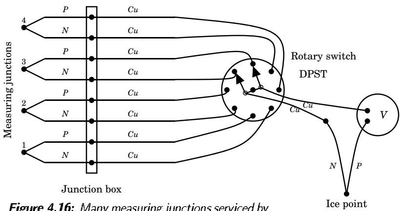
Figure 4.16: Many measuring junctions serviced by a single reference junction (DPST is a double pole single throw switch)
