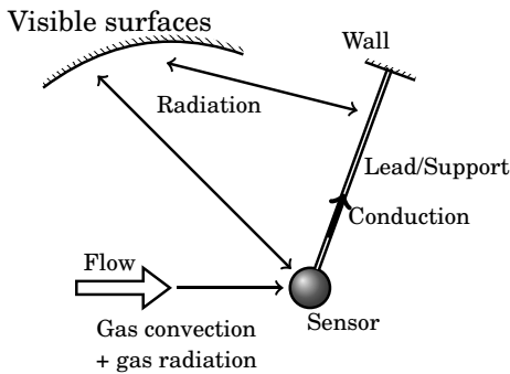
Figure 5.5: Heat transfer paths for a sensor in gas flow
