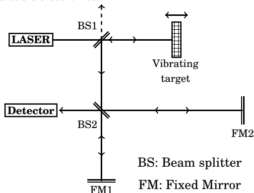
Figure 14.15: Schematic to explain the working principle of a Laser Doppler Vibrometer
