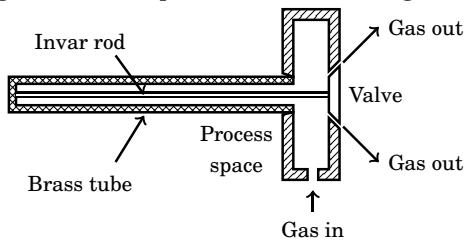
Figure 4.57: Thermostat for maintaining constant temperature in a process space
