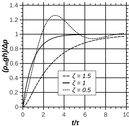
Figure 7.5: Response of U - tube manometer to step input
