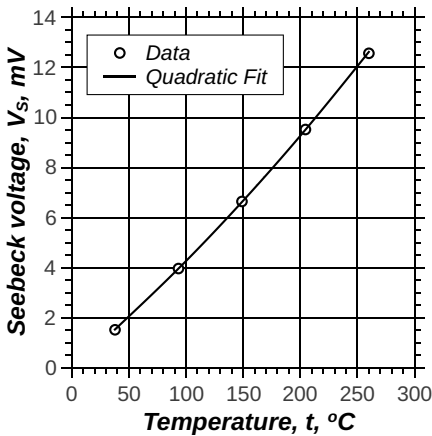
Figure 4.7: Comparison between data and the fit for a Copper Constantan thermocouple pair
