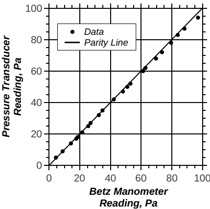
Figure 16.5: Parity plot comparing the DP gauge reading with Betz manometer reading
