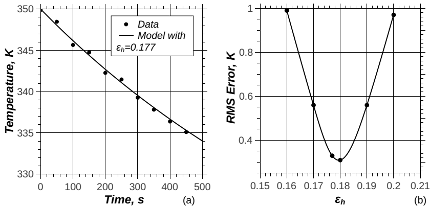
Figure 12.14: (a) Comparison of data with fit in Example 12.2 (b) Variation of rms error with chosen value of \epsilon_h
