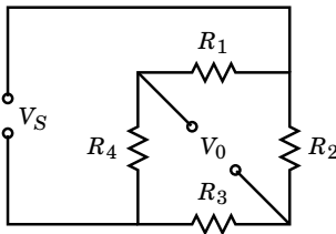
Figure 7.12: Basic DC bridge circuit for strain measurement. V_S = Battery voltage V_0 = Gauge output
