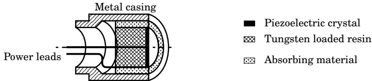
Figure 8.27: Sectional view of a piezoelectric transducer
