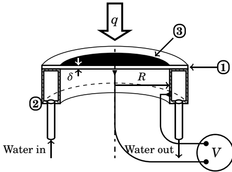
Figure 6.1: Schematic of a Gardon or foil type heat flux gauge
