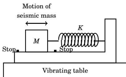
Figure 14.7: Accelerometer scheme specified in Example 14.3
