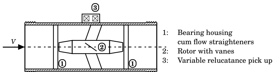
Figure 9.18: Schematic of a Turbine flow meter
