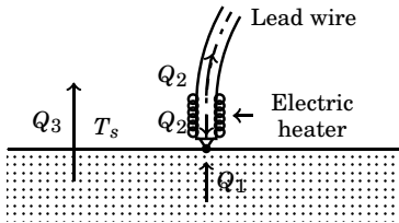
Figure 5.2: Schematic of a compensated probe
