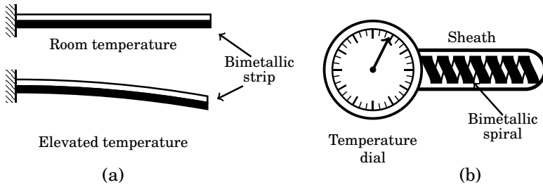
Figure 4.54: Schematics of Bimetallic strip thermometers (a) Cantilever type (b) Spiral type
