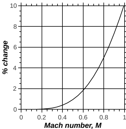
Figure 8.6: Percent difference in Pressure ratio with compressible and incompressible assumptions recorded by a Prandtl tube as a function of flow Mach number
