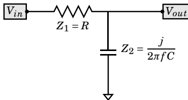
Figure 15.14: Low pass filter
