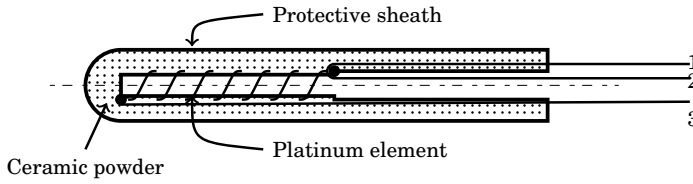
Figure 4.29: Schematic of a typical PRT sensor with three wire arrangement
