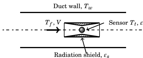
Figure 5.12: Use of radiation shield in fluid temperature measurement
