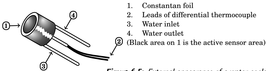
Figure 6.5: External appearance of a water cooled Gardon gauge
