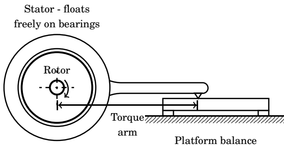
Figure 14.19: Electric generator used as a dynamometer
