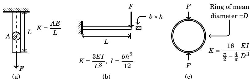
Figure 14.3: Several configurations for measuring force with the appropriate spring constants: (a) Rod in tension or compression (b) Cantilever beam (c) Thin ring
