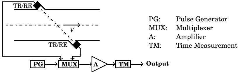
Figure 8.35: Wetted type ultrasonic mean velocity meter
