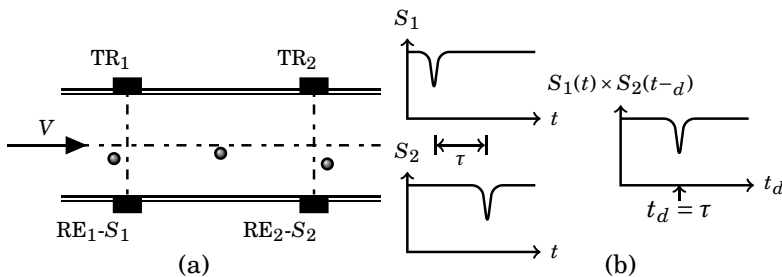
Figure 8.38: (a) Cross correlation type velocity meter (b) Cross correlation time measurement
