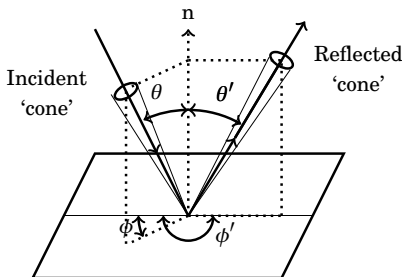
Figure 12.2: Bi-angular reflection at a surface
