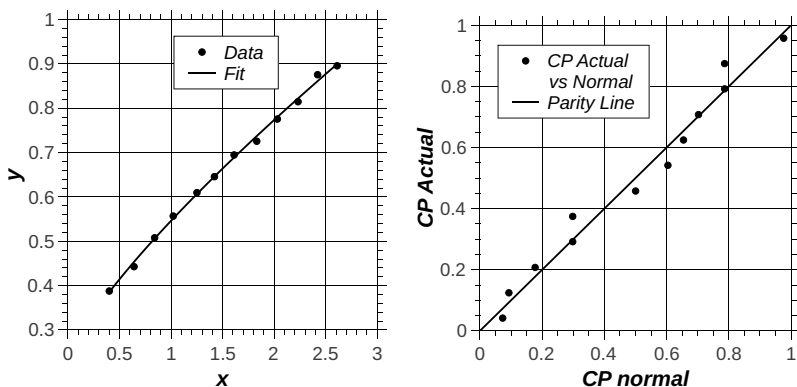
Figure 2.6: (a) Non-linear fit to data obtained using QtiPlot (b) Test for normality of deviates in Example 2.4
