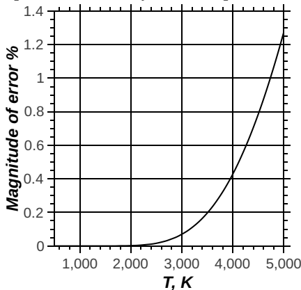
Figure 4.41: Error in using Wein's approximation instead of the Planck function
