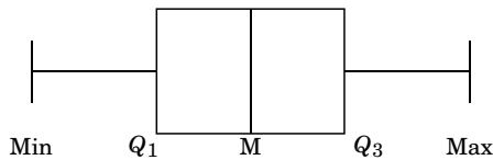
Figure 1.8: Box and whisker plot: M - Median, Q_1 - Lower quartile, Q_3 - Upper quartile, Min - Lower extreme, Max - Upper extreme
