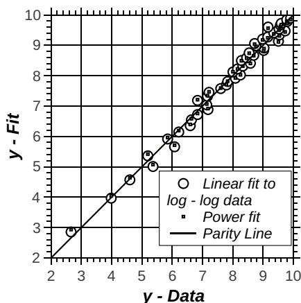
Figure 2.10: Parity plot comparing two ways of obtaining the fit
