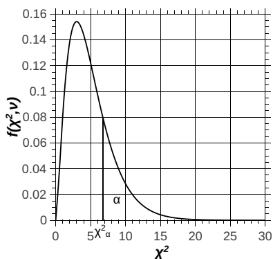
Figure 2.8: \alpha as fraction of area under the \chi^2 distribution
