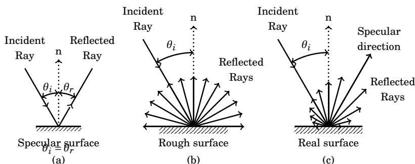
Figure 12.1: Schematic representation of reflection at an opaque surface: (a) Specular surface (b) Diffuse surface (c) Real surface
