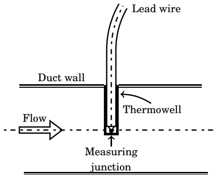
Figure 5.4: Measurement of temperature of a moving fluid
