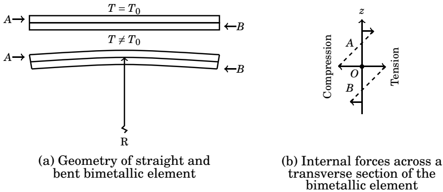
Figure 4.55: Bimetallic element analysis
