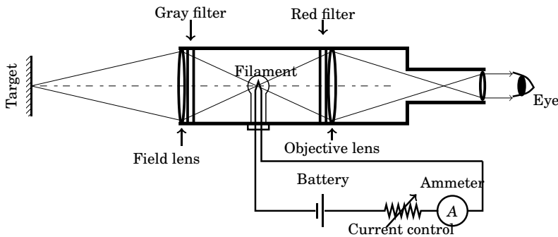
Figure 4.46: Schematic of a vanishing filament pyrometer
