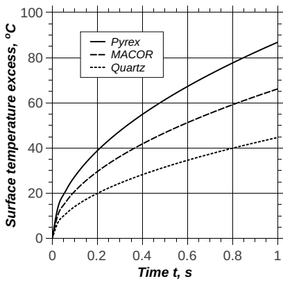
Figure 6.13: Surface temperature response with three different substrates given in Table 6.2. Incident flux is q = 10^5 \text{ W/m}^2 .
