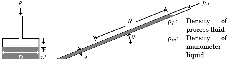
Figure 7.3: Well type inclined tube manometer
