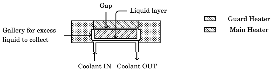
Figure 11.3: Guarded hot plate apparatus for the measurement of thermal conductivity of liquids
