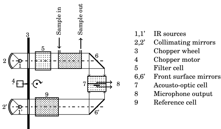
Figure 13.3: Details of a typical NDIR system
