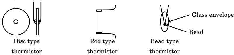
Figure 4.35: Typical thermistor types
