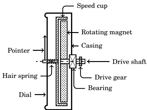
Figure 14.22: Sectional view of a speedometer or a tachometer
