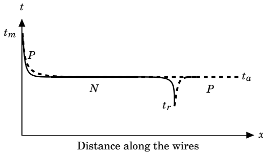
Figure 4.10: Temperature variations along the wires
