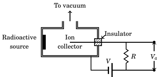
Figure 7.31: Schematic of an Alphanatron gauge
