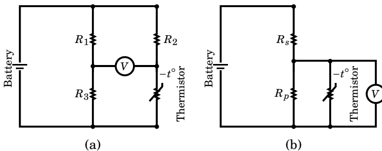
Figure 4.38: (a) Thermistor bridge circuit (b) Alternate measuring circuit, essentially a voltage divider
