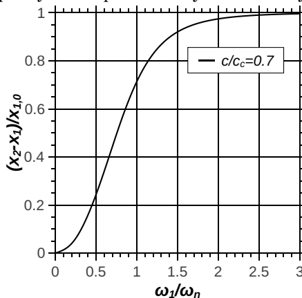
Figure 14.11: Amplitude response of a system with damping ratio of 0.7
