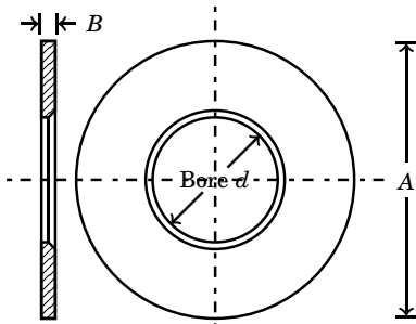
Figure 9.7: Orifice plate specifications
