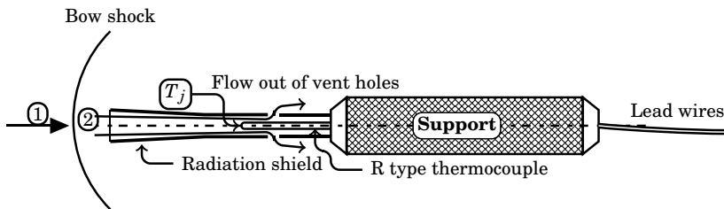
Figure 10.1: Shielded thermocouple stagnation temperature probe in a supersonic stream (Based on NASA Technical Memorandum 4407, March 1993)
