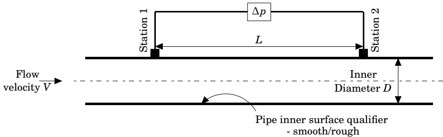
Figure 3.3: Schematic of an experimental set up for friction factor measurement in pipe flow
