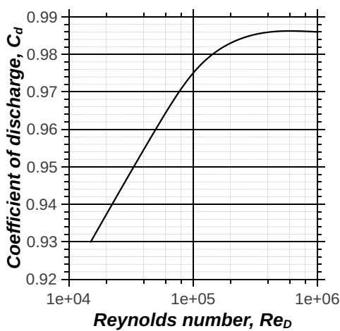
Figure 9.12: Variation of coefficient discharge of a venturi with pipe Reynolds number
