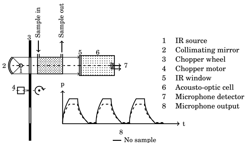
Figure 13.2: Sketch for explaining the principle of NDIR
