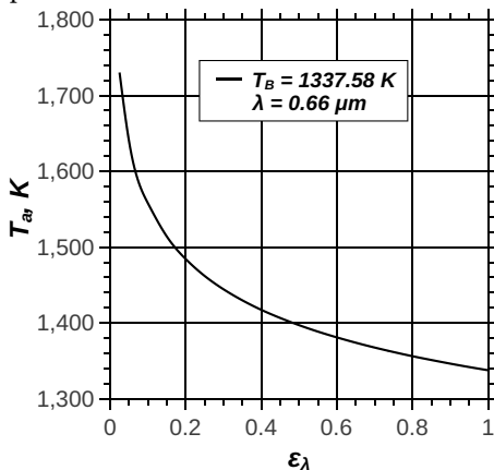
Figure 4.45: Temperature a surface whose brightness temperature equals gold point temperature of 1337.58 K ( \lambda = 0.66 \mu\text{m} )
