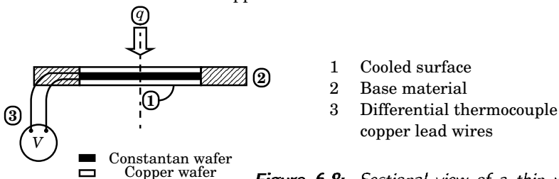
Figure 6.8: Sectional view of a thin wafer type cooled heat flux gauge
