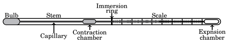
Figure 4.51: Construction details of a typical liquid in glass thermometer
