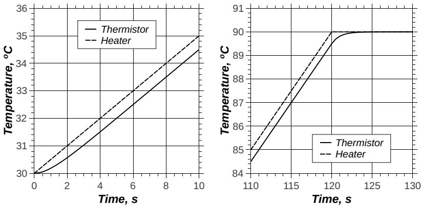
Figure 4.64: Thermistor response to heater input in Example 4.22
