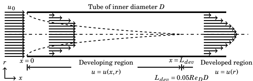
Figure 11.18: Laminar flow in a circular tube
