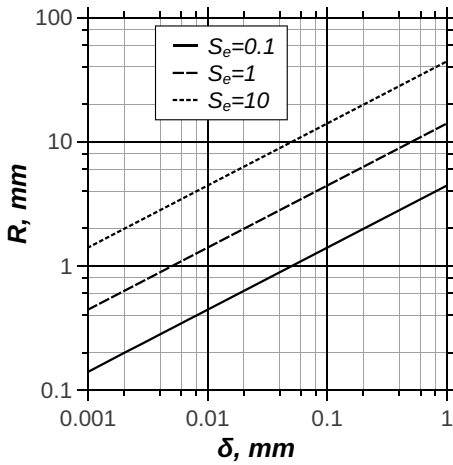
Figure 6.3: Proportions of foil gauge for desired sensitivity values
