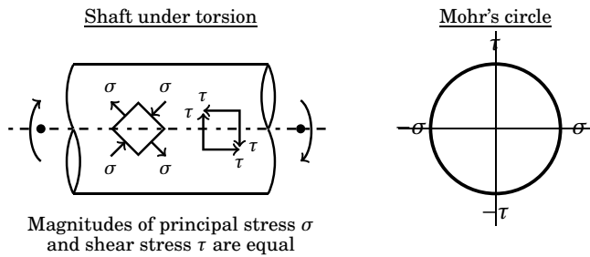
Figure 14.20: Stresses on the surface of a shaft in torsion
