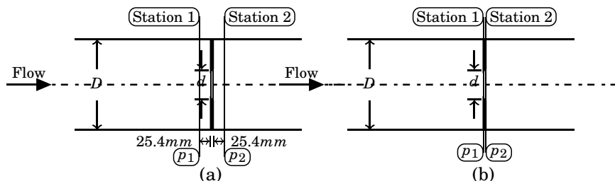
Figure 9.5: Schematic of a sharp edged orifice with (a) flange taps, (b) Corner taps.
