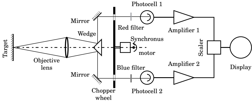
Figure 4.49: Schematic of a two color pyrometer
