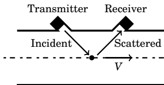
Figure 8.28: Measurement of fluid velocity by Doppler shift method
