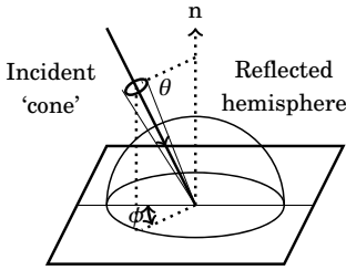
Figure 12.3: Directional hemispherical reflectivity
