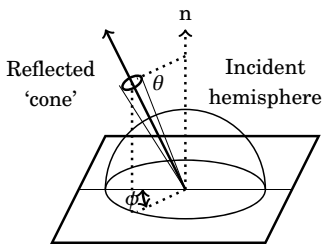
Figure 12.4: Hemispherical directional reflectivity
