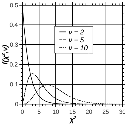
Figure 2.7: \chi^2 distribution
