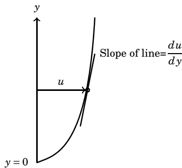
Figure 11.17: Newton law of viscosity explained
