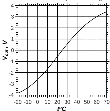
Figure 4.39: Voltmeter reading variation with thermistor temperature
