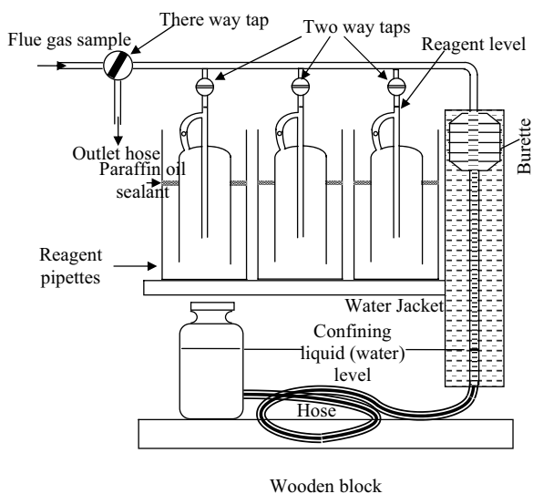
Figure 13.11: Schematic of an Orsat analyzer
