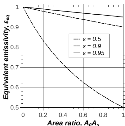
Figure 4.44: Variation of effective emissivity of a cavity radiator with area ratio
