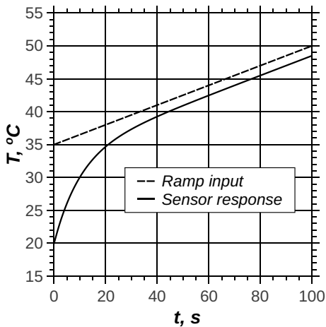
Figure 4.63: Typical response of a first order system to ramp input
