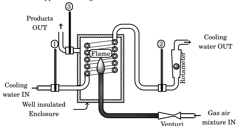
Figure 11.16: Schematic of a continuous flow calorimeter. 1 - 3 are precision thermometers
