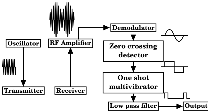
Figure 8.29: Measurement of fluid velocity by Doppler shift method
