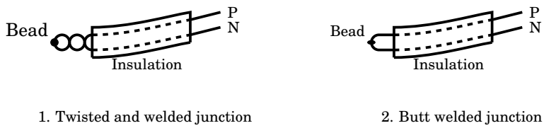
Figure 4.21: More junction types
