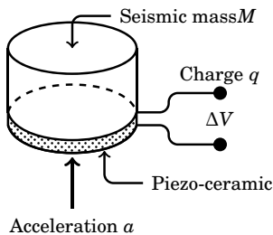
Figure 14.14: Piezoelectric accelerometer
