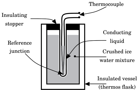
Figure 4.15: Ice point reference junction
