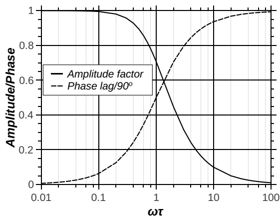
Figure 4.66: Amplitude and phase of a first order system subject to periodic input
