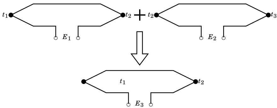
Figure 4.13: Illustration of the law of intermediate temperatures. Note that E_3 = E_1 + E_2 .
