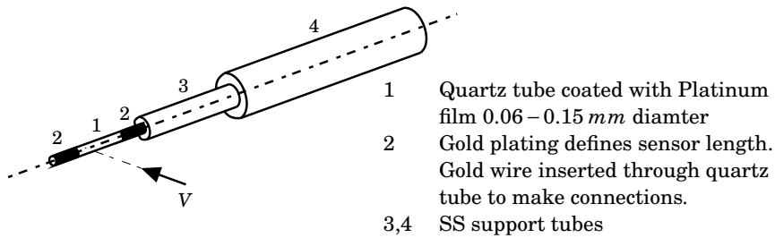
Figure 8.20: Cylindrical hot film probe
