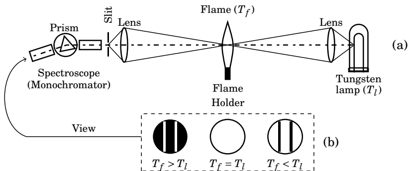
Figure 4.50: Schematic of set up for the 'line reversal' technique
