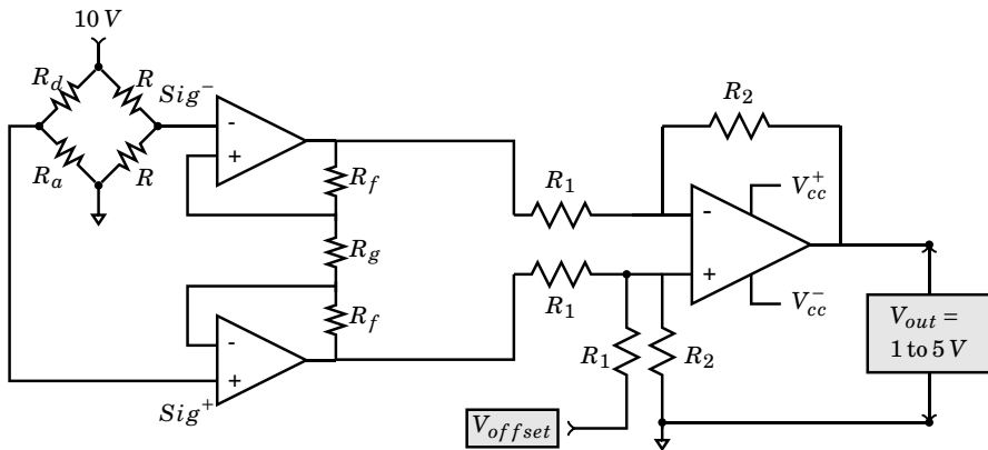
Figure 15.12: Signal conditioner for a full bridge
