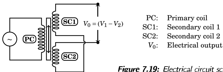
Figure 7.19: Electrical circuit schematic of the LVDT
