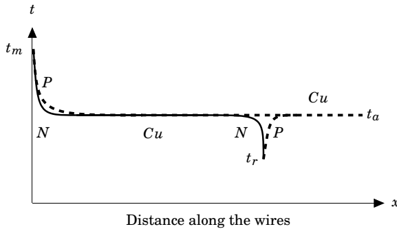
Figure 4.14: Temperature variations along the wires of a practical thermocouple circuit
