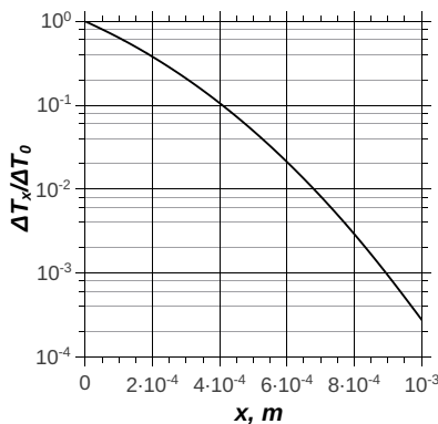
Figure 6.16: Temperature at various depths within the substrate at t = t_{max} = 74 \text{ ms}
