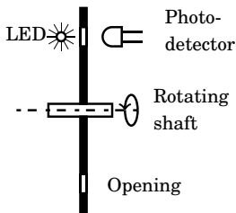
Figure 14.23: Optical RPM measurement
