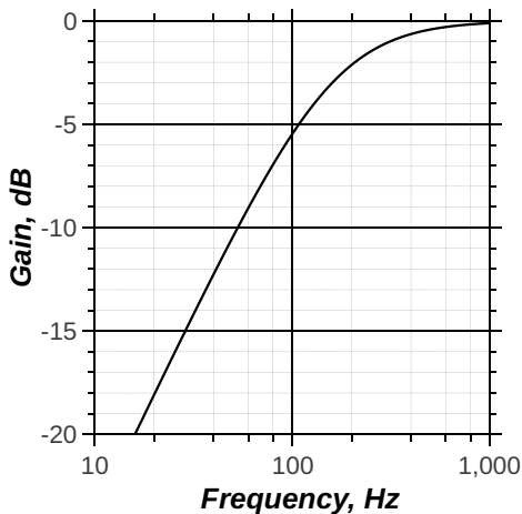
Figure 15.17: High pass filter frequency response
