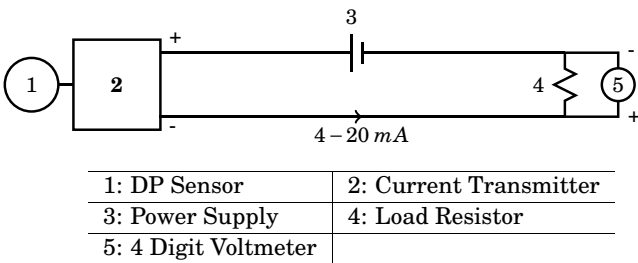
Figure 15.21: Differential Pressure (DP) sensor with 4 – 20 mA current loop
