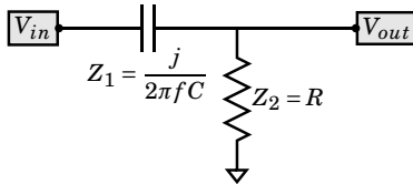
Figure 15.16: High pass filter
