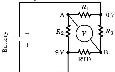
Figure 4.34: Bridge circuit for Example 4.7
