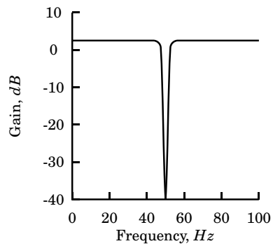
Figure 15.19: Frequency response of a notch filter designed to filter 50 Hz component
