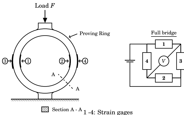
Figure 14.5: Schematic of a proving ring
