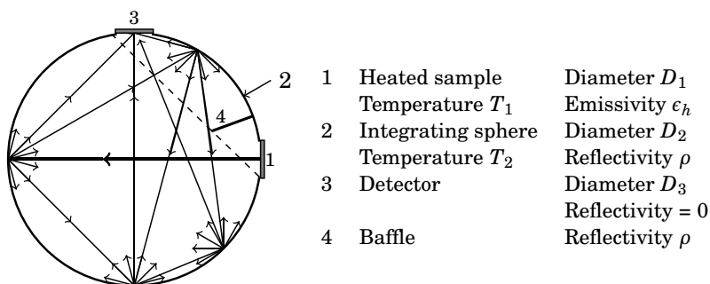
Figure 12.9: Integrating sphere arranged for measurement of hemispherical emissivity
