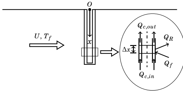
Figure 5.15: Sketch explaining thermometer well analysis
