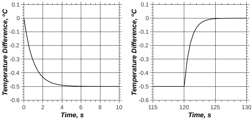
Figure 4.65: Temperature difference between thermistor and heater vs time in Example 4.22
