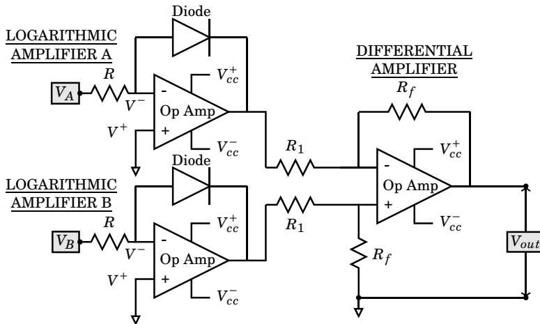
Figure 15.9: Schematic of a circuit for taking the ratio of two signals
