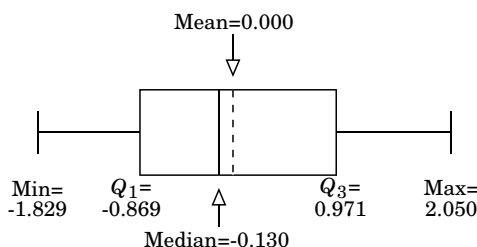
Figure 1.9: Box and whisker plot for Example 1.6
