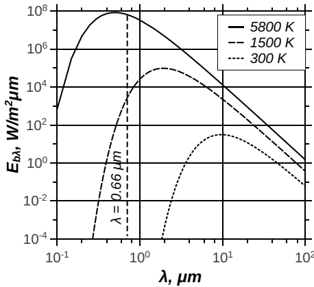
Figure 4.42: Black body characteristics and the Wein's displacement law (wavelength of 0.66 \mu m is normally used in optical Pyrometry)
