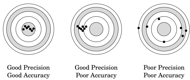
Figure 1.3: Precision and accuracy explained through a familiar example
