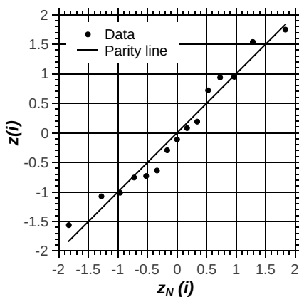
Figure 1.11: Q-Q plot for sample data in Example 1.8
