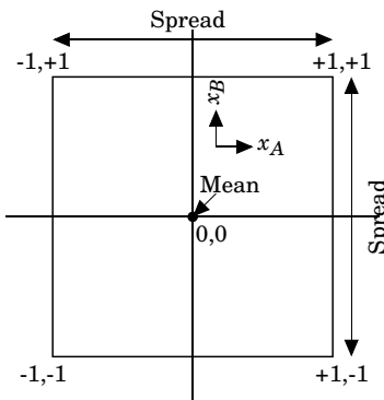
Figure 3.1: Interpretation of 2^2 factorial experiment
