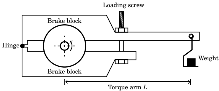
Figure 14.18: Schematic of a Prony brake
