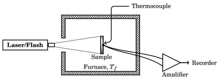
Figure 11.7: Schematic of the laser flash apparatus
