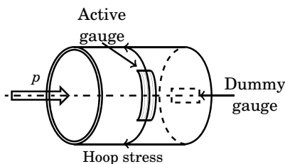
Figure 7.9: Pressure tube with bonded strain gauge
