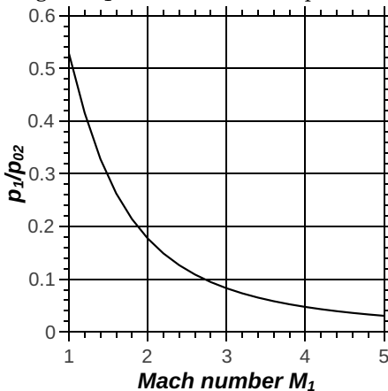
Figure 8.8: Pressure ratio Mach number relation for supersonic flow
