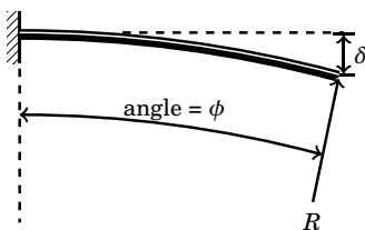
Figure 4.56: Bimetallic element geometry in Example 4.18
