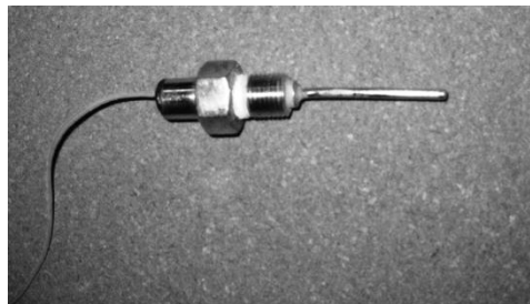
Figure 5.13: External appearance of a thermometer well probe using a thermocouple
