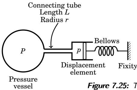
Figure 7.25: Transient in a bellows type gauge
