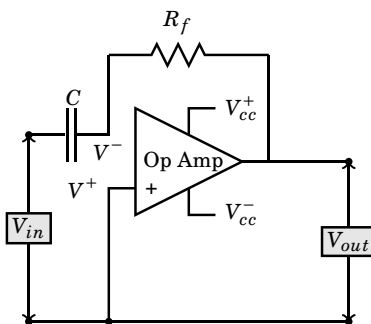
Figure 15.7: Differentiating amplifier
