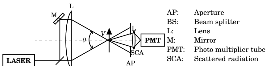
Figure 8.30: Schematic of the fringe system
