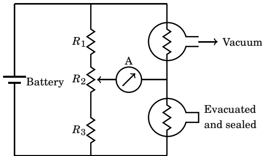
Figure 7.29: Pirani gauge with temperature compensation
