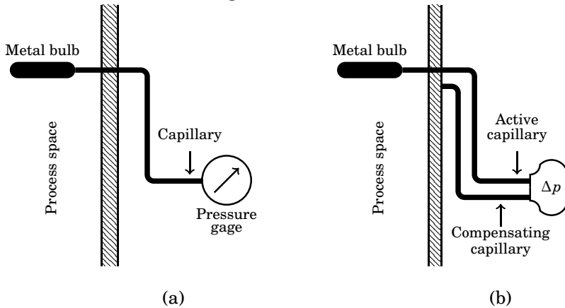
Figure 4.53: Construction details of liquid in metal thermometers
