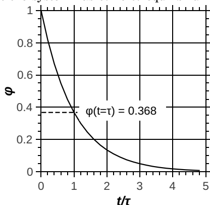
Figure 4.61: Response of a first order system to a step change in temperature
