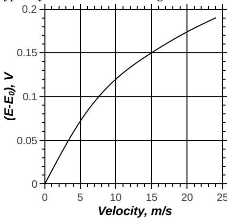
Figure 8.19: Output of a typical micro machined hot wire probe in the CC mode. Length of wire L = 100 \mu\text{m} , Resistance at room temperature = 2000 \Omega .
