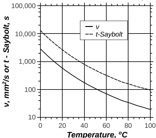
Figure 11.21: Time to drain in standard Saybolt test of 10W50 engine oil as a function of temperature
