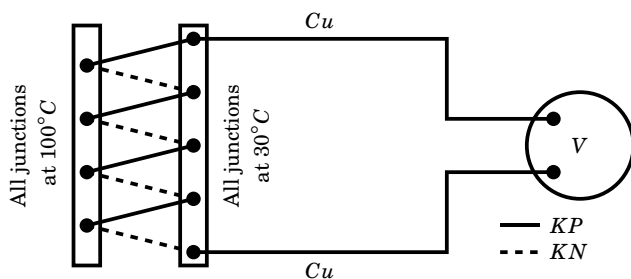
Figure 4.26: Thermopile circuit for Example 4.4
