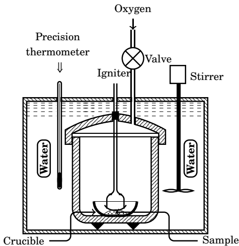
Figure 11.13: Schematic of a Bomb calorimeter
