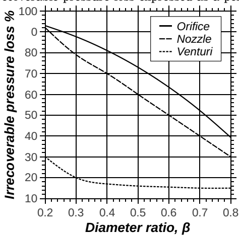
Figure 9.13: Irrecoverable pressure loss comparisons
