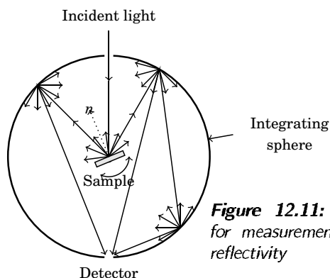
Figure 12.10: Integrating sphere arranged for measurement of hemispherical directional reflectivity
