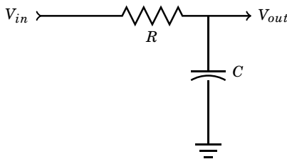
Figure 4.60: Electrical analog of a first order thermal system
