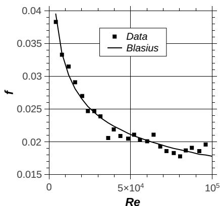
Figure 3.5: Experimental verification of the Blasius friction factor formula for flow through a smooth tube
