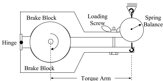
Figure 14.25: Prony brake arrangement for Example 14.7
