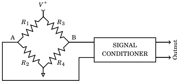
Figure 16.6: Strain gauges in full bridge configuration
