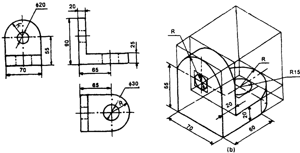
Fig. 9.34 Angle Plate
