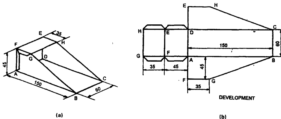
Fig. 7.15 Rectangular Scoop
