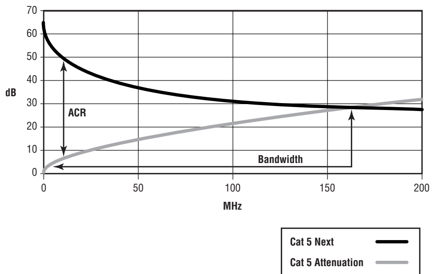
FIGURE 1.19: Attenuation-to-crosstalk ratio for a Category 5 chan- nel link
