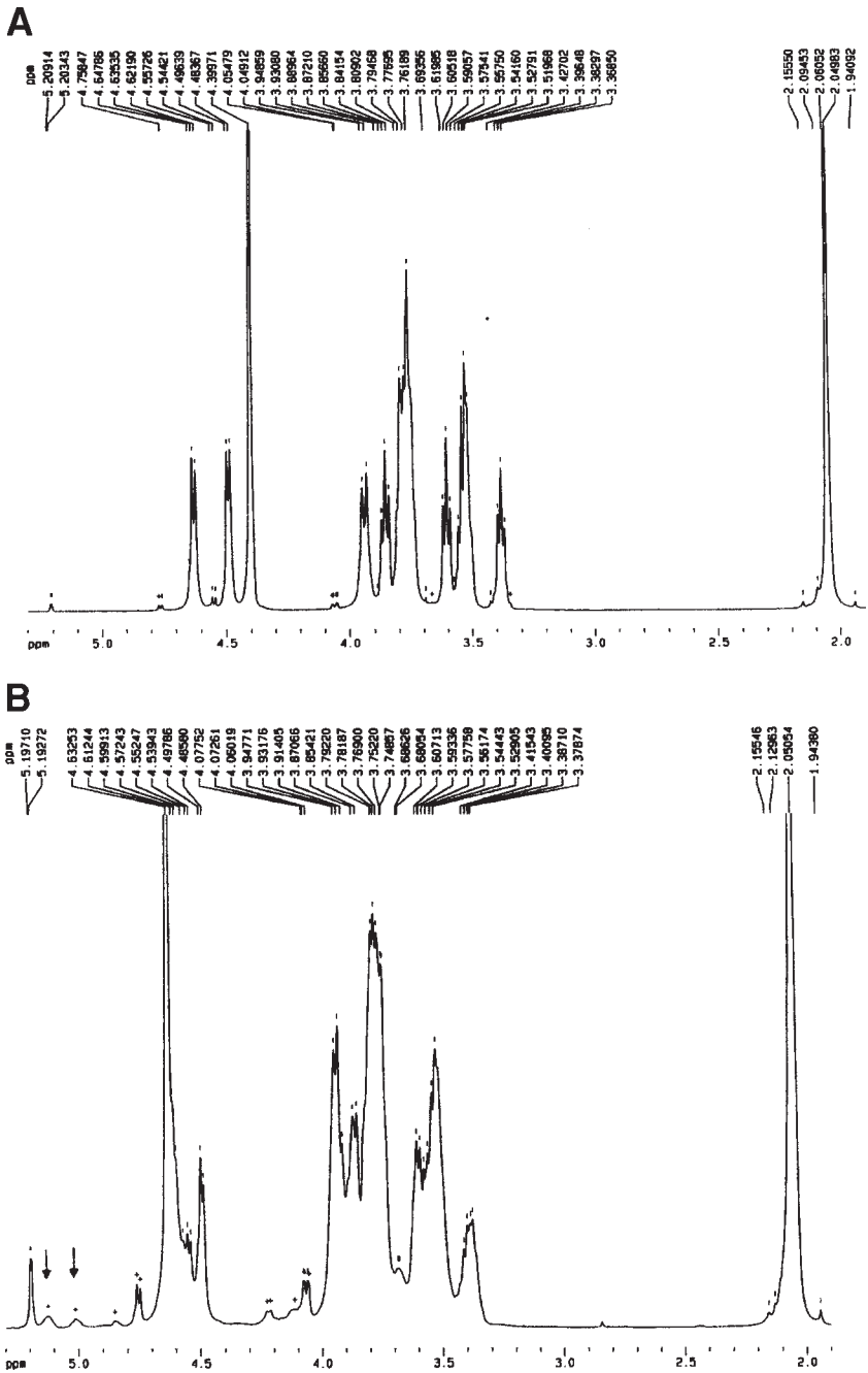
Figure 5. (A) ^3\text{H} -NMR spectrum of HA-sodium salt. (B) ^3\text{H} -NMR spectrum of ACP ^{\text{®}} . Arrows point to the 5.12- and 5.01-ppm peaks.
