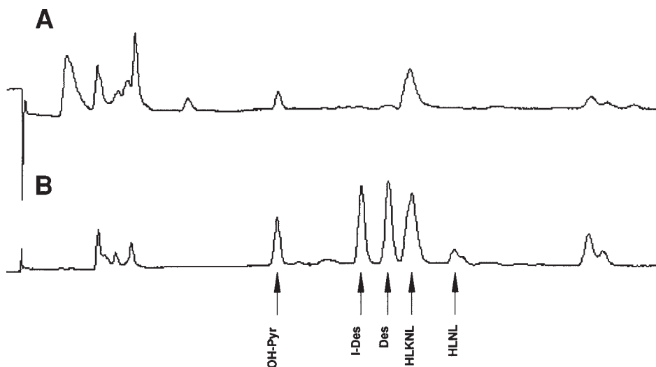
Fig. 1. (A) Typical crosslink profile of tissue-engineered cartilage from an amino acid analyzer using the method described here. The two crosslink peaks hydroxylysylpyridinoline (OH-Pyr) and hydroxylysino-keto-norleucine (HLKNL) are indicated. (B) Profile of crosslink standards run using the same analysis program. Additional crosslink standards to those above are Isodesmosine (I-Des), Desmosine (Des), and hydroxylysino-norleucine (HLNL).
