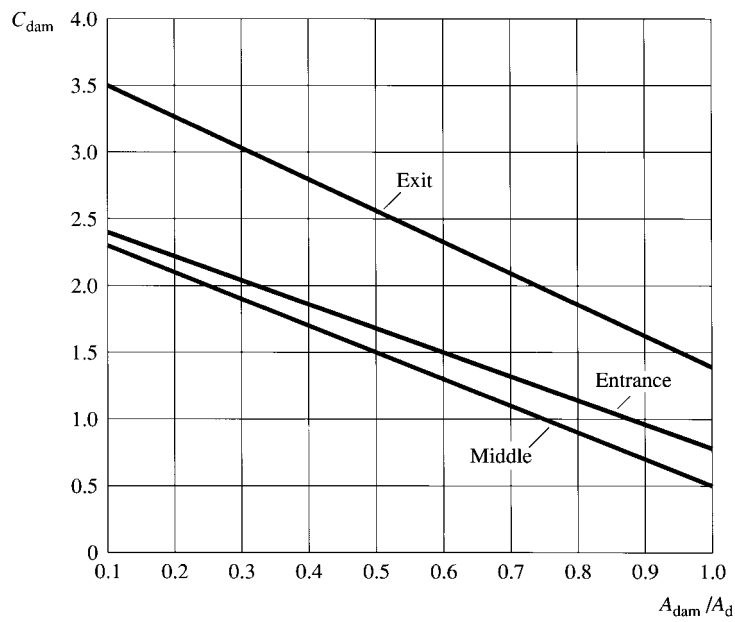
FIGURE 5.21 Local loss coefficient C_{dam} of air damper. (Source: ASHRAE Transactions 1988, Part I. Reprinted by permission.)
