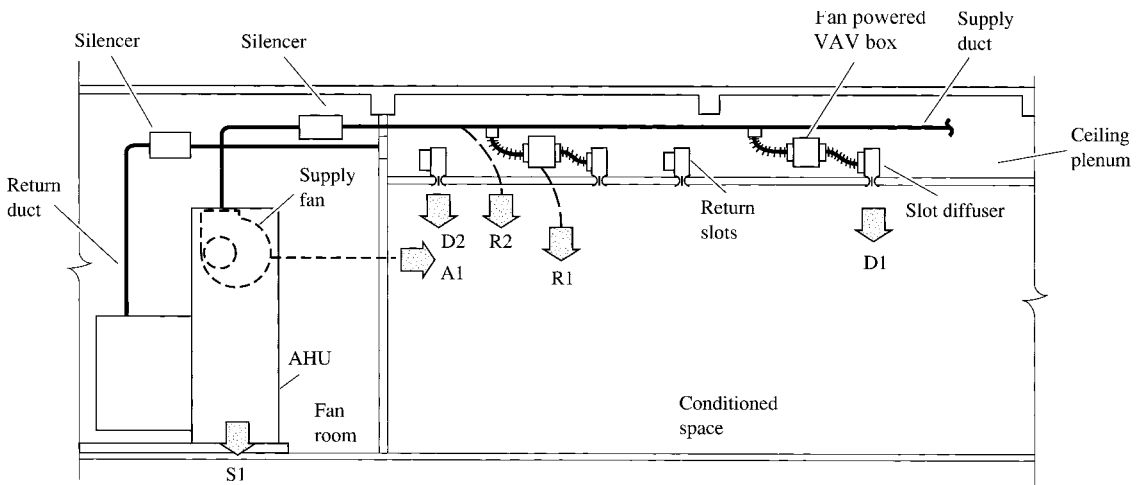
FIGURE 19.1 Fan room and sound paths.
