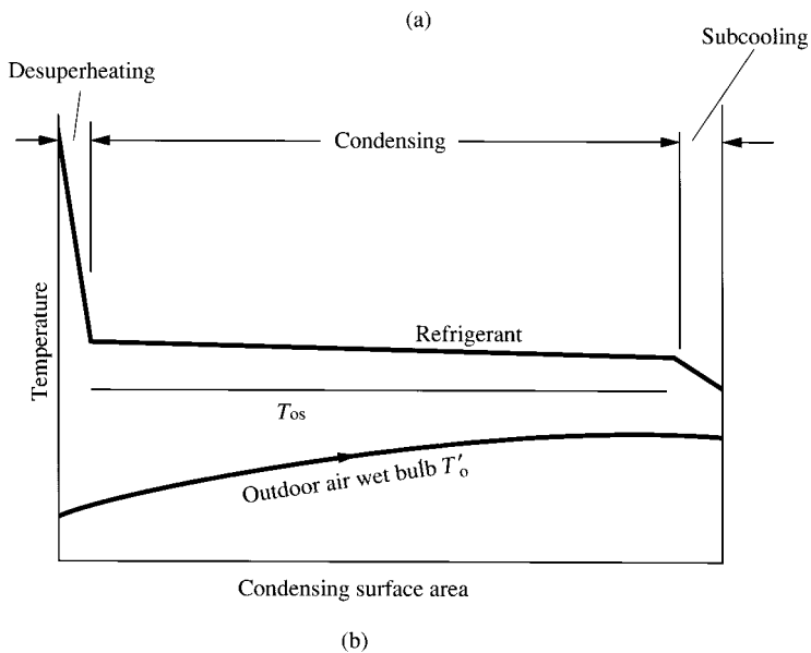
FIGURE 10.12 A typical evaporative condenser: (a) schematic diagram; (b) temperature curves.
