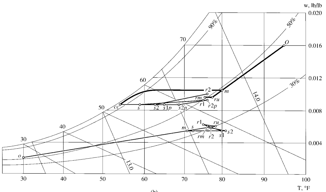
FIGURE 20.29 Constant-volume multizone system with reheat: (a) schematic diagram; (b) air conditioning cycle.
