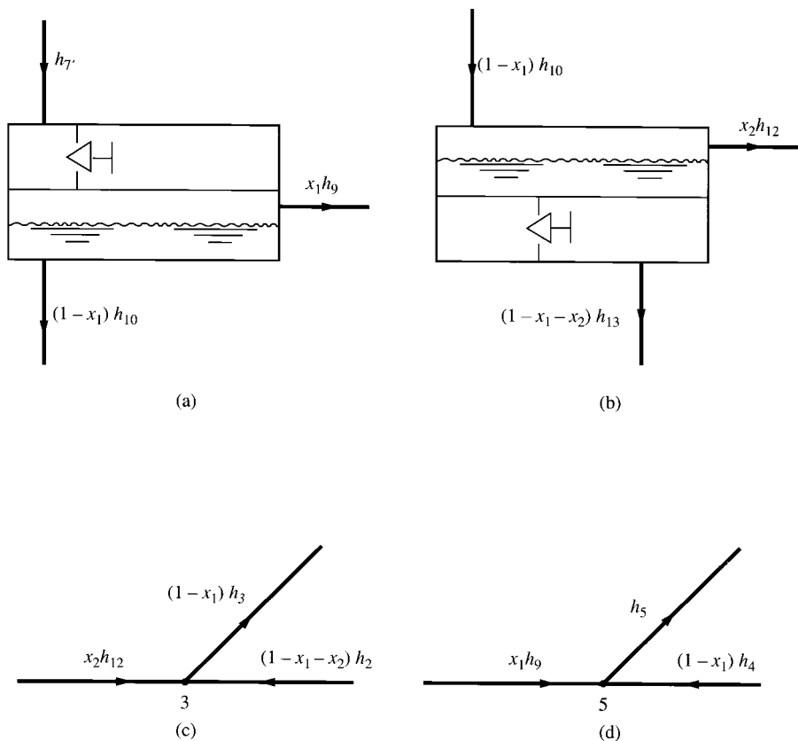
FIGURE 9.10 Heat balance of refrigerants entering and leaving the high-pressure and low-pressure flash cooler and mixing points. (a) High-pressure flash cooler; (b) low-pressure flash cooler; (c) at the mixing point before entering second-stage impeller; (d) at the mixing point before entering third-stage impeller.
