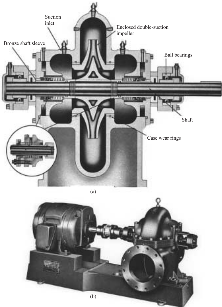
FIGURE 7.11 A double-suction, horizontal split-case, single-stage centrifugal pump. (a) Sectional view; (b) centrifugal pump and motor assembly.
