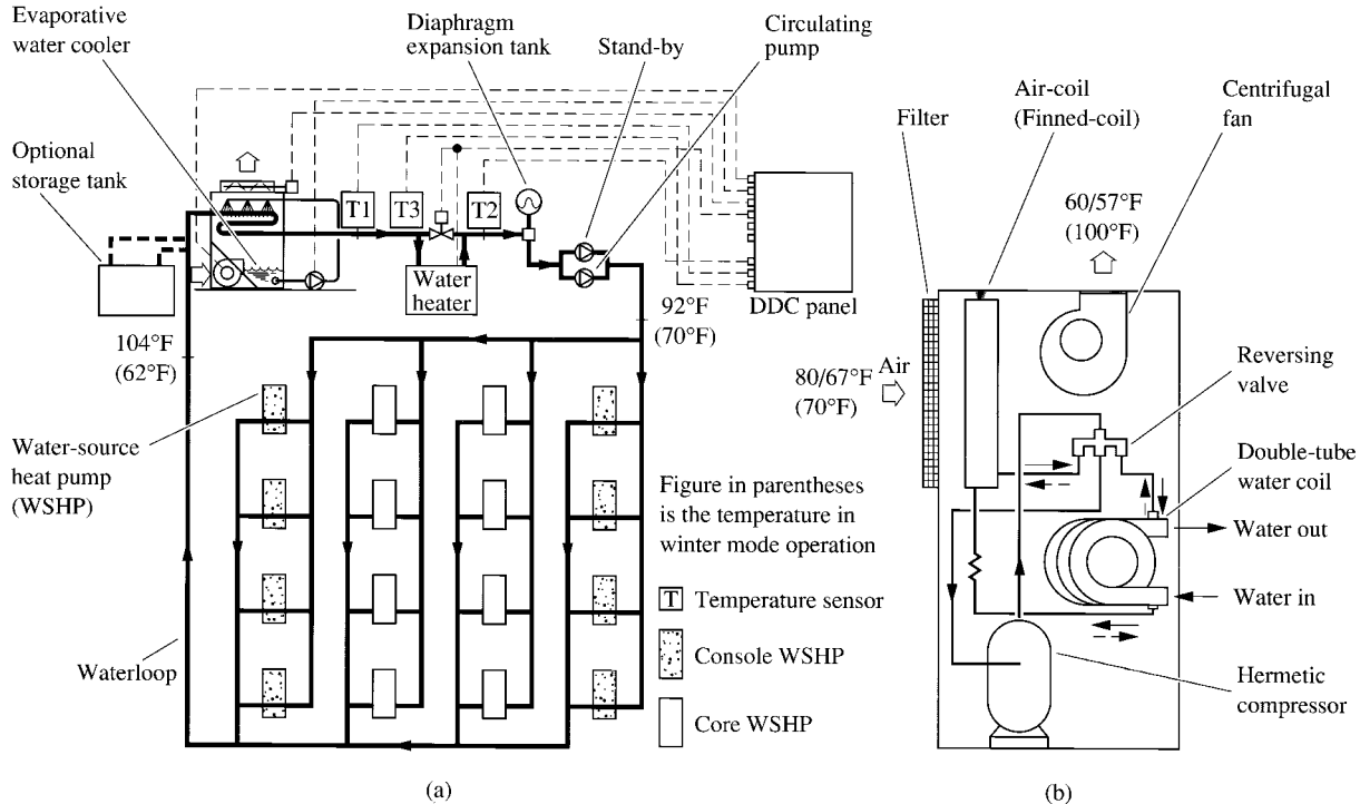
FIGURE 28.6 A typical closed-circuit water-source heat pump system: (a) schematic diagram; (b) water-source heat pump.
