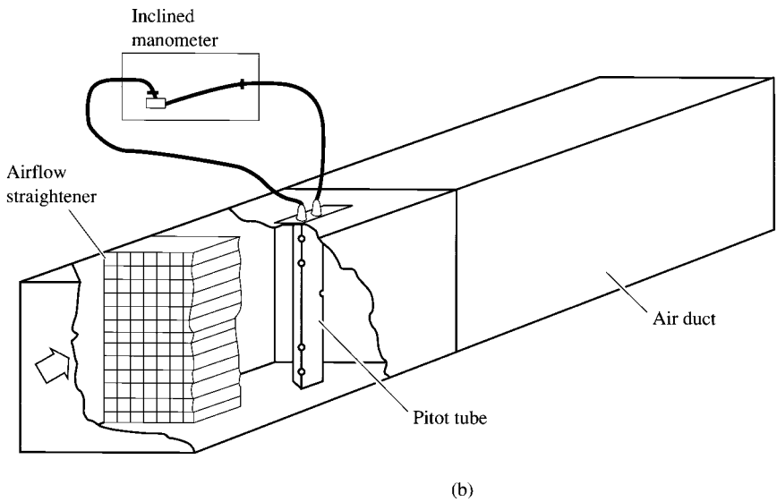
FIGURE 5.11 (a) A temperature sensor and (b) a typical pitot tube flow-measuring station.
