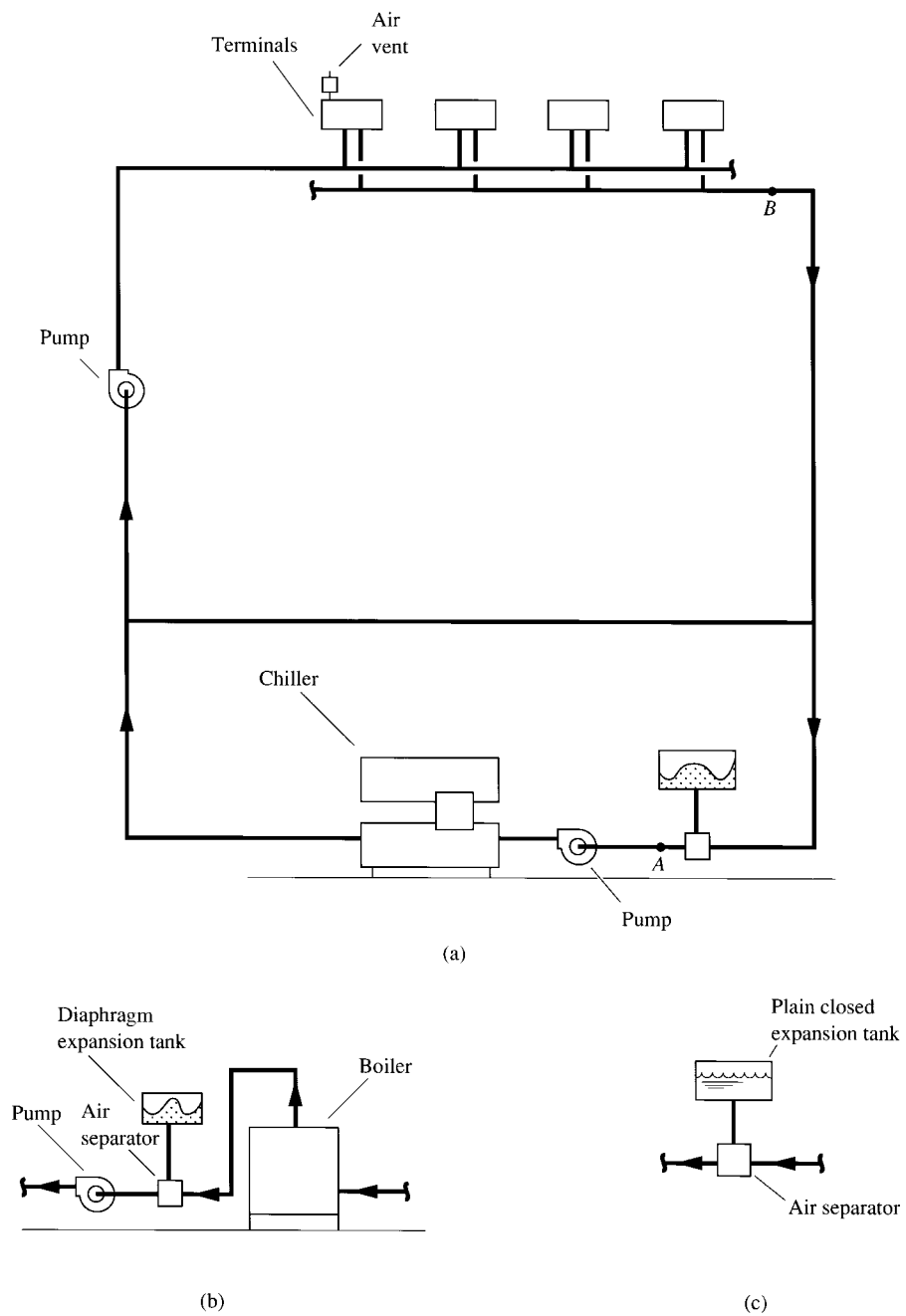
FIGURE 7.8 Closed expansion tank for a water system. (a) Diaphragm expansion tank in a chilled water system. (b) Diaphragm expansion tank in a hot water system. (c) Plain closed expansion tank.
