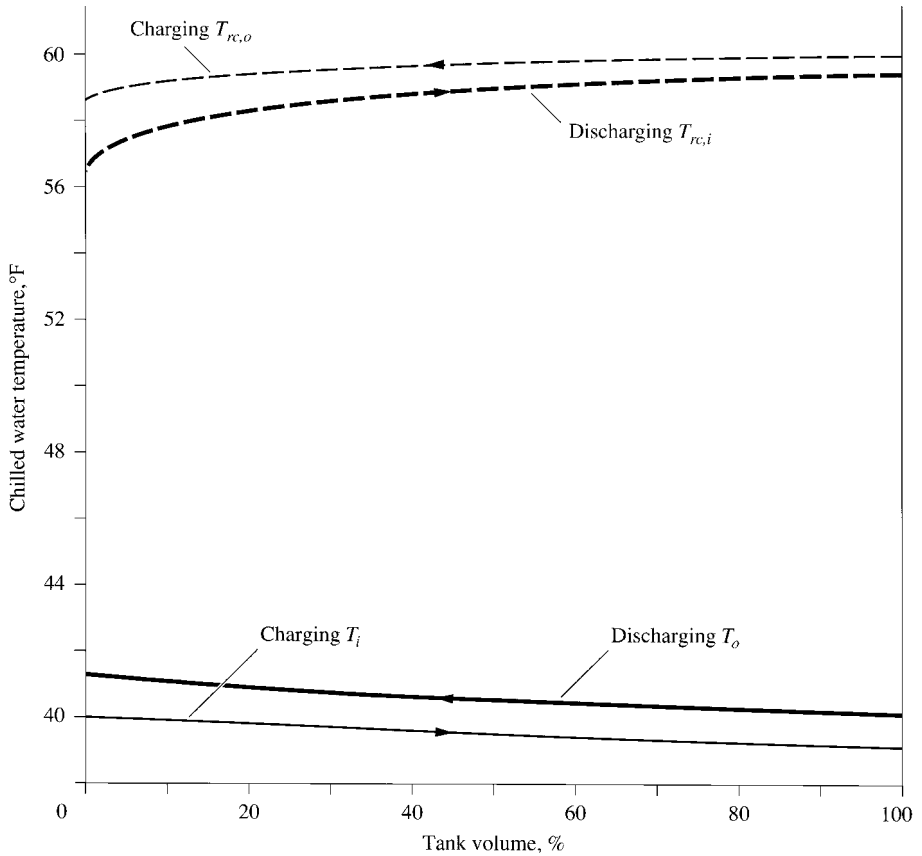
FIGURE 31.9 Chilled water temperature versus tank volume curves during charging and discharging processes.
