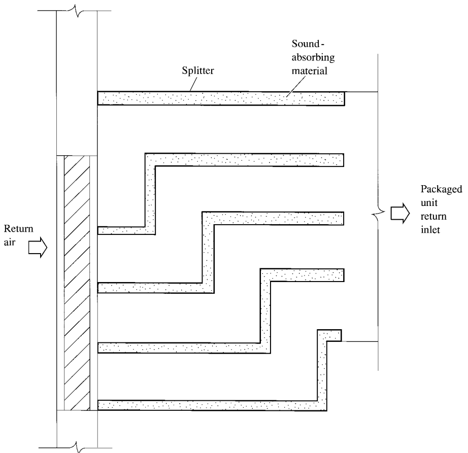
FIGURE 19.3 Sound-attenuating plenum.
