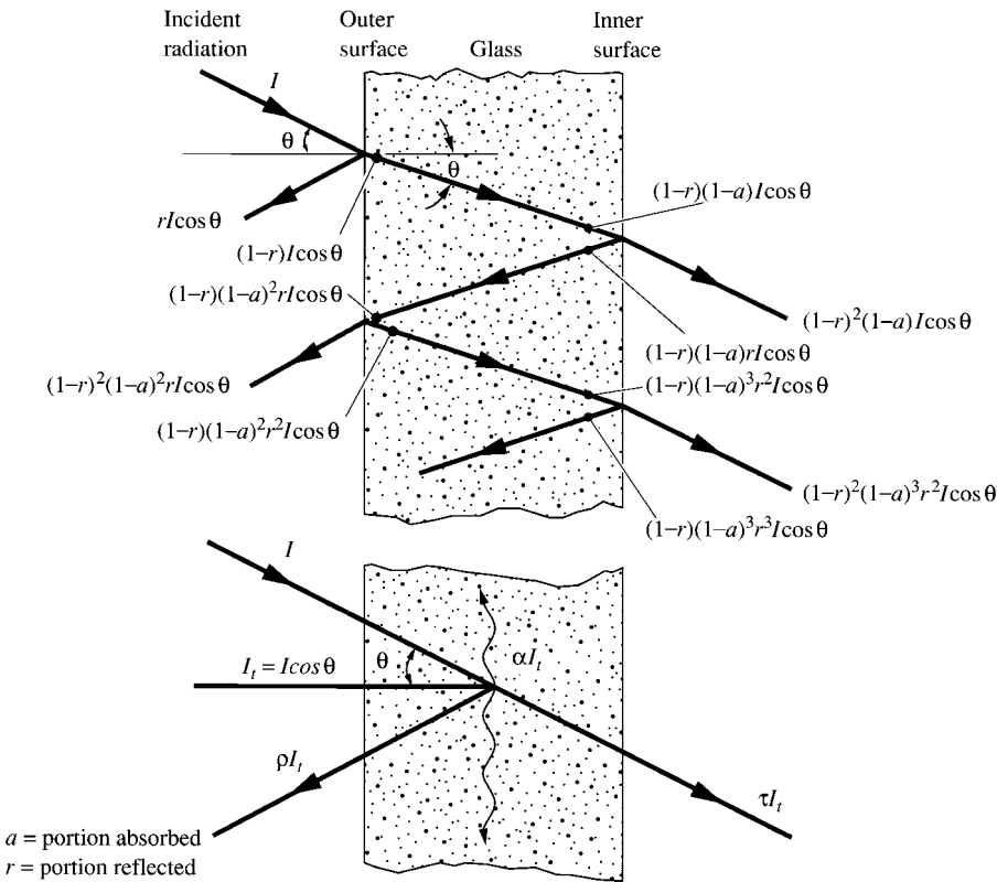
FIGURE 3.9 Simplified representation of multiple transmissions, reflections, and absorptions of solar radiation at glass surfaces.
