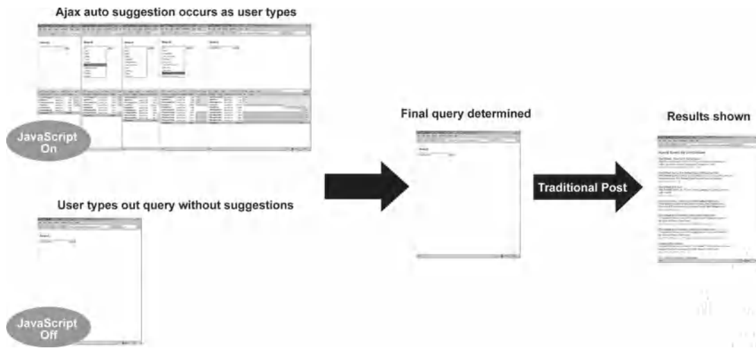
FIGURE 9-1 Suggest and search with and without Ajax
