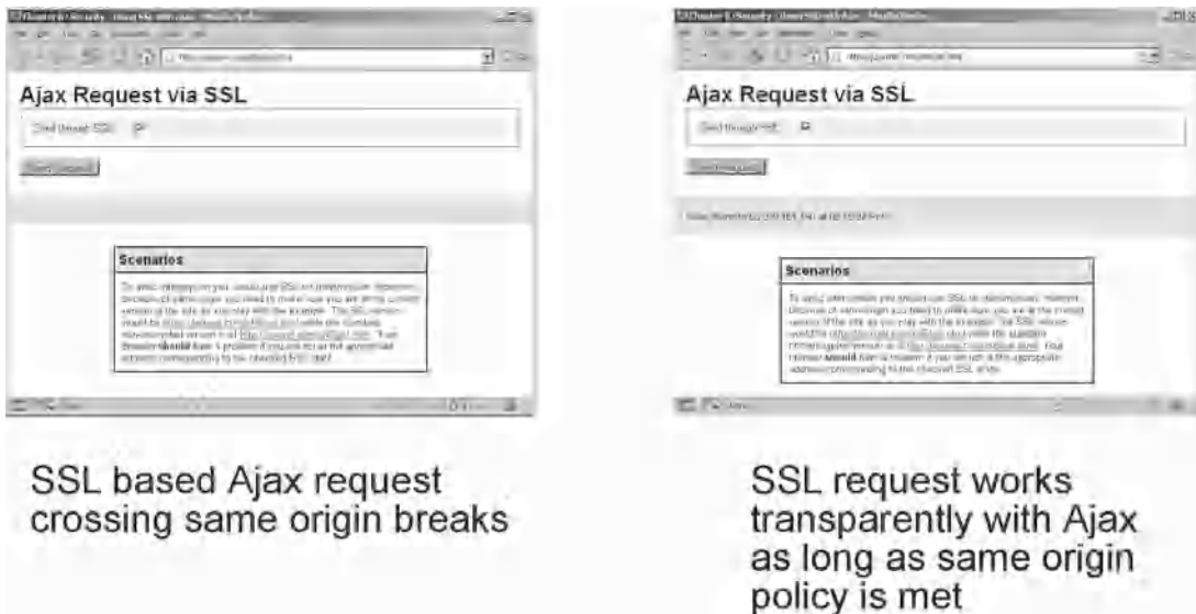
FIGURE 7-7 SSL and Ajax work together fine as long as same origin is respected.
