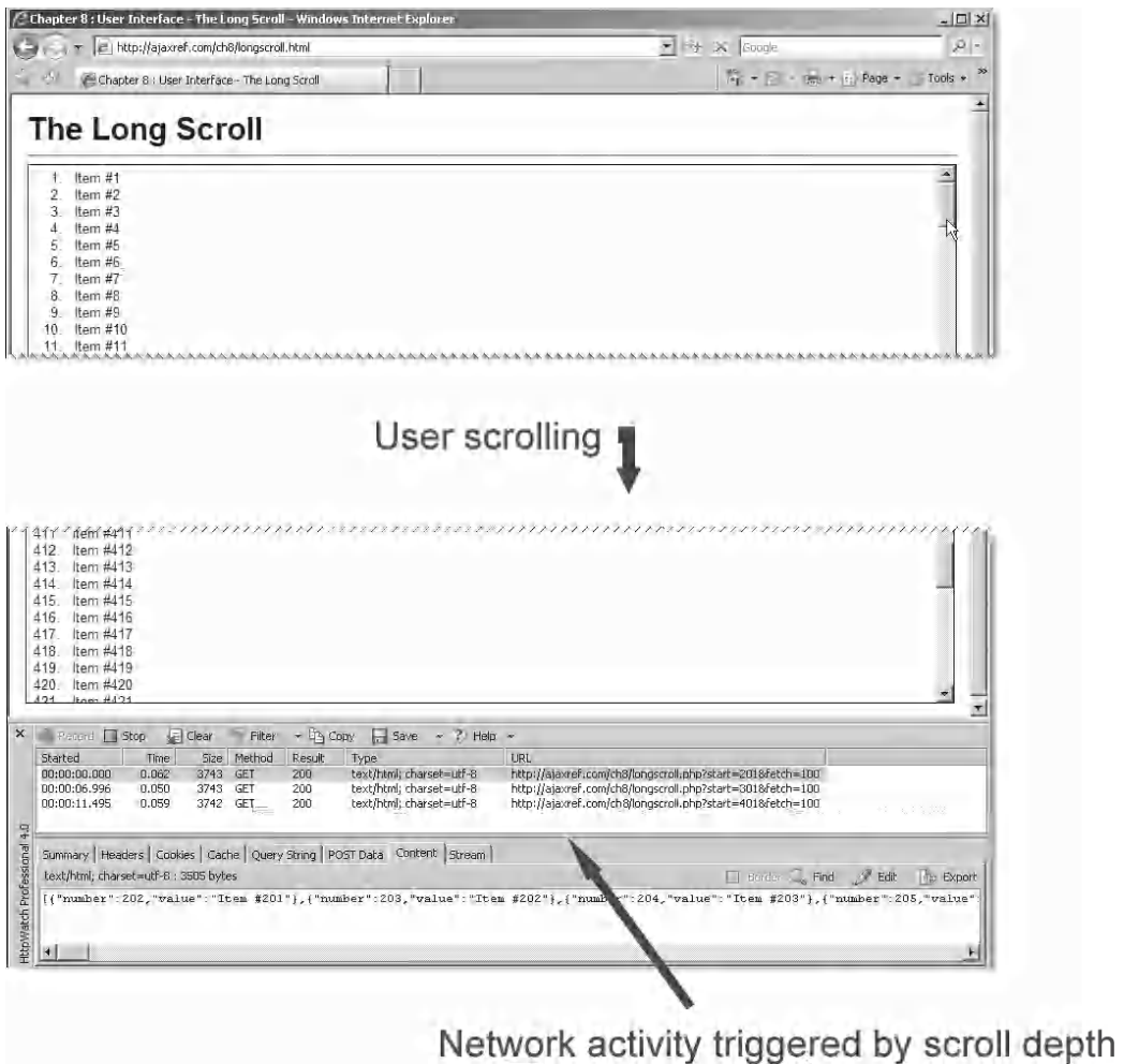
FIGURE 8-17 Scroll to fetch data
