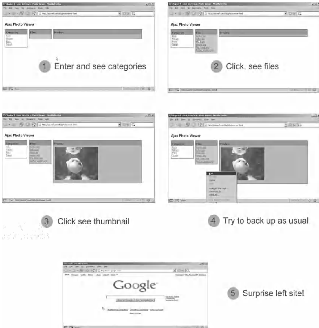
FIGURE 8-21 The back button blues
