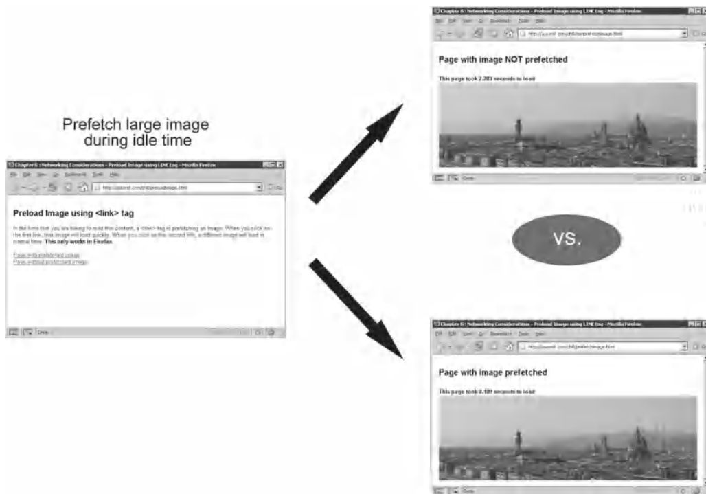
FIGURE 6-22 Big savings via browser-native prefetching
