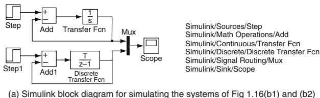
(a) Simulink block diagram for simulating the systems of Fig. 1.16(b1) and (b2)
