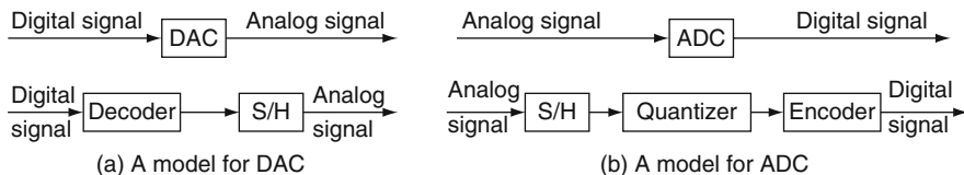
Fig. 5.18 Models for DAC and ADC
