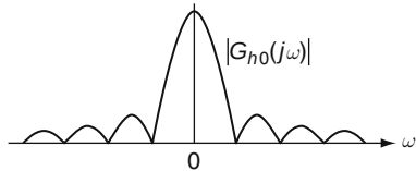
(b) The magnitude response of a z.o.h.
