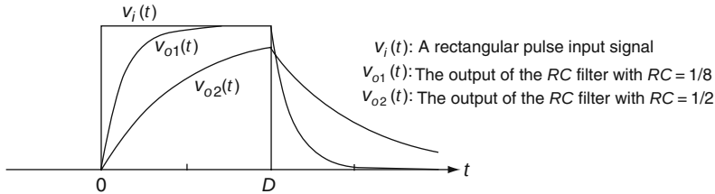
(b) The output voltages to a single rectangular pulse input
