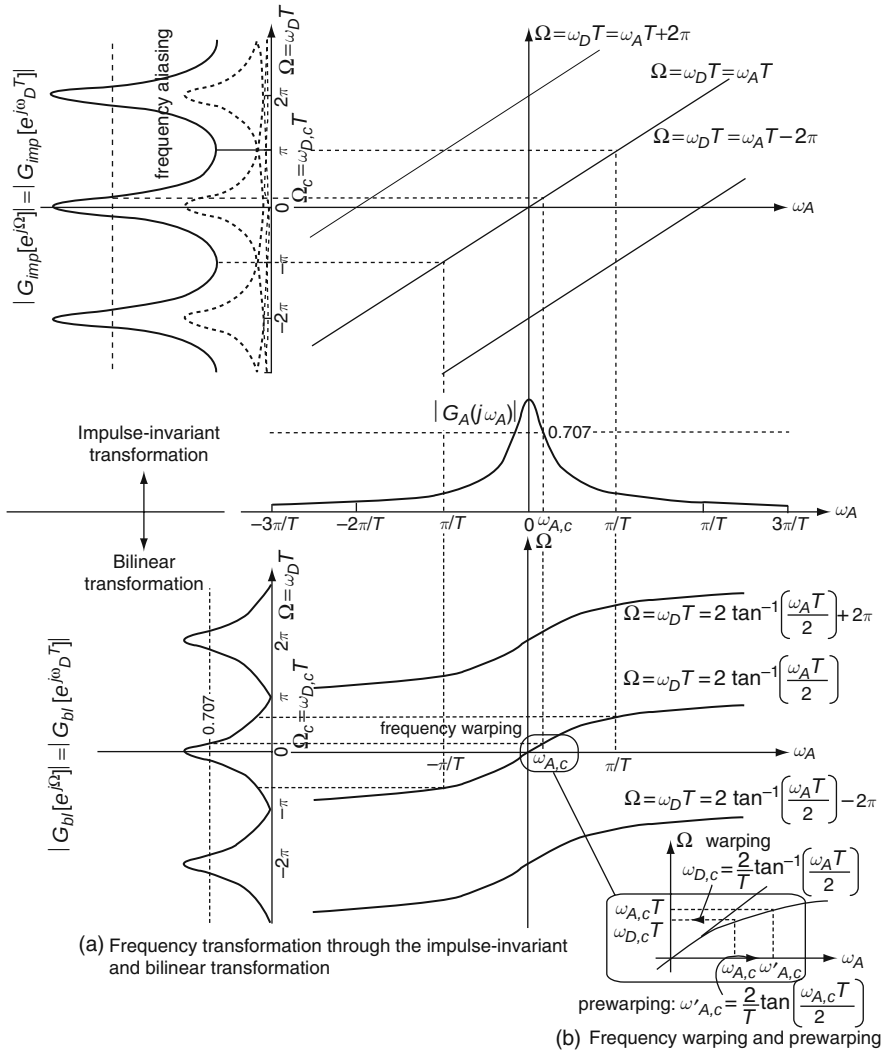
Fig. 6.8 Frequency transformation
