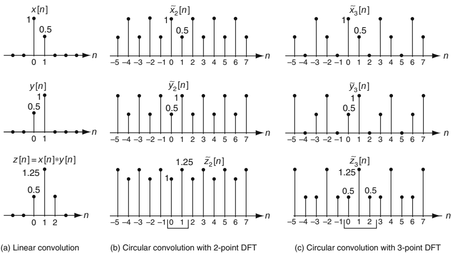
Fig. 3.10 Linear and circular convolutions with DFT
