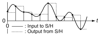
(a) The input and output of a S/H
