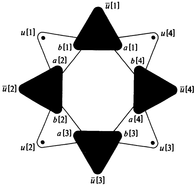
Figure 3.2 Truth setting component T_i when m=4 (subscripts have been deleted for simplicity). Either all the sets of T_i^f (the shaded sets) or all the sets of T_i^t (the unshaded sets) must be chosen, leaving uncovered all the u_i[j] or all the \bar{u}_i[j] , respectively.
