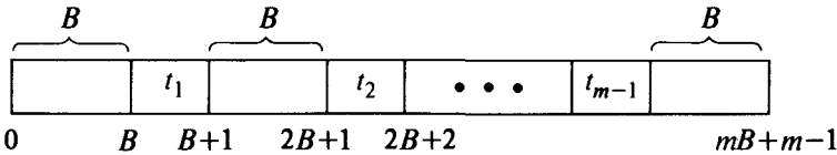
Figure 4.9 The form required of a sequence meeting the constraints of an instance of SEQUENCING WITHIN INTERVALS obtained by transforming an instance of 3-PARTITION in the proof of Theorem 4.5.
