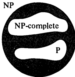
Figure 2.6 The world of NP, revisited.
