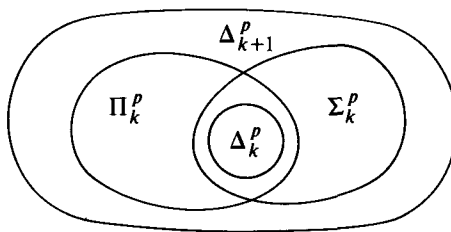
Figure 7.5 Containment relationships within the polynomial hierarchy.
