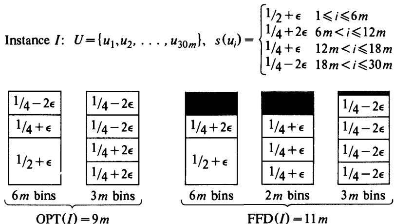
Figure 6.3 Instances I with \text{OPT}(I) arbitrarily large such that \text{FFD}(I) equals (11/9)\text{OPT}(I) .
