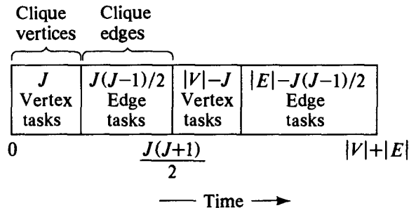
Figure 3.10 Diagram of the desired schedule for an instance of MINIMUM TARDINESS SEQUENCING corresponding to a CLIQUE of size J .
