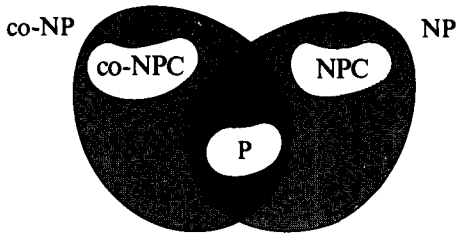
Figure 7.2 The world of NP and vicinity (assuming P \neq NP and NP \neq \text{co-NP} ). It may or may not be the case that P = NP \cap \text{co-NP} .
