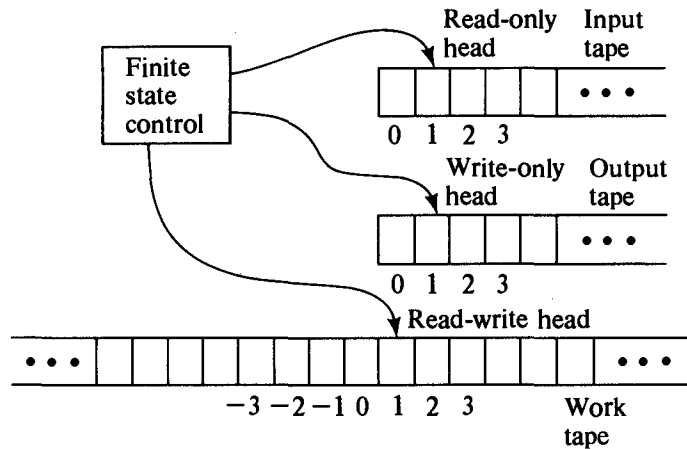
Figure 7.6 Schematic representation of a DTM model in which it is possible to use less than linear space.
