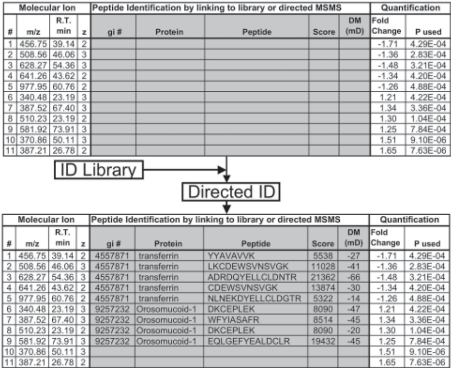
Fig. 4. Identification (ID) using libraries. After obtaining profiling data, matches to the ID library are linked. Unmatched components of interest (low p -values) are targeted for ID by directed tandem mass spectrometry. Finally, differentially profiled proteins can be observed. Proteins with more than one peptide showing consistency in fold change, as shown in the figure, are more reliable. There still may be profiled molecular ions that are difficult to identify because of poor fragmentation or the presence of posttranslational modifications.
