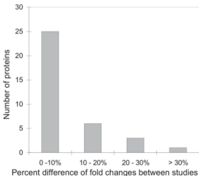
Fig. 5. Histogram of percent difference in fold changes recorded on repeat analysis (1D liquid chromatography–mass spectrometry rheumatoid arthritis studies separated by 10 mo). Data is shown for 35 statistically significant ( p < 0.05 ) putative protein biomarkers.
