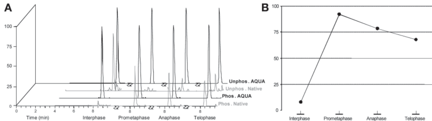
Fig. 2. Liquid chromatography-selected reaction monitoring (LC-SRM) analysis of cell-cycle, stage-specific phosphorylation of separase at serine 1126. (A) Absolute quantification (AQUA) and native LC-SRM channels for the phosphorylated and unphosphorylated tryptic peptides containing serine 1126 at interphase, prometaphase, anaphase, and telophase. The individual ion chromatograms are normalized to the intensity of each AQUA peptide. Note the relative decrease in intensity of the phosphorylated peptide signal after release from nocodazole, and the concomitant increase in signal for its unphosphorylated cognate. (B) The peak areas for each species in A is transformed into percent phosphorylation values at each time point.
