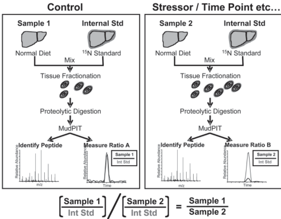
Fig. 5. General approach for measuring relative protein differences using metabolically labeled internal standards (IS). Each sample is mixed with an identical ^{15}\text{N} -enriched IS prior to sample preparation. Differences are evaluated using a ratio of two ratios to minimize systematic errors and to facilitate relative abundance measurements between greater than two samples.
