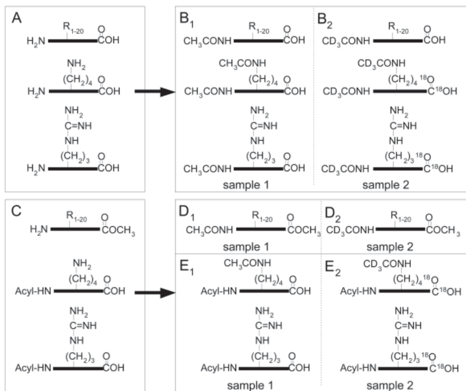
Fig. 1. A scheme for tagging amino and carboxyl termini of peptides simultaneously. The amino acid side chains in this illustration are on the C-terminal amino acid of the peptide. The bold solid line is the rest of the peptide backbone. (A) illustrates the general types of peptides obtained from unblocked proteins. (B 1 ) shows how these peptides would be derivatized when a proteome sample was tryptic digested in \text{H}_2^{16}\text{O} and derivatized with N\text{-(}^1\text{H}_3\text{)acetoxy succinimide} . (B 2 ) shows how peptides from a second sample would be derivatized when they were tryptic digested in \text{H}_2^{18}\text{O} and derivatized with N\text{-(}^2\text{H}_3\text{)acetoxy succinimide} . (C) illustrates peptides that would be obtained from proteins that are either N-terminally or C-terminally blocked. A methyl ester is used as an example of a C-terminal block. Differential labeling of the C-terminally blocked peptides from two samples is illustrated in (D 1 ) and (D 2 ) . Differential labeling of the N-terminally blocked peptides from these samples is seen in (E 1 ) and (E 2 ) . Note that in the case of terminally blocked peptides, only one end of the peptide is labeled. After differential labeling of the samples they are mixed and analyzed by liquid chromatography–mass spectrometry.
