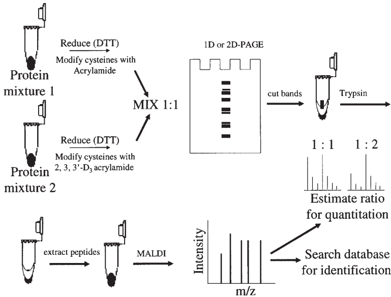
Fig. 1. Diagram depicting the general scheme for relative quantification. The cysteines from two protein mixtures in which the relative protein quantification needs to be determined are separately reduced and alkylated using acrylamide and D 3 -acrylamide. The two samples are then mixed in a 1:1 ratio and the proteins are separated using gel electrophoresis. The proteins of interest are excised from the gel, digested with trypsin, and the tryptic peptide maps obtained by MALDI-TOF. The isotopic envelopes of the cysteine-containing peptides are used to determine the relative quantities of the proteins in the two samples. A schematic representation of the isotopic envelope for a cysteine-containing peptide in the case when the protein is present in equal amounts and in a 1:2 ratio in the two samples is shown. The same mass spectrum is used for identifying or confirming the protein. Reproduced with permission from ref. 9 .
