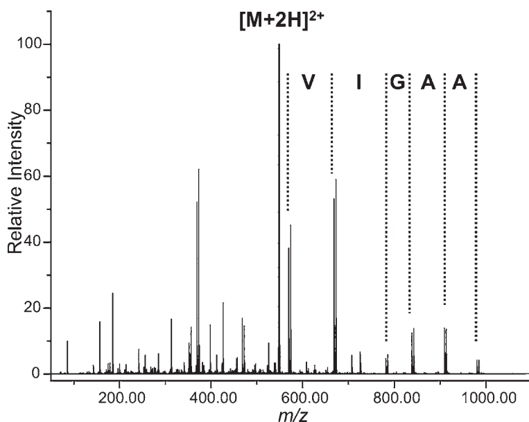
Fig. 3. Tandem mass spectrum of a pair of peptides carrying ^{18}\text{O} or ^{16}\text{O} labels at their carboxyl termini. Pairs of fragment ions containing the C-termini ( \gamma ions) are indicated, from which a partial sequence has been deduced.
