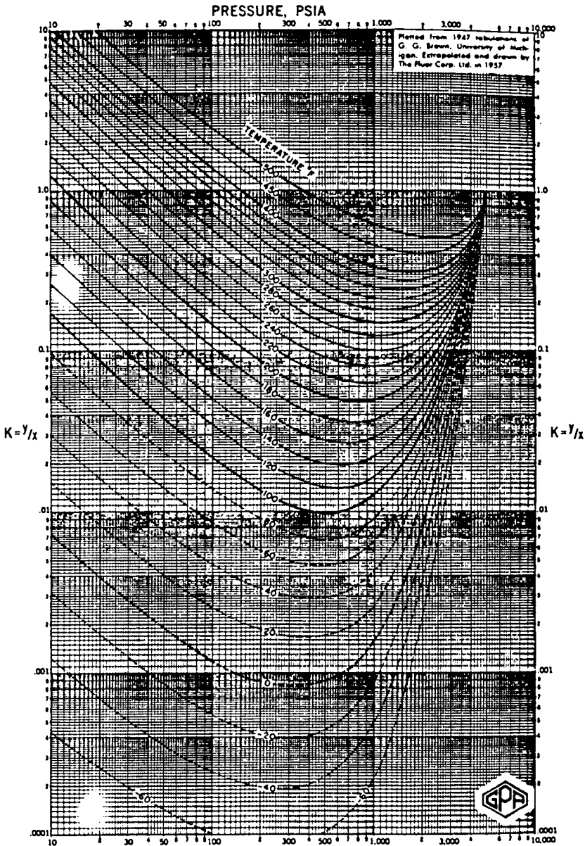
Figure 9. Heptane. Conv. press. 5,000 psia. Courtesy of the Gas Processors Suppliers Association. Published in the GPA Engineering Data Book, Tenth Edition, 1987.
