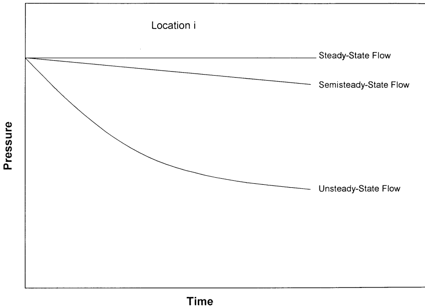
Figure 6-3. Flow regimes.
