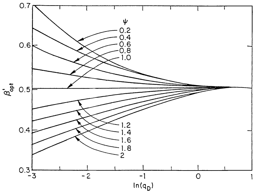
Figure 9-26. Optimum well placement for two-cone case. (After Paptzacos, P. et. al., courtesy SPE, 1989.)
