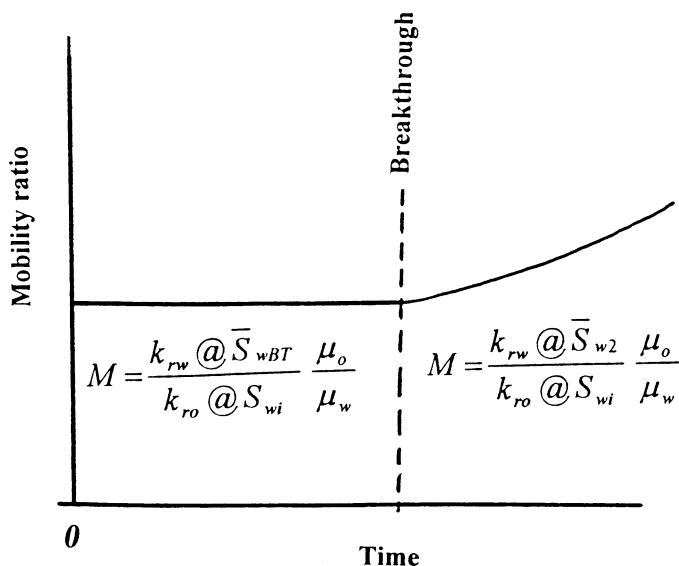
Figure 14-33. Mobility ratio versus time relationship.
