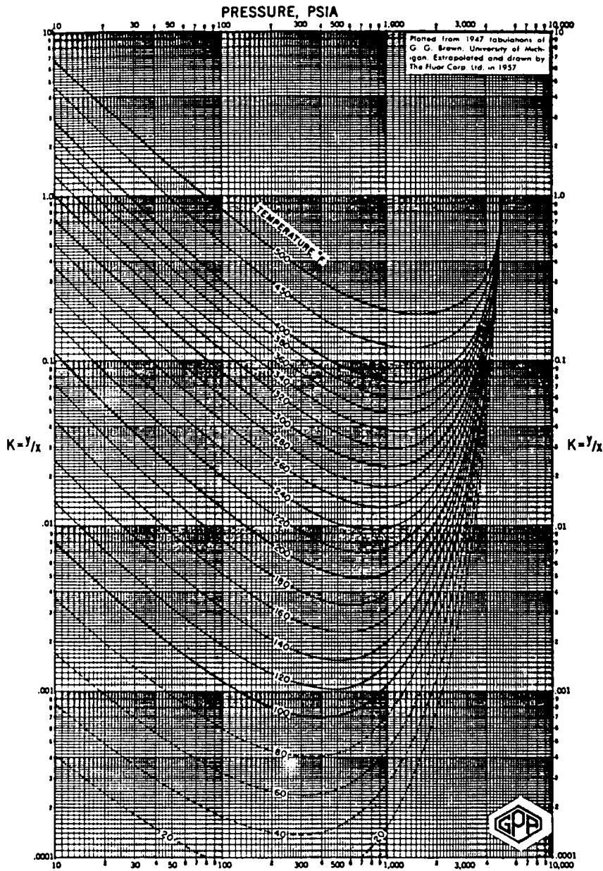
Figure 12. Decane. Conv. press. 5,000 psia. Courtesy of the Gas Processors Suppliers Association. Published in the GPPA Engineering Data Book, Tenth Edition, 1987.
