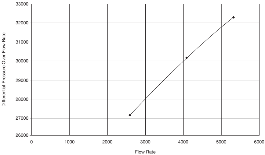
Figure 8-12. Pseudopressure method.
