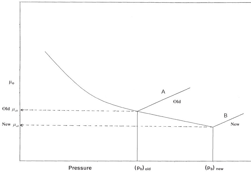
Figure 3-11. Extrapolating oil viscosity above new p_b .
