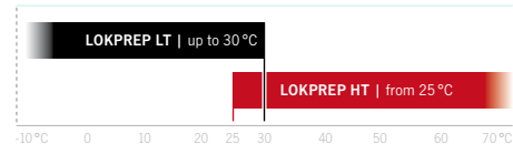
LOKPREP application depending on the ambient temperature in °C
