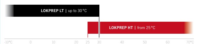
LOKPREP application depending on the ambient temperature in ^{\circ}\text{C}
