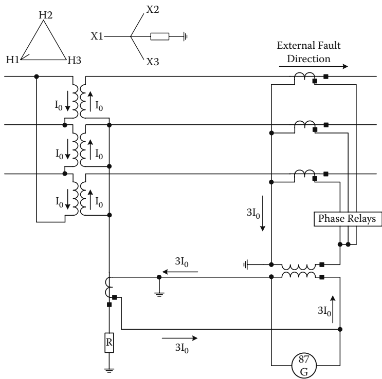
FIGURE 11.12 Ground-differential scheme of a Delta-Wye transformer
