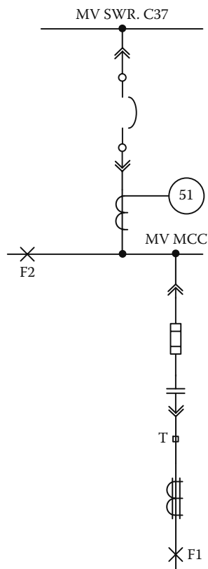
FIGURE 7.15 Medium-voltage MCC
