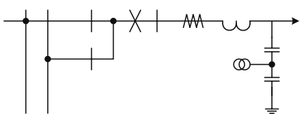
FIGURE 12.7 Double-bus arrangement
