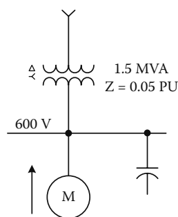
FIGURE 15.9 Example of a resonance risk calculation
