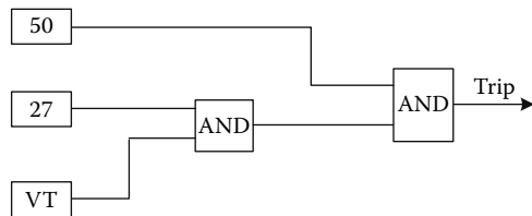
FIGURE 11.37 Inadvertent emerging (AF) using voltage-supervised current relay
