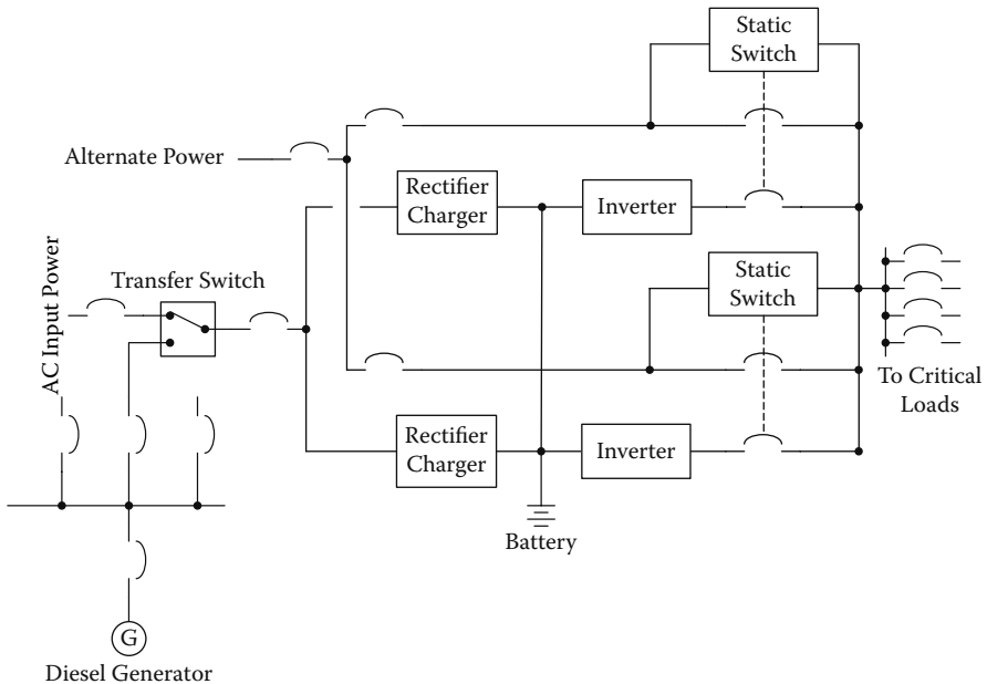
FIGURE 2.3 Redundant UPS
