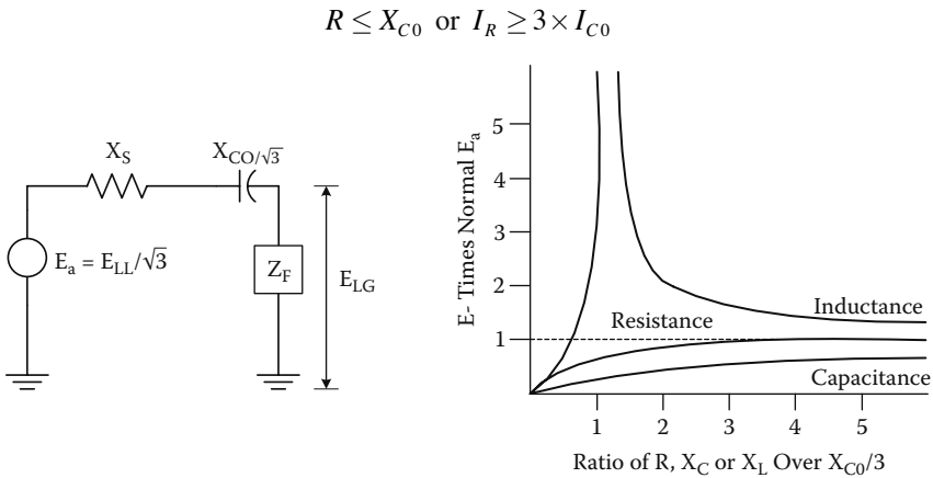
FIGURE 4.4 Overvoltage due to ground fault through an impedance
