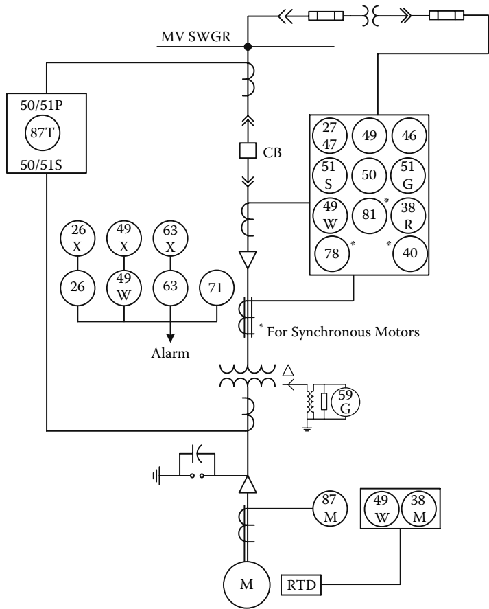
FIGURE 11.20 Typical protection features for MV motor and captive (unit) transformer
