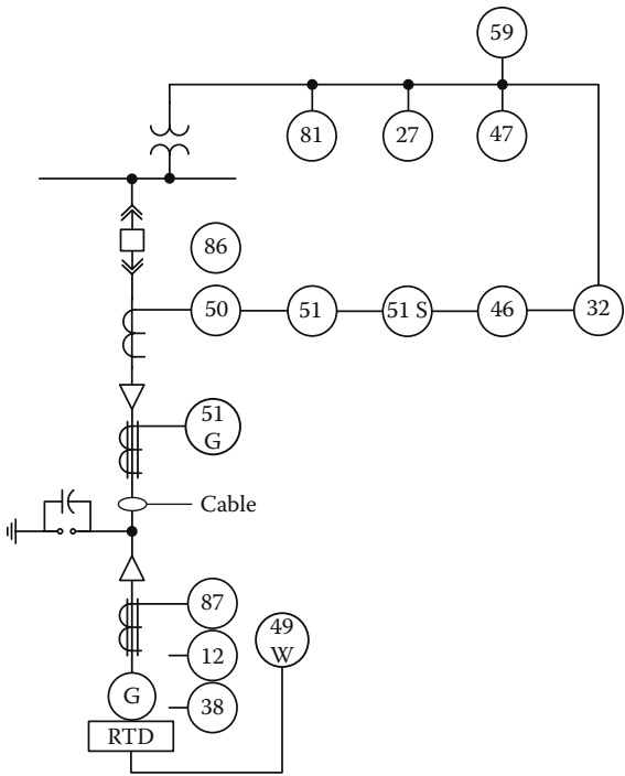
FIGURE 14.17 Typical protection features for an industrial generator
