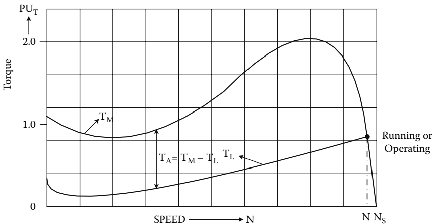
FIGURE 9.3 Speed–torque curve
