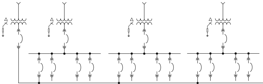
FIGURE 2.8 Sparring transformer
