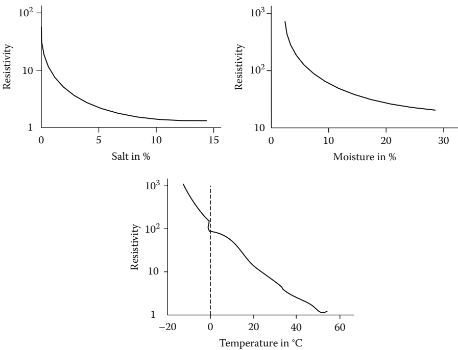
FIGURE 13.3 Earth-resistivity variations
