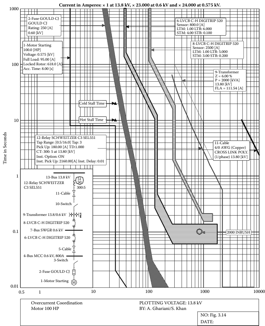
FIGURE 3.14 Overcurrent coordination
