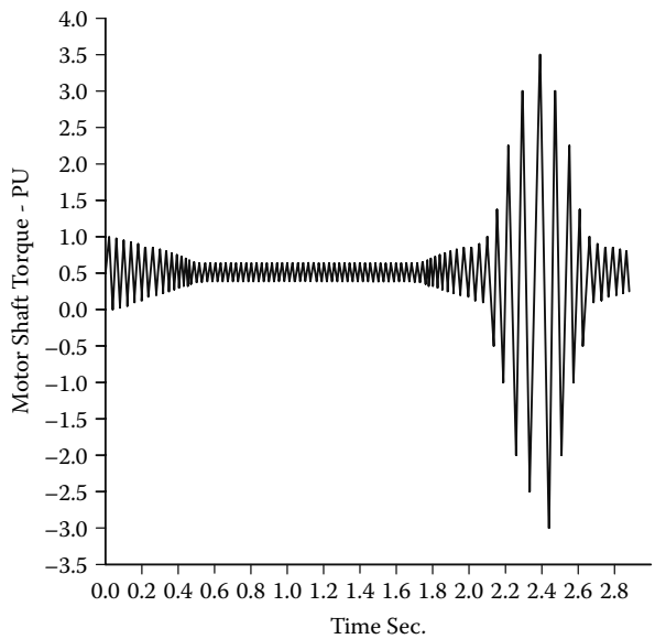
FIGURE 9.14 Torque pulsation
