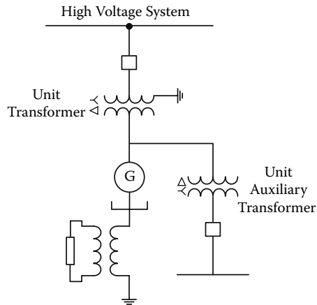
FIGURE 14.9 Unit-connected generator
