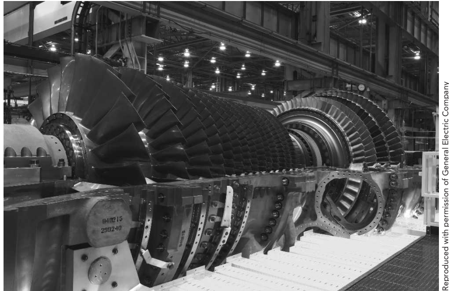
Fig. 10.3 Photograph of a multiple-stage axial-flow compressor rotor for a gas turbine.
