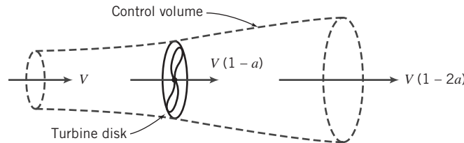
Fig. 10.40 Control volume and simplified notation used to analyze wind turbine performance.
