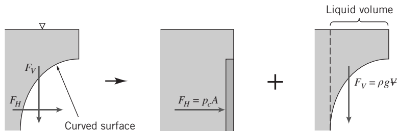
Fig. 3.8 Forces on curved submerged surface.
