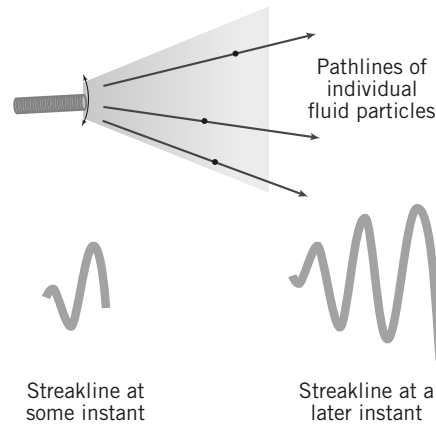
Fig. 2.5 Pathlines and streaklines for flow from the exit of an oscillating garden hose.
