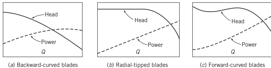
Fig. 10.25 General features of performance curves for centrifugal fans with backward-, radial-, and forward-curved blades.
