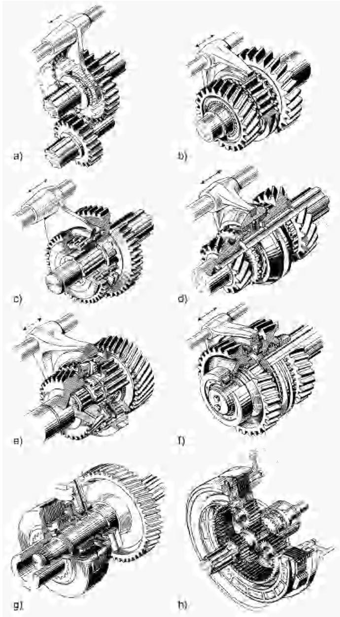
Fig. 9.1. Internal shifting elements in automotive transmissions. a Sliding gear; b dog clutch engagement; c pin engagement; d synchronizer without locking mechanism; e synchronizer with locking mechanism; f servo lock synchronizer mechanism (Porsche system); g hydraulically activated multi-plate clutch for powershift transmission; h hydraulically activated multi-plate brake for planetary gear [9.17]
