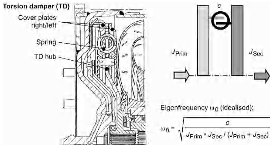
Fig. 10.37. Mechanical torsional vibration damper in a torque converter
