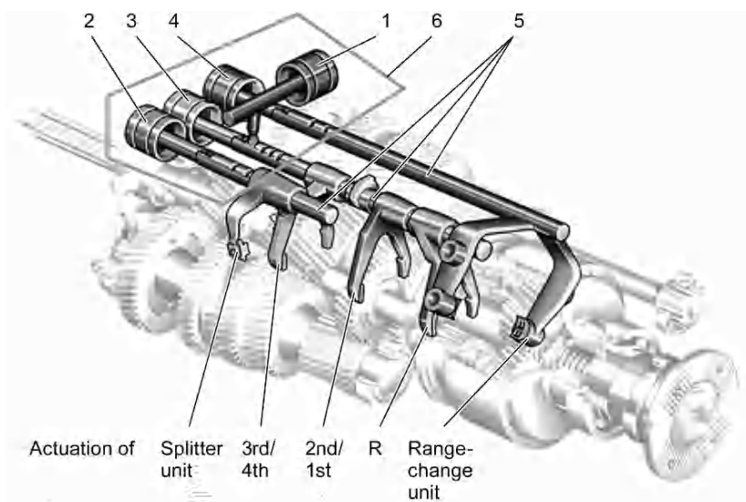
Fig. 12.42. Internal gearshift system of the 16-speed three-range automated gearbox ZF AS-Tronic 16 AS 2230 TD. 1 Selector cylinder for main gearbox; 2 shift cylinder for splitter unit; 3 shift cylinder for main gearbox; 4 shift cylinder for range-change unit; 5 selector bars and shift forks; 6 transmission actuator module
