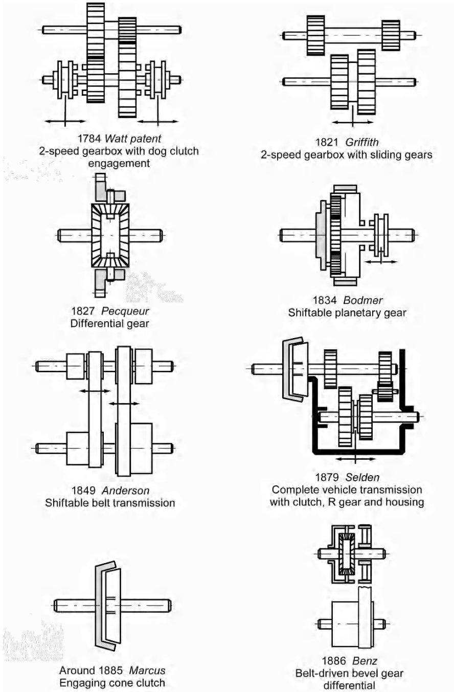
Fig. 1.12. Early vehicle components and gears
