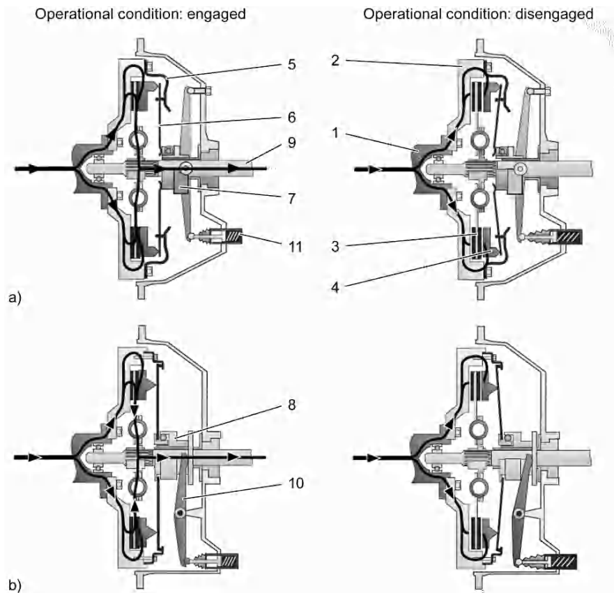
Fig. 10.8. Schematic diagram of push-type (a) and pull-type (b) clutch actuation with operational conditions and power flows. 1 Engine crankshaft; 2 flywheel; 3 clutch plate; 4 pressure plate with support for 6; 5 pressure plate housing with support for 6; 6 diaphragm spring with release tongues; 7 push-type release device; 8 pull-type release device; 9 transmission input shaft; 10 release lever; 11 slave cylinder
