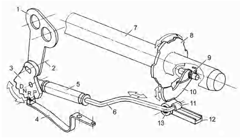
Fig. 9.47. Parking lock with radially acting locking pawl (see also Figure 12.22). 1 Gearshift lever on the transmission; 2 axis selector shaft; 3 detent plate ( P park position, R reverse gear position, N neutral position, D drive position); 4 detent spring; 5 compression spring; 6 connecting rod; 7 output shaft; 8 parking lock wheel; 9 return spring; 10 pawl; 11 locking roller; 12 guide; 13 roller bearing
