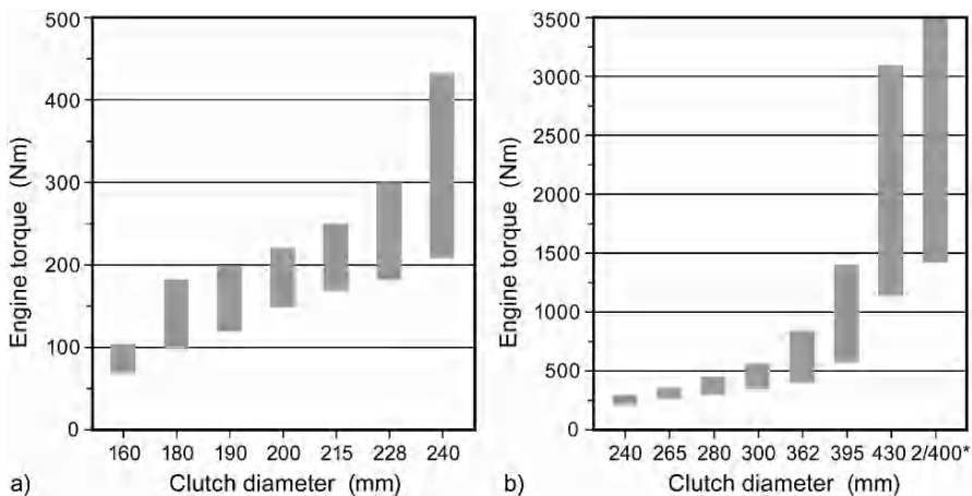
Fig. 10.11. Bandwidths of practical clutch designs for a passenger cars/vans and b commercial vehicles [10.37]. * two-plate clutch
