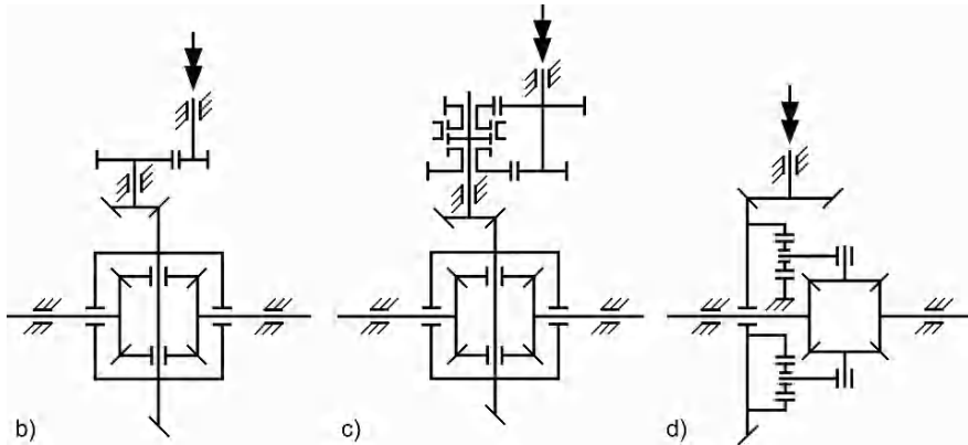
Fig. 6.72. (continued) b countershaft; c two-speed with spur gear countershaft; d two-speed with planetary gear (top: engaged; bottom: not engaged)
