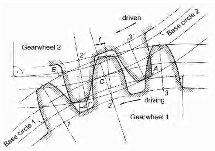
Fig. 7.22. Meshing impact resulting from deformed teeth [7.29]
