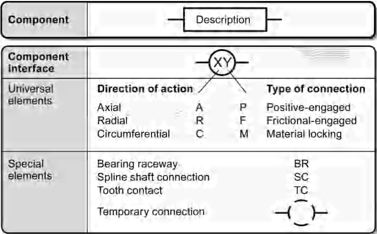
Fig. 17.14. Elements of the function block diagram for the single-cone synchronizer
