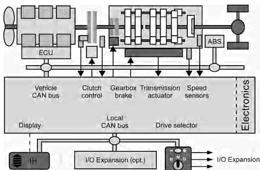
Fig. 13.4. System diagram for an automated manual transmission (AMT) using the example of a 16-speed commercial vehicle transmission
