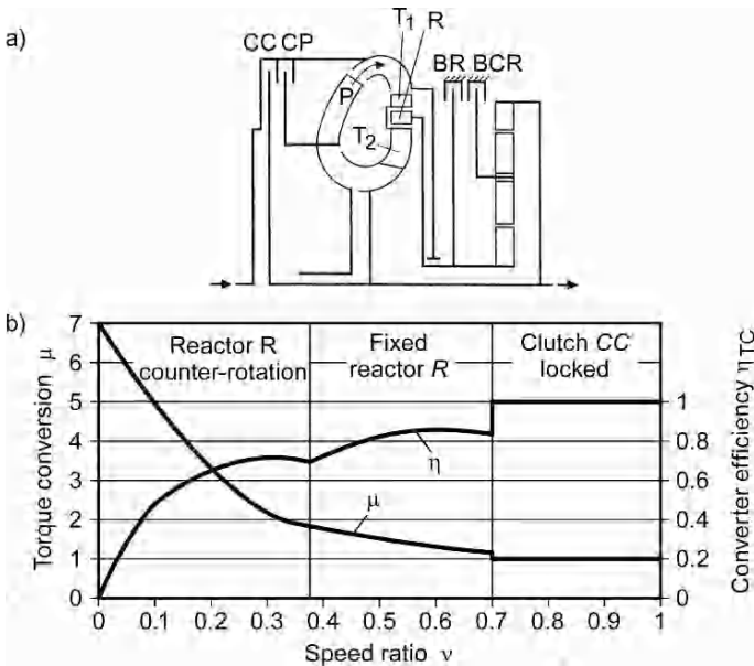
Fig. 10.43. Torque converter with internal power-split (SRM principle Doromat, Renk).
