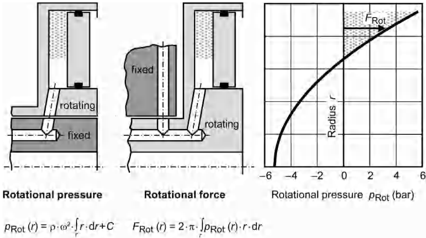
Fig. 9.43. Rotational pressure in rotating, oil-filled piston chambers
