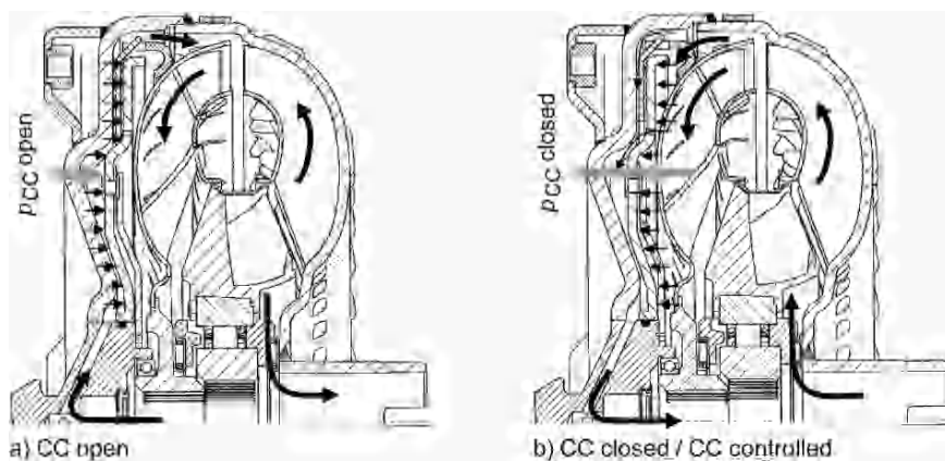
Fig. 10.36. Working principle of slip-controlled torque converter lock-up clutches (SCC) with a 2-line converter. a Open; b closed and controlled
