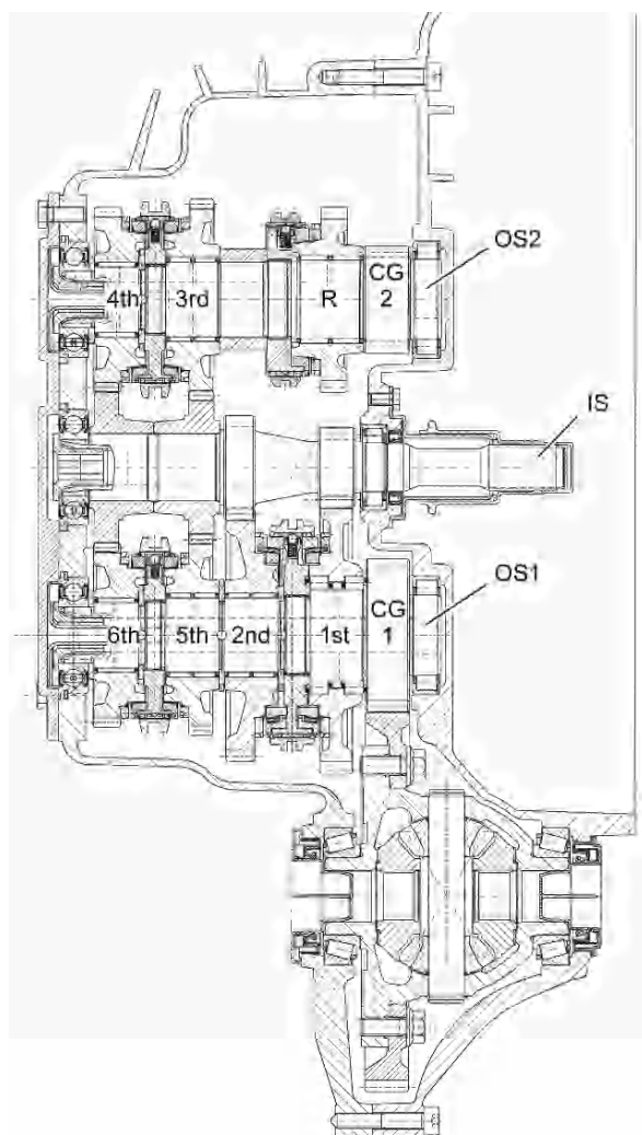
Fig. 12.7. 6-speed manual passenger car gearbox Getrag 285, gearbox diagram Figure 6.21a
