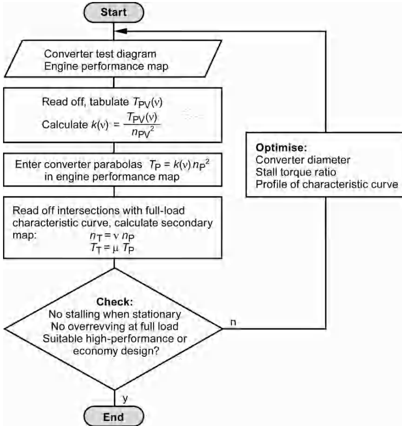
Fig. 10.29. Manual calculation algorithm for converter calculation
