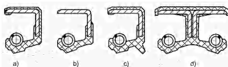
Fig. 11.25. Rotary shaft seals, basic types. a Rubber elastic external shell; b metallic housing; c with additional dust lip; d double seal for fluid separation
