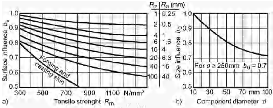
Fig. 8.14. For circular cross-sections: a surface effect b_s ; b size effect b_0
