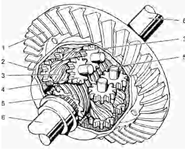
Fig. 12.61. Self-locking differential with worm gears, TORSEN. 1 Driving crown gear; 2 differential housing; 3 worm gears; 4 spur gear toothings; 5 worms; 6 output shafts
