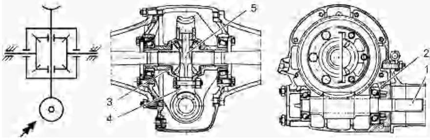
Fig. 12.54. Axle drive of the Peugeot 404 with worm gear drive. 1 Worm shaft; 2 angular contact ball bearing; 3 differential cage; 4 worm gear; 5 bevel gear differential
