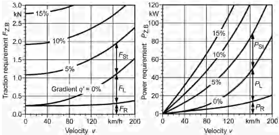
Fig. 3.4. Traction required and the resultant power required for a mid-size passenger car. For vehicle data see Figure 5.3
