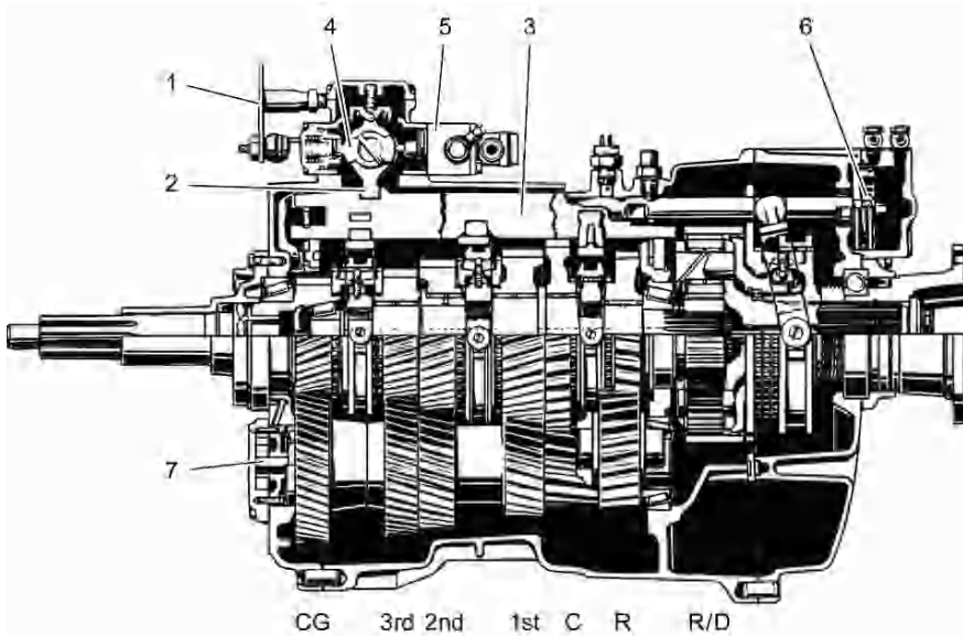
Fig. 12.34. 9-speed (4 x 2 + crawler) commercial vehicle gearbox ZF 9 S 109 with direct drive design; gearbox diagram and power flows Figure 6.53. 1 Connection for turning shaft remote control; 2 selector finger; 3 selector bars; 4 cam plate; 5 shift valve for the range-change unit; 6 shift cylinder for the range-change unit; 7 lubricating oil pump; CG constant gear; C crawler; R/D range-change unit: R range; D direct
