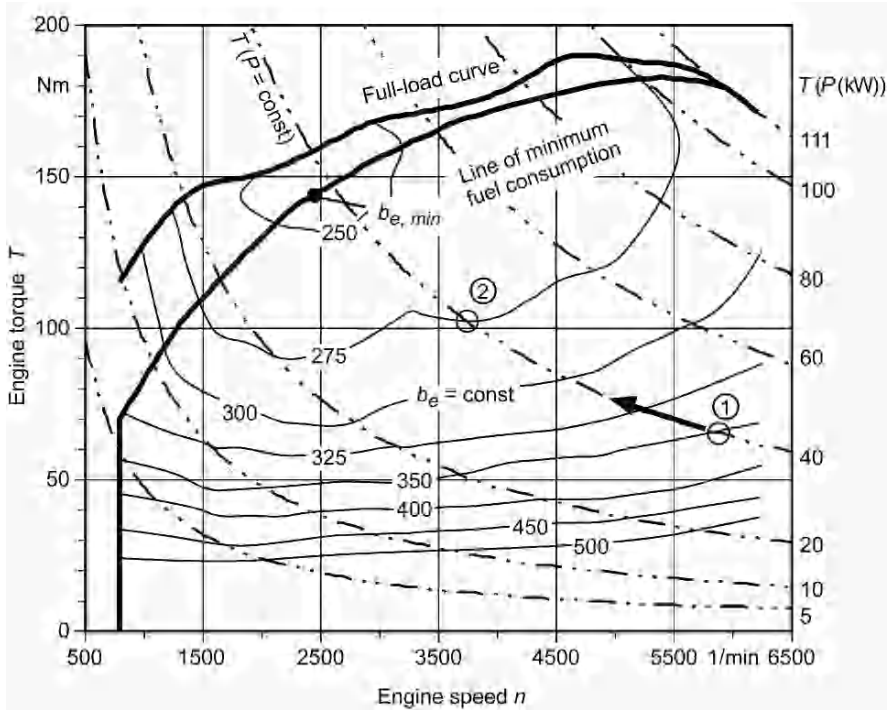
Fig. 3.18. Engine map (“onion diagram”), specific fuel consumption b_e in g/kWh. Consumption map of a 2.0 litre spark ignition engine with 111 kW
