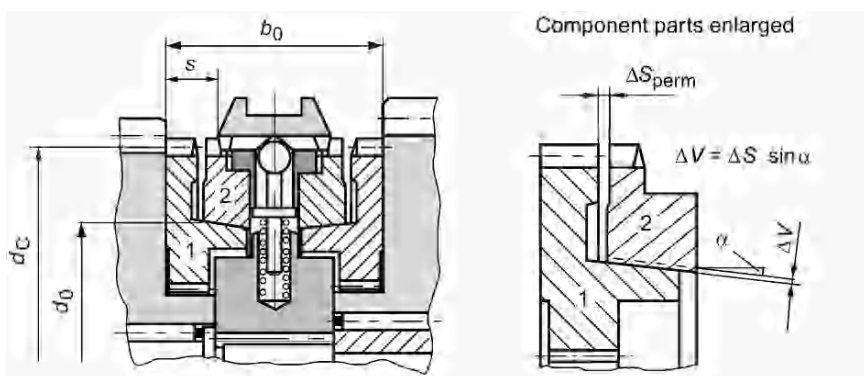
Fig. 9.11. Dimensions. b_0 Overall pack length; d_0 nominal diameter; d_c clutch diameter; \Delta S wear path; \Delta S_{perm} permissible wear path incl. clearance; s shift stroke at the gearshift sleeve; \Delta V wear at the synchronizer ring; \alpha cone angle
