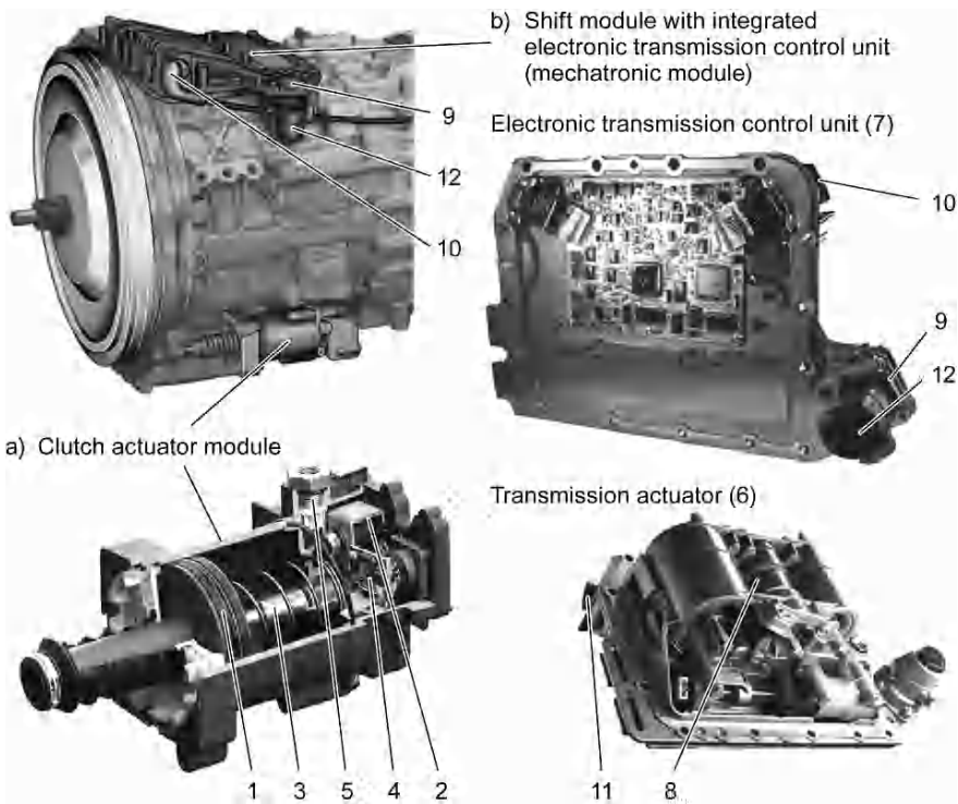
Fig. 12.43. Position and structure of the clutch and shift module of the 16-speed three-range automated gearbox ZF AS-Tronic 16 AS 2230 TD. a Clutch actuator module: 1 actuating piston; 2 magnet valves for controlling clutch actuators; 3 travel sensor; 4 evaluating electronics; 5 compressed air connection with non-return valve; b transmission actuator with integrated electronic TCU (shift module): 6 transmission actuator; 7 electronic TCU; 8 magnet valves, shift cylinders and sensors; 9 pressure limiting valve; 10 gearbox connector; 11 vehicle connector; 12 compressed air connection
