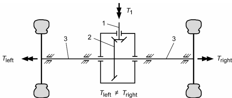
Fig. 6.73. Principle of a rigid, non-compensating differential gear. 1 Drive; 2 bevel gear; 3 axle shaft
