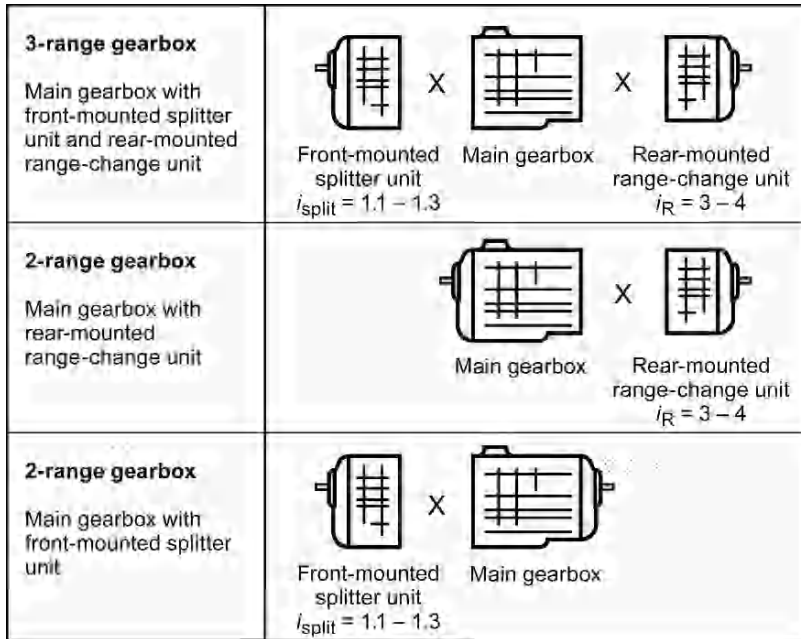
Fig. 6.50. Conventional configurations with two-range and three-range gearboxes
