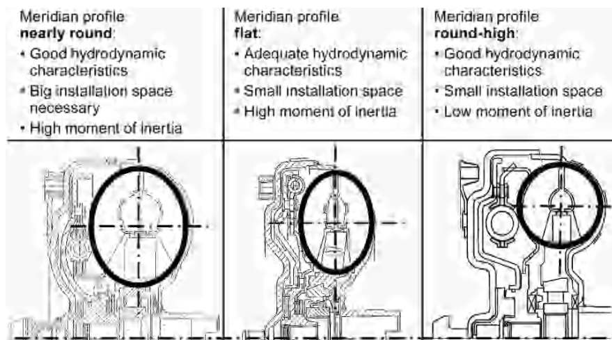
Fig. 10.33. Influence of the meridian profile on hydrodynamic characteristics, installation space and moment of inertia [10.35]
