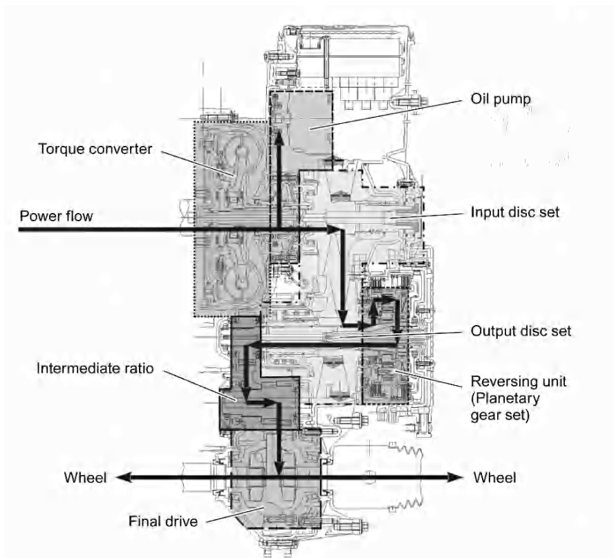
Fig. 12.31. The continuously variable automatic passenger car gearbox Mercedes-Benz Autotronic
