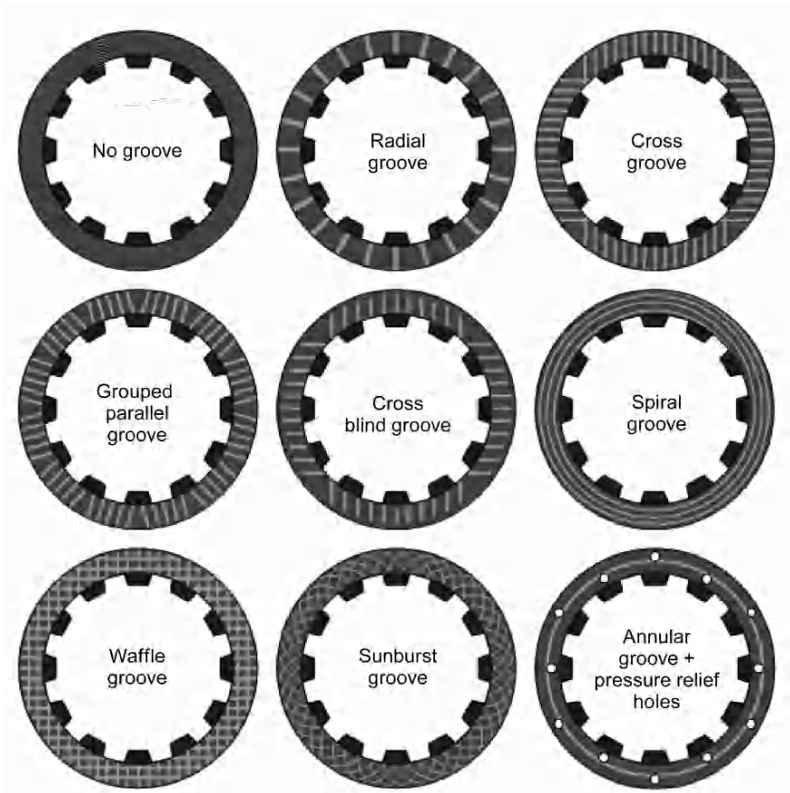
Fig. 9.42. Typical grooving of friction linings (Source: ZF)
