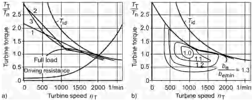
Fig. 10.25. The three Trilok converters from Figure 10.24. a In the turbine map; b Trilok converter 3 in the consumption map
