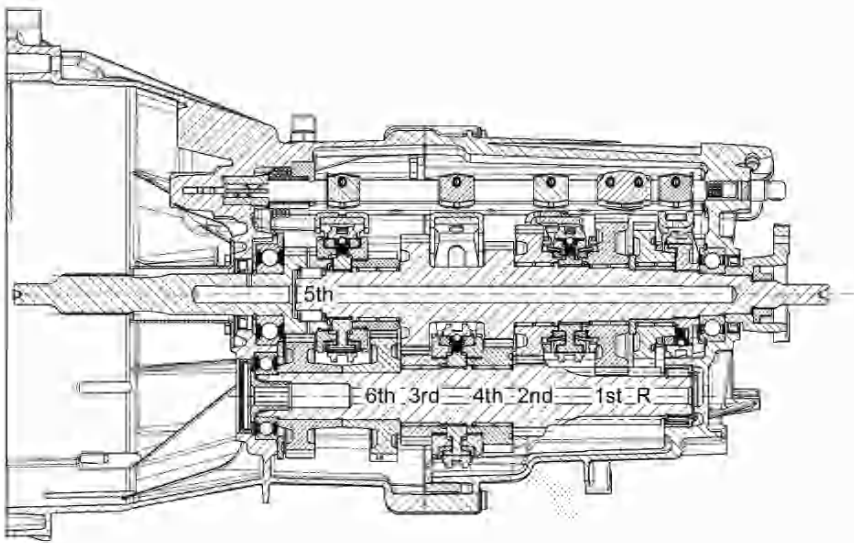
Fig. 12.11. 6-speed manual passenger car gearbox Getrag 217, spark ignition engine design; gearbox diagram Figure 6.22a
