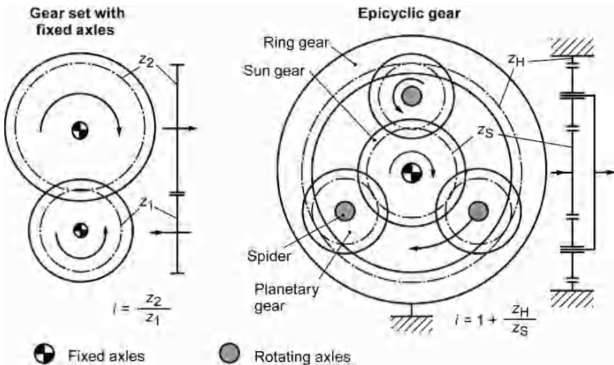
Fig. 6.15. Gear set with fixed axes and epicyclic gear
