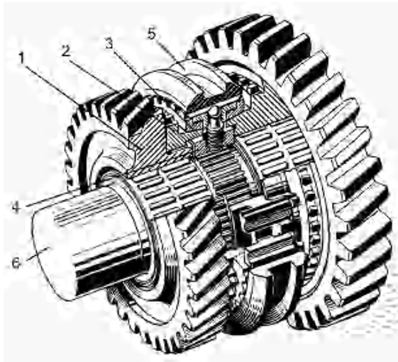
Fig. 9.7. Single-cone synchronizer (ZF-B), see also Figure 9.12.
