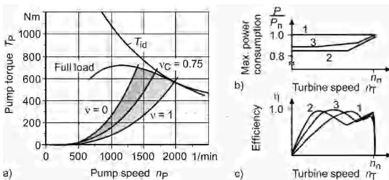
Fig. 10.24. Trilok versions of the converters in Figure 10.23. a Engine operating map with torque converter 3; b maximum power consumption; c efficiency
