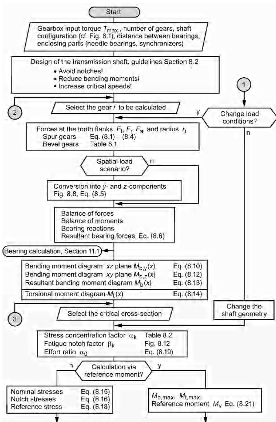
Fig. 8.16. Flow chart for designing transmission shafts
