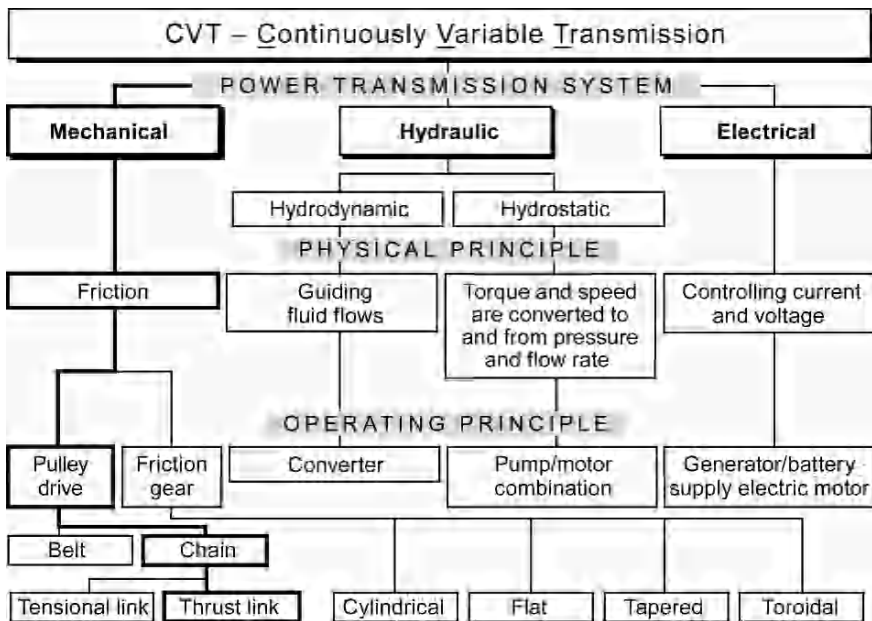
Fig. 6.40. Overview of CVT designs
