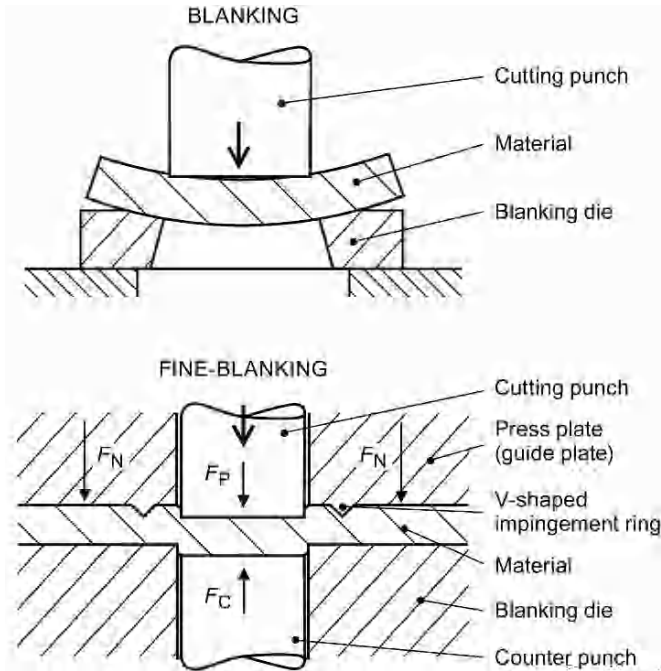
Fig. 16.10. Sheet separation: blanking and fine-blanking [16.7]
