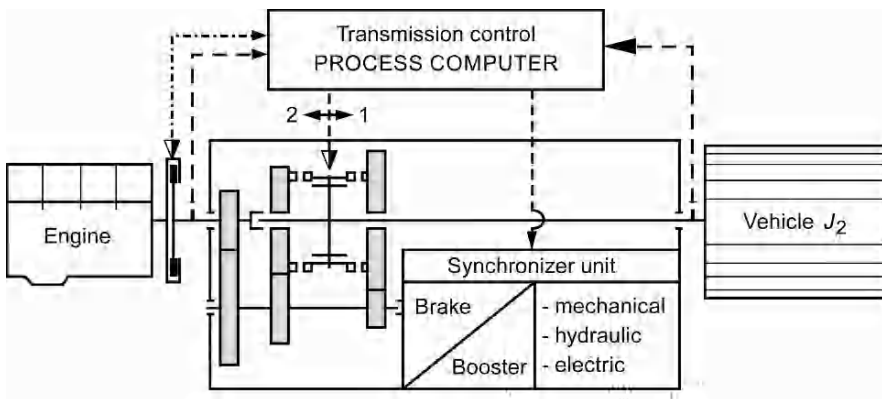
Fig. 9.30. Principle of central synchronization
