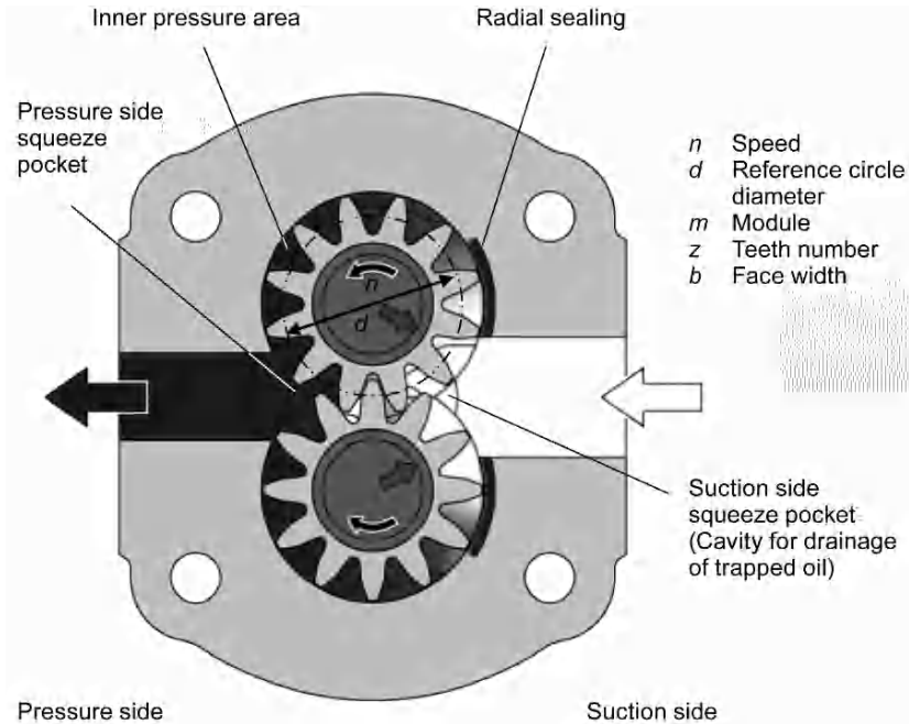
Fig. 11.14. Structure of an external gear pump
