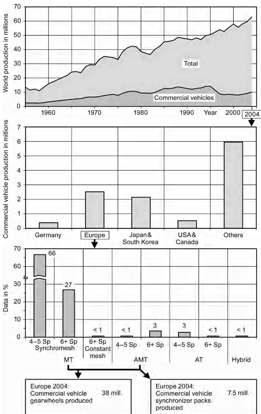
Fig. 2.18. Output figures for commercial vehicles (from [2.16])
