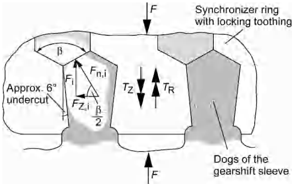
Fig. 9.23. Decomposition of forces at a locking tooth. Opening torque T_Z
