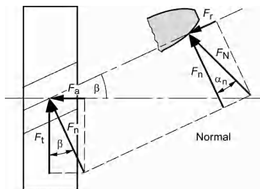
Fig. 8.7. Forces acting at the tooth flanks of a helical-cut spur gear
