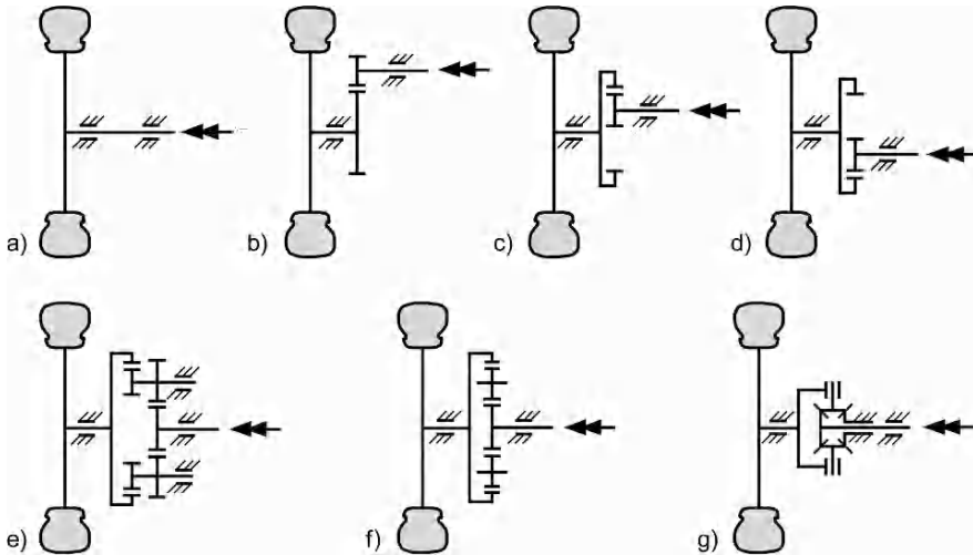
Fig. 6.75. Schematic view of the hub drives. a Without wheel hub drive; b spur gear countershaft with external toothings; c spur gear countershaft with internal toothings, above the wheel axis; d spur gear countershaft with internal toothings, below the wheel axis; e spur gear planetary drive, double planetary drive; f spur gear planetary drive; g bevel gear planetary drive
