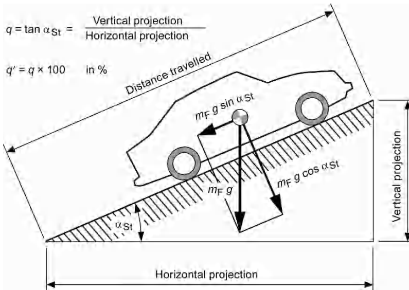
Fig. 3.2. Forces acting on the vehicle travelling uphill
