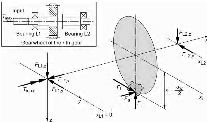
Fig. 8.6. Loading of the transmission input shaft of the theoretical model (single-stage countershaft transmission)
