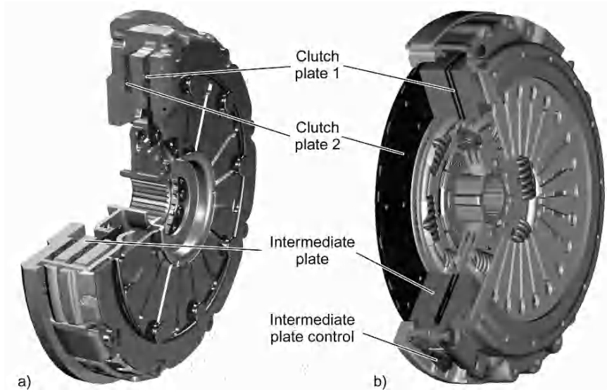
Fig. 10.12. a Two-plate clutch for highly motorised passenger cars (ZF Sachs MF2/228), b commercial vehicle two-plate clutch with intermediate plate control (ZF Sachs) [10.7]
