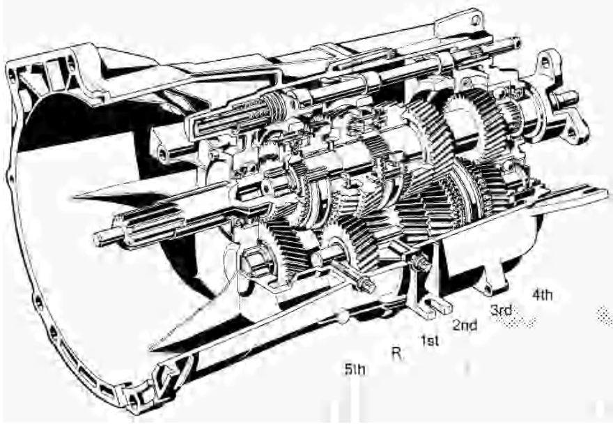
Fig. 12.2. 5-speed manual passenger car gearbox ZF S 5-31, gearbox diagram Figure 6.19b
