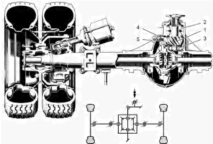
Fig. 12.55. Axle with single ratio, Mercedes-Benz HL 2/11, axle drive shown rotated 90°. 1 Pinion; 2 tapered roller bearing; 3 cylindrical roller bearing; 4 fulcrum pad; 5 crown gear
