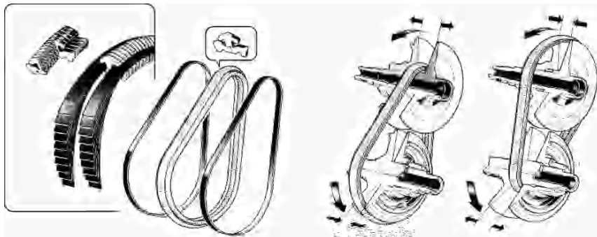
Fig. 6.42. Elements of a thrust link chain and principle of operation of the variator [6.43]
