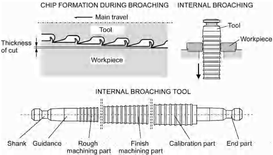
Fig. 16.8. Broaching
