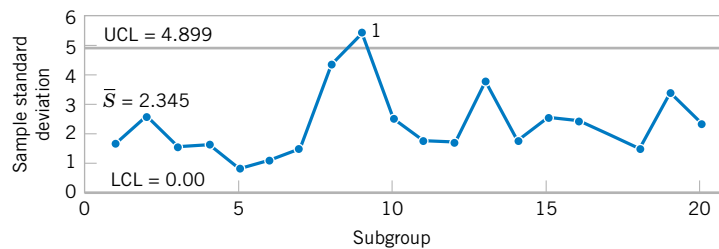
Figure 16-9. The S control chart for vane opening.
