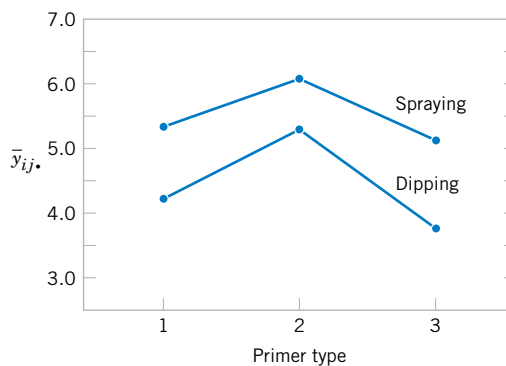
Figure 14-8 Graph of average adhesion force versus primer types for both application methods.
