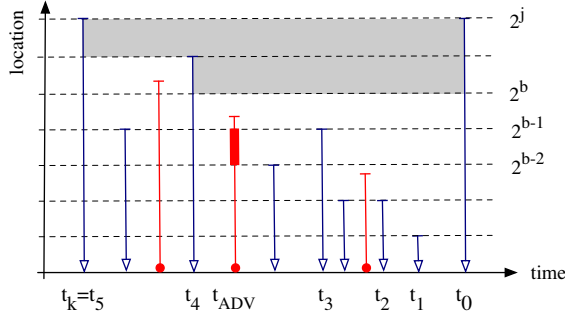
Fig. 1. An example for the analysis of BALANCE's cost at time t_0 . The line (the vertical axis) is shown in the logarithmic scale. The algorithm's transmissions end with empty triangles. The adversary's transmissions end with circles. The algorithm's cost at t_0 is charged to the waiting cost of packets within the shaded area and the 2^{b-1} -to- 2^{b-2} segment of the adversarial transmission (marked with thick line) at t_{ADV} .
