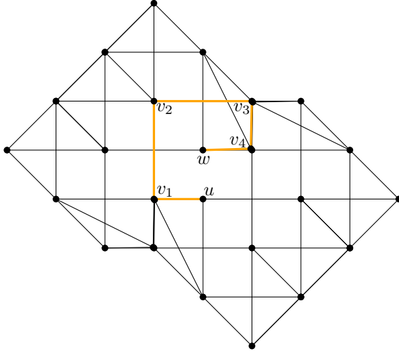
Fig. 9. A lower bound for the \theta_4 -graph. One of the shortest paths from u to w goes via v_1 , v_2 , v_3 , and v_4 .
