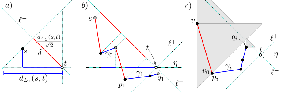
Fig. 4. a) The segment \delta having length d_{L_1}(s,t)/\sqrt{2} . b) The 0-edges of \sigma_{s \rightarrow t} have disjoint projections on \ell^- and the 1-edges have disjoint projections on the horizontal line passing through t . The slope between the endpoints of the maximal paths \gamma_0 and \gamma_1 is less than 1. c) The slope between p^i with q^i is smaller than 1.
