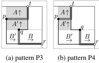
Fig. 6. Types (top = \uparrow / right = \rightarrow ) of the sites inside rectangles A , A' , B , and B' . Fat edges: result after rerouting-ing.
