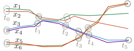
Fig. 1. For m = 2 and \delta > t_4 - t_3 there are four maximal groups: \{x_1, x_2\} , \{x_3, x_4\} , \{x_5, x_6\} , and \{x_1, \dots, x_4\}
