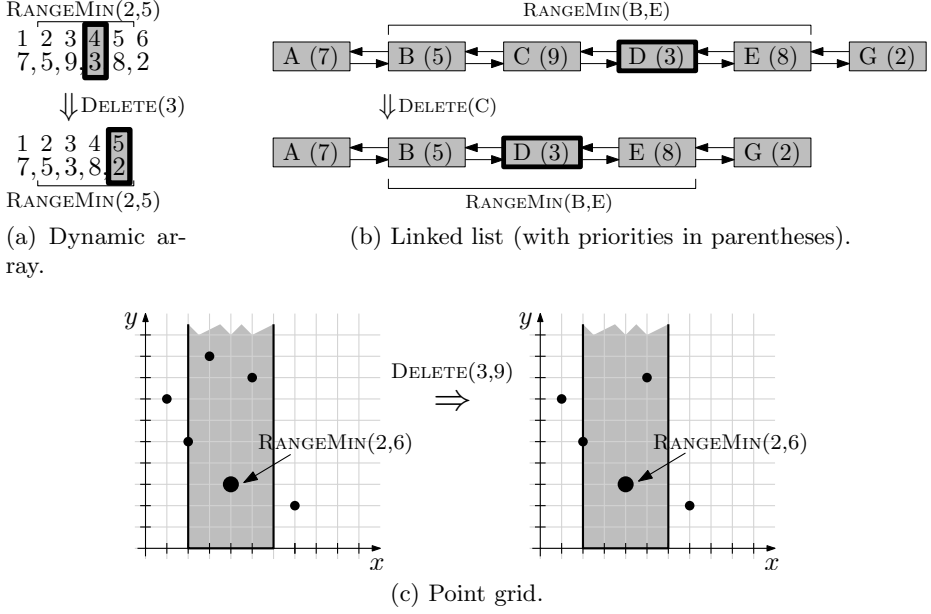
Fig. 1. Different versions of dynamic range minimum queries. Range Minima are shown in bold.
