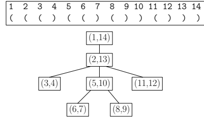
Fig. 2. An example of a well-formed parenthesis string and its associated forest expression
