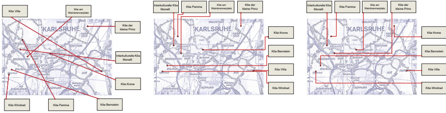
(a) original labeling of kindergartens in Karlsruhe, Germany (b) opo -labeling computed by the algorithm of Bekos et al. [4] (c) po -labeling using the same ports as (b)
