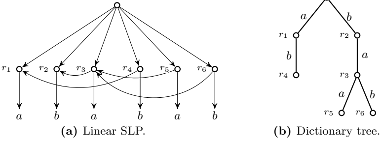
Fig. 2. A Linear SLP compressing the string abbaabbaabab and the dictionary tree obtained from the Linear SLP
