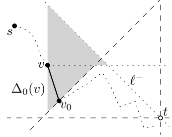
Fig. 3. If v is a t -protected point, then edge vv_0 is light in any path \sigma_{s \rightarrow t} that contains it
