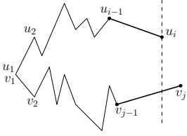
Fig. 4. The s -th vertex u_i from the left and its associated vertices u_{i-1} , v_j and v_{j-1}
