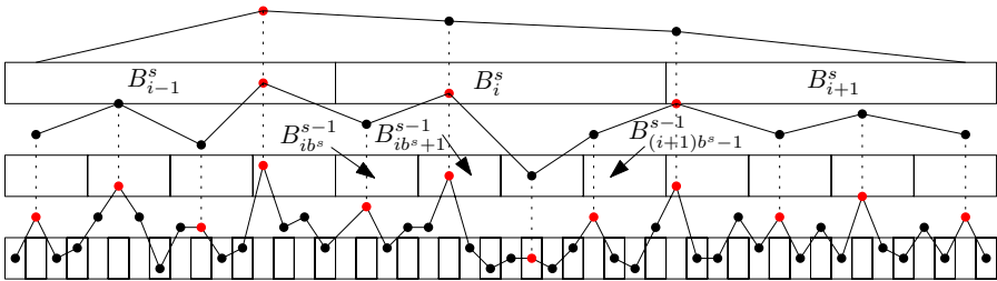
Fig. 1. Computing the approximate NNLN values for the maximum elements of the 3b sub-blocks of B_{i-1}^s , B_i^s and B_{i+1}^s
