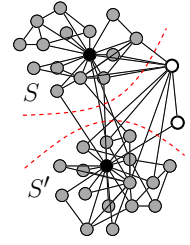
Fig. 2. Indecisive vertices (white)
