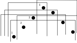
Fig. 4. A point set witnessing c(k) \geq 2k - 1 for k = 4
