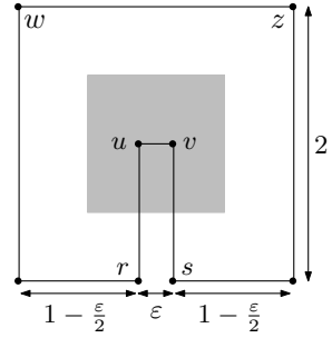
Fig. 1. Any triangulation of P with the \alpha -distance property requires many Steiner points
