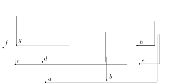
Fig. 1. The LEX ordering of a \perp -EPG representation: a < b < c < d < e < f < g < h
