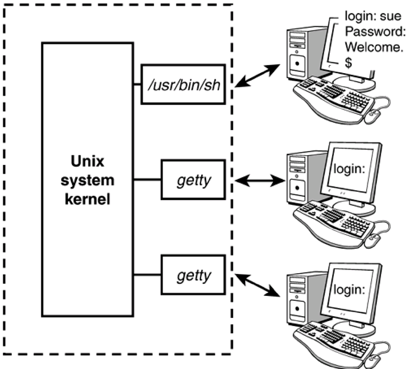
Figure 3.4. login executes /usr/bin/sh .
