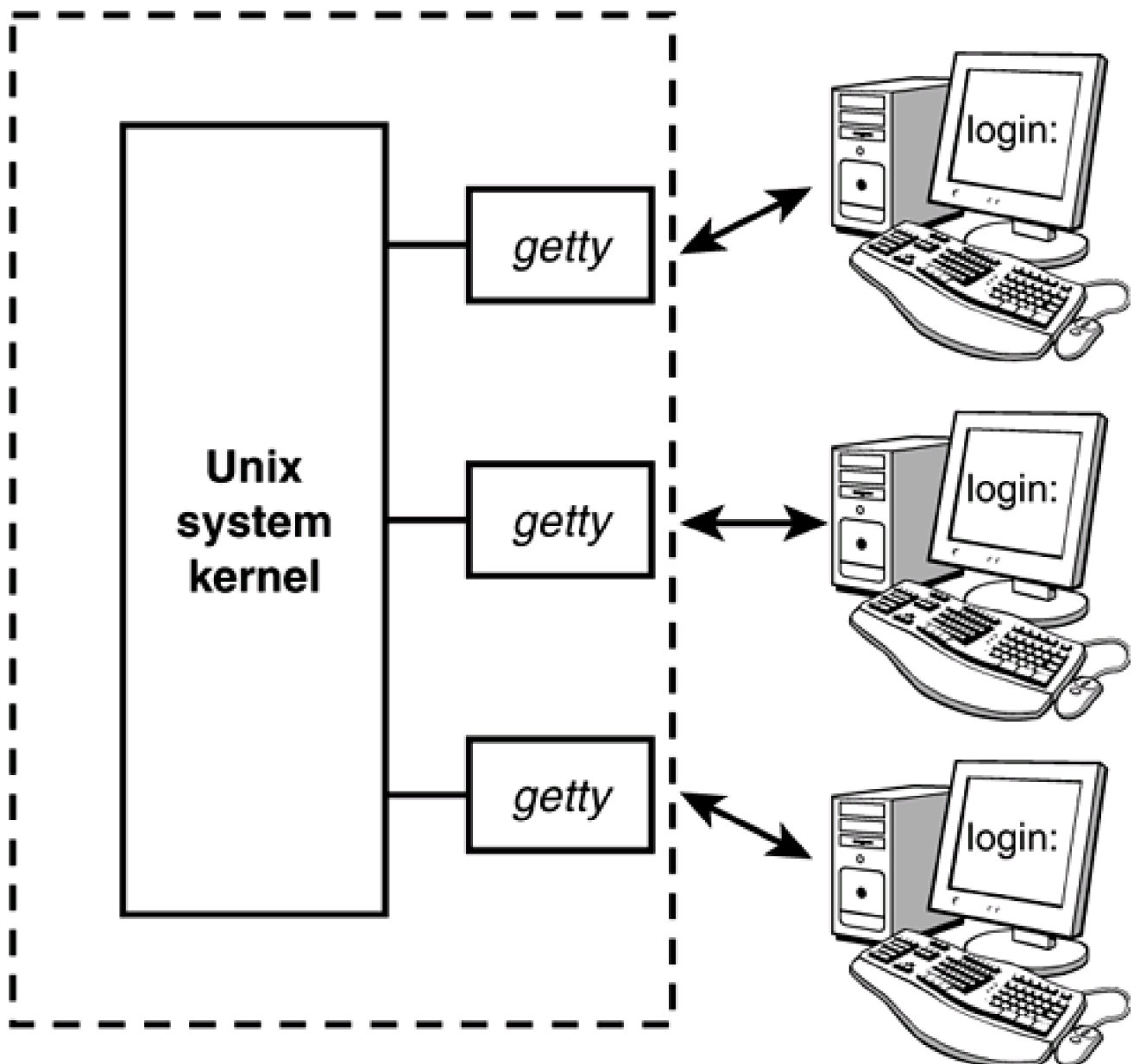
Figure 3.2. The getty process.
