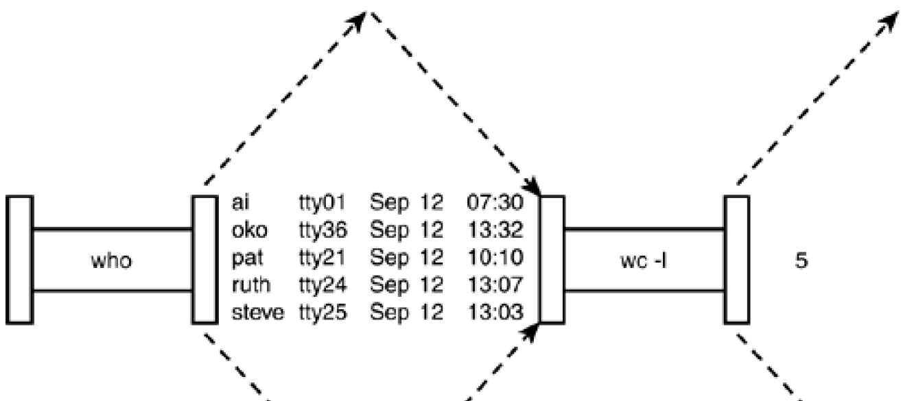
Figure 2.12. Pipeline process: who | wc -l .
