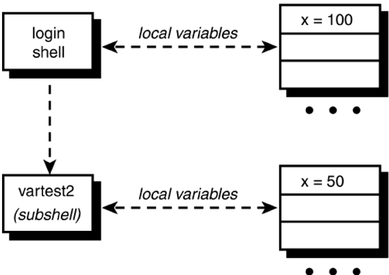
Figure 11.3. vartest2 executes x=50 .
