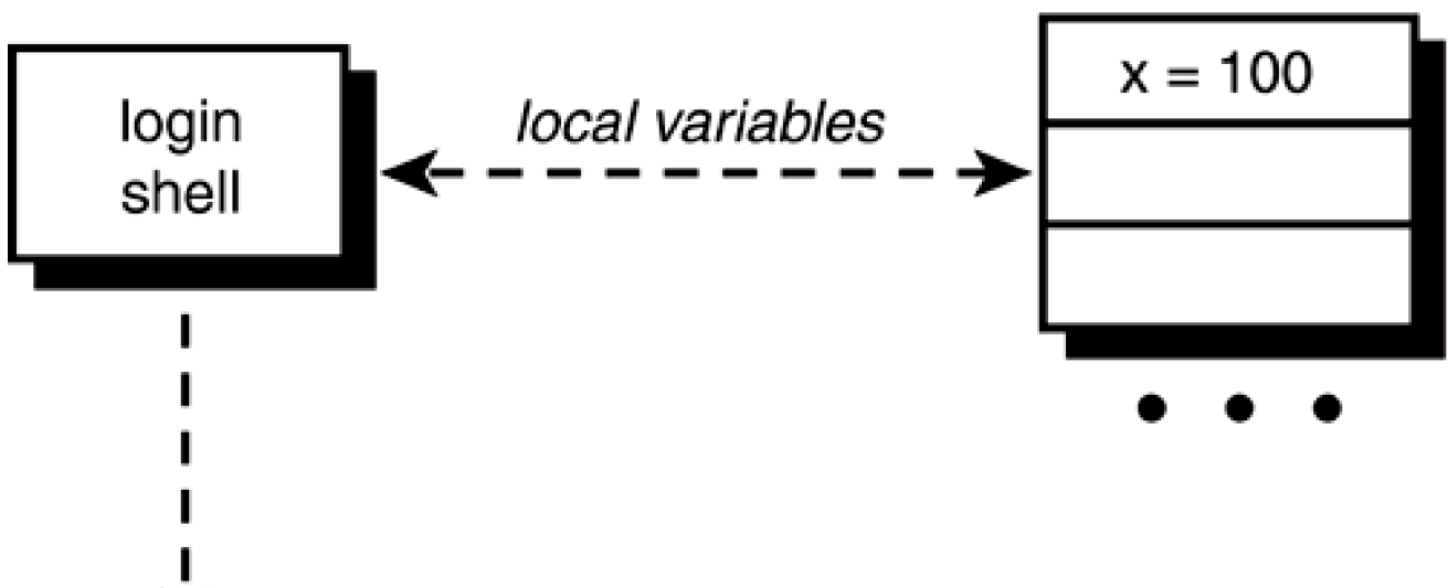
Figure 11.2. Login shell executes varTest2 .
