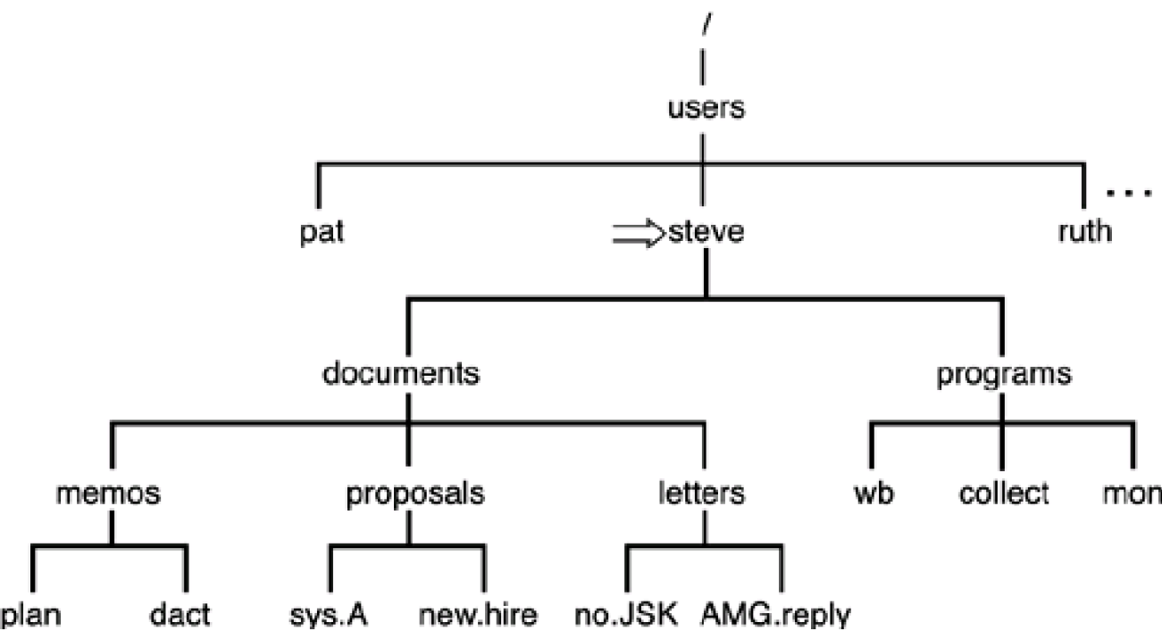
Figure 2.4. Current working directory is steve .
