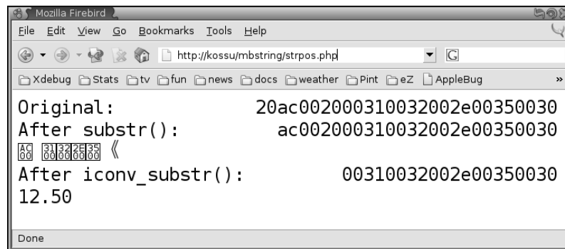
Fig. 9.17 Problems without iconv_strops() .
