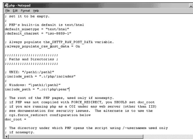
Fig. 10.2 Example php.ini modifications
