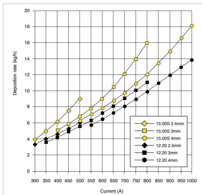
Deposition rate comparison OK Tubrod 15.00S and OK Autrod 12.20 / OK Flux 10.71.
