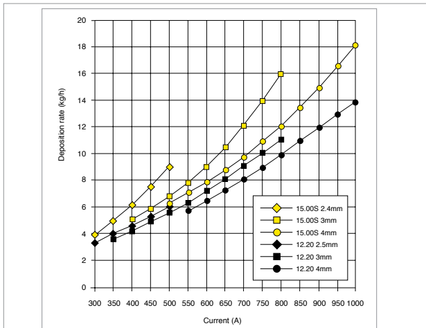
Deposition rate comparison OK Tubrod 15.00S and OK Autrod 12.20 / OK Flux 10.71.
