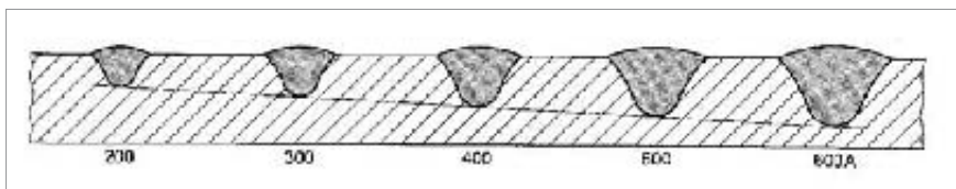
Effect of welding current on weld profile.
