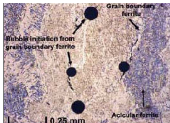
Hydrogen bubble initiation and propagation from \alpha grain boundary.
