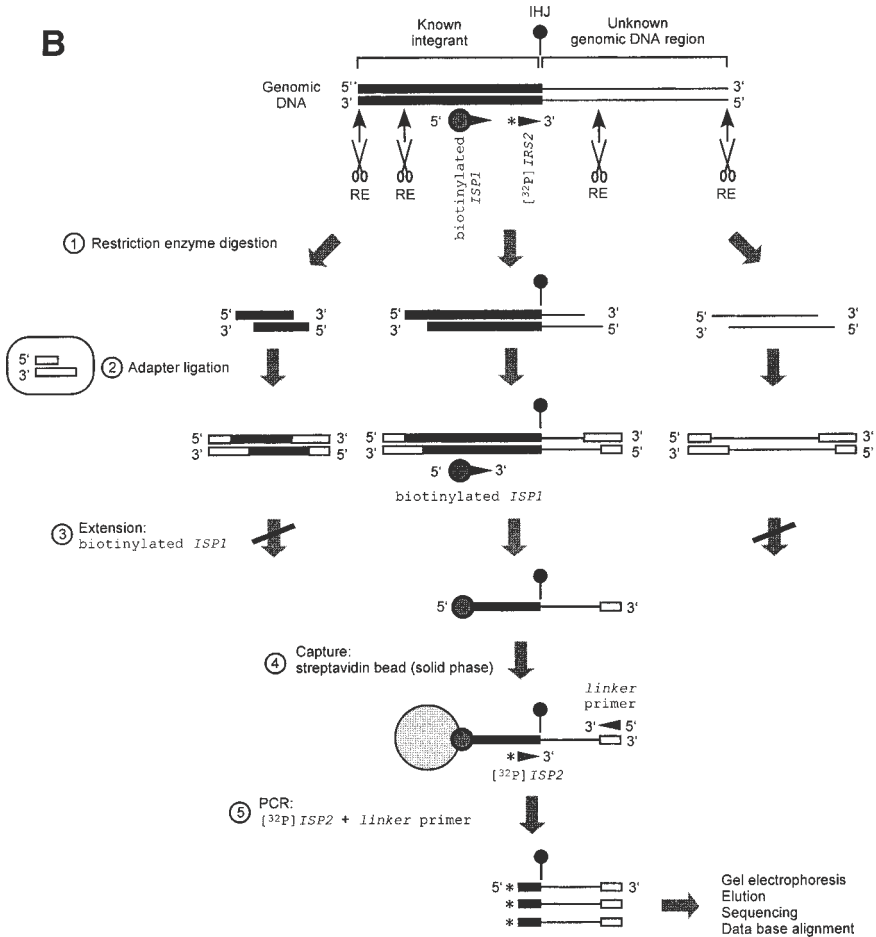
Fig. 7. Outline of application for the C-PCR into AP- or LA-PCR. Two complementary strands of DNA have been shown at the top. The heavy and thin line regions represent the integrant fragment and cellular genomic unknown sequence, respectively. The position of IHJ is indicated by closed circle or square. (A, facing page) Principle for C-PCR modification in AP-PCR. For detail manipulation see (92). (B) Principle for C-PCR modification in LA-PCR. For detail manipulations see (93).
