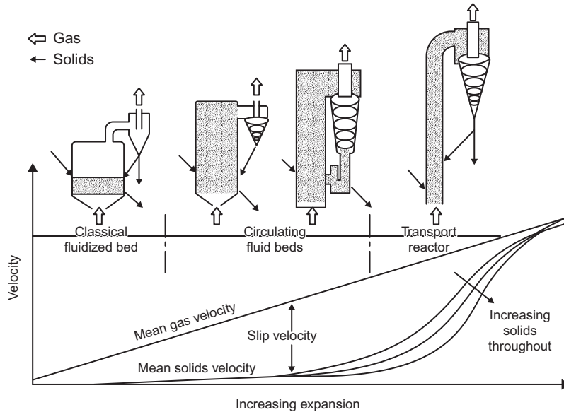
Figure 5.16 Velocity versus bed expansion. Source: Fig. 21-1, Page 690, CH21 FLUIDIZED BED COMBUSTION. Black & Veatch. Power Plant Engineering. CBS Publishers & Distributors. Chapman & Hall, Inc. New York 1996.
