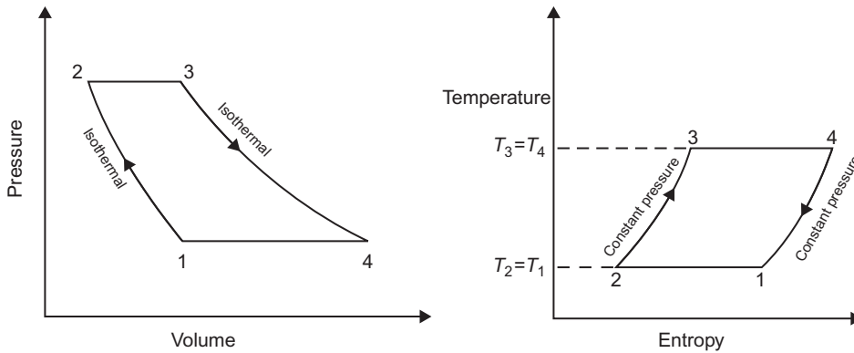
Figure 1.7 Ericsson cycle.
