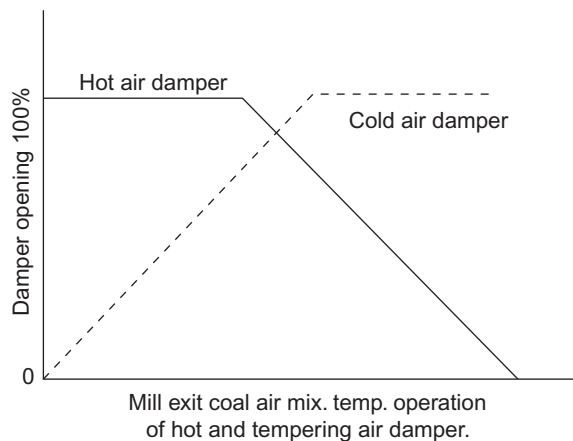
Figure 10.26 Hot air damper & cold air damper opening.
