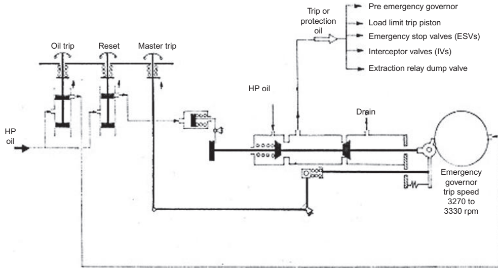
Figure 6.35 Emergency trip valve.
