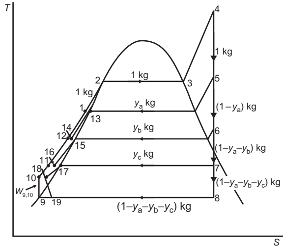
Figure 1.15 Triple extraction regenerative cycle.
