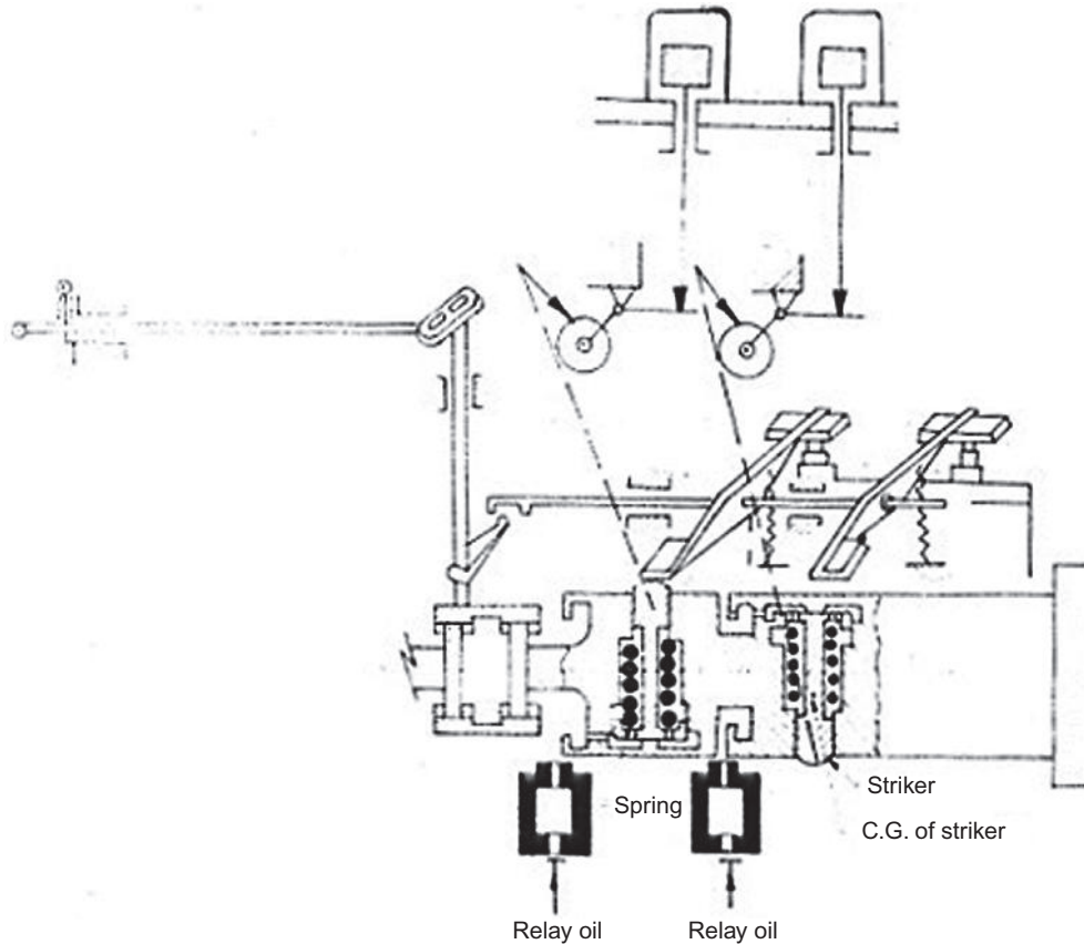
Figure 6.36 Overspeed governor.
