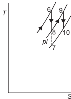
Figure 7.16 T-S diagram of turbine reheat. Source: Fig. 12.11, Page 241, Gas Power Cycles, [6].
