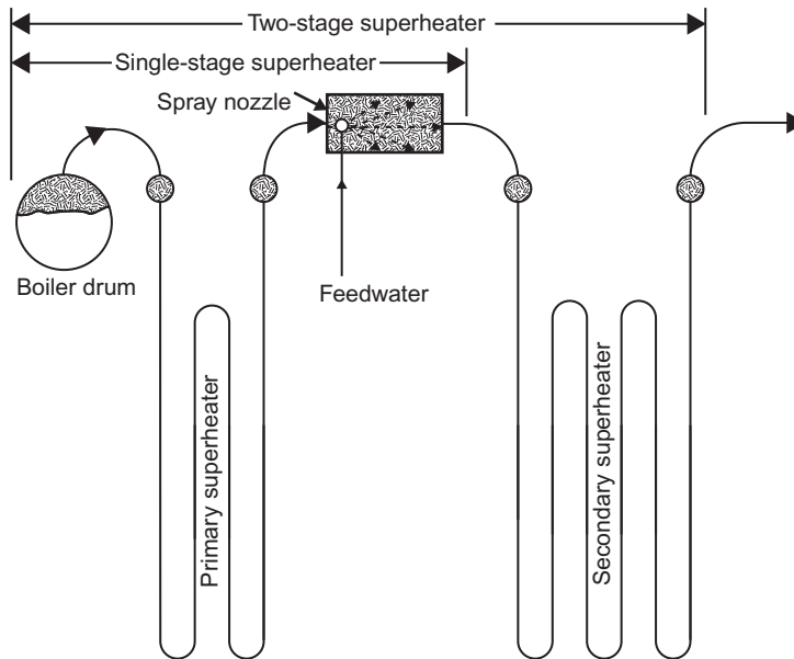
Figure 10.19 Direct contact type attemperer. Source: Fig. 16.29, P269. CH16: Superheaters, Reheaters and Attemperers [7].
