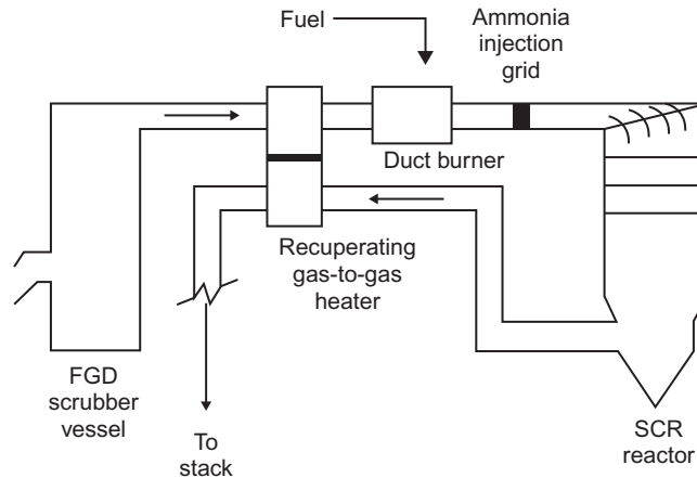
Figure 14.20 Location of SCR after FGD. Source: http://www.epa.gov/ttnecatc1/dir1/cs4-2ch2.pdf .
