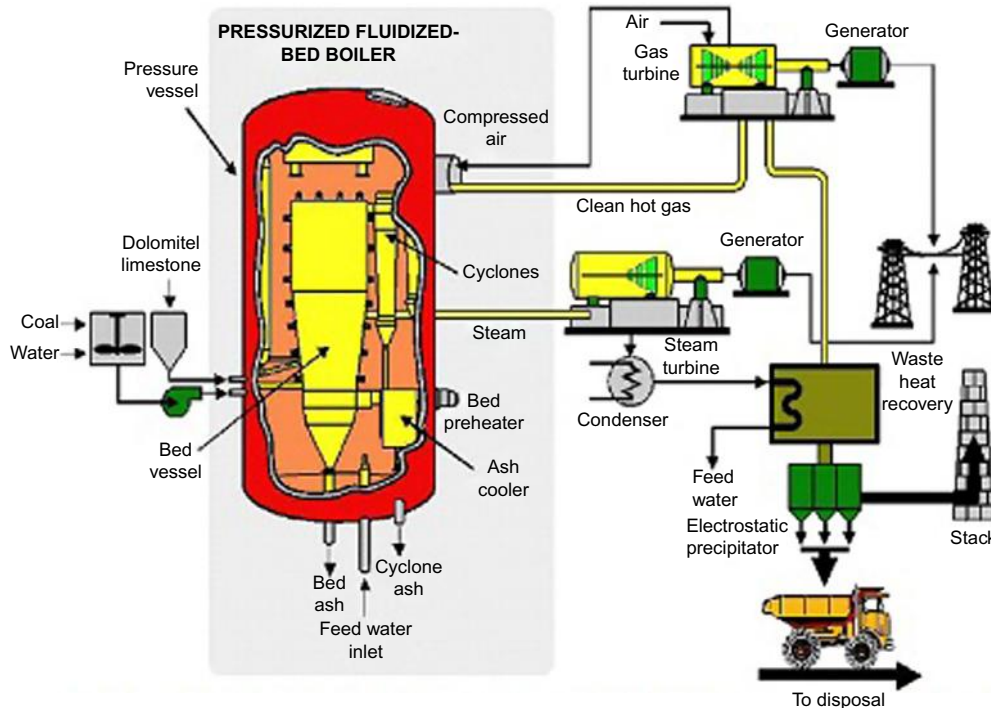
Figure 5.22 PFBC combustor with associated equipment. Source: http://dc222.4shared.com/doc/ckLfP5e/preview.html .
