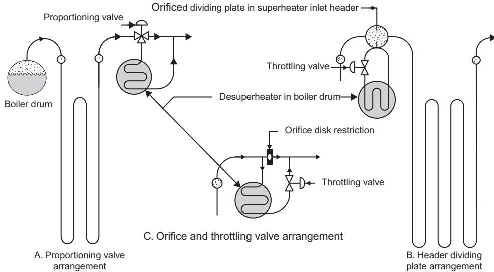
Figure 10.18 Submerged type attemperer. Source: Fig. 16.27, P268. CH16: Superheaters, Reheaters and Attemperers [7].
