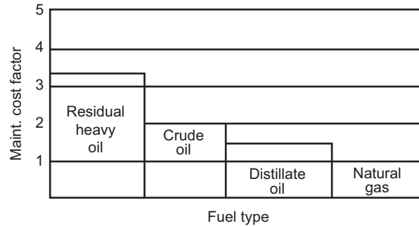
Figure 7.2 Effect of fuel on maintenance cost.
