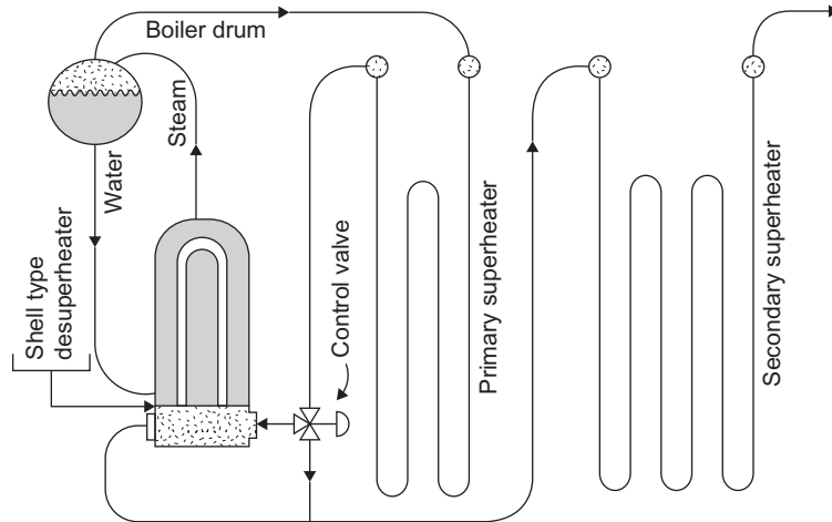
Figure 10.17 Shell and tube type attemperer. Source: Fig. 16.25, P267. CH16: Superheaters, Reheaters and Attemperators [7].
