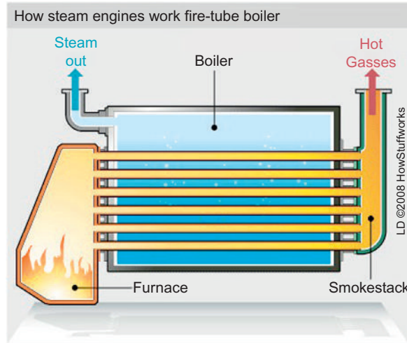
Figure 2.10 Fire-Tube Boiler. Source: http://science.howstuffworks.com/transport/engines-equipment/steam2.htm .
