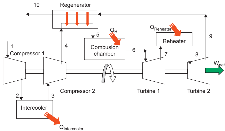
Figure 7.18 A gas turbine with intercooling, reheating & regeneration. Source: Figure 9, Page 9, Section 8.9-10 The Brayton Cycle With Regeneration, Intercooling And Reheating by Denise Lane.
