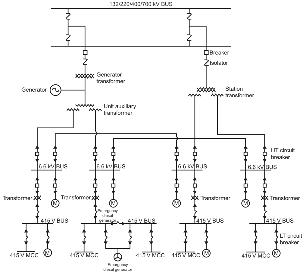
Figure 9.32 Typical electrical distribution system.
