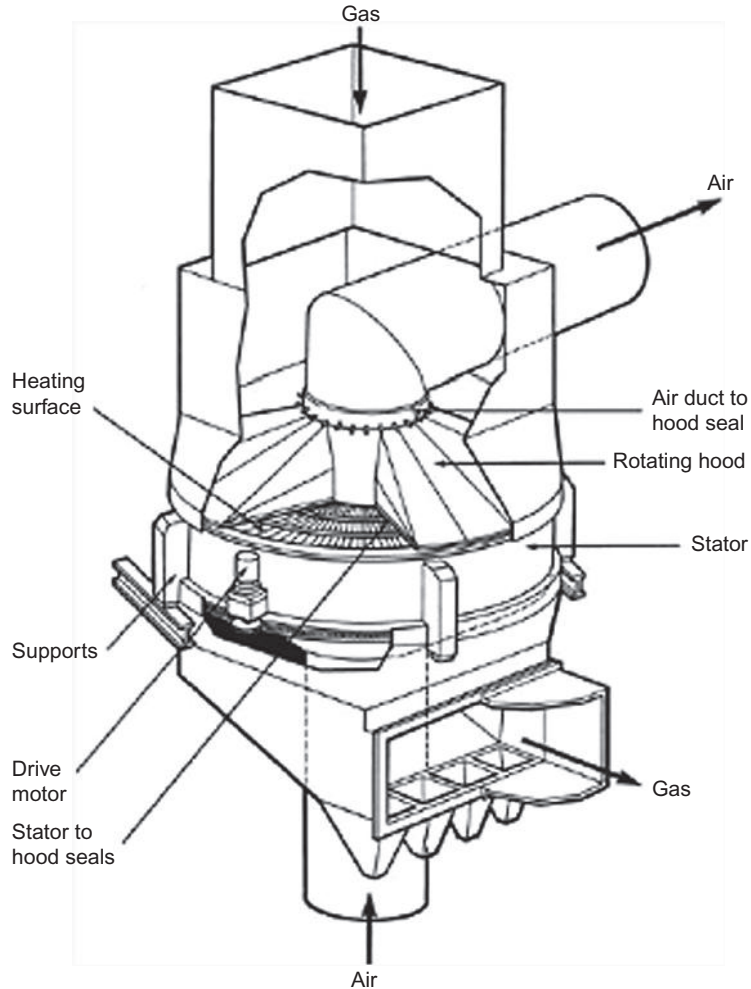
Figure 2.23 Rothemuhle air heater. Source: Fig. 20, Page 20-11, STEAM Its Generation and Use (41st Edition) . The Babcock and Wilcox Company.
