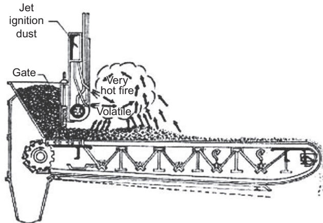
Figure 2.12 Chain-grate overfeed stoker. Source: P 9-18, SECTION 9, POWER GENERATION Editors, Theodore Baumeister and Lionel S. Marks. Mechanical Engineers' Handbook (6th Edition), 1958. McGraw-Hill Book Company, Inc.
