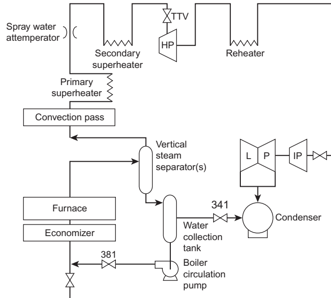
Figure 2.27 Separator drain circulation system of a supercritical boiler. Source: P17. Paper on STEAM GENERATORS USC AND A-USC STEAM CONDITIONS by Paul Weitzel, Niranjn Pawgi & Aaron Virgo at Partnership to Advance Clean Energy – Deployment. Babcock & Wilcox Company 2013. November 21–23, 2013. New Delhi. (US AID & Ministry of Power, Govt. of India).
