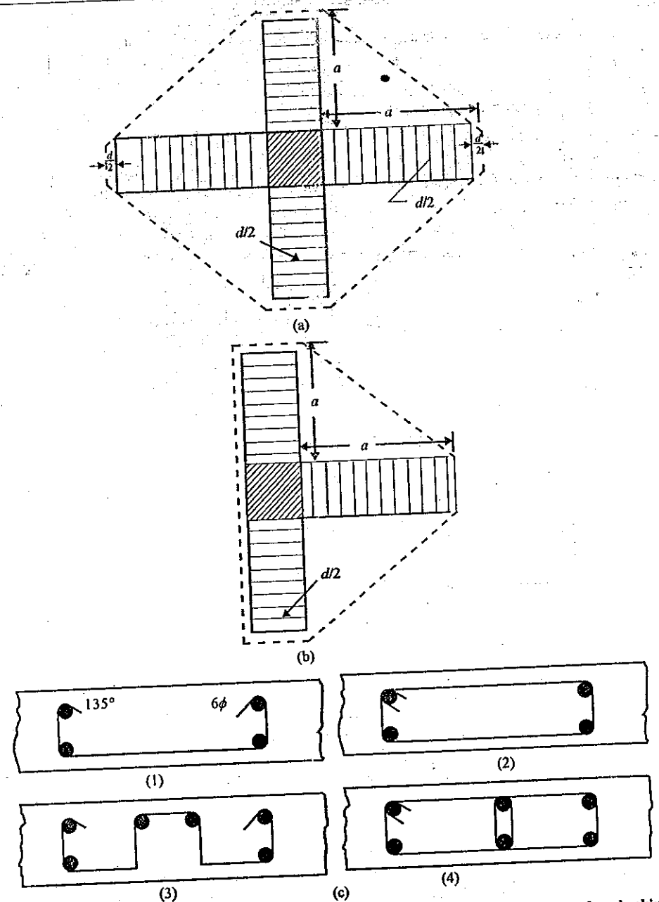
Fig. 12.7 Reinforcing flat slabs for shear by ACI method: (a) Critical perimeter for checking shear for internal columns; (b) critical perimeter for external columns; and (c) details of steel reinforcements.
