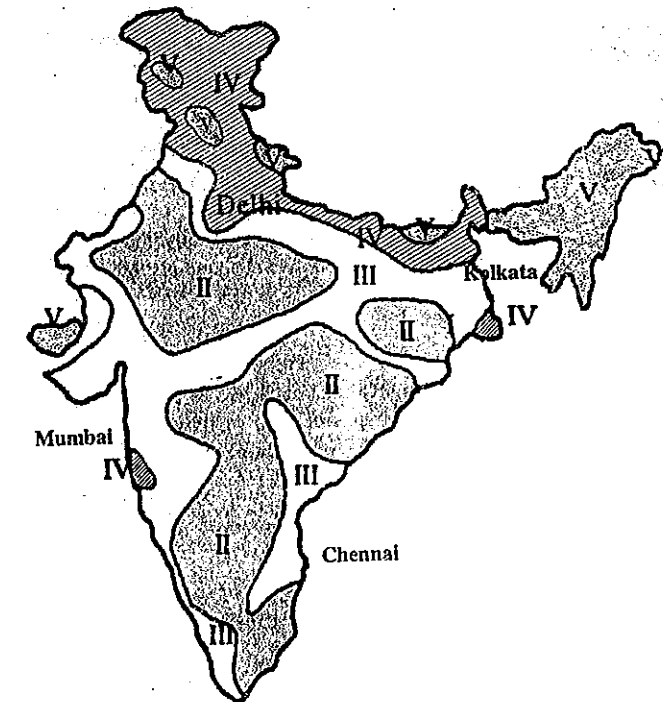
Fig. 18.1 Seismic zones in IS 1893 (2002) (Fifth revision).
