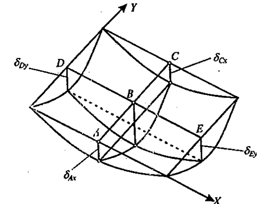
Fig. 1.3 Deflection of slabs: \delta_{Bx} and \delta_{By} are deflections of middle strips in X and Y directions, respectively.
