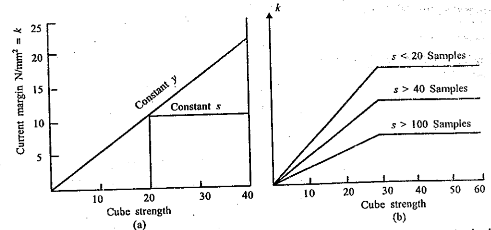
Fig. 25.5 Influence of assumptions on current margin: (a) Effect of assuming constant standard s and constant coefficient variation v ; (b) effect of number of samples on standard deviation.
