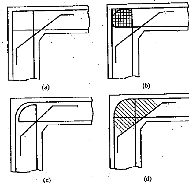
Fig. 20.10 Detailing of knee joints: (a) 90° opening corners of members with percentage of steel \leq 1 : splay steel to be 50% of main steel; (b) joints under alternating loads; (c) alternative to (a); and (d) members with more than 1% steel (SP 34 page 110).
