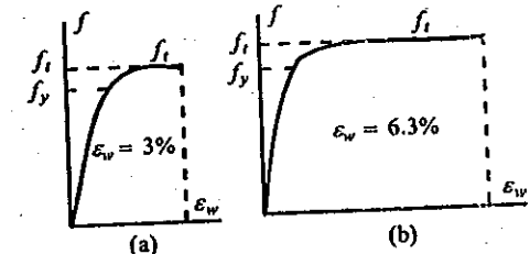
Fig. 22.5 Classes of steel: (a) Class N steel; and (b) class H steel.
