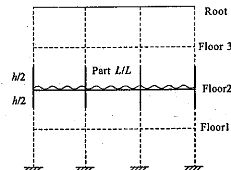
Fig. 18.2 Seismic load on second floor.
