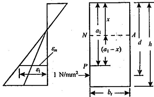
Fig. 2.4 Estimation of E_m for point P of a beam section.
