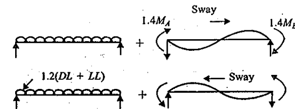
Fig. 21.2 Calculation of design shear for beams.
