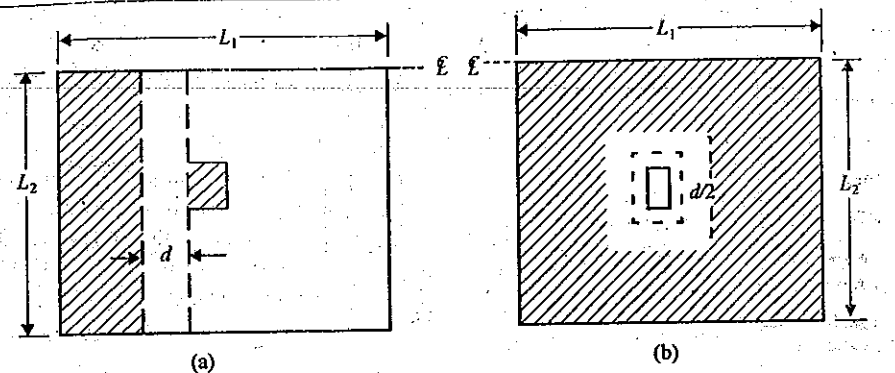
Fig. 12.1 Design shears at an interior column support in flat slabs: (a) One-way shear or beam shear; and (b) punching shear or two-way shear.
