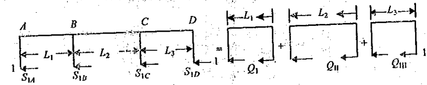
Fig. 9.2 Column shears by portal method.
