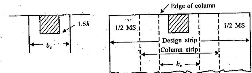
Fig. 11.8(a) Breadth of effective moment transfer strip involved in transfer of unbalanced moment [ACI 318].
