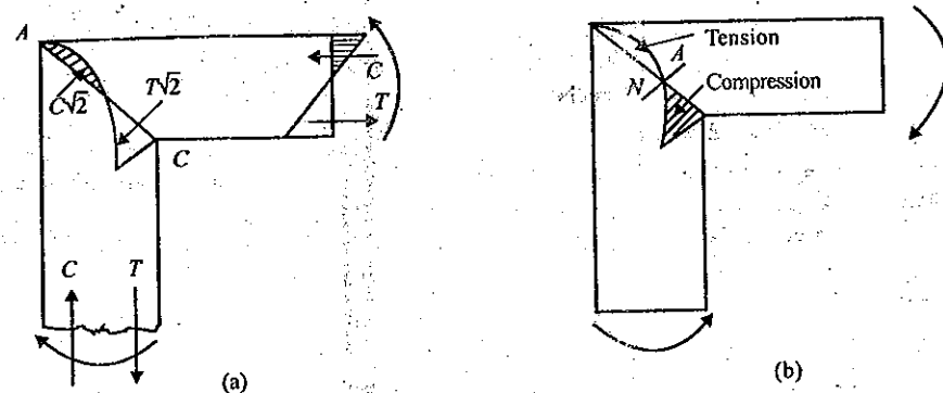
Fig. 20.9 Distribution of stresses along the corner diagonal in opening and closing joints; and (a) opening joint; and (b) closing joint.
