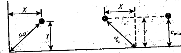
Fig. 2.1 Factors affecting crackwidth in beams.
