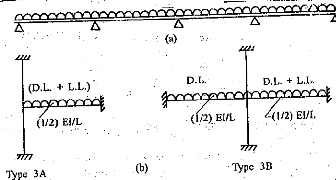
Fig. 8.5 Analysis allowed for beams and columns in BS:8110: (a) 'Continuous beam simplification' for beams; and (b) sub-frames for columns.
