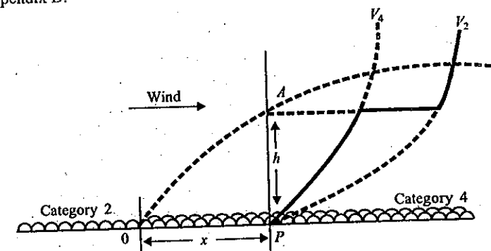
Fig. 7.2 Velocity change with height: Change of terrain from less rough to more rough ( V_2 is height-velocity profile for terrain category 2 and V_4 that for the category 4. Curve OA is the fetch developed height relationship for category 4 at point P ).
