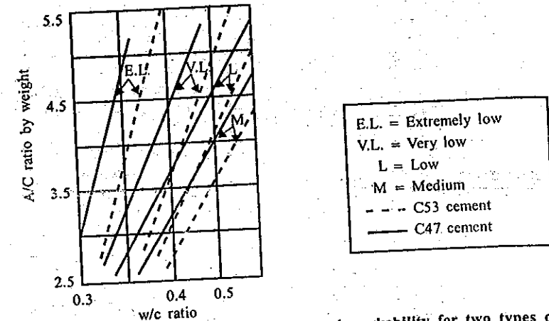
Fig. 24.5 Typical relation between aggregate-cement ratio and workability for two types of cement using 20 mm granite and gravel aggregates, refer [10].
