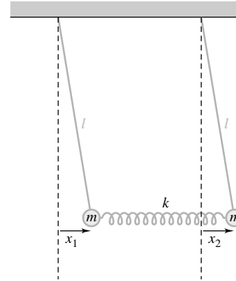
Figure 36 Coupled pendulums
