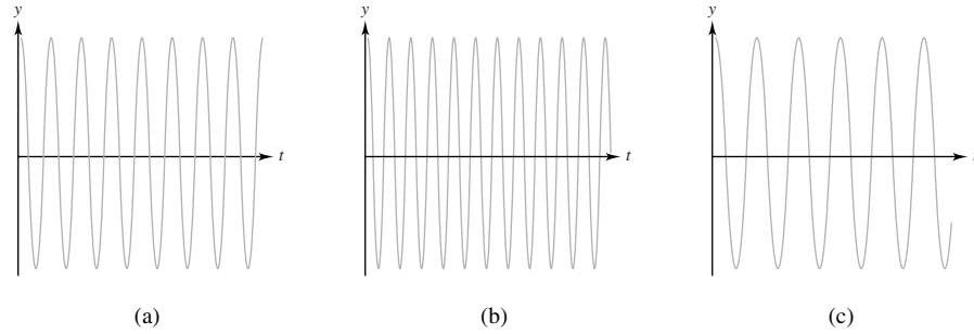
Figure 2 (a) Sinusoidal oscillation, (b) stiffer spring, and (c) heavier mass
