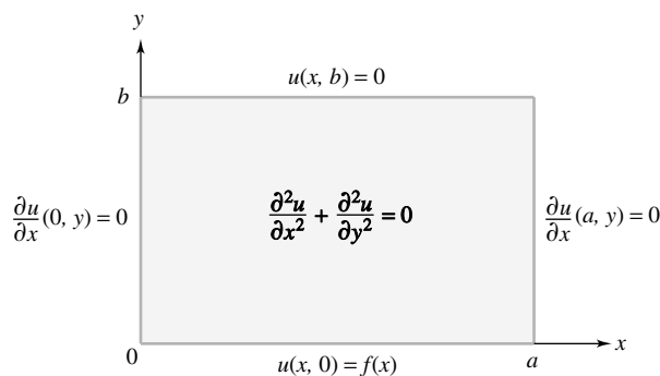
Figure 25 Mixed boundary value problem
