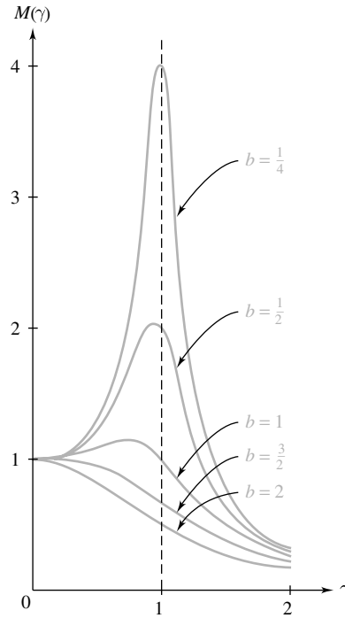
Figure 33 Frequency response curves for various values of b
