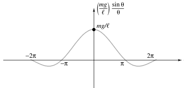
Figure 19 Pendulum “stiffness”
