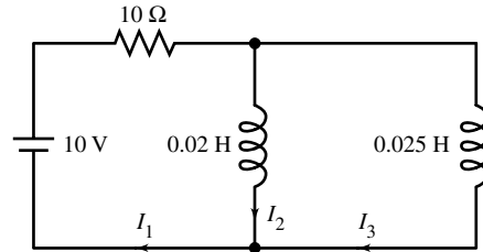
Figure 41 RL network for Problem 12
