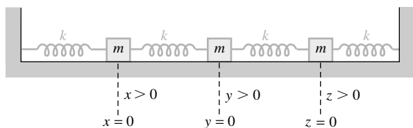
Figure 32 Coupled mass-spring system with three degrees of freedom
