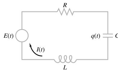
Figure 9 RLC series circuit
