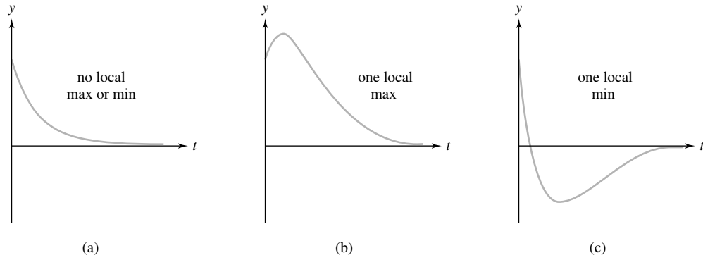
Figure 29 Overdamped vibrations
