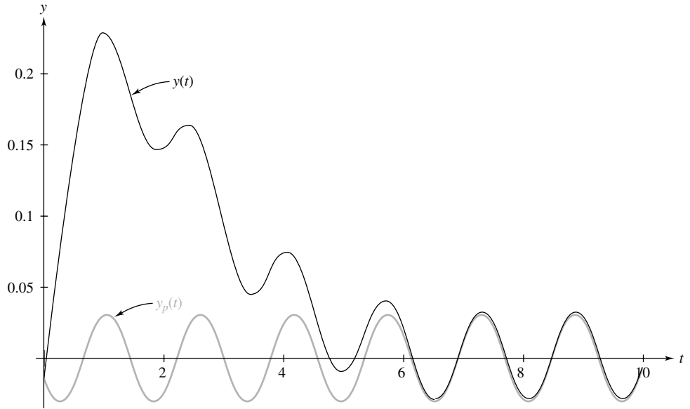
Figure 32 Convergence of y(t) to the steady-state solution y_p(t) when m = 4 , b = 6 , k = 3 , F_0 = 2 , \gamma = 4
