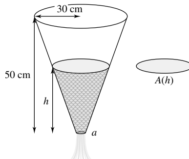
Figure 14 Conical tank
