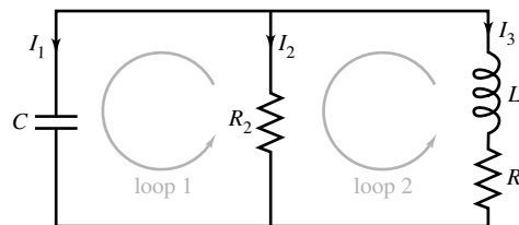
Figure 52 Electrical circuit for Problem 17
