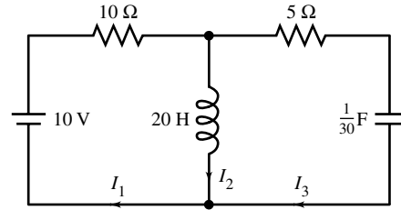
Figure 40 RLC network for Problem 11
