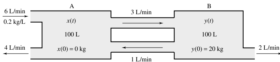
Figure 2 Mixing problem for interconnected tanks
