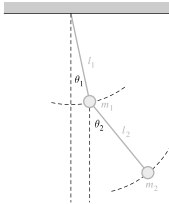
Figure 35 Double pendulum
