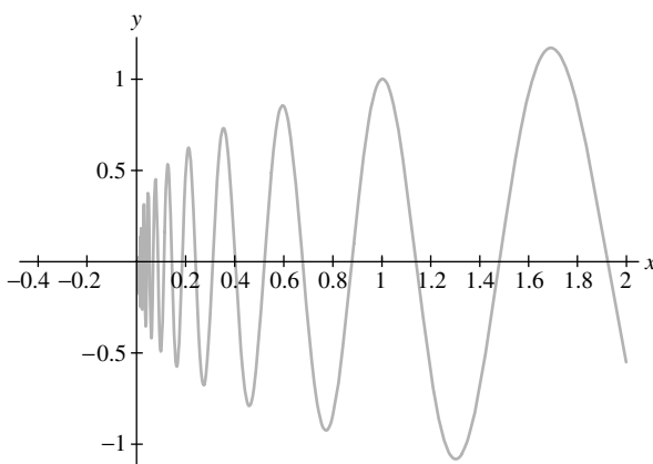
Figure 7 Graph of x^{0.3}\cos(12 \ln x)
