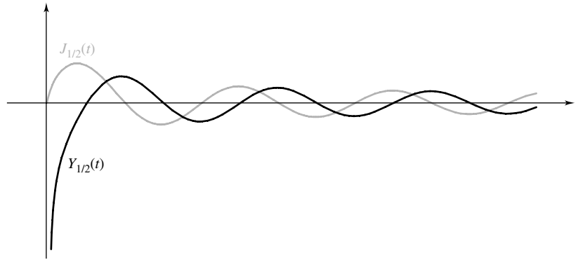
Figure 14 Bessel functions
