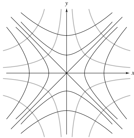
Figure 11 Families of orthogonal hyperbolas
