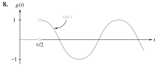
Figure 17 Function in Problem 8
