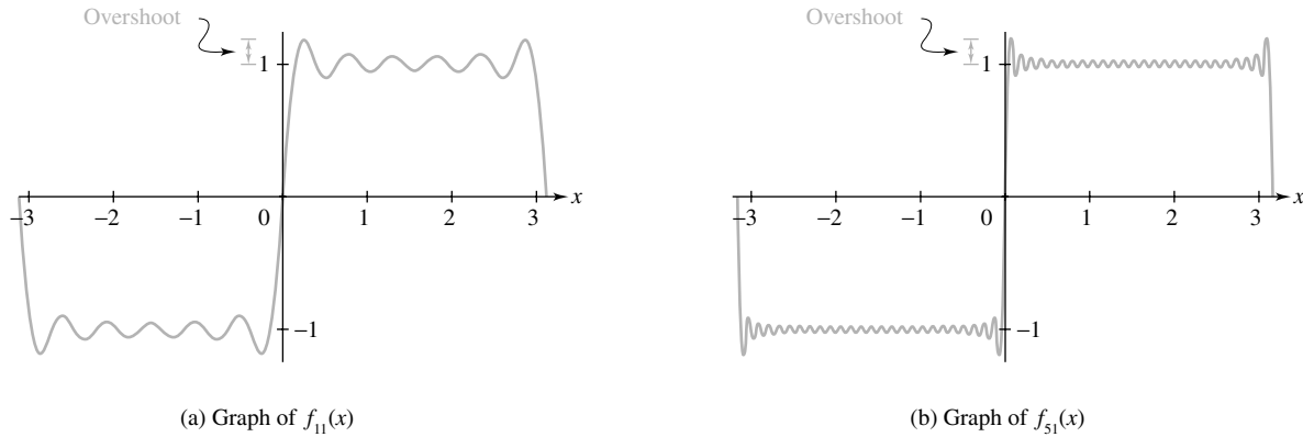
Figure 12 Gibbs phenomenon for partial sums of Fourier series
