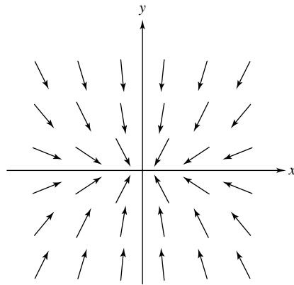
Figure 9 Direction field for Example 1
