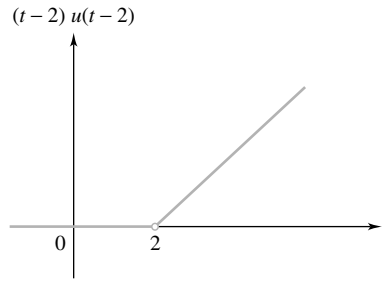
Figure 12 Graph of solution to Example 4
