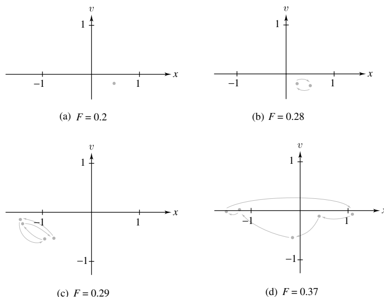
Figure 46 Poincaré sections for the Duffing equation (7) with b = 0.3 and \gamma = 1.2
