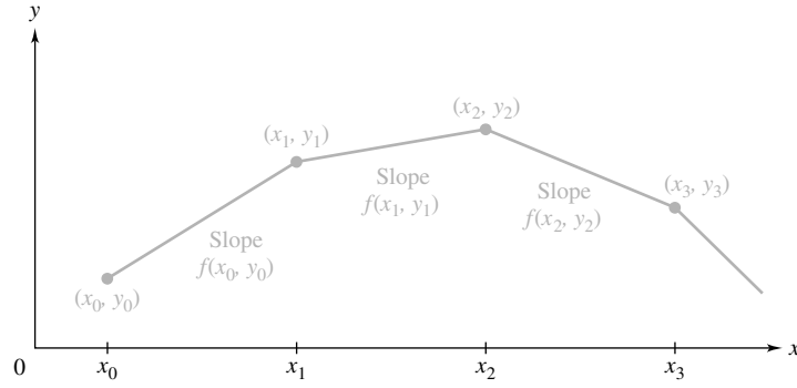
Figure 15 Polygonal-line approximation given by Euler's method
