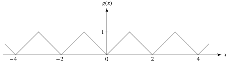
Figure 11 Periodic extension of f(x) = |x| , -1 < x < 1
