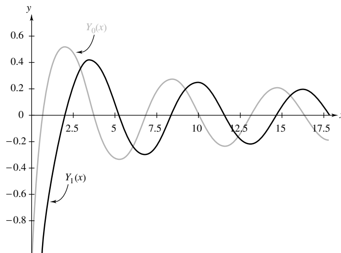
Figure 15 Graphs of the Bessel functions Y_0(x) and Y_1(x)
