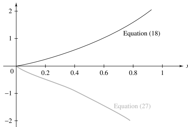
Figure 10 Partial sum approximations to solutions of Example 2
