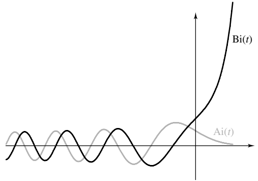
Figure 13 Airy functions
