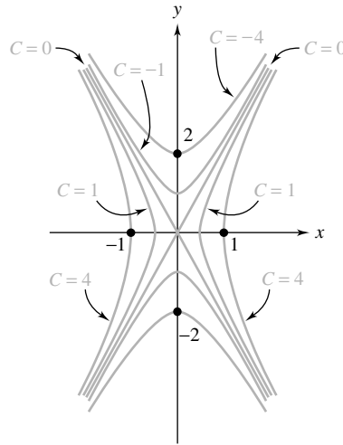
Figure 4 Implicit solutions 4x^2 - y^2 = C
