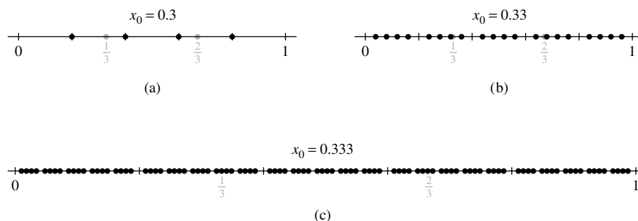
Figure 50 Plots of the map x_{n+1} = 2x_n \pmod{1} for x_0 = 0.3, 0.33 , and 0.333
