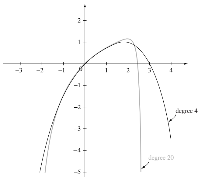
Figure 8 Partial sums approximating the solution y_1(x) of Example 3
