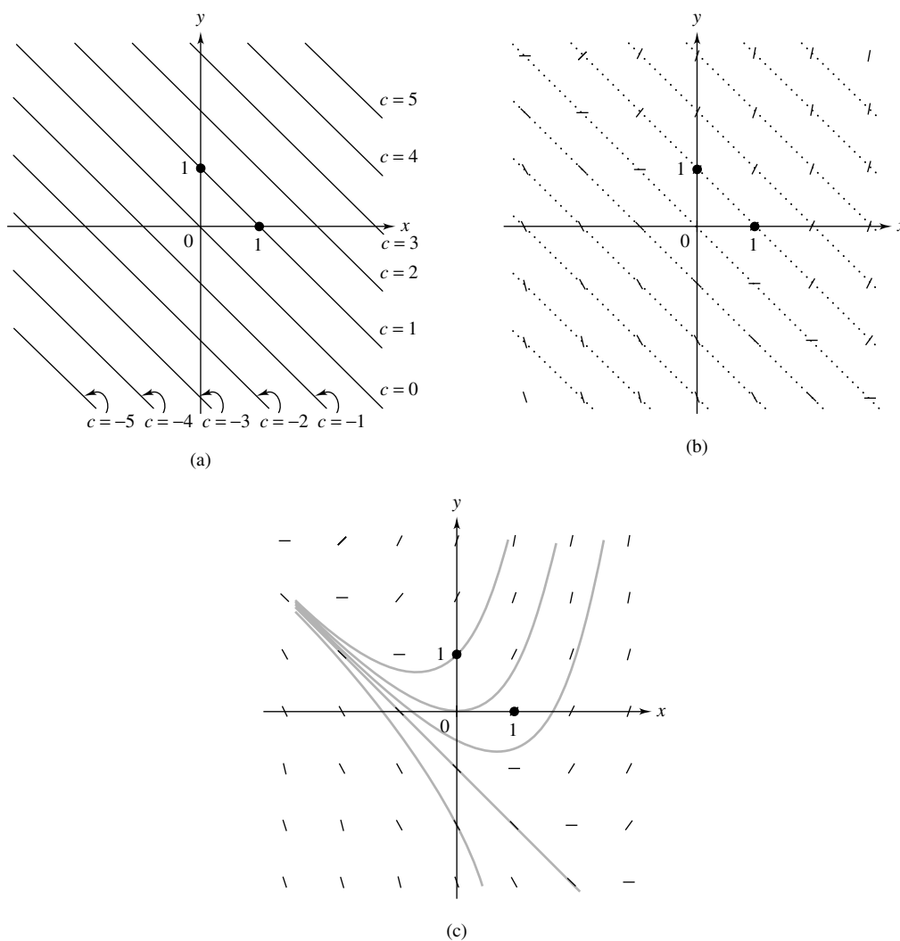
Figure 11 (a) Isoclines for y' = x + y (b) Direction field for y' = x + y (c) Solutions to y' = x + y
