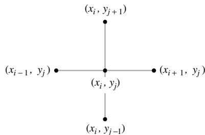
Figure 33 Approximate solution u_{i,j} at (x_i, y_j) is obtained from values at the ends of the cross
