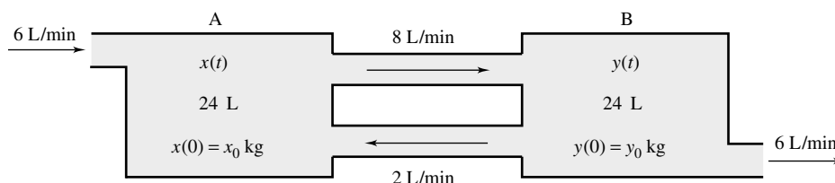
Figure 1 Interconnected fluid tanks
