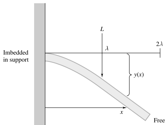
Figure 29 Beam imbedded in a support under a concentrated load at x = \lambda
