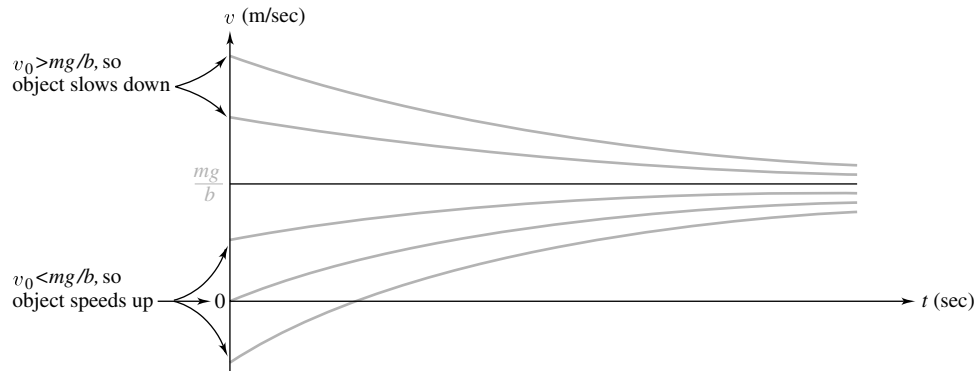
Figure 2 Graph of v(t) for six different initial velocities v_0 . ( g = 9.8 \text{ m/sec}^2 , m/b = 5 \text{ sec} )
