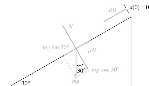
Figure 11 Forces on an object on an inclined plane
