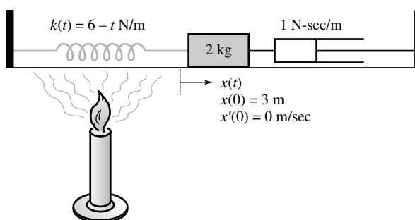
Figure 6 A mass-spring system whose spring is being heated
