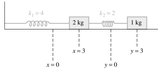
Figure 27 Coupled system at initial displacement
