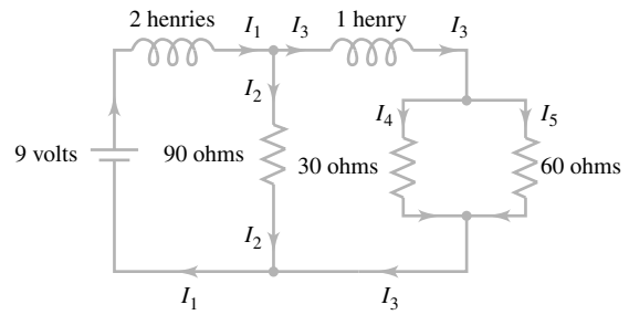
Figure 8 RL network for Problem 33
