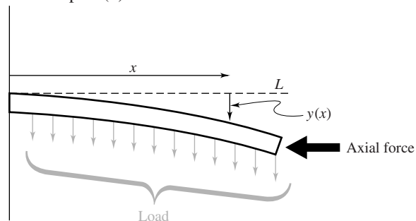
Figure 2 Deformation of a beam under axial force and load
