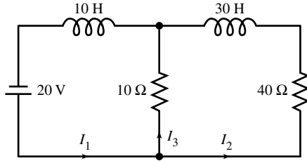
Figure 39 RL network for Problem 10
