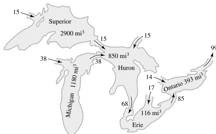
Figure 55 Compartmental model of the Great Lakes with flow rates ( \text{mi}^3/\text{yr} ) and volumes ( \text{mi}^3 )
