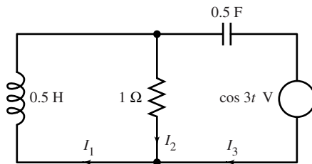
Figure 42 RLC network for Problem 13
