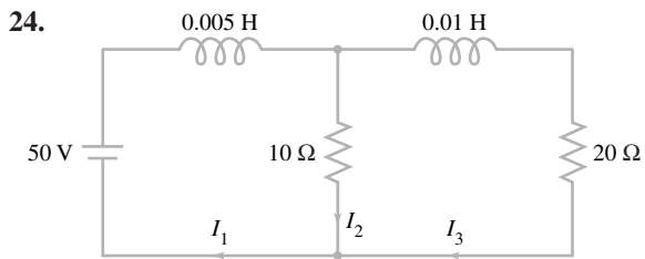
Figure 31 RL network for Problem 24
