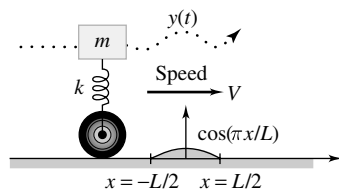
Figure 11 Speed bump
