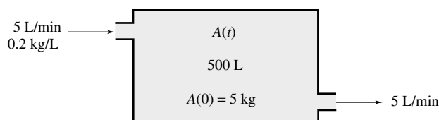
Figure 6 Mixing problem with equal flow rates
