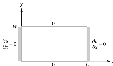
Figure 17 Plate with insulated sides
