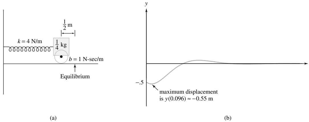
Figure 31 Mass-spring system and graph of motion for Example 3
