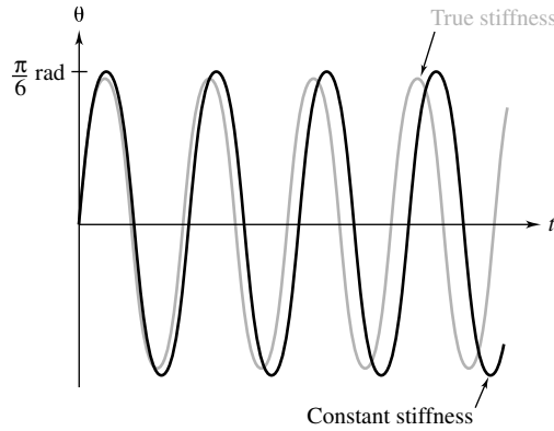
Figure 20 Small-amplitude pendulum motion
