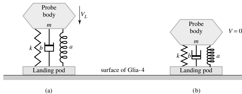
Figure 53 Schematic of the probe landing system. (a) The system at the instant of impact. The springs are not stretched or compressed, the thrusters have been turned off, and the velocity is V_L downward. (b) The probe has reached a state of rest on the surface, and the springs are compressed enough to support the weight. Between states (a) and (b), the probe oscillates relative to the landing pod.
