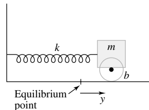
Figure 1 Damped mass–spring oscillator
