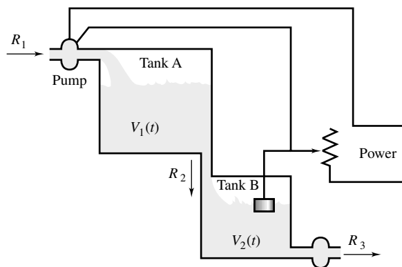
Figure 3 Feedback system with pooling delay
