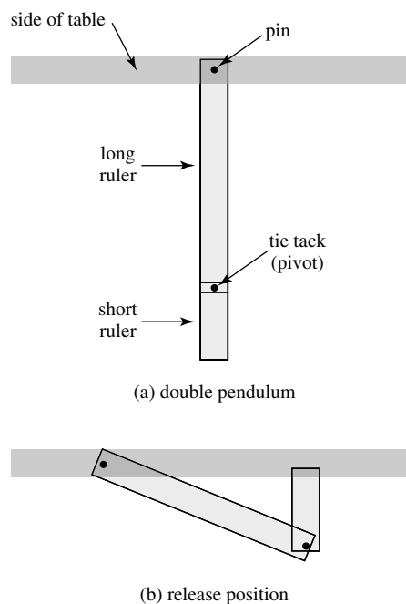
Figure 51 Double pendulum as a chaos machine
