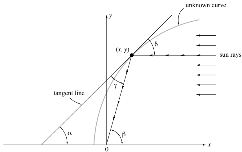
Figure 16 Curve that generates a solar collector
