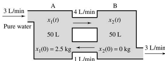
Figure 2 Mixing problem for interconnected tanks
