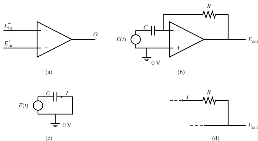
Figure 20 Op amp differentiator
