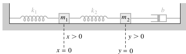
Figure 33 Coupled mass-spring system with one end damped
