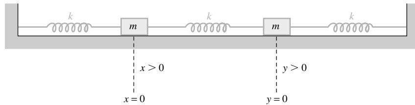
Figure 29 Coupled mass–spring system with fixed ends
