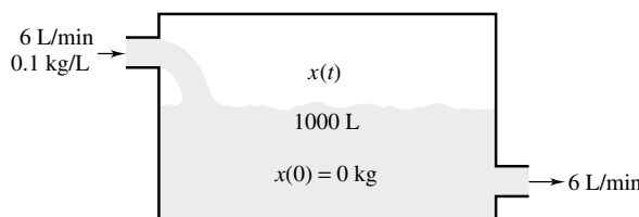
Figure 2 Mixing problem with equal flow rates
