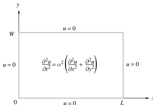
Figure 20 Vibrating membrane
