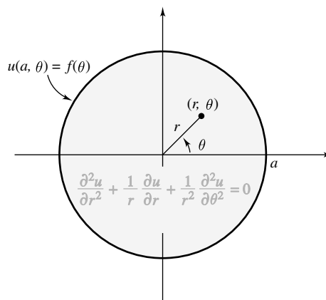
Figure 27 Steady-state temperature distribution in a disk
