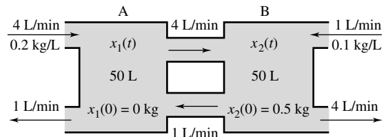
Figure 9 Mixing problem for interconnected tanks
