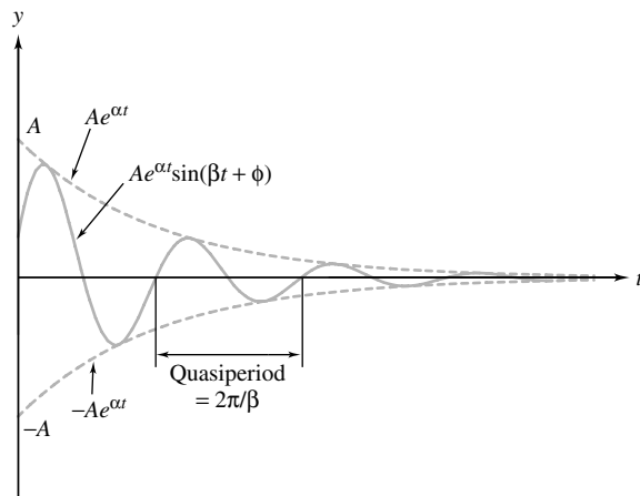
Figure 28 Damped oscillatory motion
