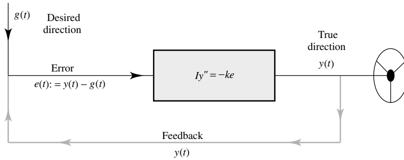
Figure 6 Servomechanism with feedback
