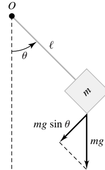
Figure 18 A pendulum
