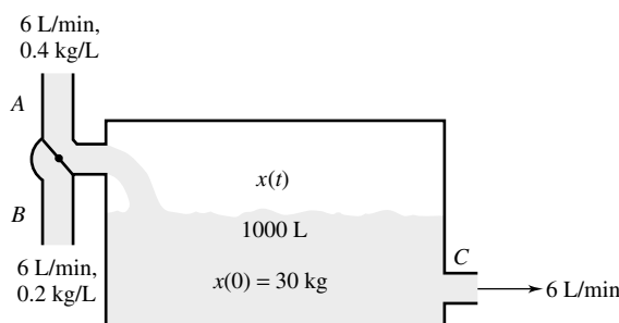
Figure 1 Mixing tank with valve A open
