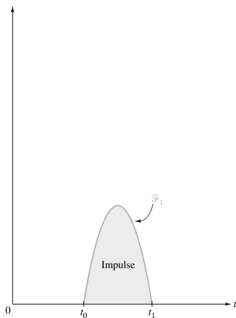
Figure 26 Force due to a blow from a hammer
