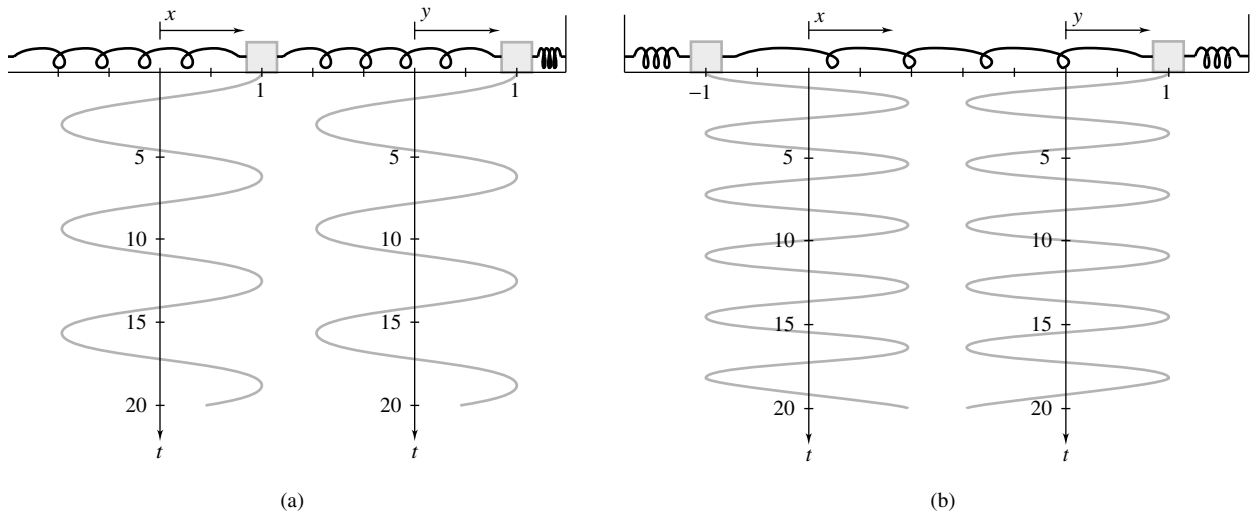
Figure 30 Normal modes for Example 2
