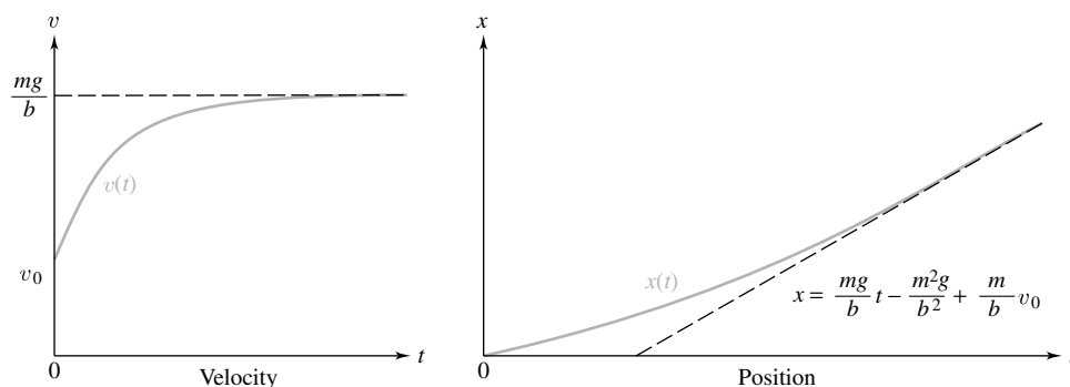
Figure 8 Graphs of the position and velocity of a falling object when v_0 < mg/b
