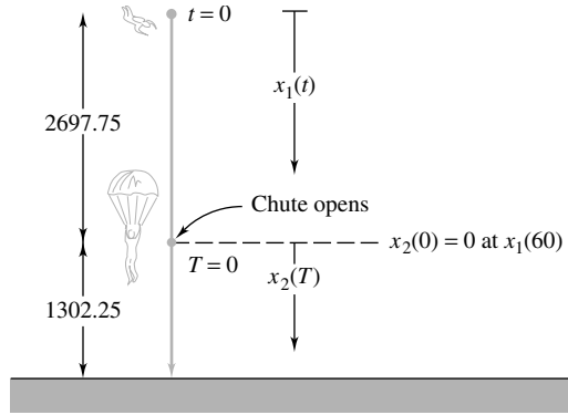
Figure 9 The fall of the parachutist
