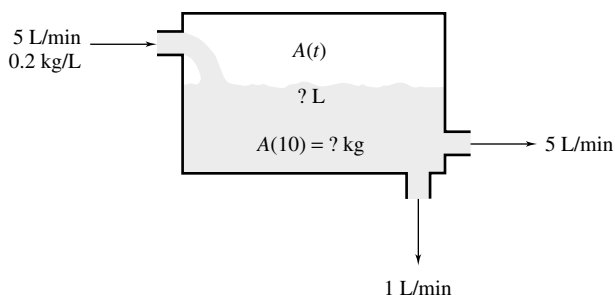
Figure 7 Mixing problem with unequal flow rates
