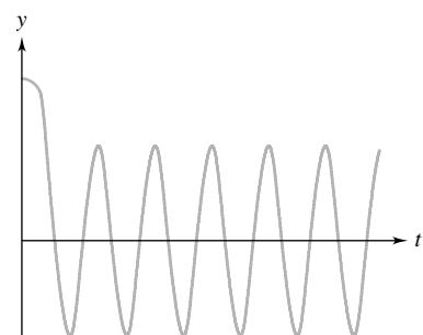
Figure 25 Solution to the Rayleigh equation
