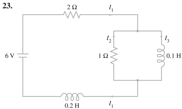
Figure 30 RL network for Problem 23
