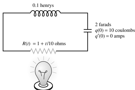
Figure 5 An RLC circuit whose resistor is being heated
