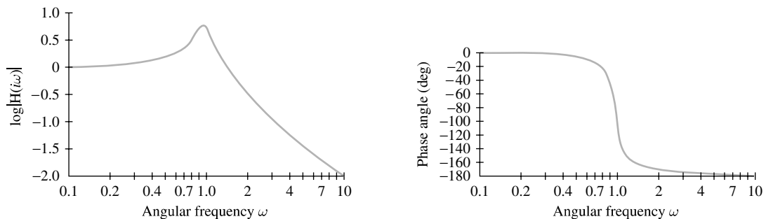
Figure 33 Bode plots for H(i\omega) = [1 + 0.2(i\omega) + (i\omega)^2]^{-1}
