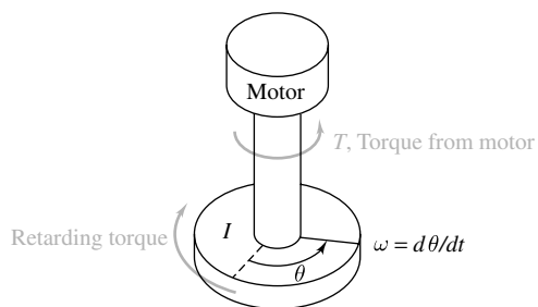
Figure 10 Motor-driven flywheel
