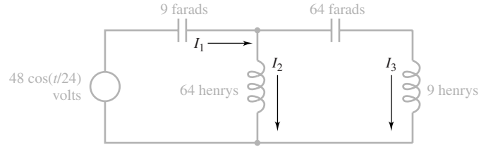
Figure 1 An electrical network
