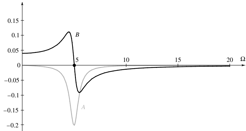
Figure 5 Vibration amplitudes around resonance
