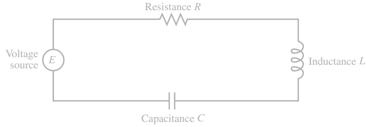
Figure 37 Schematic representation of an RLC series circuit
