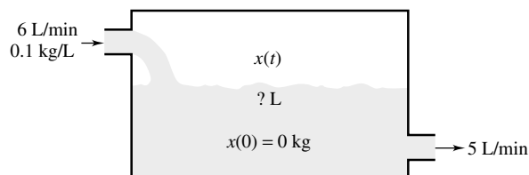
Figure 3 Mixing problem with unequal flow rates
