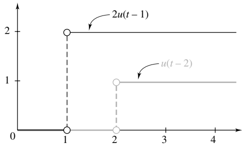
Figure 8 Two-step functions expressed using the unit step function
