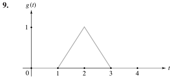
Figure 18 Function in Problem 9
