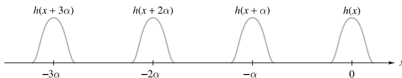
Figure 22 Traveling wave
