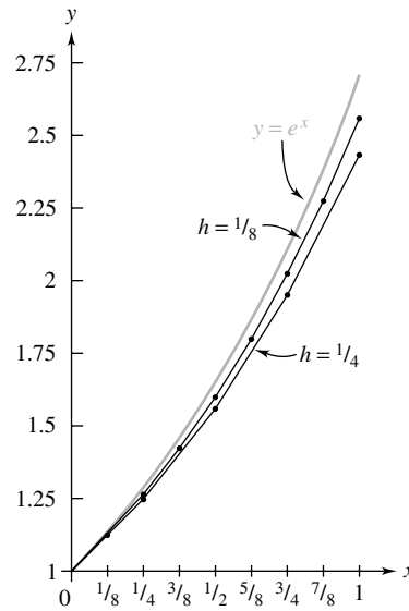
Figure 16 Approximations of e^x using Euler's method with h = 1/4 and 1/8
