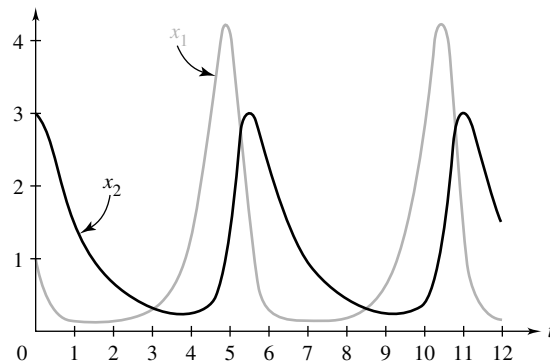
Figure 6 Graphs of the components of an approximate solution to the Volterra–Lotka system (17)
