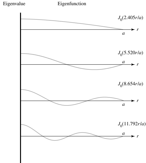
Figure 31 Bessel eigenfunctions
