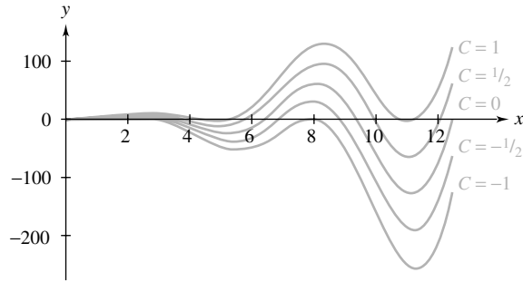
Figure 5 Graph of y = x^2 \sin x + Cx^2 for five values of the constant C
