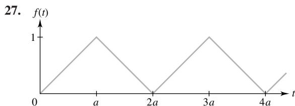
Figure 22 Triangular wave
