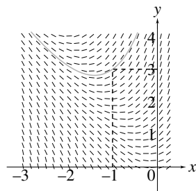
Figure 2 The solution curve in Problem 1(b).
