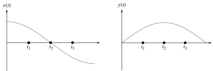
Figure 7 Solution pair for system (1)
