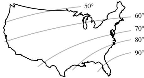
Figure 8 Level curves of F(x, y)
