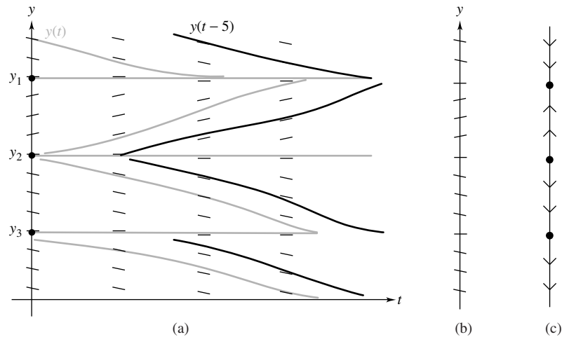
Figure 17 Direction field and solutions for an autonomous equation
