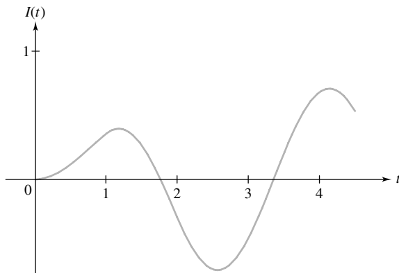
Figure 13 Solution to Example 5
