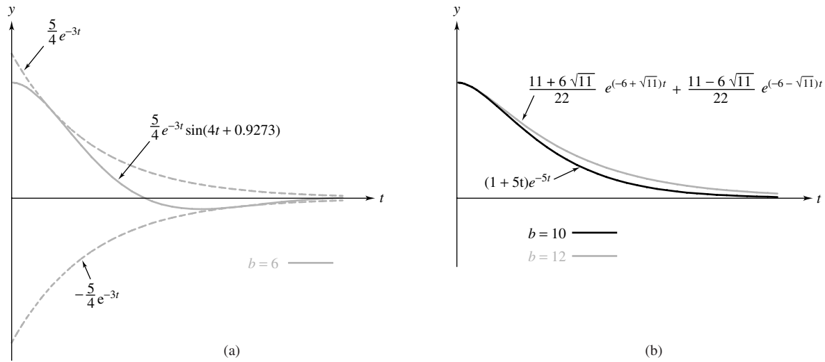
Figure 30 Solutions for various values of b
