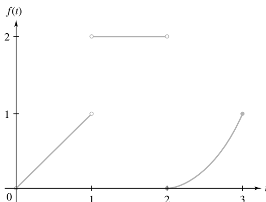
Figure 4 Graph of f(t) in Example 6
