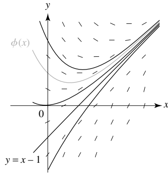
Figure 6 Direction field and sketch of \phi(x) for Problems 9 (f, g)
