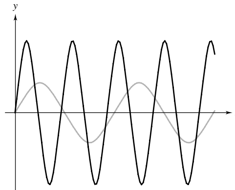
Figure 16 Solution graphs for the Duffing equation
