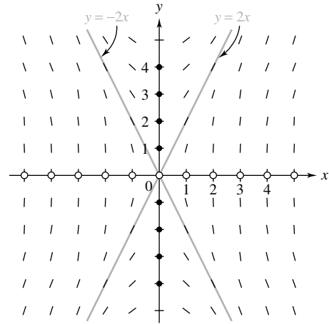
Figure 13 Direction field for dy/dx = 4x/y
