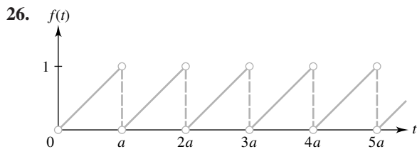
Figure 21 Sawtooth wave
