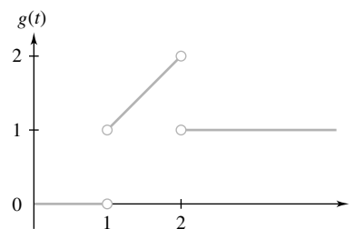
Figure 16 Function in Problem 7
