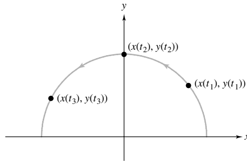
Figure 8 Phase plane trajectory of the solution pair for system (1)
