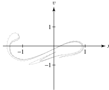
Figure 47 Poincaré section for the Duffing equation (7) with b = 0.3 , \gamma = 1.2 , and F = 0.5
