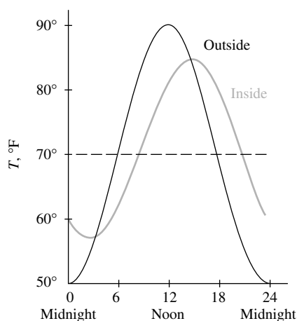
Figure 6 Temperature variation inside and outside an unheated building
