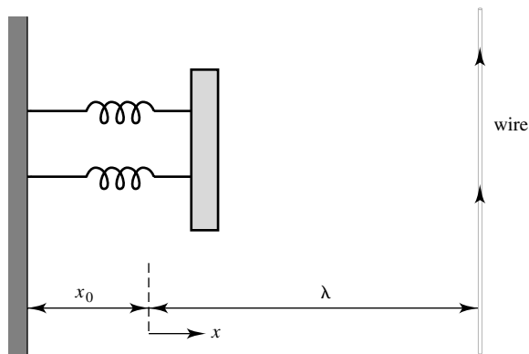
Figure 17 Bar restrained by springs and attracted by a parallel current
