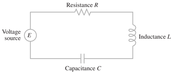
Figure 25 Schematic representation of an RLC series circuit
