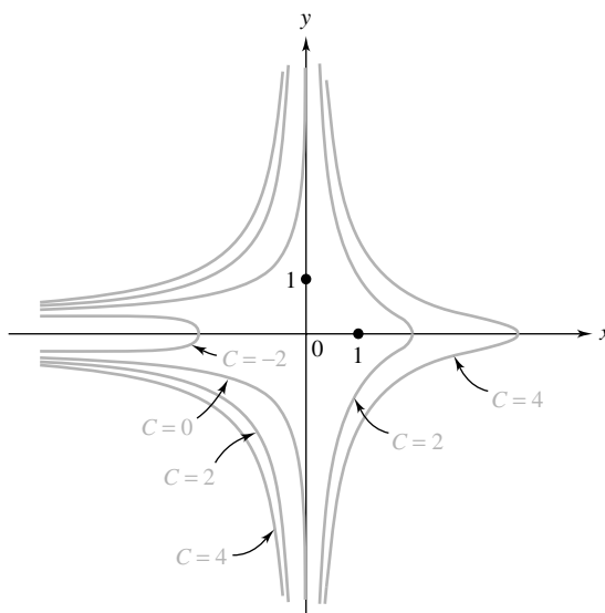
Figure 9 Solutions of Example 1
