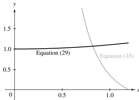
Figure 11 Partial sum approximations to solutions of Example 3
