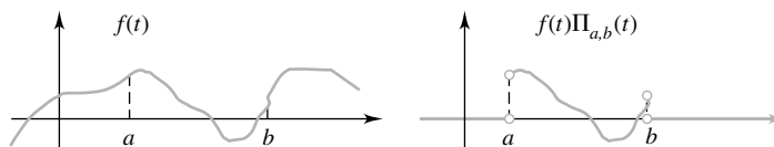
Figure 10 The windowing effect of \Pi_{a,b}(t)
