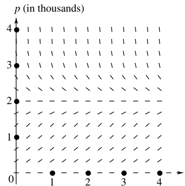
Figure 10 Direction field for logistic equation
