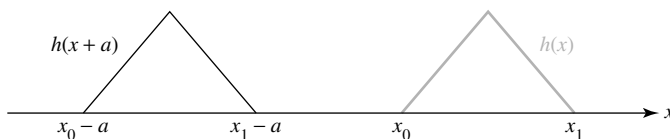
Figure 21 Graphs of h(x) and h(x + a)
