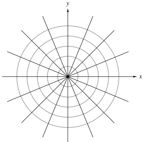
Figure 10 Orthogonal trajectories for concentric circles are lines through the center
