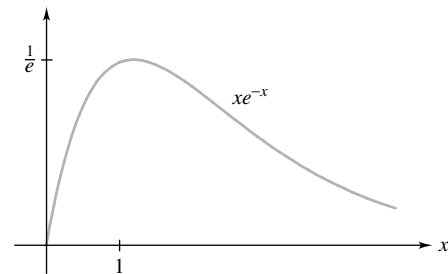
Figure 24 Graph of xe^{-x}
