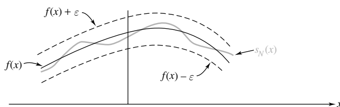
Figure 10 An \varepsilon -corridor about f
