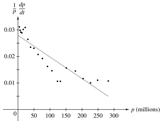
Figure 5 Scatter data and straight line fit
