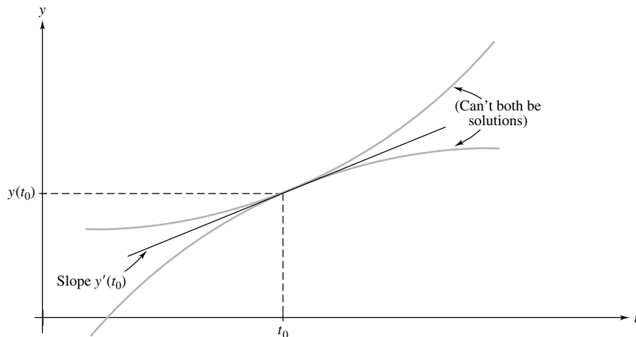
Figure 6 y(t_0), y'(t_0) determine a unique solution
