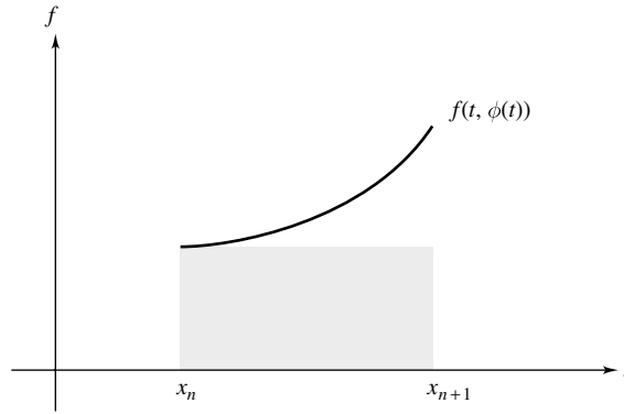
Figure 14 Approximation by a rectangle
