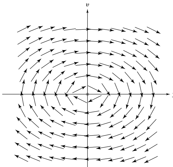
Figure 13 Direction field for Example 4
