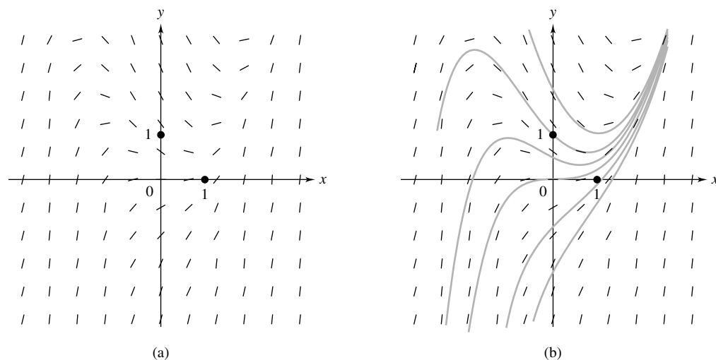
Figure 6 (a) Direction field for dy/dx = x^2 - y (b) Solutions to dy/dx = x^2 - y
