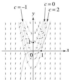
Figure 9 Solution to Problem 15
