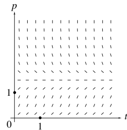
Figure 4 Direction field for Problem 5(a)
