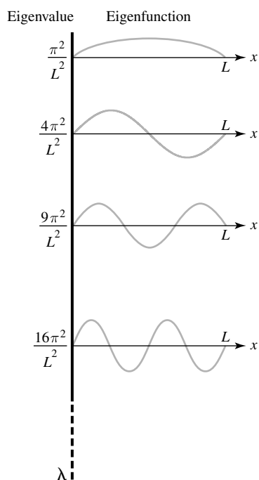
Figure 2 Eigenfunctions
