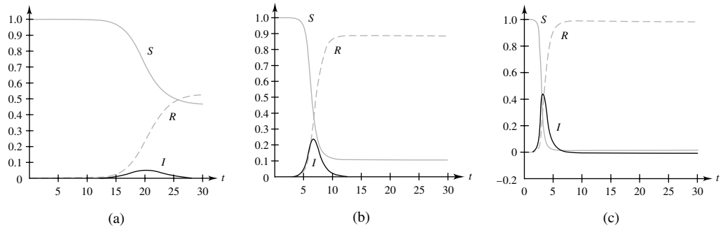
Figure 22 SIR simulations (a) k = 1.4 , a = 2.0 ; (b) k = 1.4 , a = 3.5 ; (c) k = 1.4 , a = 6.0
