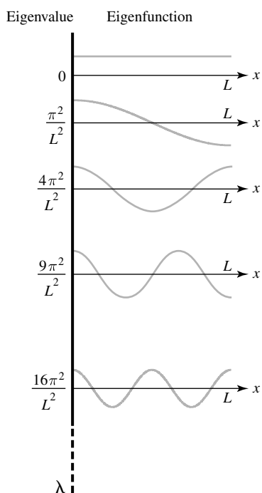
Figure 15 Cosine eigenfunctions
