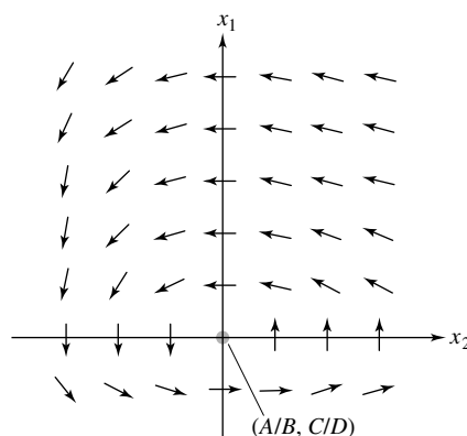
Figure 20 Typical direction field diagram for the Volterra–Lotka system
