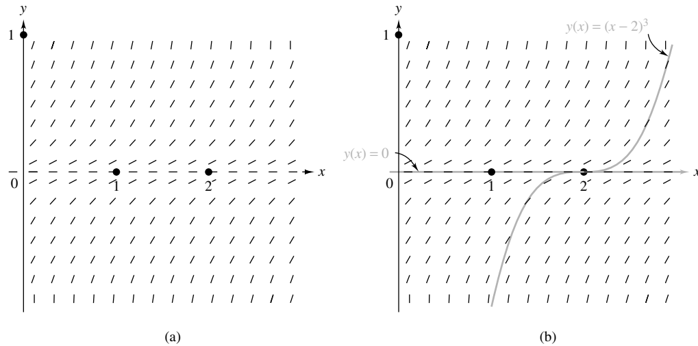
Figure 9 (a) Direction field for dy/dx = 3y^{2/3} (b) Solutions for dy/dx = 3y^{2/3} , y(2) = 0
