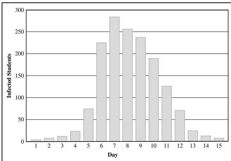
Figure 25 Flu data for Problem 11
