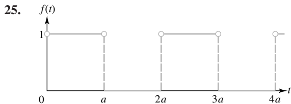
Figure 20 Square wave
