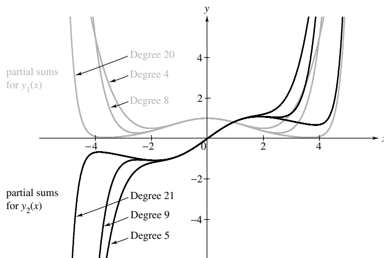
Figure 4 Partial sum approximations to solutions for Example 3
