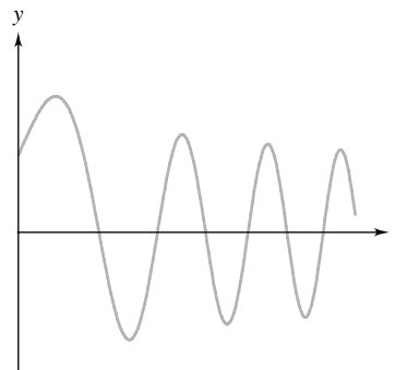
Figure 12 Solution to equation (14)
