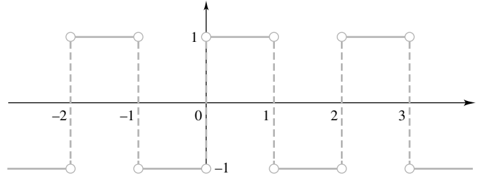
Figure 14 Graph of square wave function f(t)
