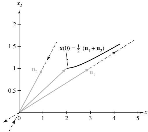
Figure 1 Trajectories of solutions for Example 3
