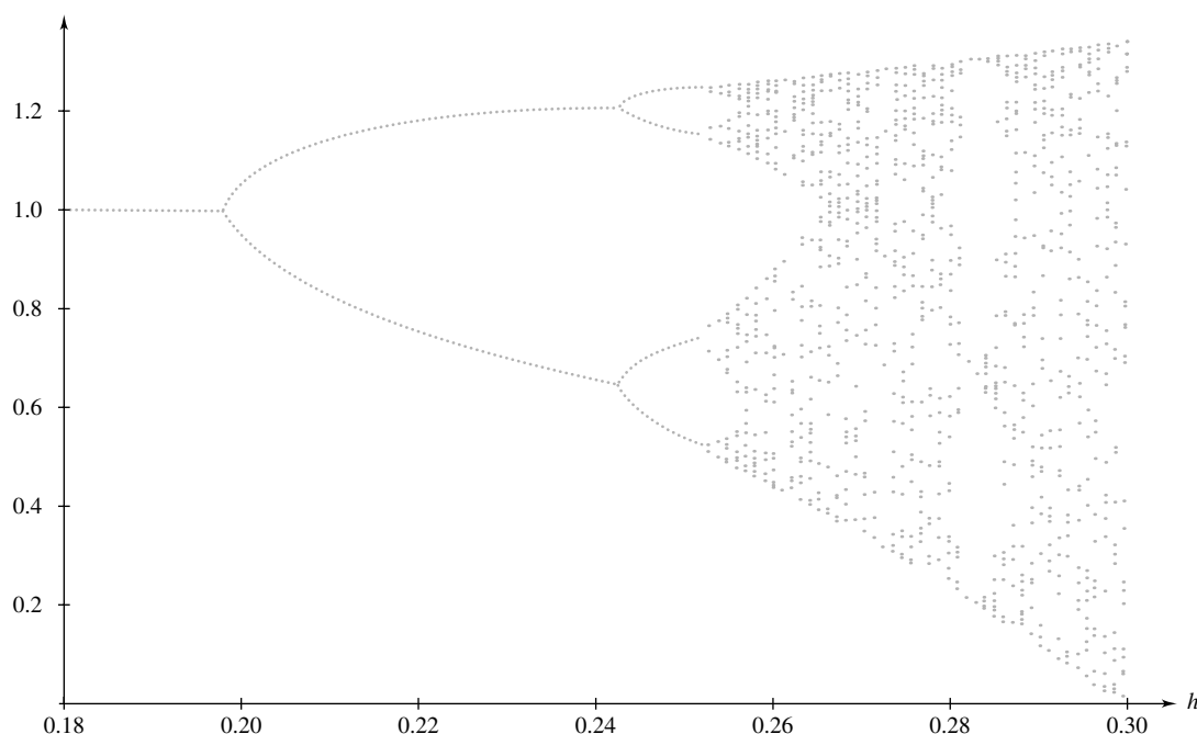
Figure 22 Period doubling to chaos
