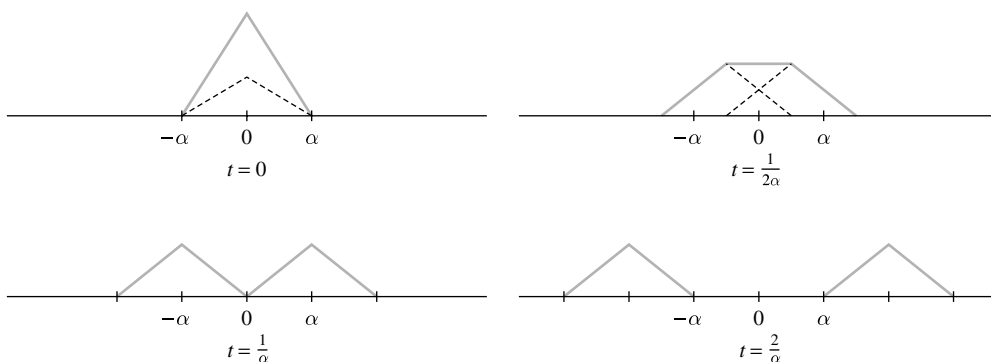
Figure 23 Decomposition of initial displacement into traveling waves
