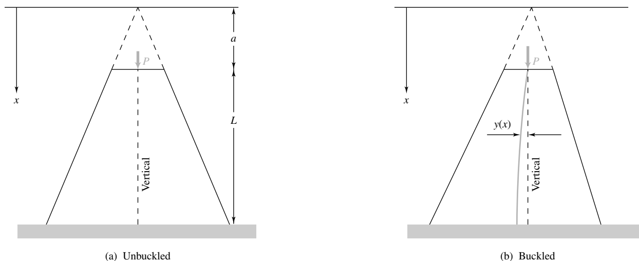
Figure 16 Buckling tower
