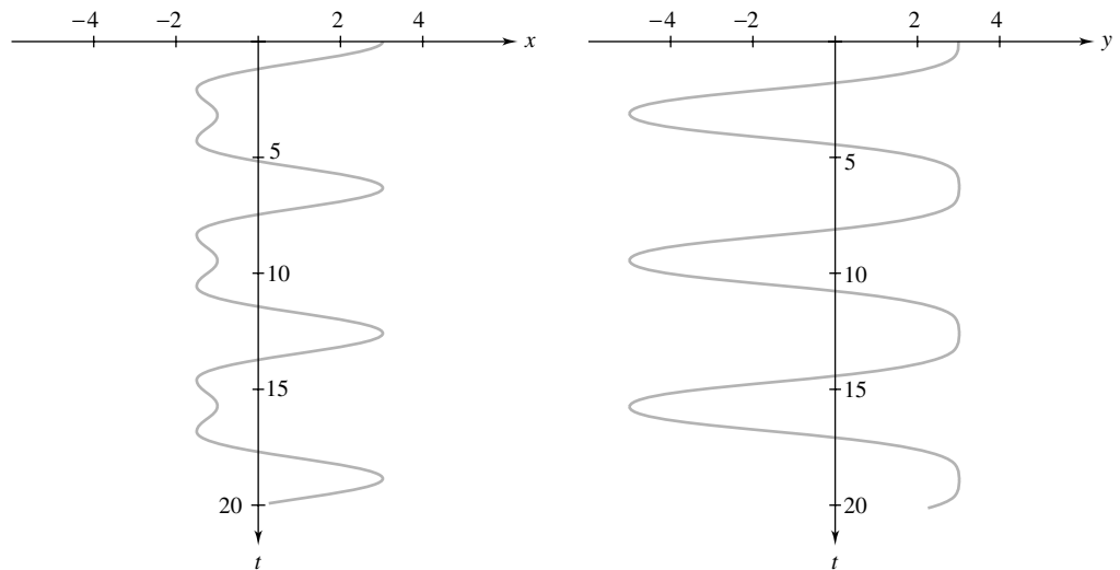
Figure 28 Graphs of the motion of the two masses in the coupled mass–spring system
