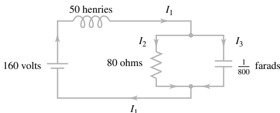
Figure 7 RLC network for Problem 22
