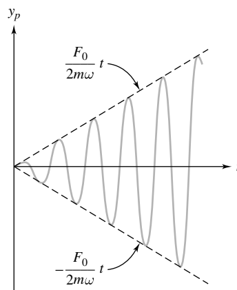
Figure 34 Undamped oscillation of the particular solution in (21)
