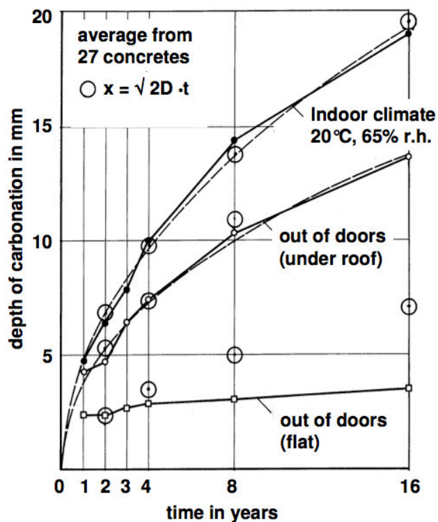
Fig. 2.6: Carbonation depth as function of time and environment [12]
