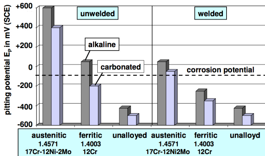
Fig. 5.7: Pitting potential E_p of deformed steel specimens in mortar-electrodes with 3 mass-% chloride depending on the steel type, the presence of welds and carbonation; potentiostatic test (oxygen evolution potential E = +600 mV SCE )
