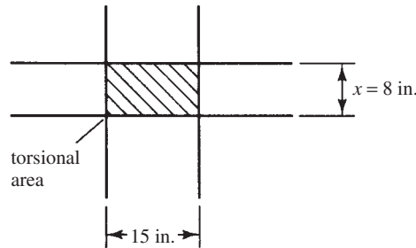
FIGURE 17.10 Torsional member.
