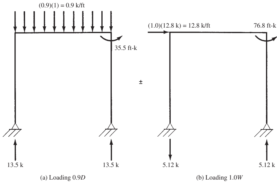
FIGURE 11.12 Nonsway and sway load cases for U = 0.9D + 1.0W .
