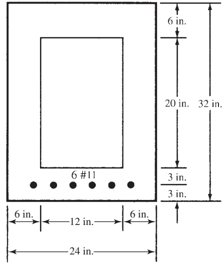
Problem 5.15 (Ans. 1075.2 ft-k)
