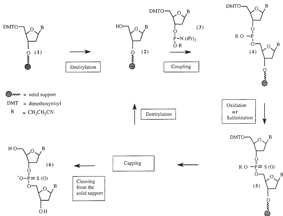
Fig. 2. Steps in solid-phase DNA synthesis.
