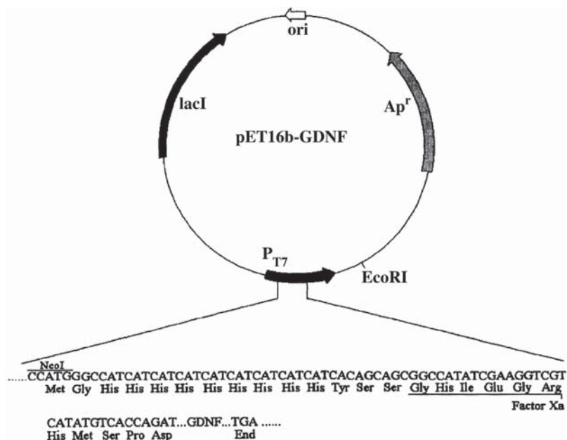
Fig. 2. pET16b-GDNF.
