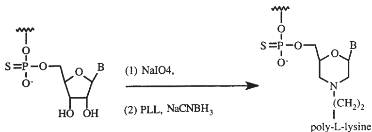
Fig. 4. Conjugating poly-L-lysines.
