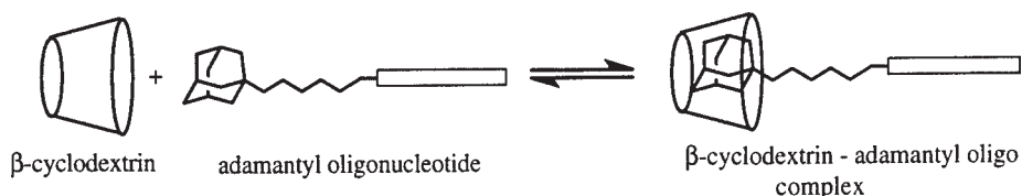
Fig. 7. Adamantane–oligonucleotide–cyclodextrin complexes.
