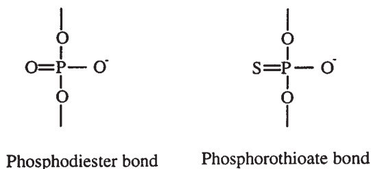
Fig. 1. Phosphorothioates.
