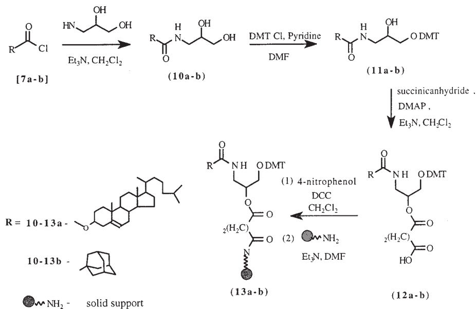
Fig. 6. Derivatizing the solid support for 3' functionalization.
