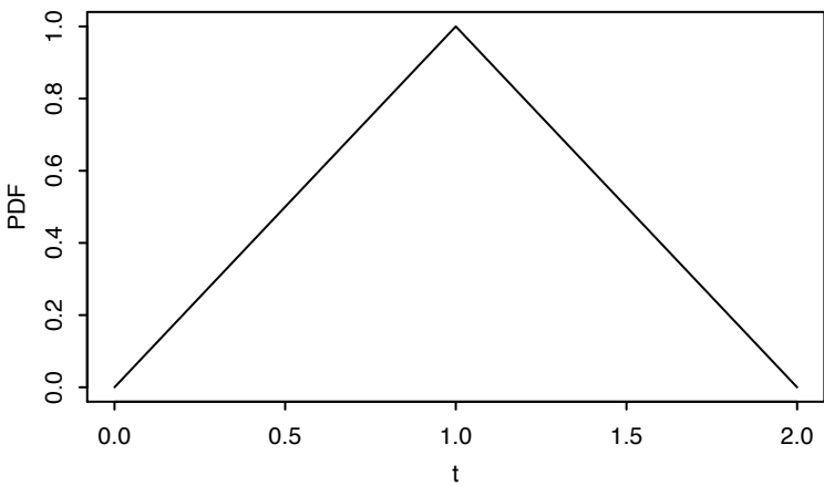
FIGURE 8.2 PDF of T = X + Y , where X and Y are i.i.d. \text{Unif}(0, 1) .
