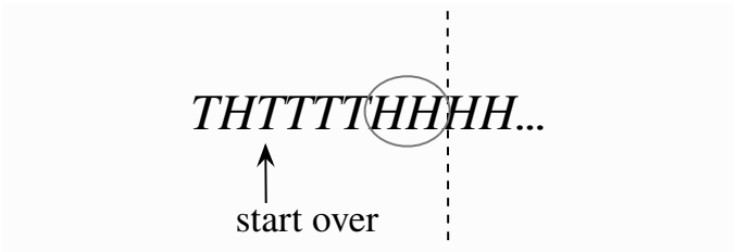
FIGURE 9.4 When waiting for HH , partial progress can easily be destroyed.
