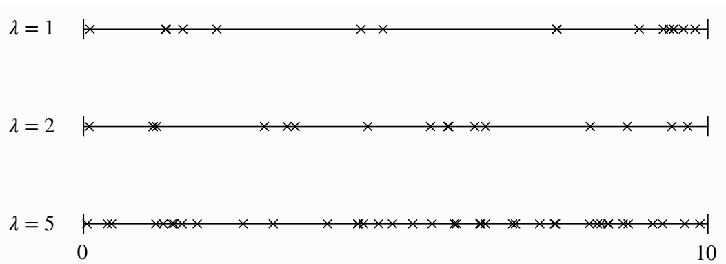
FIGURE 13.1 Simulated Poisson process in one dimension, for \lambda = 1, 2, 5 .
