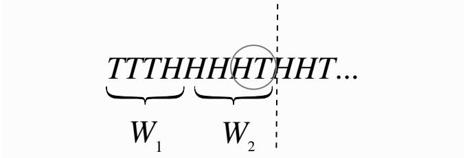
FIGURE 9.3 Waiting time for HT is the waiting time for the first Heads, W_1 , plus the additional waiting time for the next Tails, W_2 . Durable partial progress is possible!
