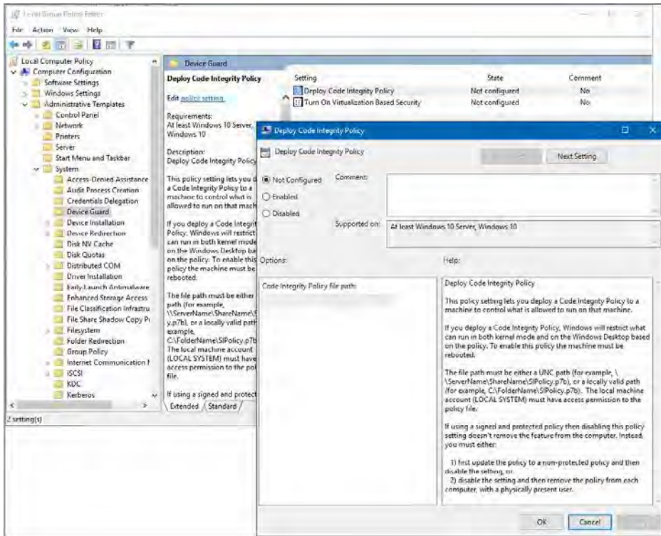
FIGURE 15-2 Device Guard is a new feature you can use to lock down a Windows 10 device so that it runs only trusted programs. These policy settings are just a small part of the deployment process.
