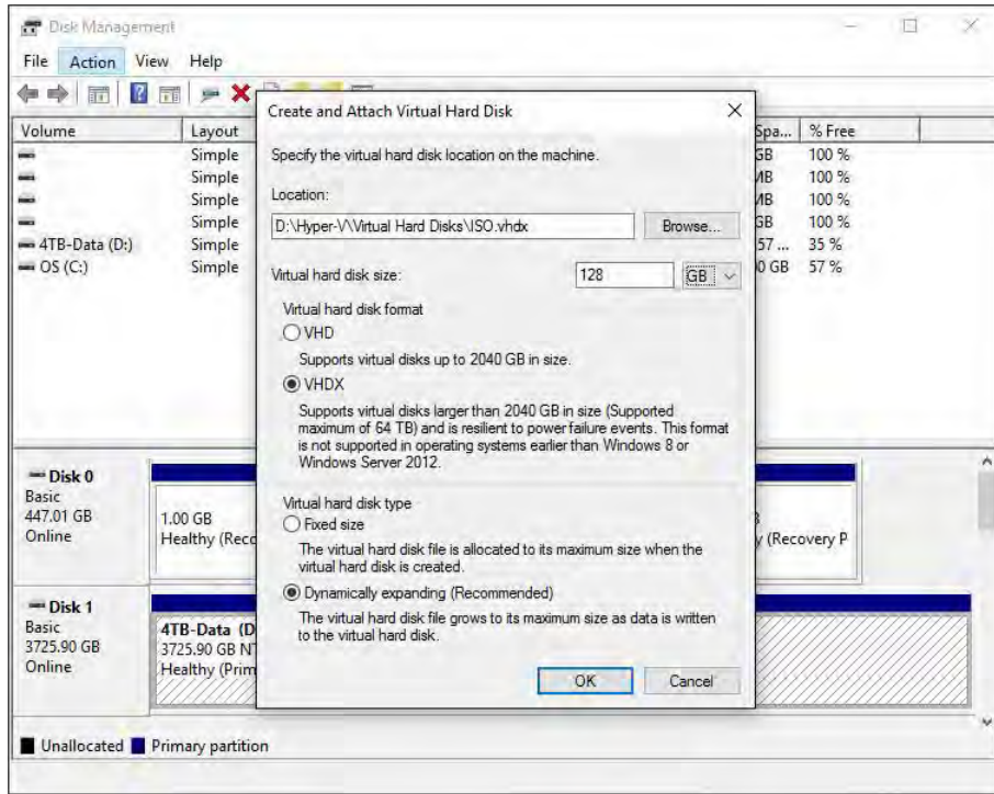
FIGURE 12-9 Click the Action menu in Disk Management and then choose Create VHD to open this dialog box. Choose a location and a file name to create a virtual hard disk that acts like a separate physical drive.
