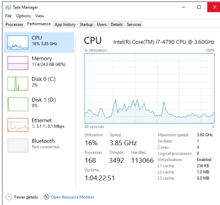
FIGURE 9-6 The Performance tab in Task Manager shows a wealth of information about CPU, memory, disk, and network usage. Note the link at the bottom to open Resource Monitor.
