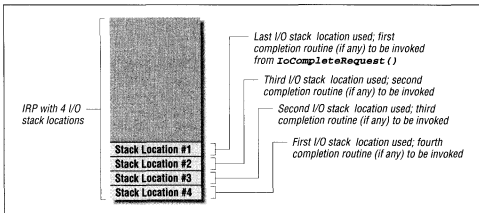
Figure 12-4. I/O manager sequence for invoking completion routines
