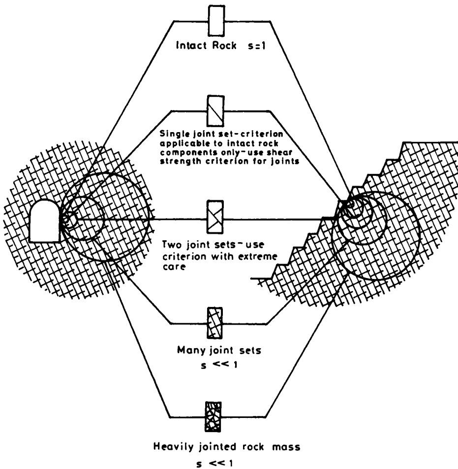
Figure 3.1: Rock mass conditions under the Hoek-Brown failure criterion (Hoek, 1994)
