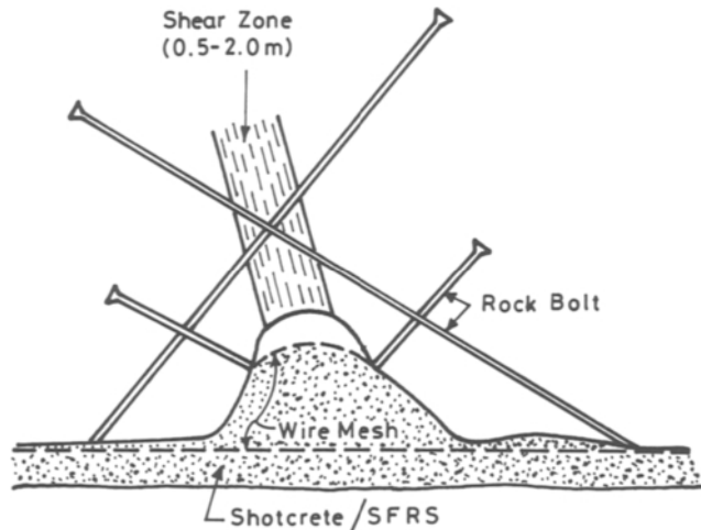
Figure 2.1: Shear zone treatment in an underground opening (Lang, 1971)
