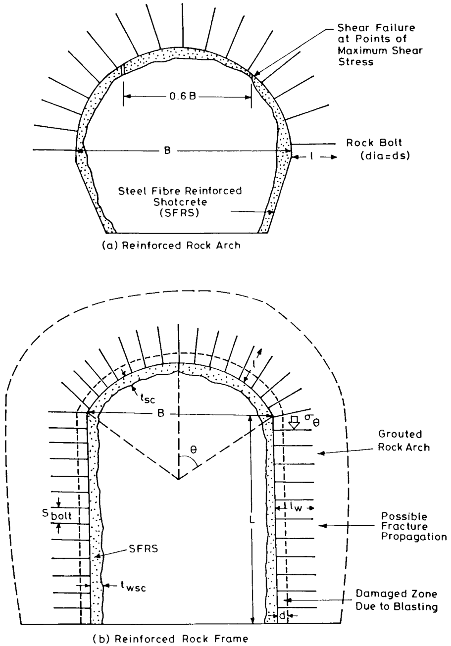
Figure 12.1: Design of support system for underground openings
