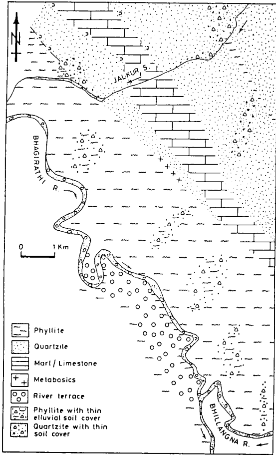
Figure 18.4: Lithological map
