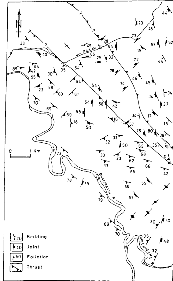
Figure 18.5: Structural map
