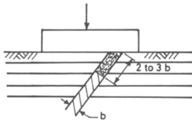
Figure 2.3: Weak seams under foundation less than 20 per cent area
