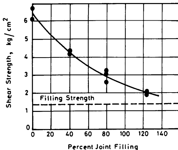
Figure 23.2: Effect of joint filling thickness on shear strength (Goodman, 1970)
