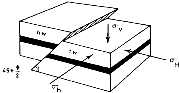
(b) Reverse or thrust fault
