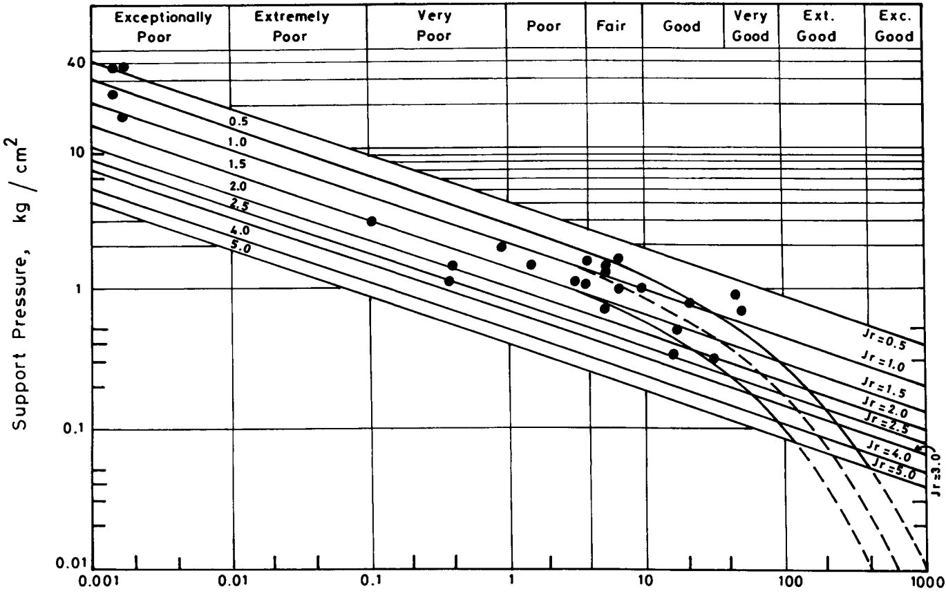
Figure 8.2: Correlation between support pressure and rock mass quality Q (Barton et al., 1974)
