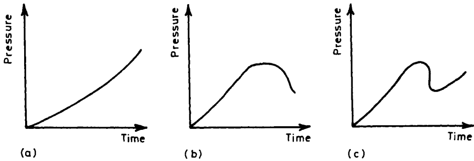
Figure 22.5: Plots to check the success of grouting (Jahde, 1937)
