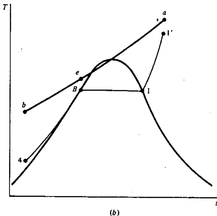
Figure 2-6 Superheat with (a) water as primary fluid, (b) gases or liquid metal as primary fluid.
