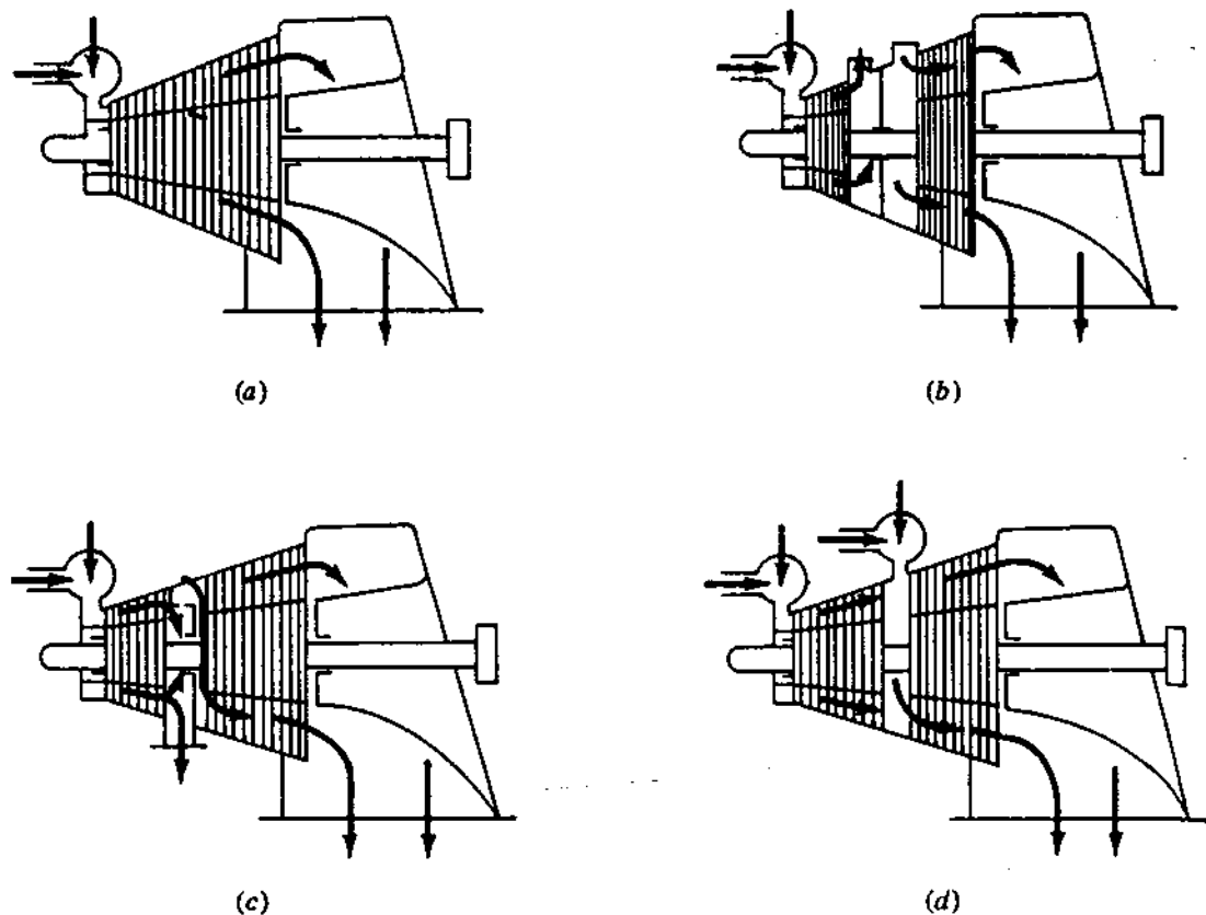
Figure 5-24 Turbine arrangements as affected by different steam paths: (a) straight through; (b) single reheat; (c) extraction; (d) induction.
