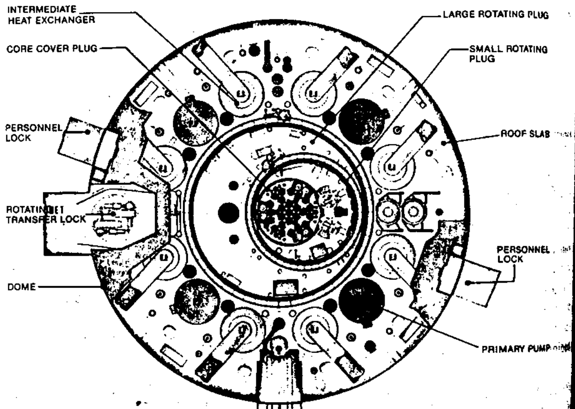
Figure 11-24 Plan view of Super Phénix reactor block.
