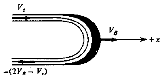
Figure 5-3 The impulse of a fluid jet on a 180° curved blade.
