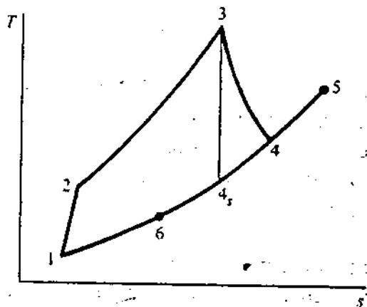
Figure 8-22 T-s diagram for the gas in Example 8-4.
