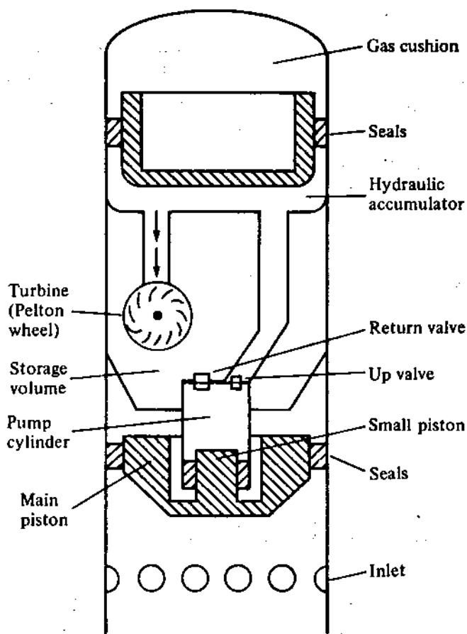
Figure 15-14 Schematic of a hydraulic-accumulator wave machine [151].
