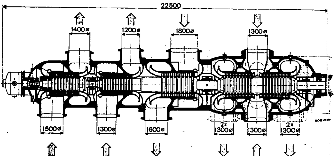
Figure 5-28 A proposed design for a helium-driver gas turbine, dimensions in millimeters [44].
