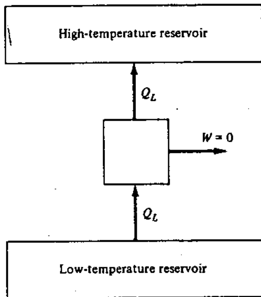
Figure 1-6 A device that violates the Clausius statement of the second law.
