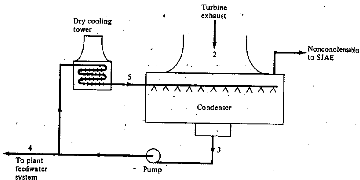
Figure 6-1 Schematic flow diagram of a direct-contact condenser of the spray type. SJAЕ = steam-jet air ejector.
