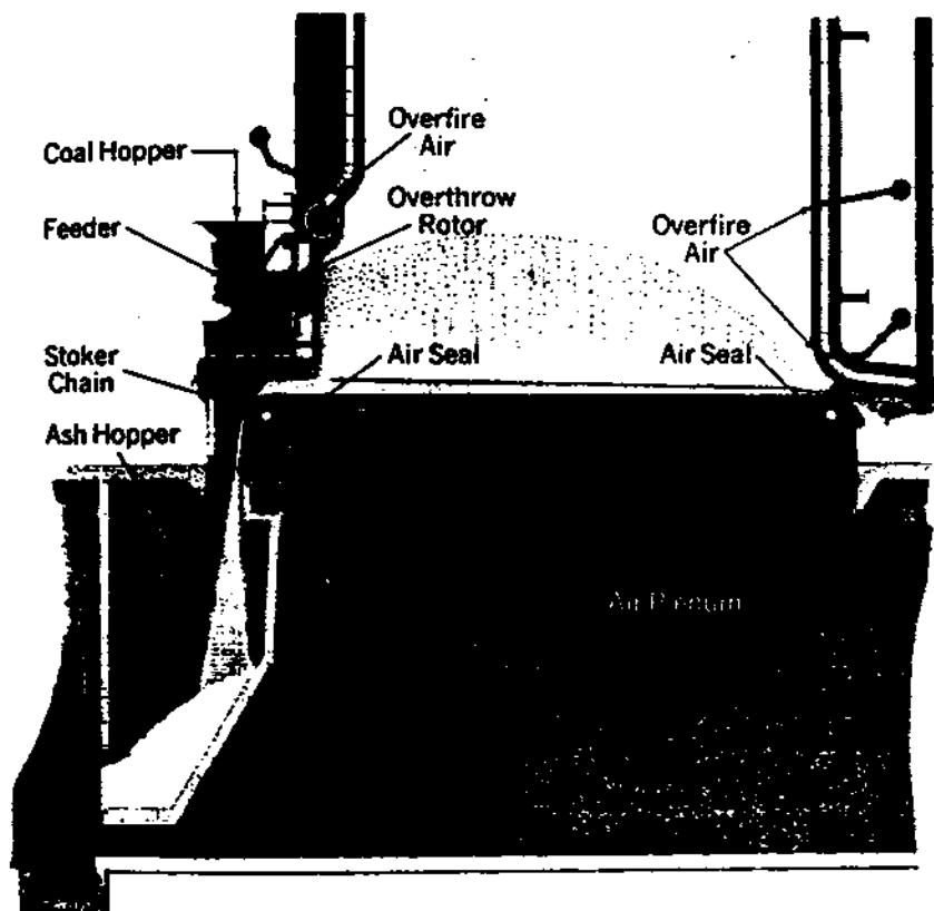
Figure 4-2 A traveling-grate spreader stoker with front ash discharge. (Courtesy Babcock and Wilcox.)
