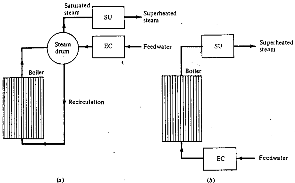
Figure 3-13 Schematic flow diagrams of (a) drum type and (b) once-through steam generators. SU = superheater, EC = economizer.
