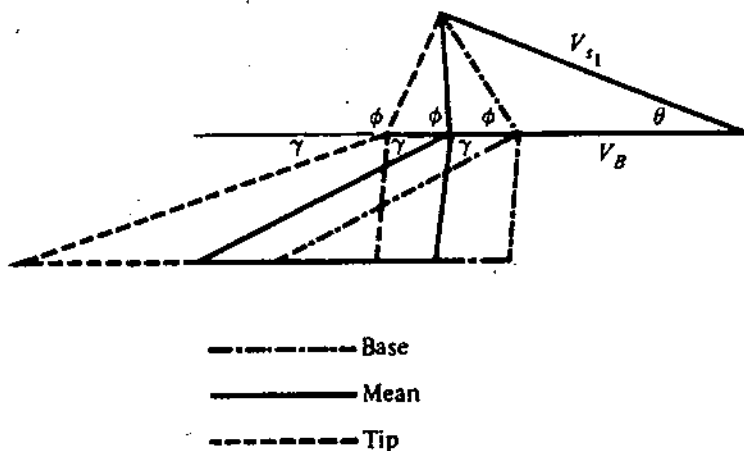
Figure 5-17 Effect of reaction blade height on entrance and exit angles, necessitating a warped radial shape. Drawn for same V_{s1} , \theta , and same exit whirl.
