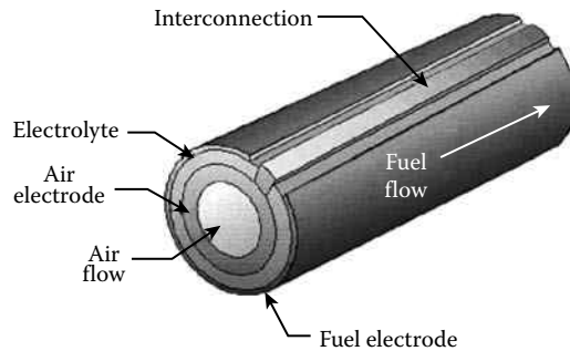
FIGURE 14.8 Tubular SOFC.
