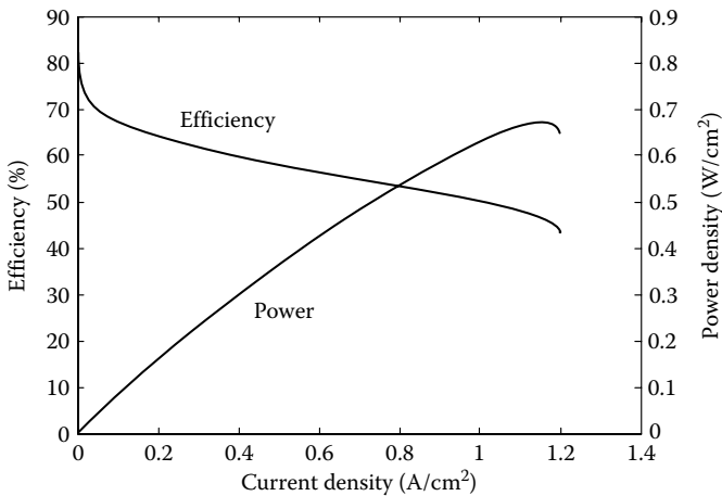
FIGURE 14.4 Operating efficiency and power density along with the current density in a hydrogen–oxygen fuel cell.
