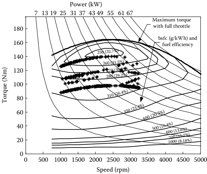
FIGURE 10.26 Engine operating points overlapping its fuel consumption map in LA92 driving cycle with CD mode.
