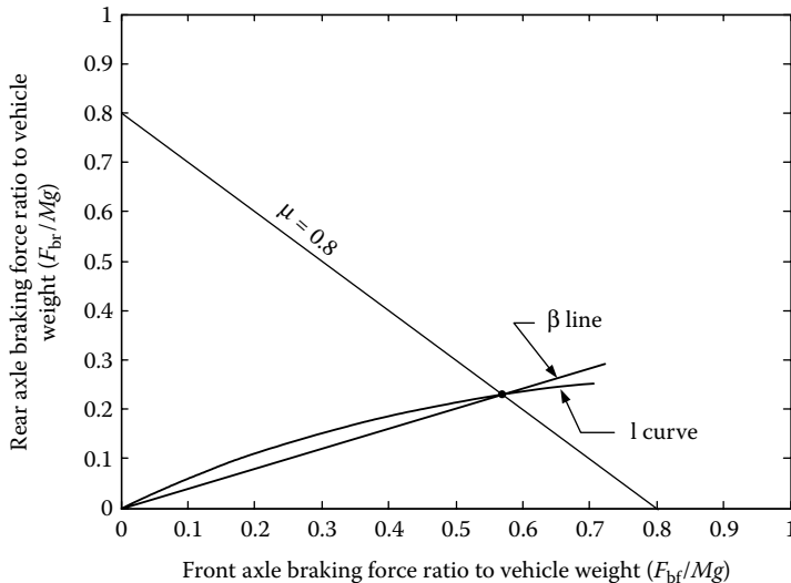
FIGURE 2.40 Ideal and actual braking force distribution curves.
