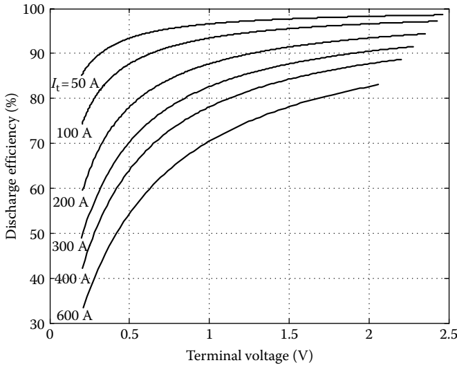
FIGURE 12.12 Discharge efficiency of the 2600F Maxwell Technologies ultracapacitor.
