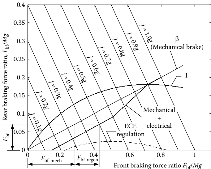
FIGURE 13.10 Braking forces varying with deceleration rate.
