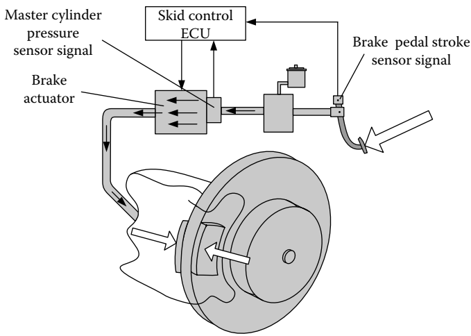
FIGURE A.10 Brake assist.
