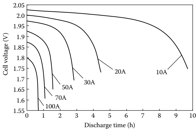
FIGURE 11.7 Discharge characteristics of the lead-acid battery.
