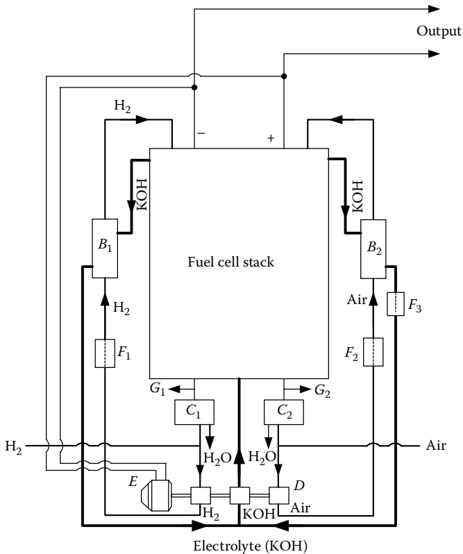
FIGURE 14.7 Circulating electrolyte and supplies of hydrogen and air in an AFC; B_1 , B_2 , heater exchangers; C_1 , C_2 , condensers; D , pampers; E , motor; F_1 , F_2 , F_3 , controls; and G_1 , G_2 , outlets. 8
