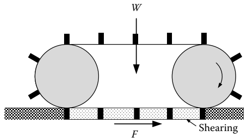
FIGURE 16.3 Shearing action of a track.
