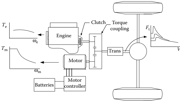
FIGURE 5.10 Two-shaft configuration.
