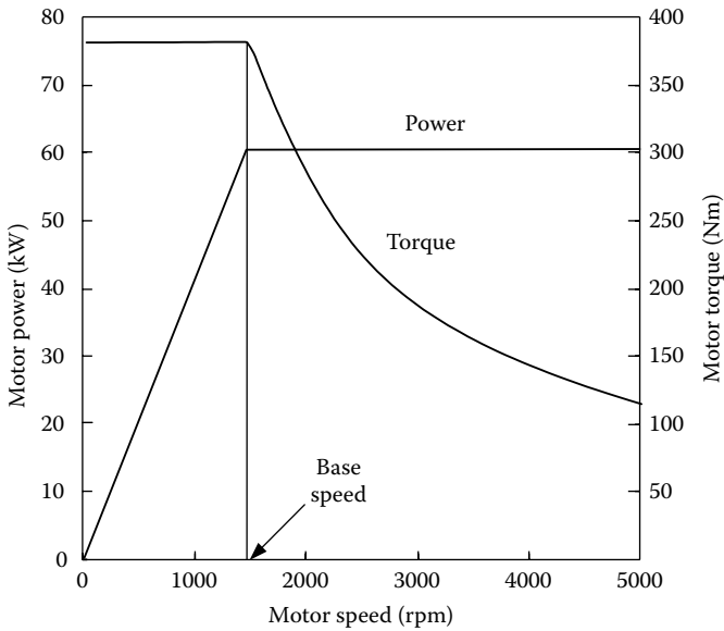
FIGURE 4.4 Typical variable-speed electric motor characteristics.
