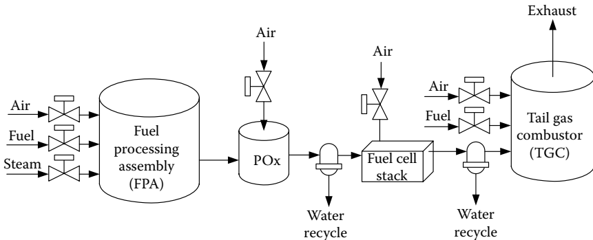
FIGURE 14.11 Fuel processing diagram. 13
