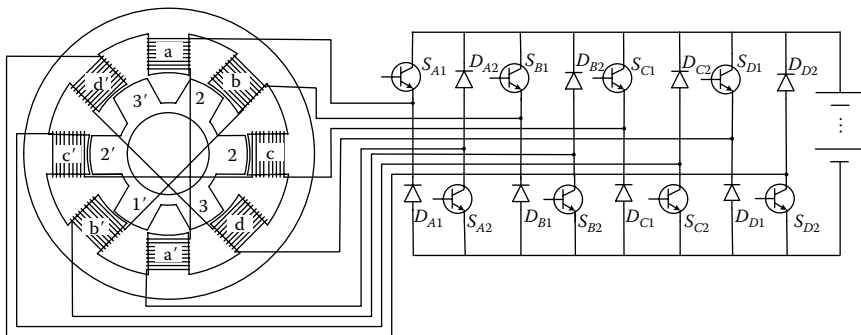
FIGURE 6.55 SRM and its power supply.
