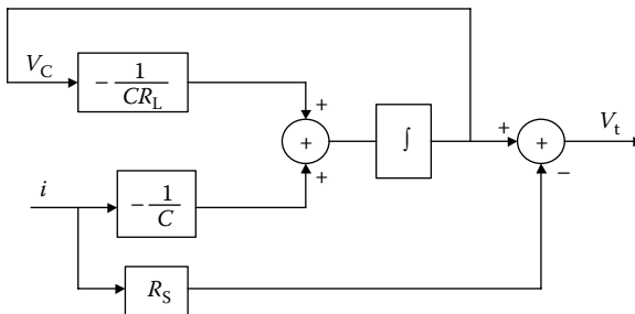
FIGURE 12.10 Block diagram of the ultracapacitor model.
