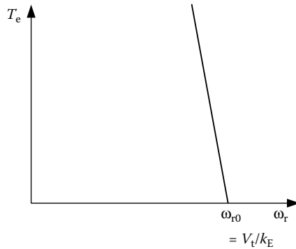
FIGURE 6.49 Speed–torque curve in the steady state with constant voltage.
