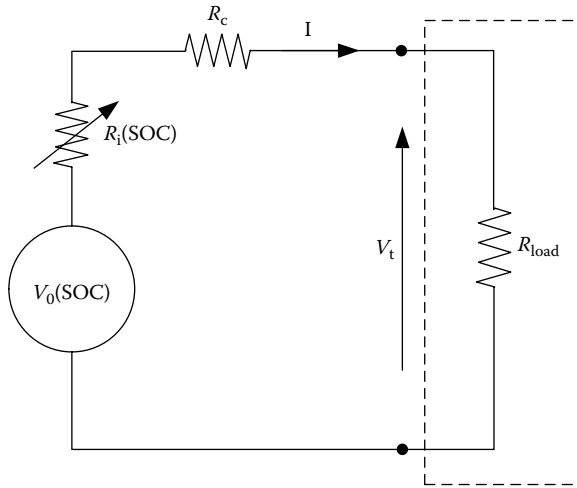
FIGURE 11.8 Battery model.
