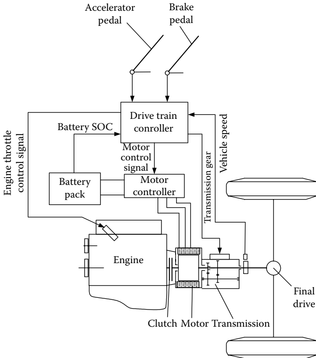
FIGURE 11.3 Configuration of the parallel connected mild hybrid electric drive train.
