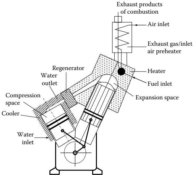
FIGURE 3.16 Diagram of a practical opposed-piston Stirling engine.
