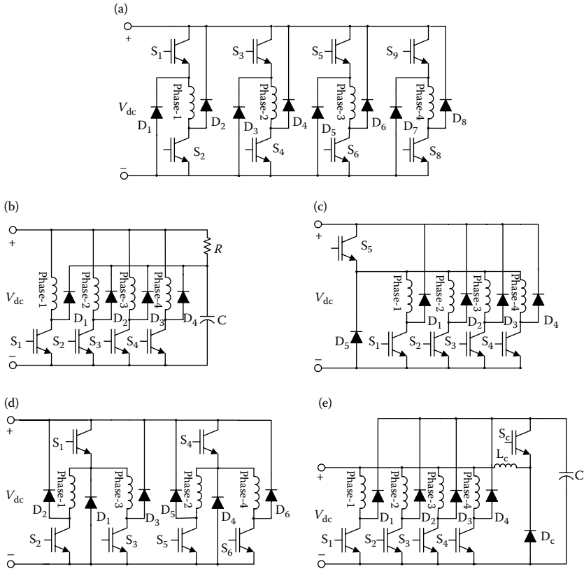
FIGURE 6.62 Different inverter topologies for SRM drives: (a) classic half-bridge converter; (b) R-dump; (c) n + 1 switches (Miller converter); (d) 1.5n switch converter; and (e) C-dump.
