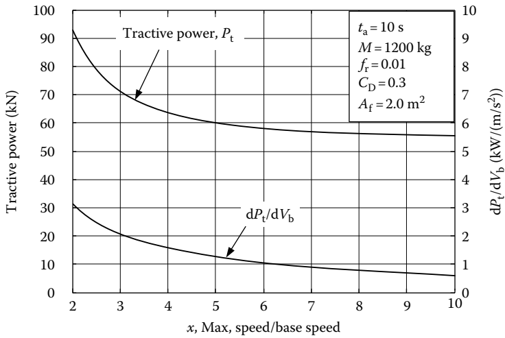
FIGURE 4.9 Power rating versus speed factor.
