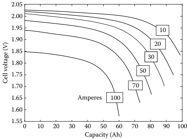
FIGURE 12.3 Discharge characteristics of a lead-acid battery.
