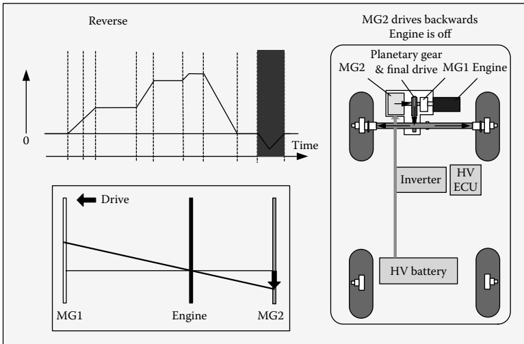
FIGURE A.22 Reverse operation.
