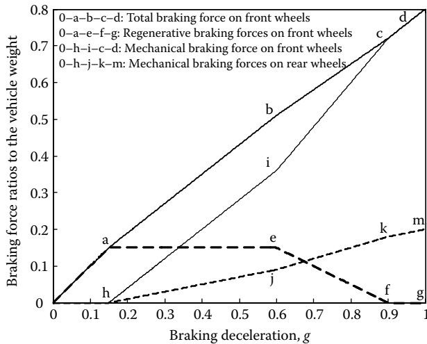
FIGURE 13.11 Braking force ratios relative to the vehicle weight varying with deceleration rate.
