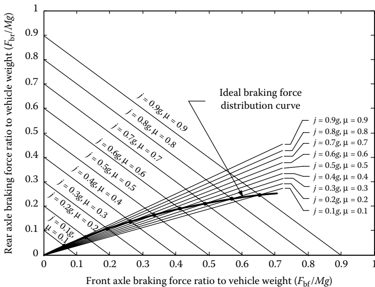
FIGURE 2.39 Ideal braking force distribution curve on the front and rear axles.
