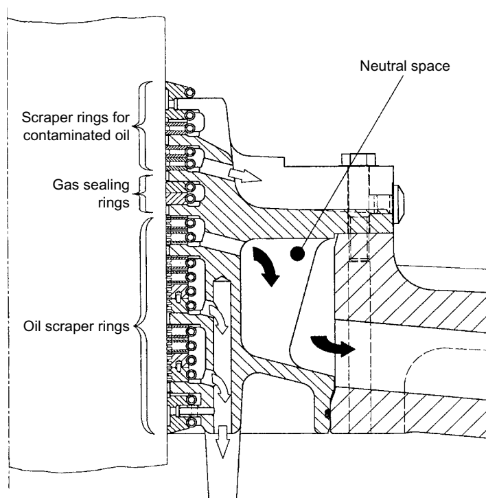
FIGURE 12.16 Piston rod gland of RTA84T engine; all rings are made of bronze
