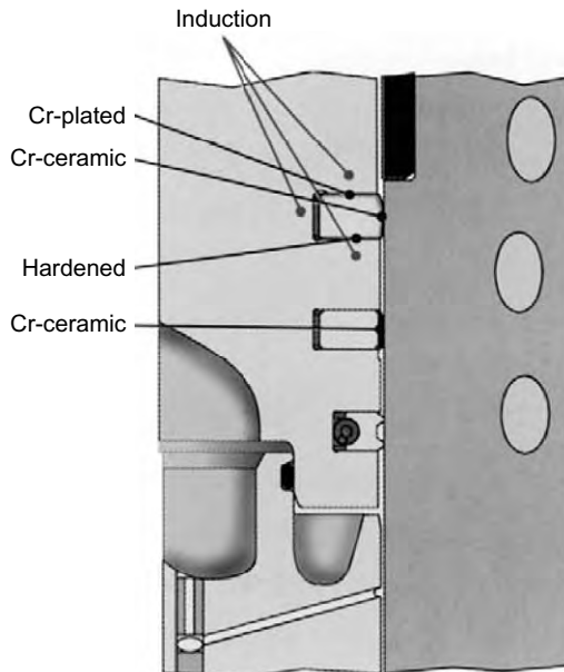
FIGURE 27.32 Three-ring pack for Wäertsilä 64 engine piston; note the anti-polishing ring incorporated in the upper cylinder liner (top right)
