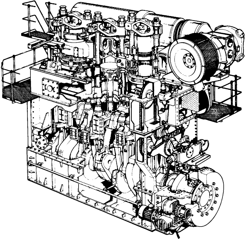
FIGURE 14.2 Cutaway drawing of a 58JS3C engine
