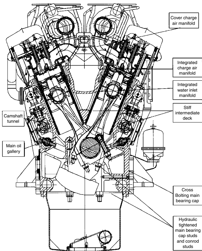
FIGURE 28.1 V-version of Anglo Belgian Corporation's DZ engine
