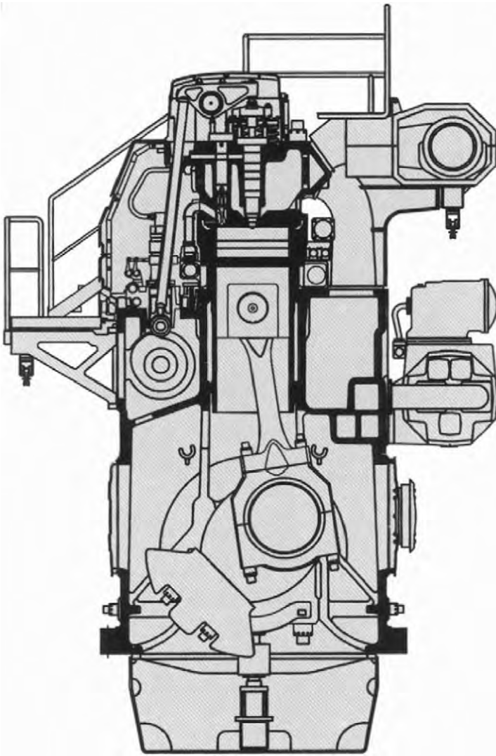
FIGURE 27.31 Cross-section of Wärtsilä 64 design
