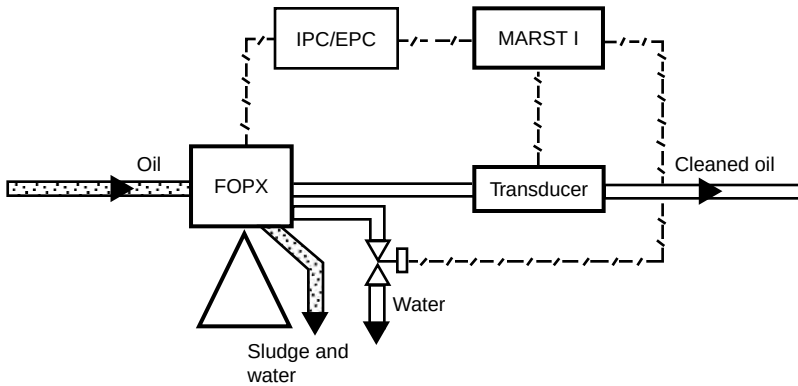
FIGURE 4.3 Schematic diagram of Alfa Laval's Alcap fuel-treatment system based on its FOPX centrifugal separator
