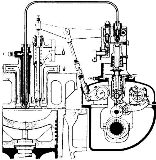
FIGURE I.10 Direct fuel injection system introduced by Sulzer in 1930, showing the reversing mechanism and cam-operated starting valve. Airless fuel injection had been adopted by all manufacturers of large marine engines by the beginning of the 1930s: a major drawback of earlier engines was the blast injection system and its requirement for large, high-pressure air compressors which dictated considerable maintenance and added to parasitic power losses
