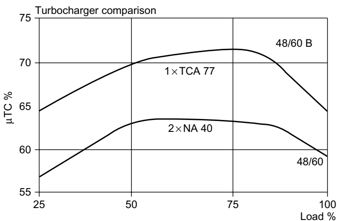
FIGURE 22.26 Comparison of turbocharger efficiencies: the MAN TCA77 on the 12V48/60B engine and the MAN NA40 on the original 12V48/60 engine
