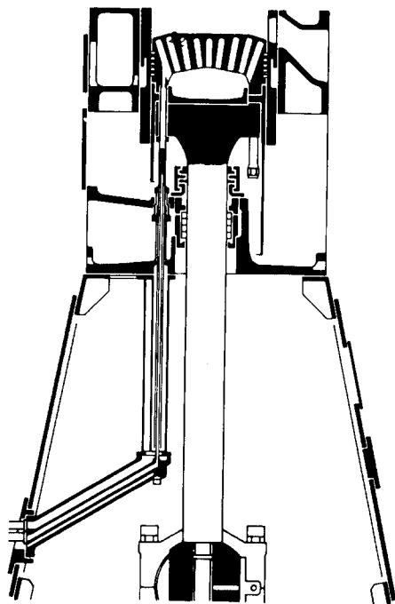
FIGURE 12.46 Arrangement of telescopic pipes for RL engine piston cooling
