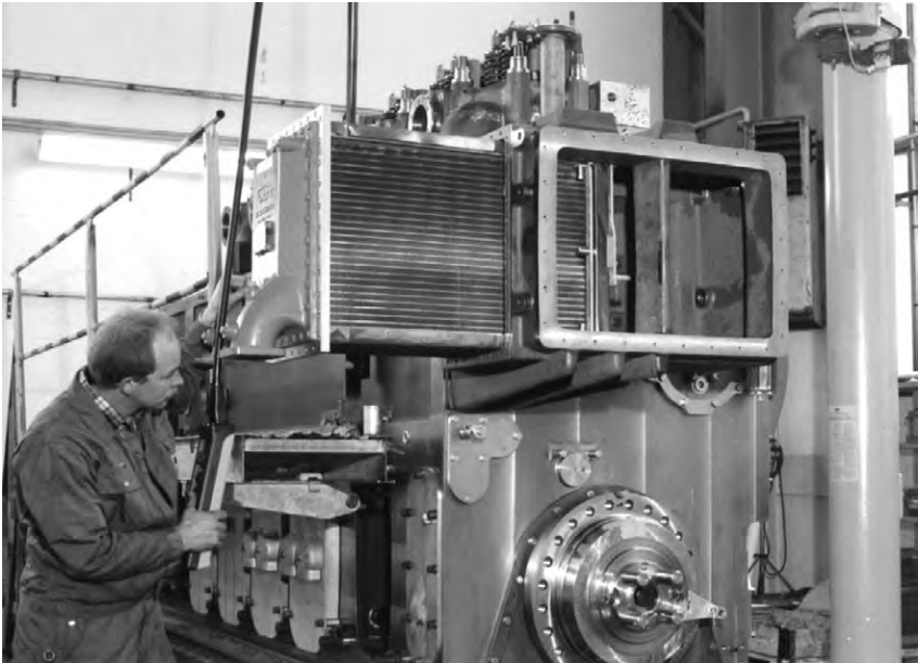
FIGURE 21.4 The M32 engine's charge air cooler is housed drawer-like in a console screwed onto the frame
