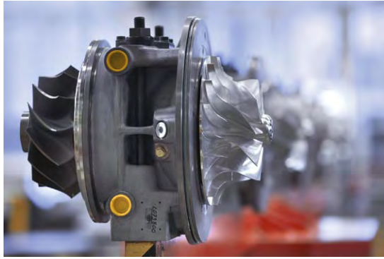
FIGURE 7.20 ABB's new generation A100 series turbocharger
