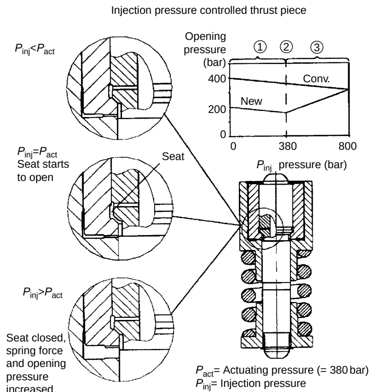
FIGURE 10.26 Fuel valve with variable opening pressure
