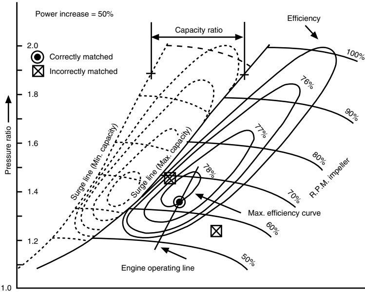
FIGURE 7.6 Turboblower characteristics
