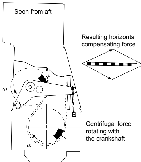
FIGURE 1.13 First-order moment compensator (MAN Diesel)
