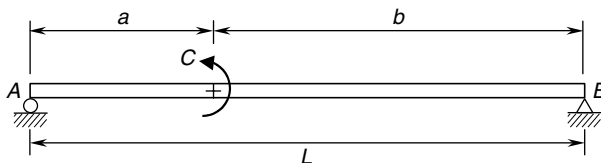
FIGURE 2.23 Concentrated couple at intermediate point.
