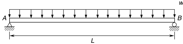
FIGURE 2.30 Uniform load.
