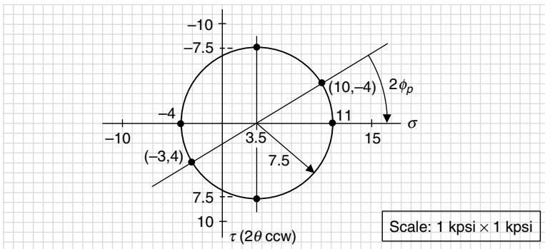
FIGURE 5.21 Principal stresses angle ( \phi_p ).
