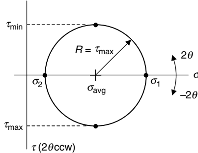
FIGURE 5.6 Mohr's circle.
