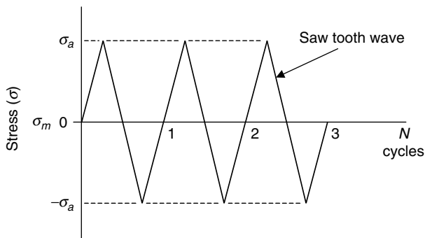
FIGURE 7.2 Reversed loading (saw tooth wave).
