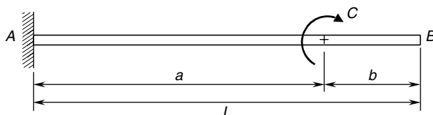
FIGURE 2.97 Concentrated couple.
