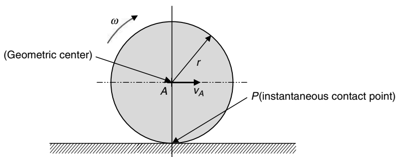
FIGURE 10.21 Velocity of a rolling wheel on a flat surface.
