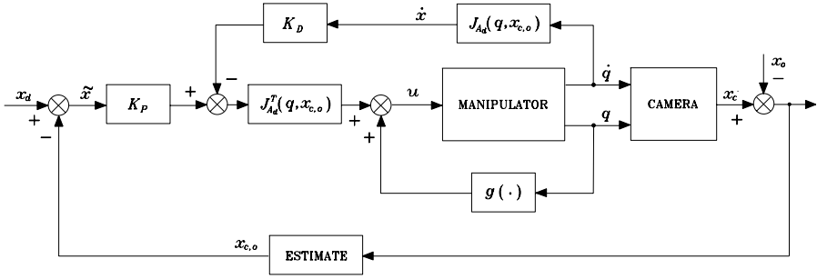
Fig. 10.14. Block scheme of position-based visual servoing of PD type with gravity compensation
