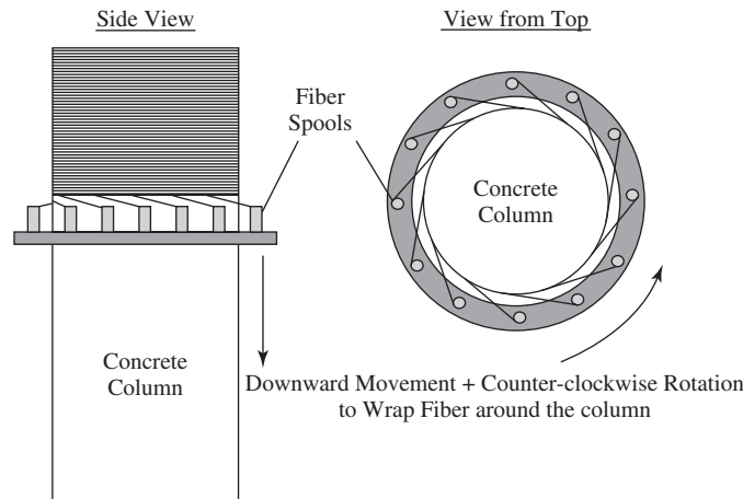
Figure 5-19 Column retrofitting using the confinement concept
