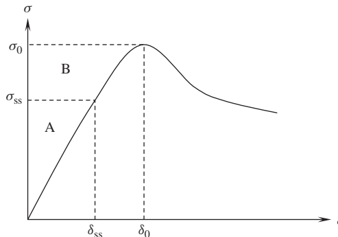
Figure 6-51 Schematic illustration of energy balance concept on a fiber bridging stress–crack opening stress–strain curve
