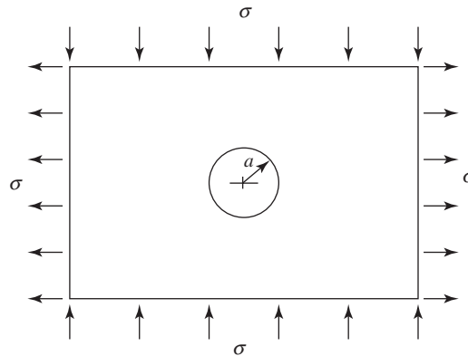
Figure 7-4 A thin plate with a circular hole subjected to pure shear
