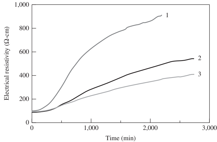
Figure 8-61 Resistivity of cement pastes ( w/c = 1.0, 0.30, 2.0, 0.40, 3.0, 0.50 )
