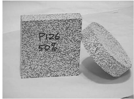
Figure 6-19 Extruded heat insulation products
