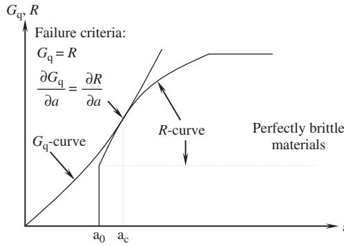
Figure 7-40 Schematic of the R -curve
