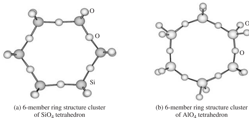
Figure 2-25 Molecular structure representing model of metakaolinite
