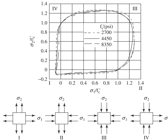
Figure 5-14 Behavior of concrete under biaxial stress
