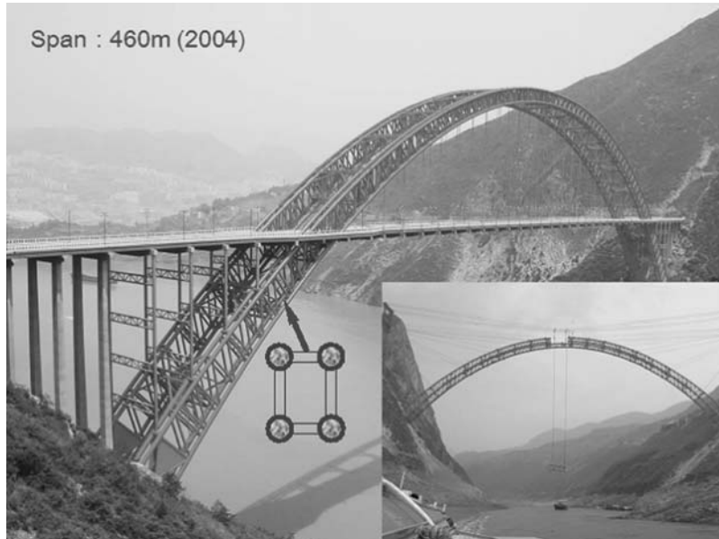
Figure 6-55 Wushan CFST arch bridge, Chongqing China
