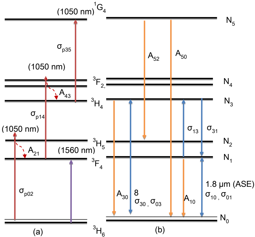
Figure 17. Pumping mechanism of a 1050 and 1560nm pumped TDFA (a) pump transitions (b) signal and ASE emission transitions.
