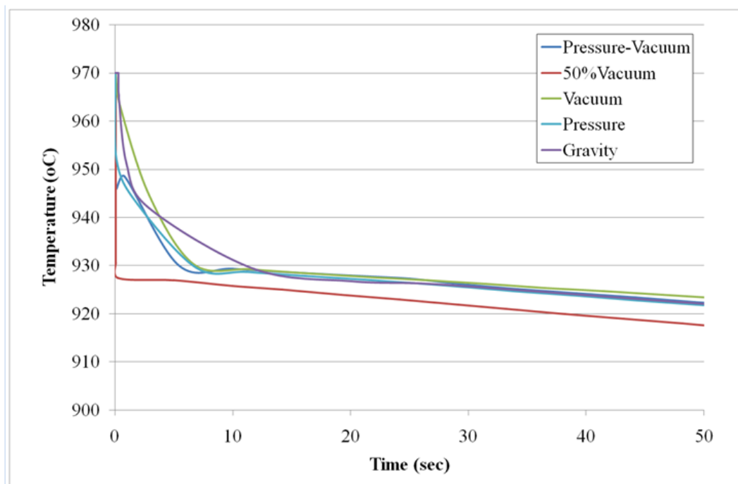
Figure 17. Numerical cooling curves obtained for the five casting cases examined, for the first 10sec of solidification.
