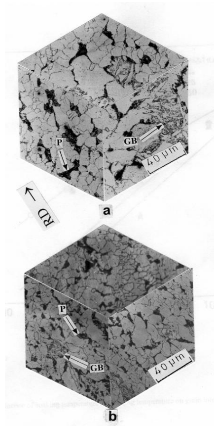
Figure 7. Composite micrographs of steel 1 soaked at 1100^{\circ}\text{C} , rolled at 800^{\circ}\text{C} and deformed (a) 25% (b) 50%.
