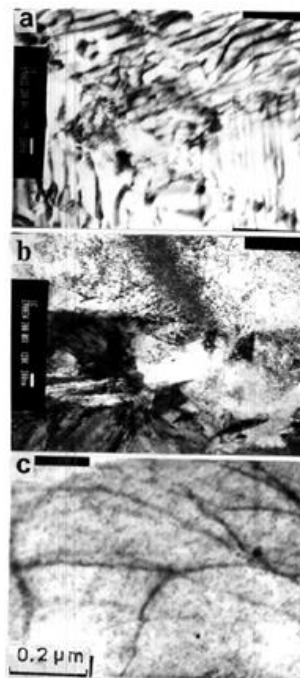
Figure 12. TEM micrographs of steel 1 soaked at 1100^{\circ}\text{C} and deformed 50% at 800^{\circ}\text{C} showing (a) pearlite (b) ferrite with high dislocation density and M/A constituent (c) ferrite containing extremely fine Nb (C,N) particles of about 100\text{\AA} size.
