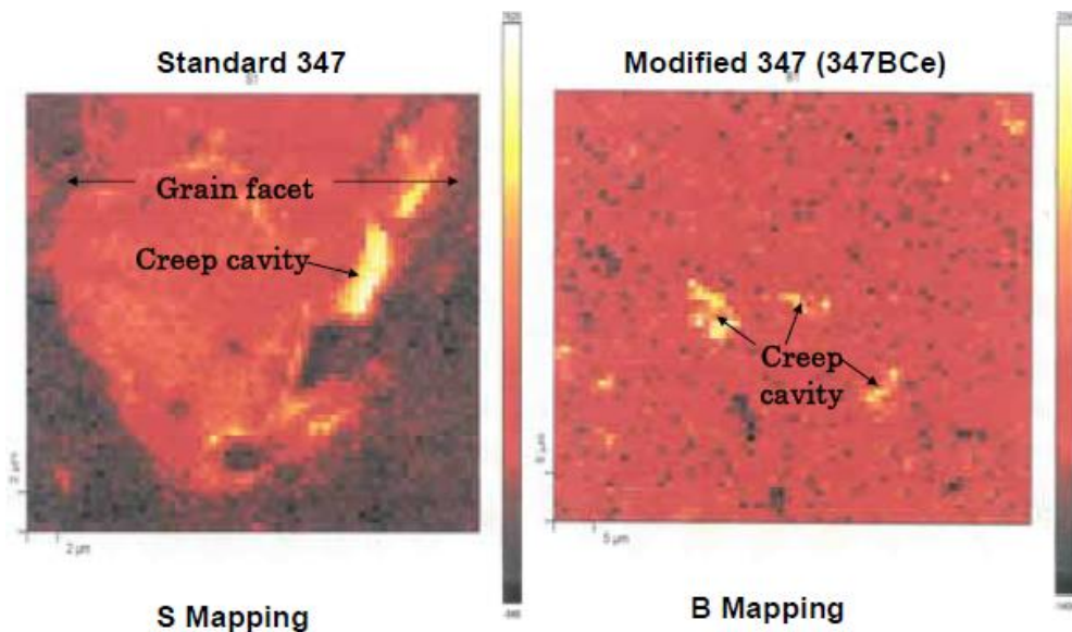
Figure 19. Auger S and B mapping of the fractured surfaces, creep exposed at 750^\circ\text{C} and 69 MPa. In standard 347 steel, extensive segregation of S is shown on creep cavity surface and slight segregation on grain boundary, and in modified 347 steel segregation of B is noticed only on creep cavity surface.
