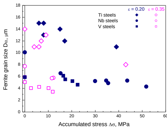
Figure 20. Ferrite grain size as a function of accumulated stress obtained at the end of hot rolling simulations carried out under different conditions of pass strain and interpass time on several low carbon microalloyed steels.
