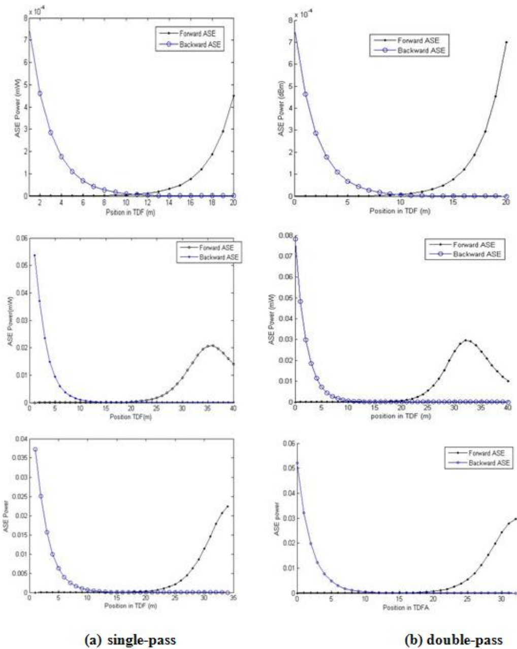
Figure 12.The forward and backward traveling ASE power against the position in TDF for both (a) single-pass and (b) double-pass TDFA.
