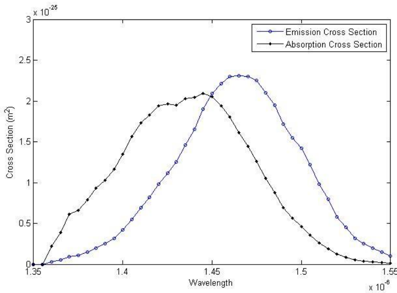
Figure 9. Emission and absorption cross-section spectra of the TDFA.
