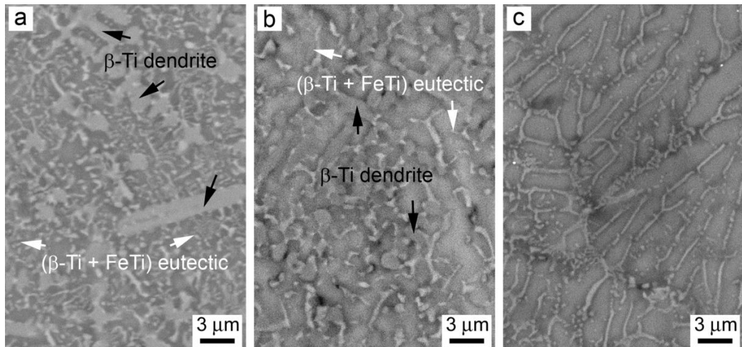
Figure 6 SEM backscattered electron images of the as-cast (\text{Ti}_{0.72}\text{Fe}_{0.28})_{100-x}\text{Ta}_x 3 mm \varnothing rods: (a) x = 0 and (b) x = 2 showing a hypoeutectic microstructure with micrometer-sized primary \beta -Ti dendritic phase embedded in an ultrafine-grained (\beta\text{-Ti} + \text{FeTi}) matrix, and (c) x = 4 showing a carcass (pseudo-hypoeutectic) microstructure.
