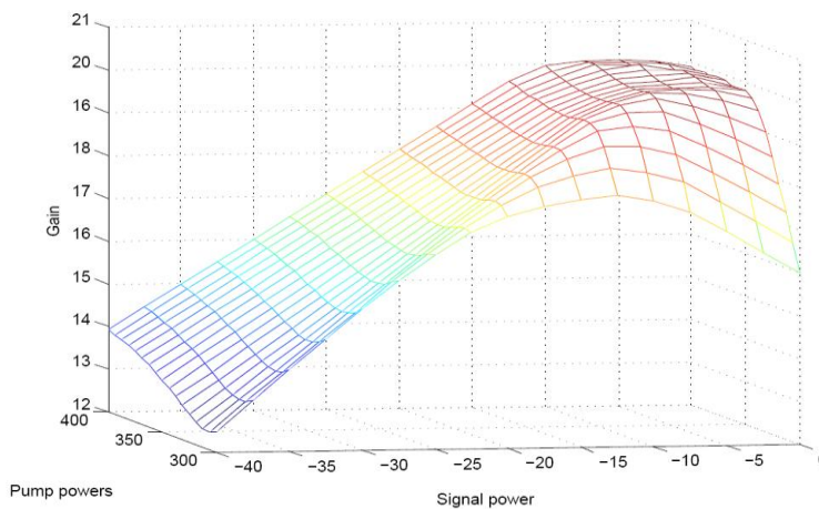
Figure 26. 3D gain characteristic as a function of pump power and signal power using a 20 m long TDF and a 1460 nm input signal wavelength.
