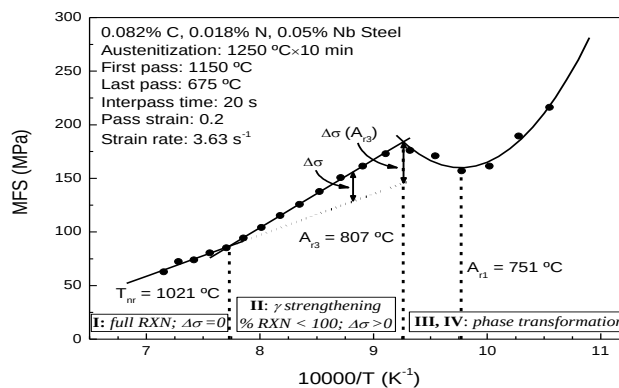
Figure 14. Dependence of Mean Flow Stress (MFS) on inverse of absolute temperature for a low carbon Nb-microalloyed steel. The no-recrystallization temperature ( T_{nr} ) is the temperature below which the recrystallization between passes starts to be incomplete.
