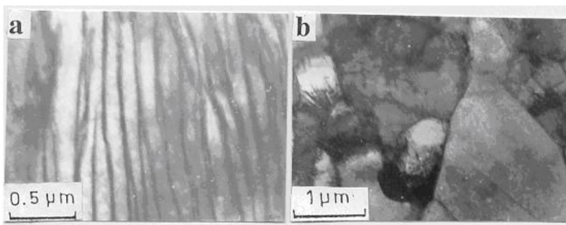
Figure 14. TEM micrographs of steel 2 deformed 50% at 800 °C showing (a) pearlite (b) non-polygonal ferrite with high dislocation density.
