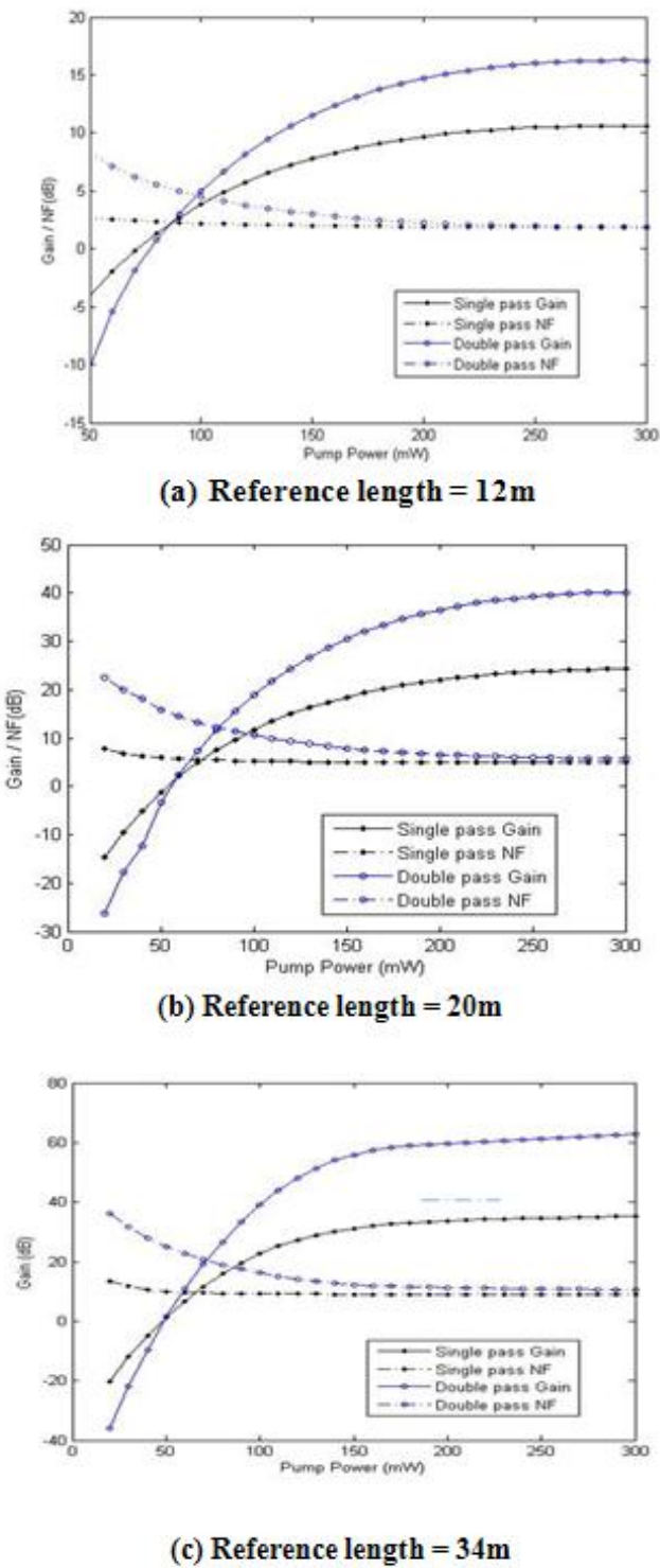
Figure 10. The gain and noise figure against pump power for both single-pass and double-pass TDFA at various reference TDF length (a) 12m (b) 20m and (3) 34m.
