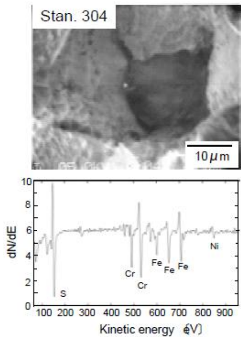
Figure 24. Scanning electron micrograph showing creep cavity surface, exposed by breaking at liquid nitrogen temperature under impact loading, of 304 steel crept for 290h ( t/tr=0.87 ) at 750°C and 63MPa, and Auger spectrum obtained from creep cavity surface.
