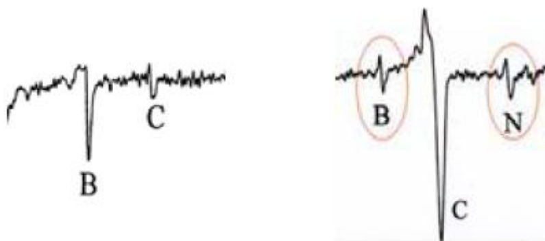
Figure 25. Scanning electron micrograph showing creep cavity surface, exposed by breaking at liquid nitrogen temperature under impact loading, of modified 304 steel crept for 10,200h ( t/t_r=0.86 ) at 750°C and 63MPa and Auger spectrum obtained from the creep cavity surface.
