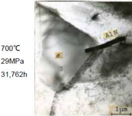
Figure 7. Rod-like AlN precipitated at \sigma phase In ruptured specimen of Heat F (Al:0.095mass%)of 316 steel.
