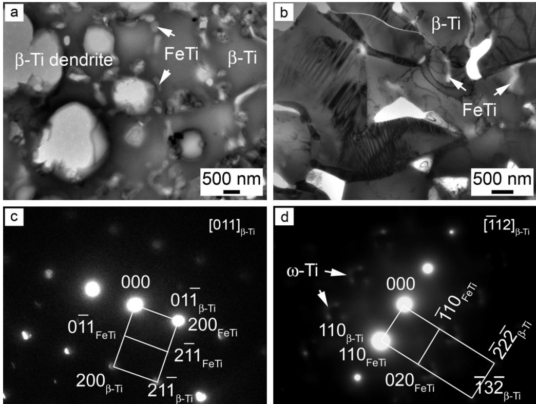
Figure 7. Bright-field TEM images of the ultrafine-grained (\text{Ti}_{0.72}\text{Fe}_{0.28})_{100-x}\text{Ta}_x alloys: (a) x = 0 and (b) x = 4 , and the corresponding SAED patterns for the eutectic matrix in: (c) x = 0 along the [011] zone axis and (d) x = 2 along the [-112] zone axis of \beta -Ti phase. The x = 2 alloy displays a similar microstructure as the x = 0 alloy.
