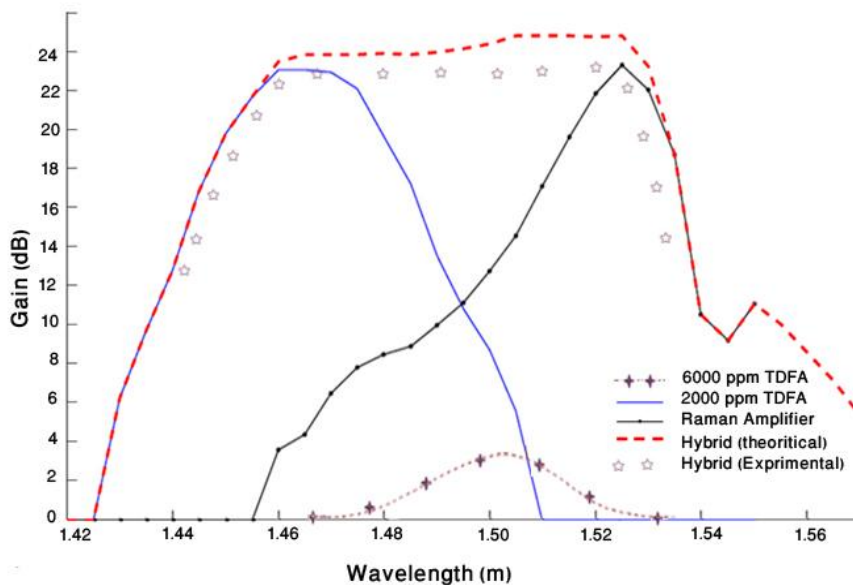
Figure 34. Gain spectra of a wideband hybrid TDFA and Raman amplifier with second stage TDFA.
