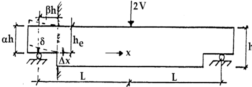
Figure 6.1. Notched beam.
