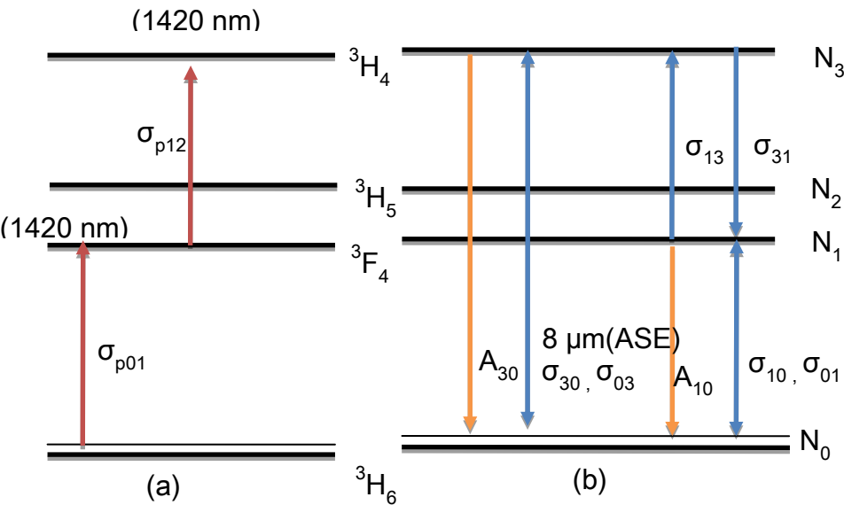
Figure 25. Pumping mechanism of a 1420nm pumped TDFA (a) absorption or pump transitions (b) signal and ASE emission transitions.
