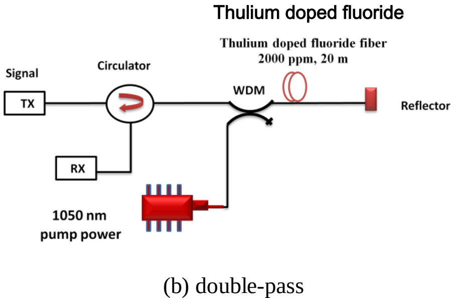
Figure 6. Configurations of the TDFA (a) single-pass (b) double-pass.
