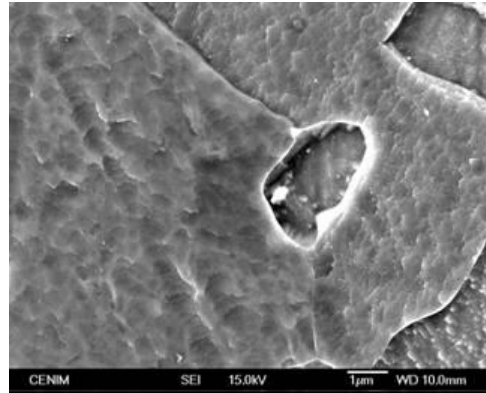
Figure 19. SEM-FEG image showing a small ferrite grain and a large VN precipitate. 0.1% C, 0.023% N, 0.151% V steel. Reheating temperature = 1230 °C x 10 min. Deformation temperature = 950 °C; \varepsilon = 0.35 ; Post-deformation holding time = 900 s.
