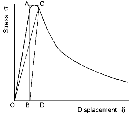
Figure3.3. Stress - displacement curve for tension, of the specimen of Figure3.1 or 3.5.
