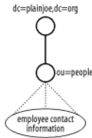
Figure 4–3. Directory namespace for company address book
