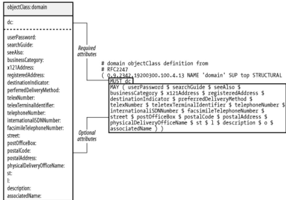
Figure 2–6. domain object class
