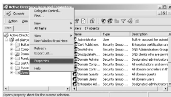
Figure 9-1. Modifying the ACL on the Users container to allow anonymous searches of user and group names
