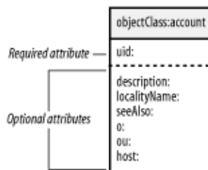
Figure 6–6. Schema for the account object class
