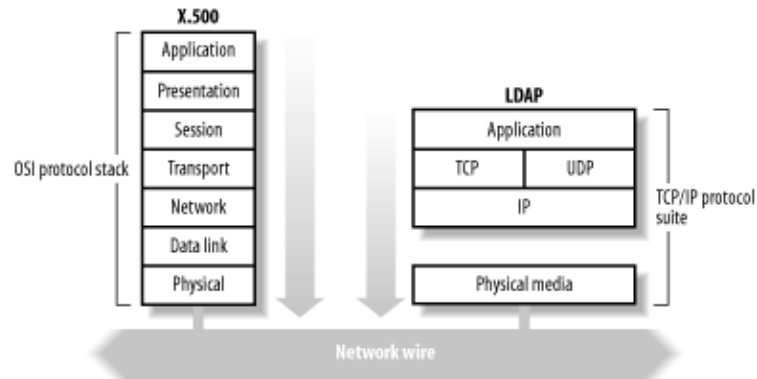
Figure 1–1. X.500 over OSI versus LDAP over TCP/IP
