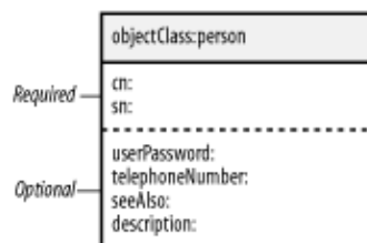
Figure 8-4. person object class
