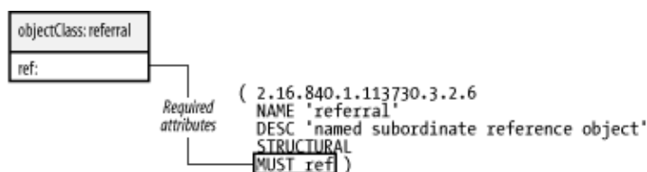
Figure 2–10. The referral object class
