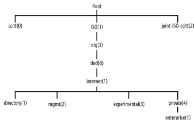
Figure 2-4. Private enterprise OID number space
