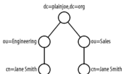
Figure 2-2. A namespace that represents Jane Smith with a unique, multivalued RDN
