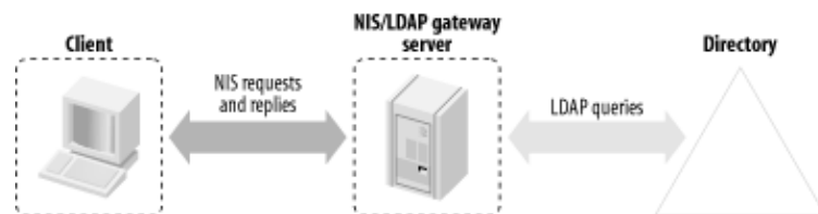
Figure 6-1. NIS/LDAP gateway
