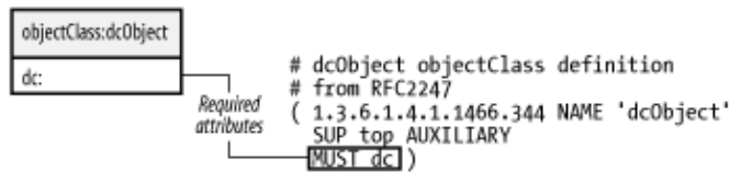
Figure 2–7. dcObject object class
