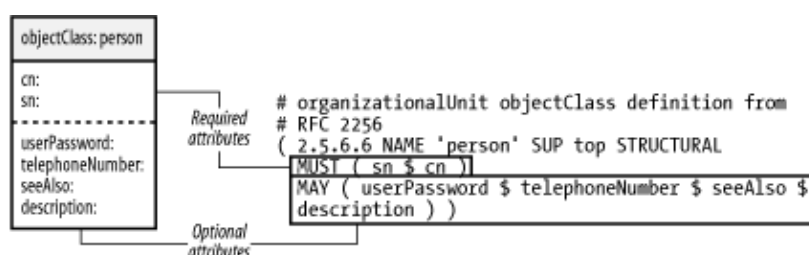
Figure 2-8. person objectClass
