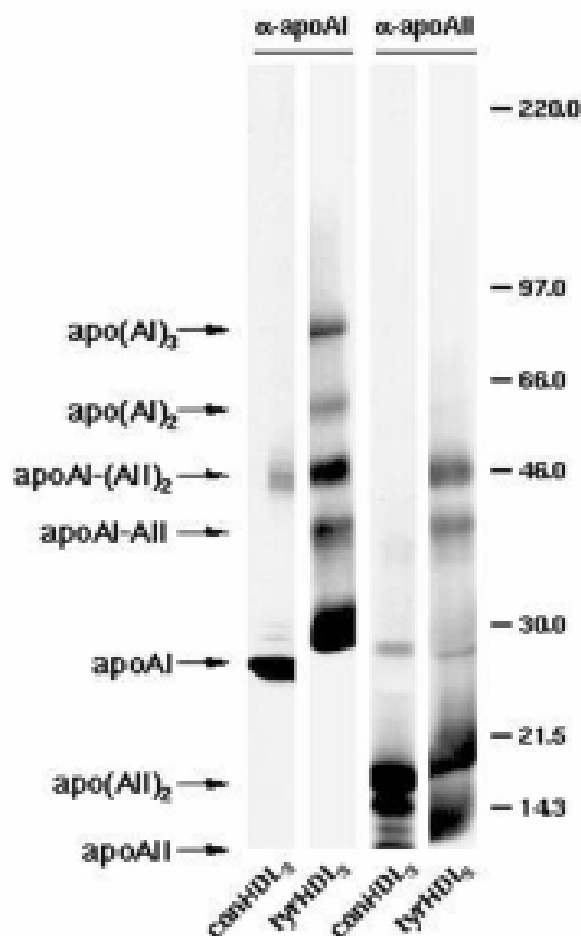
Fig. 1. Immunoblot analysis of apolipoprotein species of tyrosylated HDL. HDL (conHDL 3 ) and tyrosylated HDL (tyrHDL 3 ) proteins were separated on a 7–20% gradient SDS-PAGE gel (5 µg protein per lane) and transferred to nitrocellulose for immunoblotting with anti-apoAI (α-apoAI) or anti-apoAII (α-apoAII) antibodies (after ref. 8 ). Positions of monomeric and multimeric apoprotein species and molecular mass standards are indicated.
