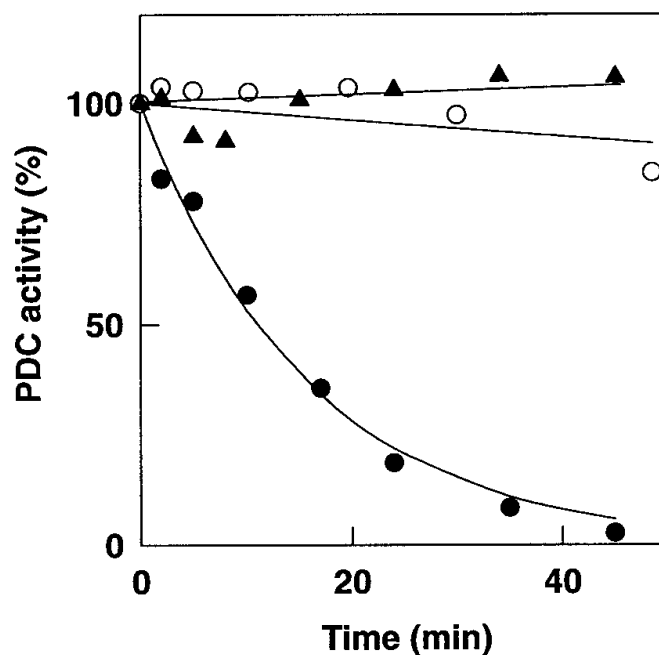
Fig. 1. Inactivation of PDC by HNE. Reconstituted PDC (16 \mu g of E1, 16 \mu g of E2-E3BP, and 8 \mu g of E3) is incubated in 80 \mu L of potassium-phosphate buffer, pH 7.5, with 0.5 mM HNE at 25° C. ○, no addition; ●, in the presence of 0.66 mM NADH; π, in the presence of 0.66 mM NADH and 3 mM cysteine. Four microliters aliquots are taken from the incubation mixture at indicated times to measure PDC activity.
