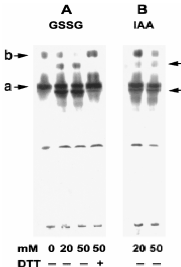
Fig. 1. The detection of hemoglobin S-glutathionylation by isoelectric focusing in erythrocytes treated with glutathione disulfide (GSSG) and iodoacetic acid (IAA). (A) 10% erythrocyte hemolysate is incubated in the presence of 0, 20, and 50 mM GSSG. (B) Erythrocytes at a hematocrit of 10% are exposed to 20 and 50 mM IAA. The incubation time with GSSG or IAA is 30 min at 37°C. Dithiothreitol (DTT, 50 mM) treatment is used to confirm that the modification is due to protein-GSH mixed disulfide formation. Arrows indicate the S-glutathionated hemoglobin. Bands a and b are hemoglobin. The bottom of the gel is the anodic side and the top of the gel is the cathodic side.
