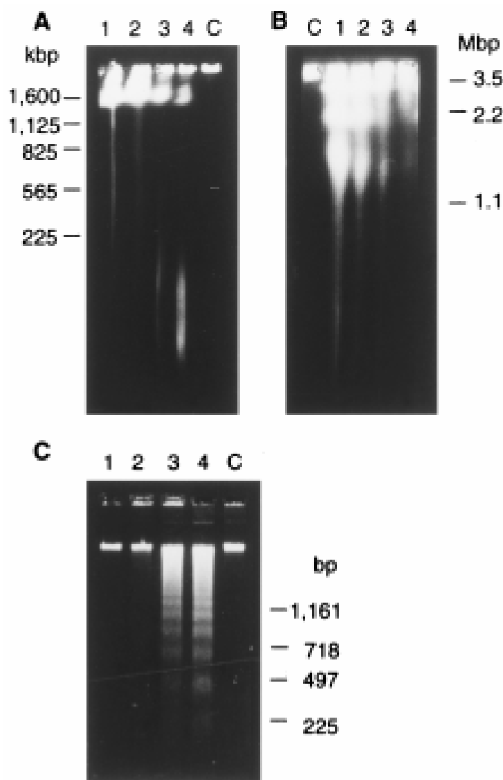
Fig. 3. PFGE ( A and B ) and AGE ( C ) analysis of double-strand DNA fragments from T-24 cells irradiated with X-ray. The cells were irradiated with 100 Gy X-ray at room temperature and then incubated with at 37°C for 0 min (lane 1), 3 h (lane 2), 10 h (lane 3), and 24 h (lane 4). Lane C shows nonirradiated and nonincubated samples. In ( A ), PFGE was carried out for 28 h at pulse time/run time of 90 s/20 h and 120 s/8 h at 175 volts. In ( B ), PFGE was carried out for 96 h at pulse time/run time 30 min/96 h, at 70 volts and after that as described for ( A ). AGE was carried out according to the method described in Subheading 3 .
