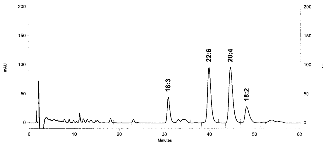
Fig. 1. Simultaneous chromatograms of LHP and LOH standards at 236 nm (A) and native unoxidized PUFA standards at 25 nm (B) . See Subheading 3.3. for HPLC conditions and Table 1 for nomenclature of peaks.
