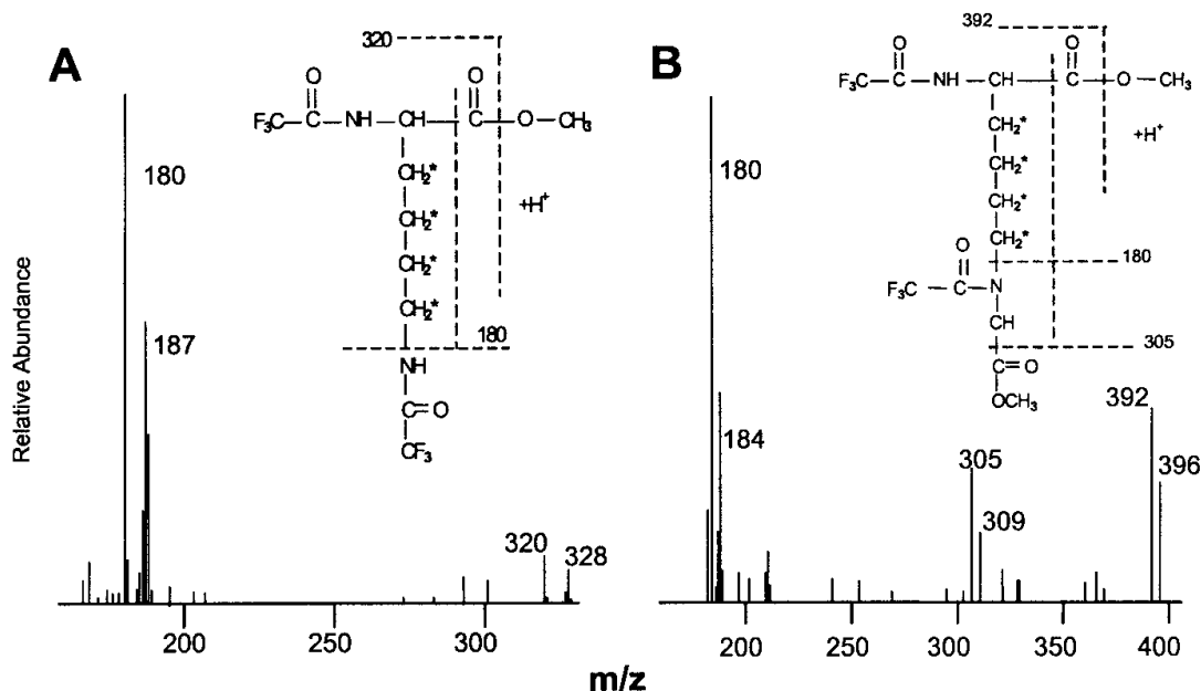
Fig. 1. Full-scan spectra of TFAME derivatives of lysine (A) and CML (B). The injected standard contained 1 \mu mol each of lysine and d_8 -lysine, and 2 nmol each of CML and d_4 -CML. Insets show fragmentation pattern. Asterisk (*) indicates heavy-labeled atoms in internal standards.
