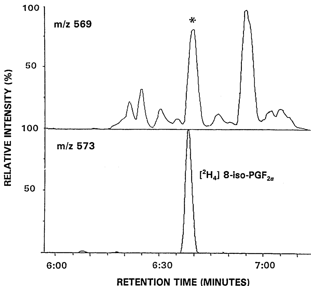
Fig. 3. Analysis of F_2 -IsoPs in plasma from a rat 4 h after treatment with \text{CCl}_4 to induce lipid peroxidation. The peak in the m/z 573 chromatogram represents the [^2\text{H}_4] 15- F_{2t} -IsoP internal standard. The peaks in the m/z 569 chromatogram represent endogenous F_2 -IsoPs. The peak denoted by the asterisk is the one routinely used to quantify the F_2 -IsoPs.
