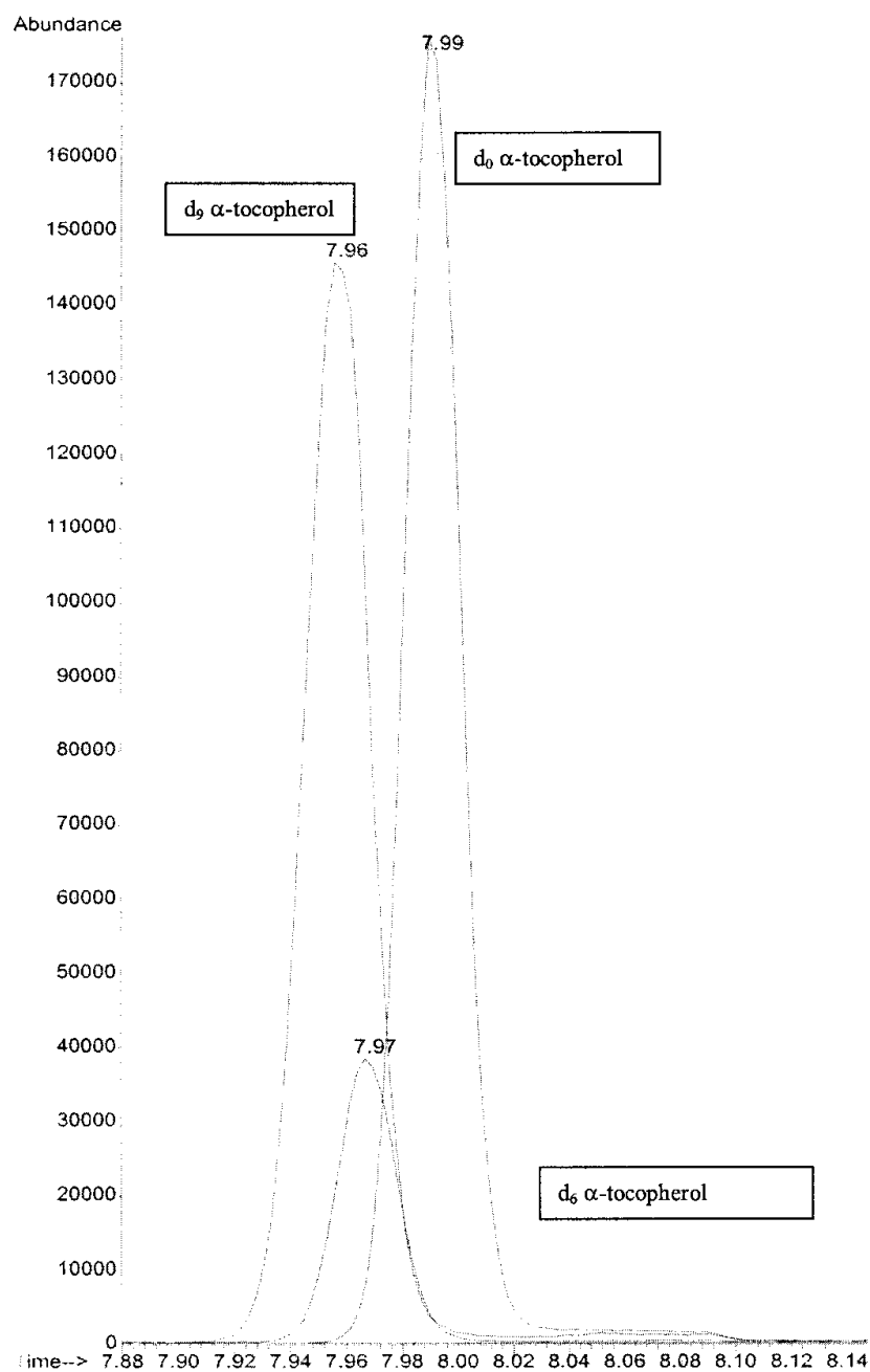
Fig. 1. Electron ionization mass spectra of silyl derivatives of d_0 , d_6 , and d_9 \alpha -tocopherol ( m/z 502, 508, and 511).
