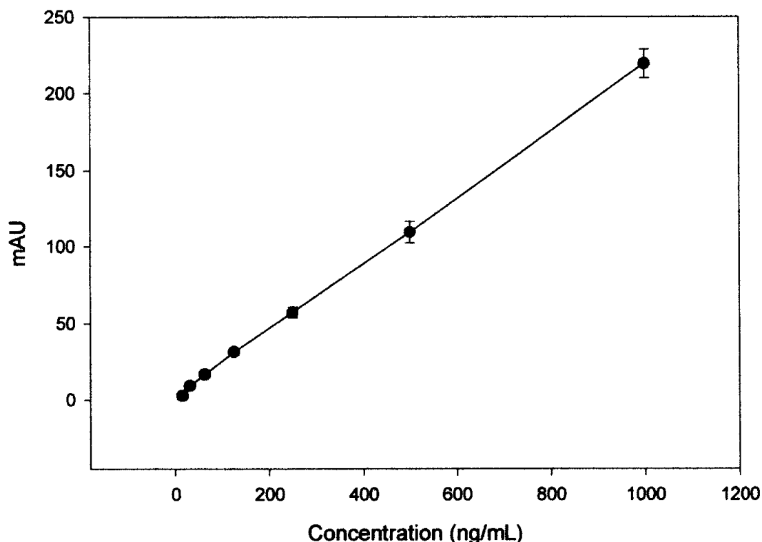
Fig. 2. A standard curve of glutamate.
