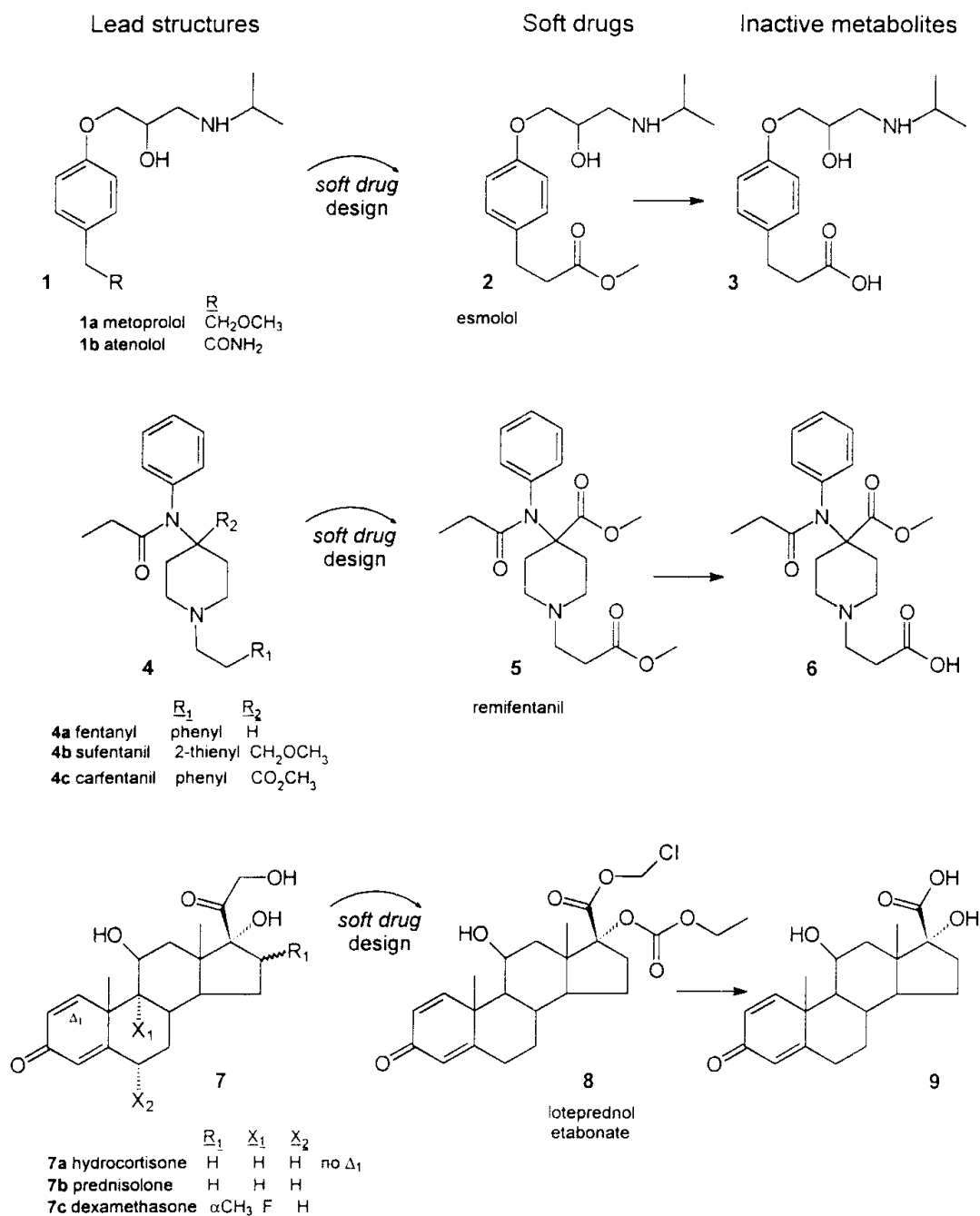
Fig. 2. Structures of esmolol ( 2 ), an ultra-short-acting \beta -blocker, remifentanil ( 5 ), an ultra-short-acting opioid analgetic, and loteprednol etabonate ( 8 ), a soft corticosteroid. For each of them, some of the corresponding (hard) lead compounds ( 1a,b , 4a–c , and 7a–c ) and the inactive metabolites resulting from the hydrolytic deactivation ( 3 , 6 , and 9 ) are also shown.
