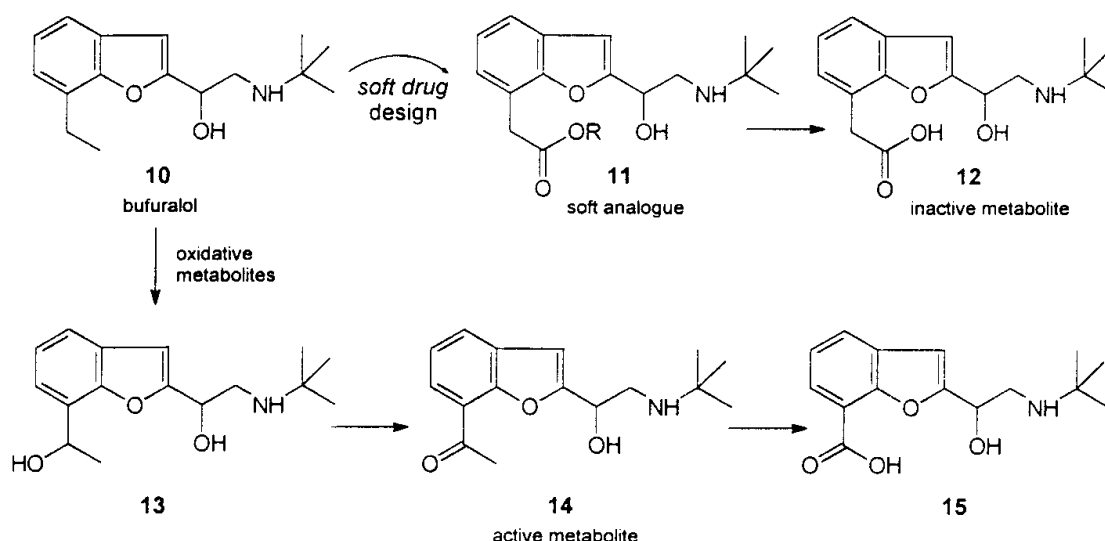
Fig. 3. Bufuralol ( 10 ), its oxidative, active metabolites ( 13 , 14 ), and the final, inactive acid ( 15 ). As the oxidative metabolites are still active and even have longer elimination half-lives, the active metabolite-based soft drug of choice should be the ketone ( 14 ), the highest active oxidative metabolite, to avoid mixtures of active components. On the other hand, starting from a hypothetical inactive metabolite ( 12 ), a variety of soft drugs ( 11 ) can be designed using the inactive metabolite-based approach that will undergo one-step hydrolytic deactivation.
